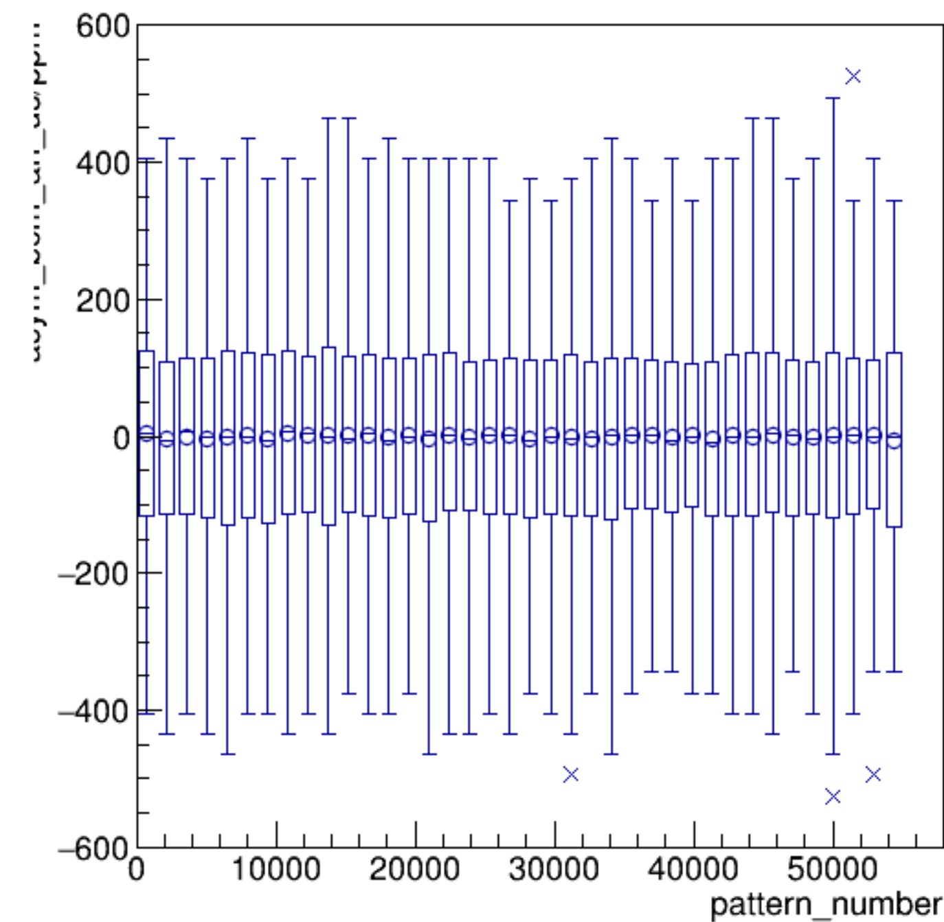
asym_bcm_an_us/ppm:pattern_number {ErrorFlag==0}
