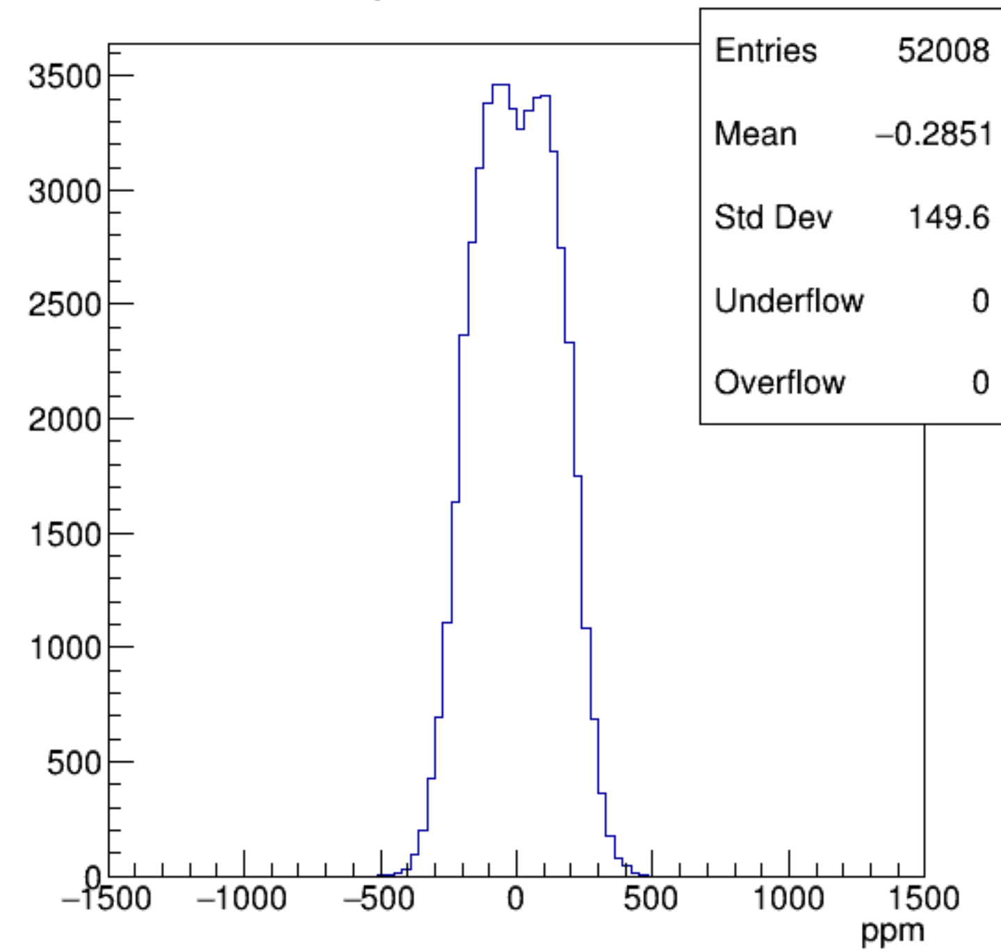
asym_bcm_an_us
