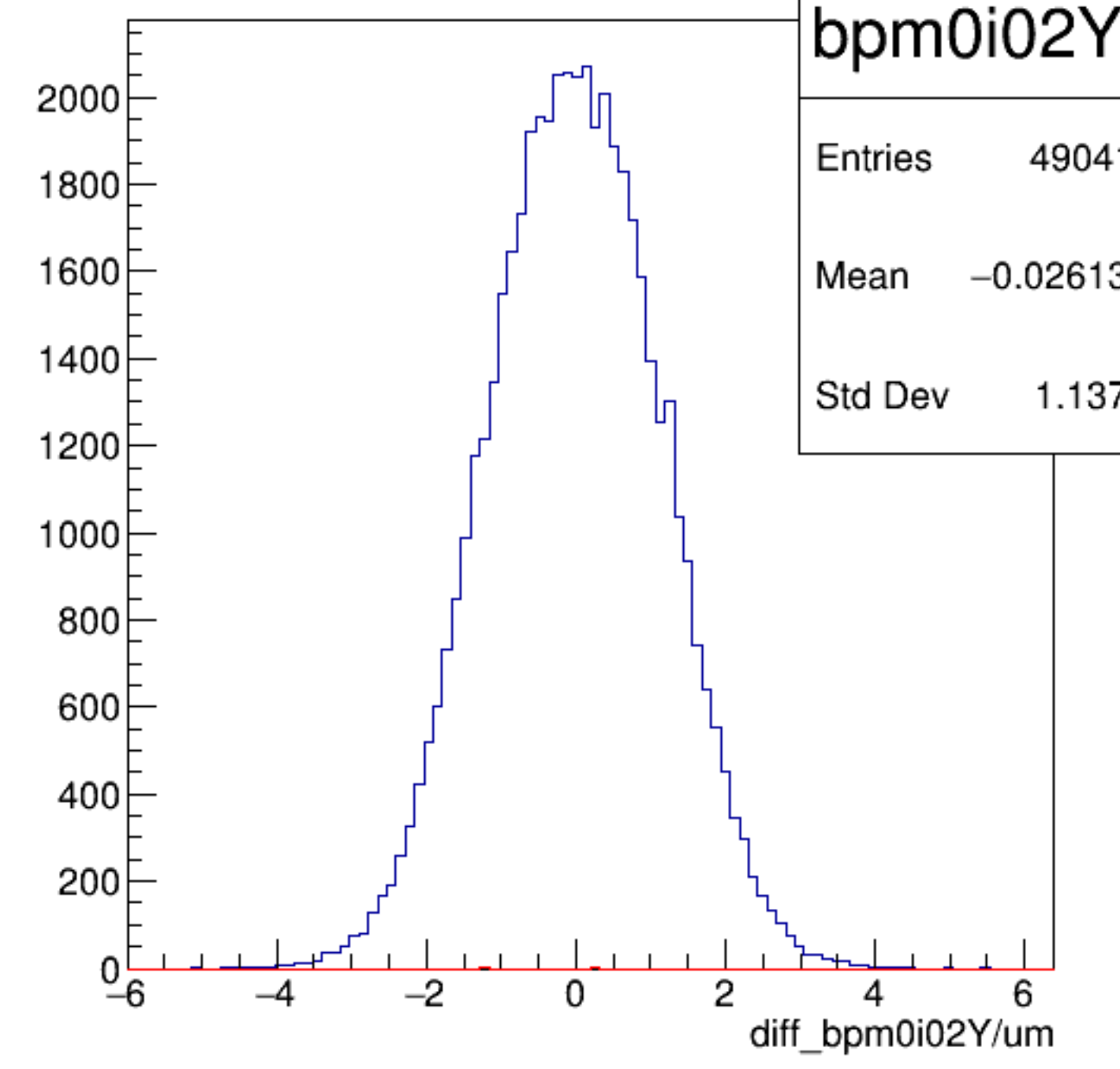
diff_bpm0i02Y/um {ErrorFlag==0}
