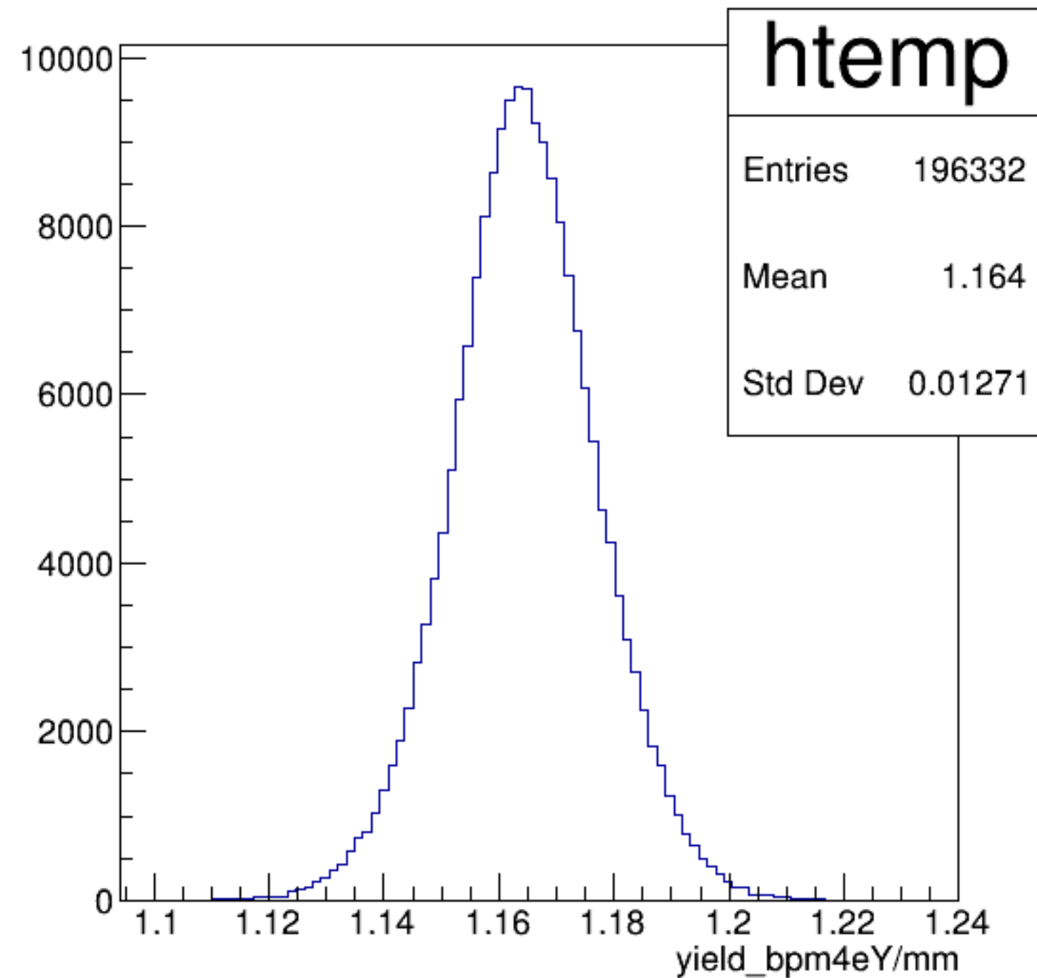
yield_bpm4eY/mm {ErrorFlag==0}
