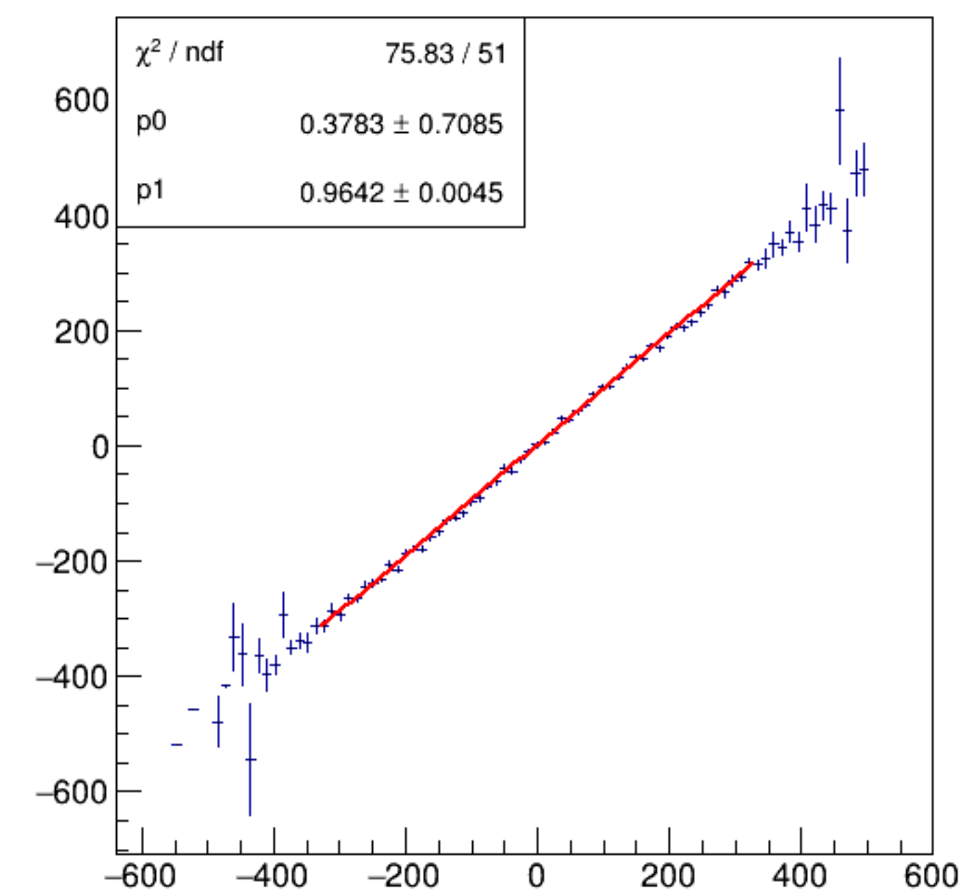
asym_bpm4acWS/ppm:Aq/ppm {ErrorFlag==0}
