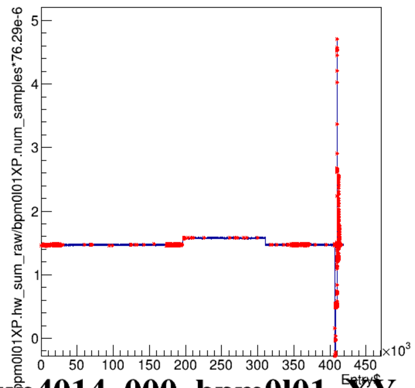
bpm0l01XP.hw_sum_raw/bpm0l01XP.num_samples*76.29e-6:Entry$
