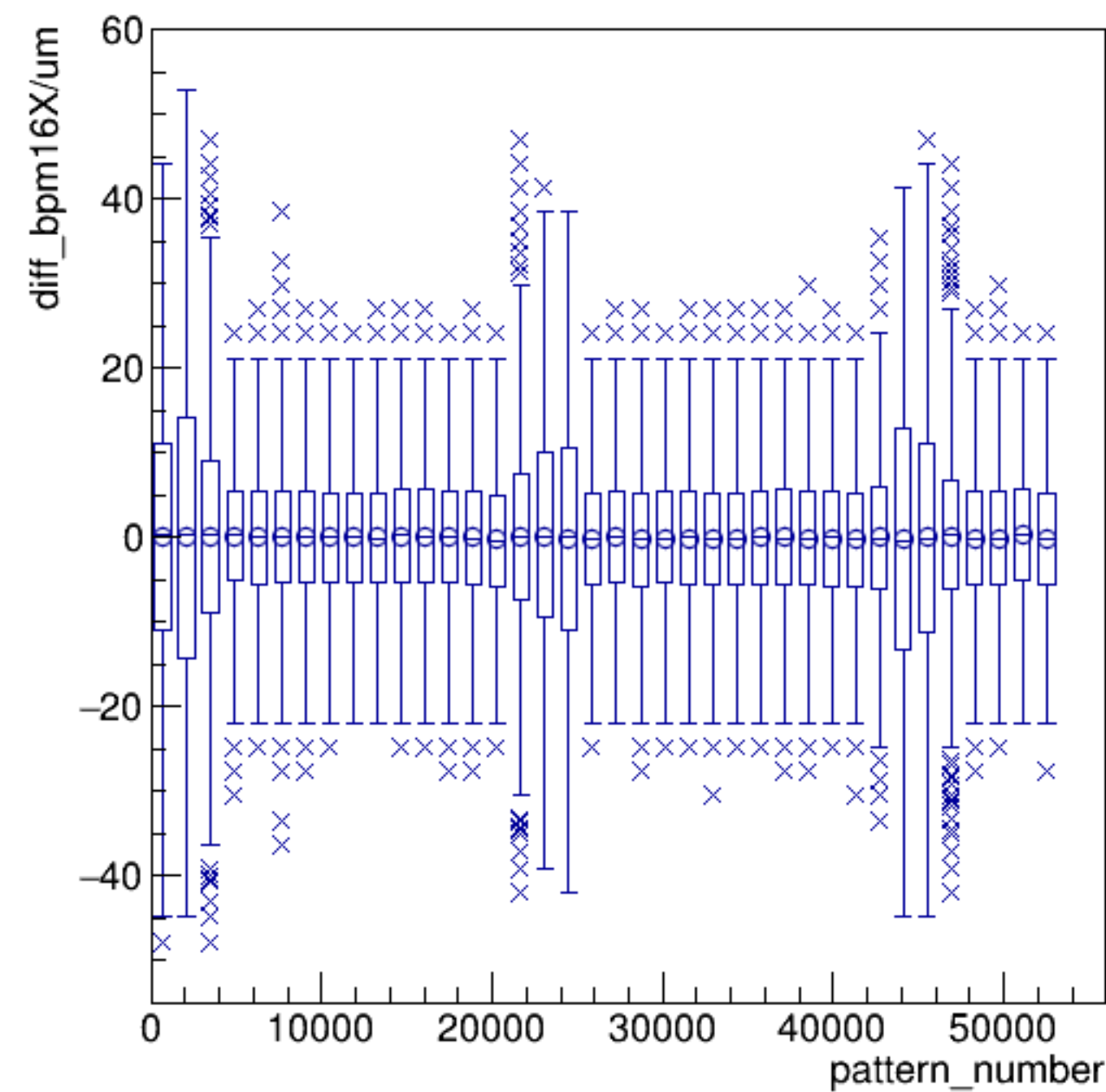
diff_bpm16X/um:pattern_number {ErrorFlag==0}
