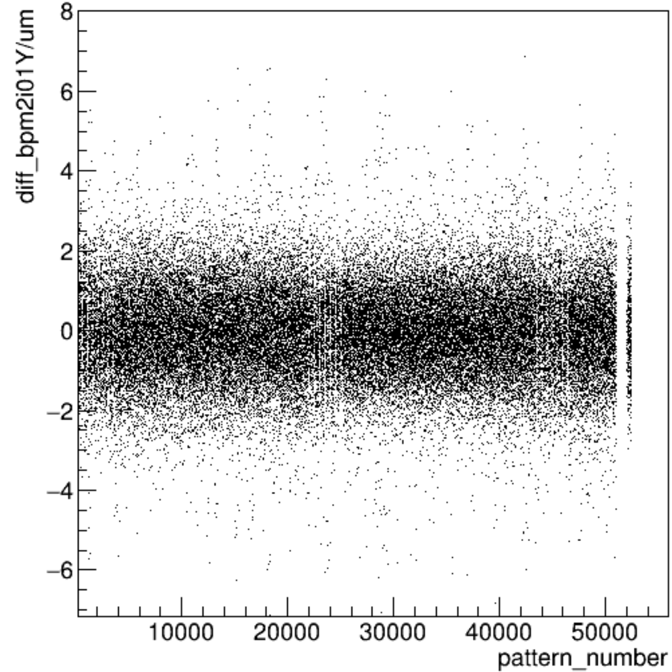
diff_bpm2i01Y/um:pattern_number {ErrorFlag==0}
