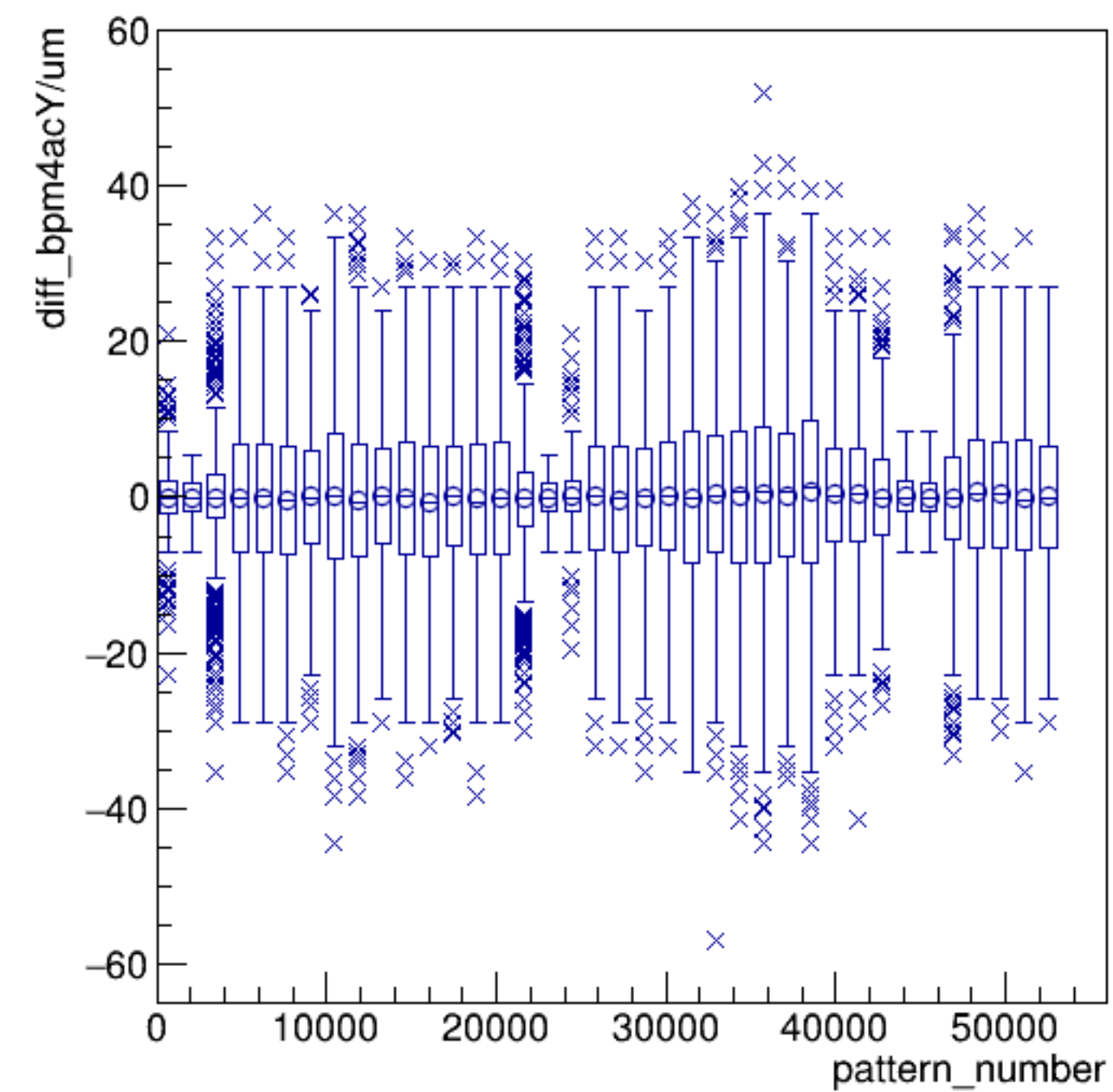
diff_bpm4acY/um:pattern_number {ErrorFlag==0}
