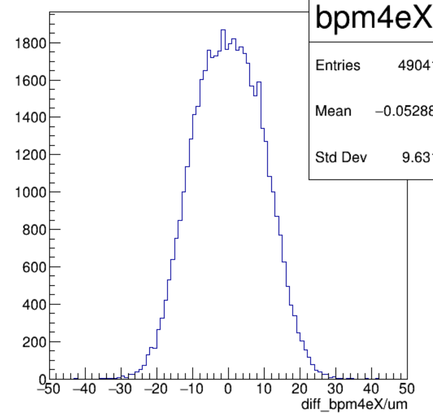
diff_bpm4eX/um {ErrorFlag==0}
