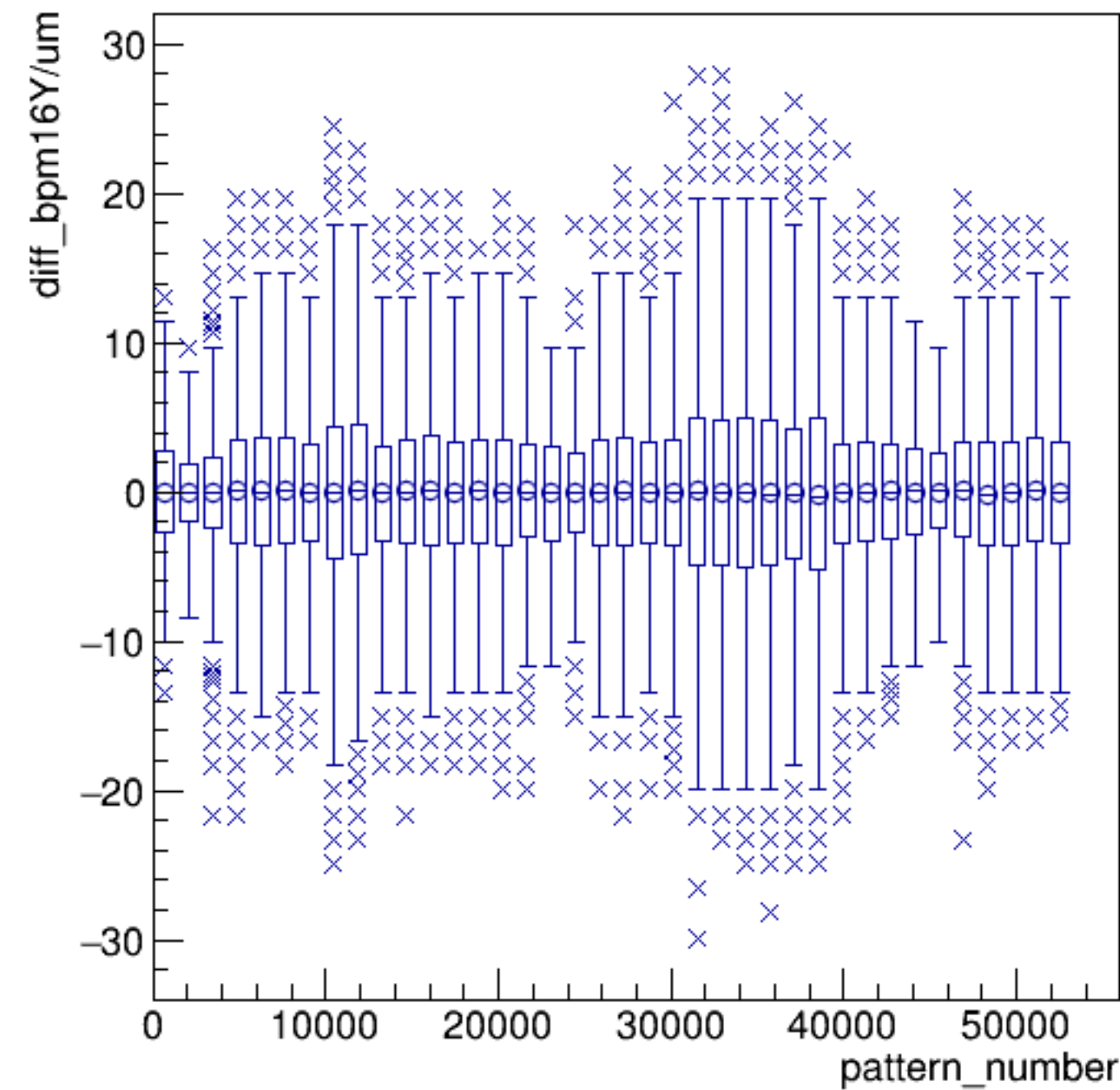
diff_bpm16Y/um:pattern_number {ErrorFlag==0}
