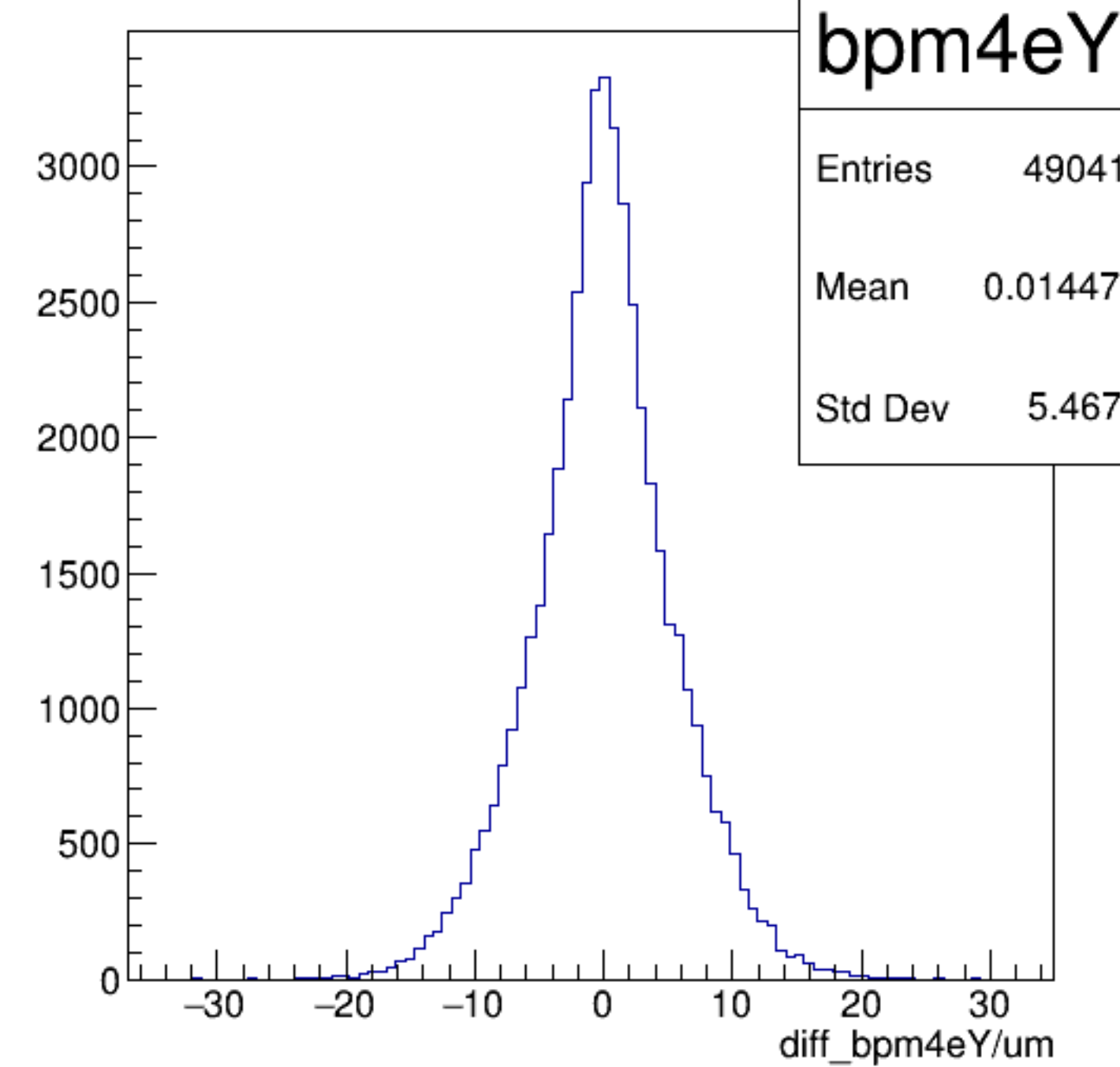
diff_bpm4eY/um {ErrorFlag==0}
