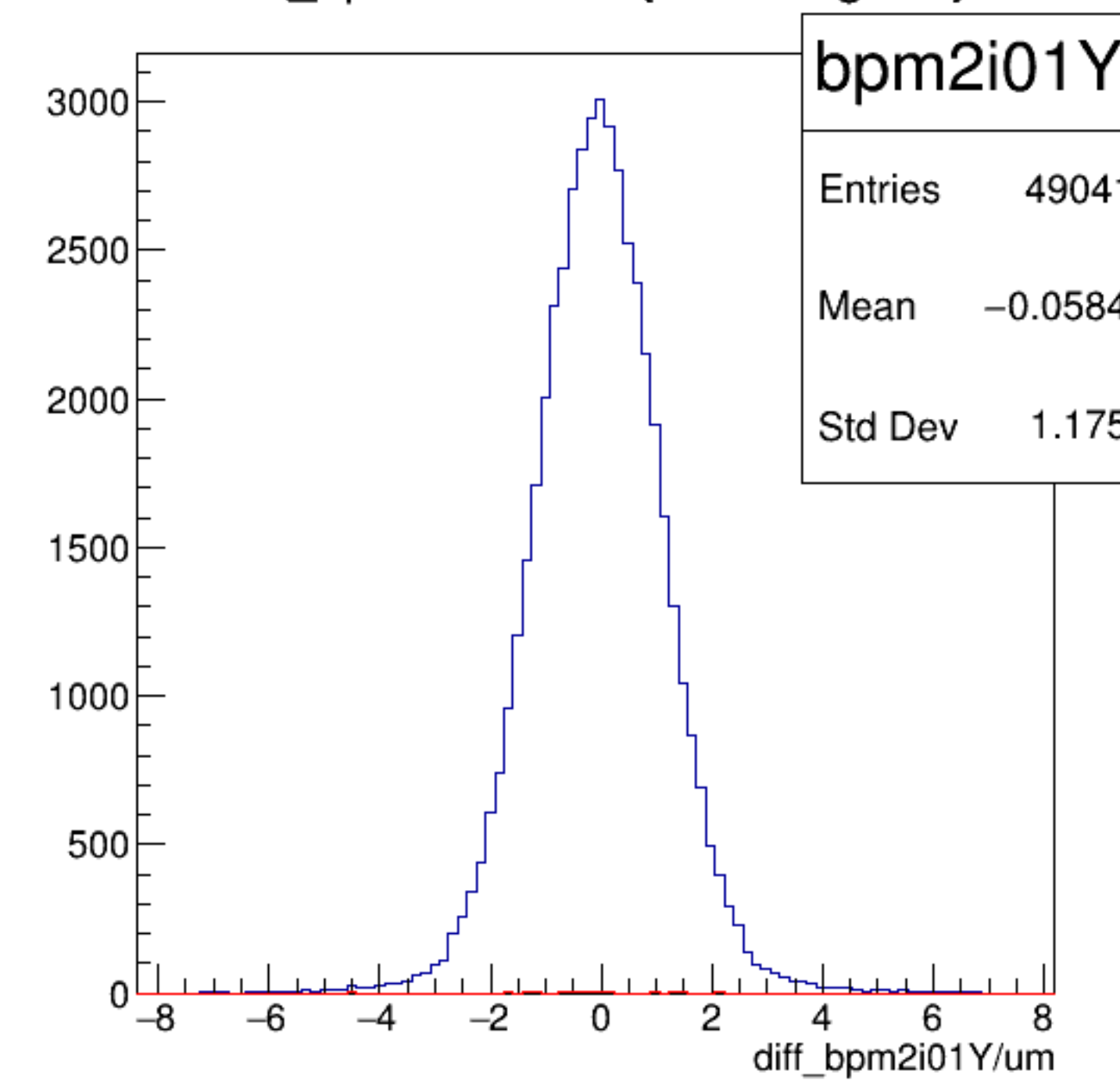
diff_bpm2i01Y/um {ErrorFlag==0}
