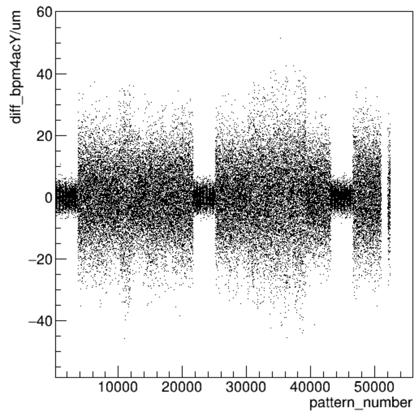
diff_bpm4acY/um:pattern_number {ErrorFlag==0}
