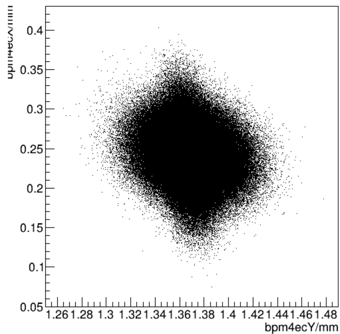
bpm4ecX/mm:bpm4ecY/mm {ErrorFlag==0}
