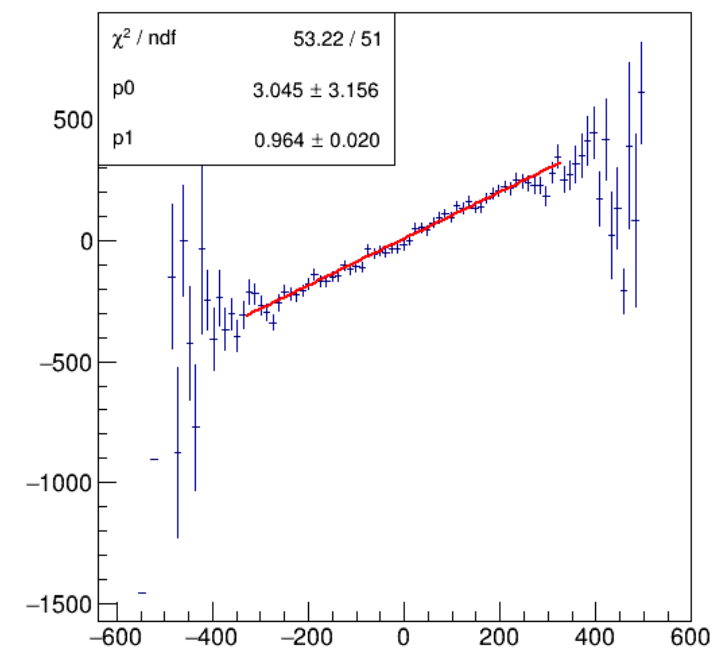
asym_bpm4ecWS/ppm:Aq/ppm {ErrorFlag==0}
