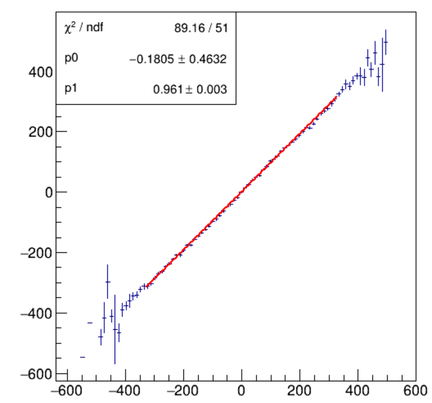
asym_bpm4eWS/ppm:Aq/ppm {ErrorFlag==0}
