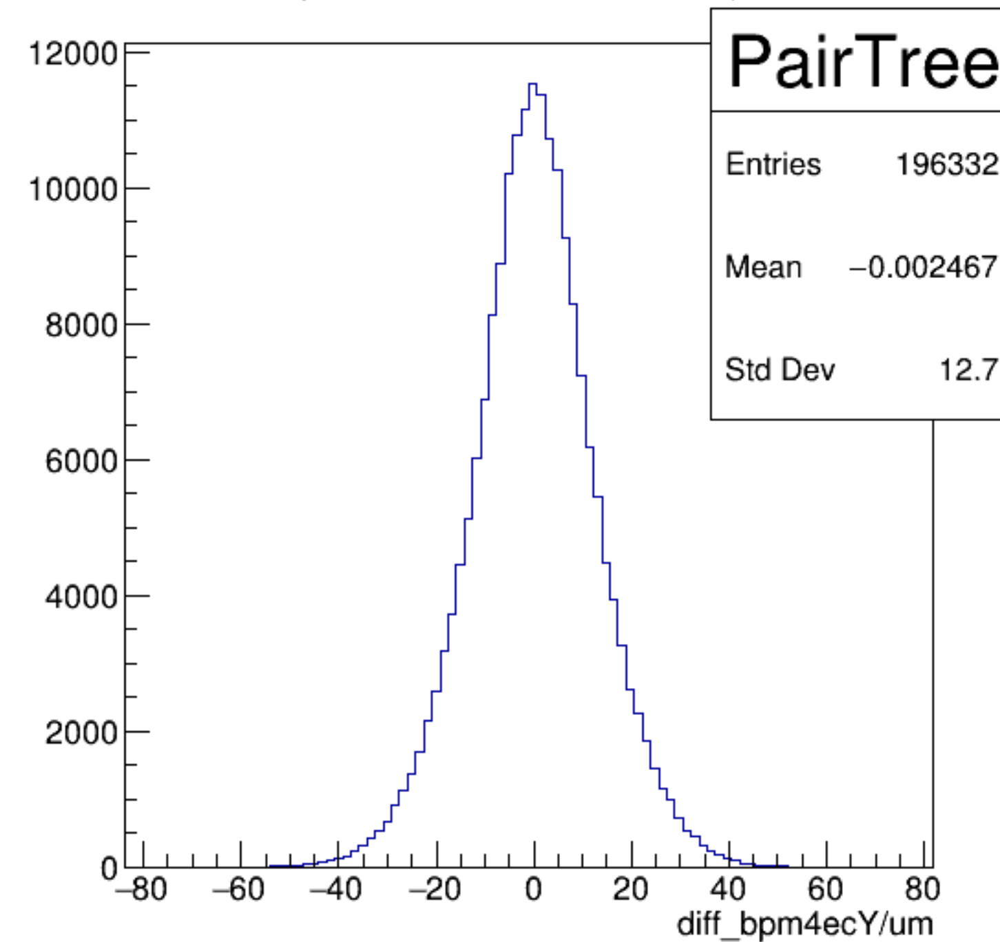
diff_bpm4ecY/um {ErrorFlag==0}
