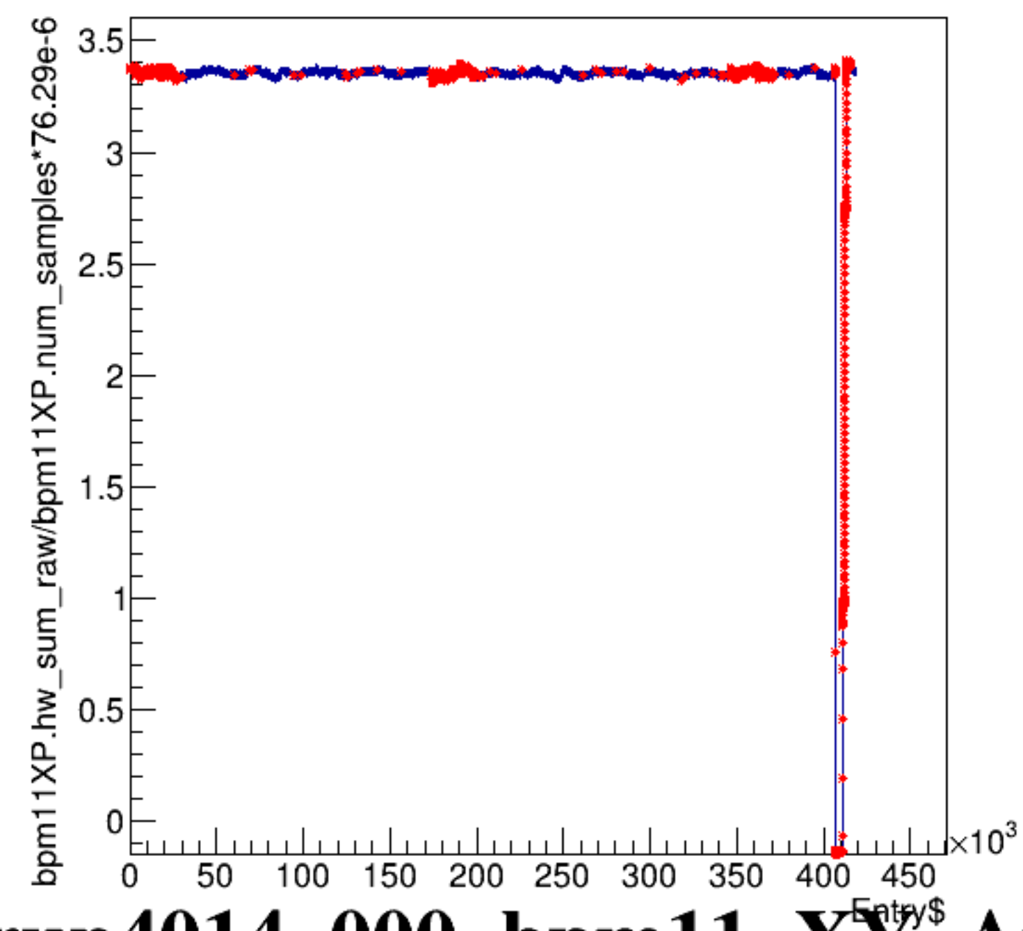
bpm11XP.hw_sum_raw/bpm11XP.num_samples*76.29e-6:Entry$
