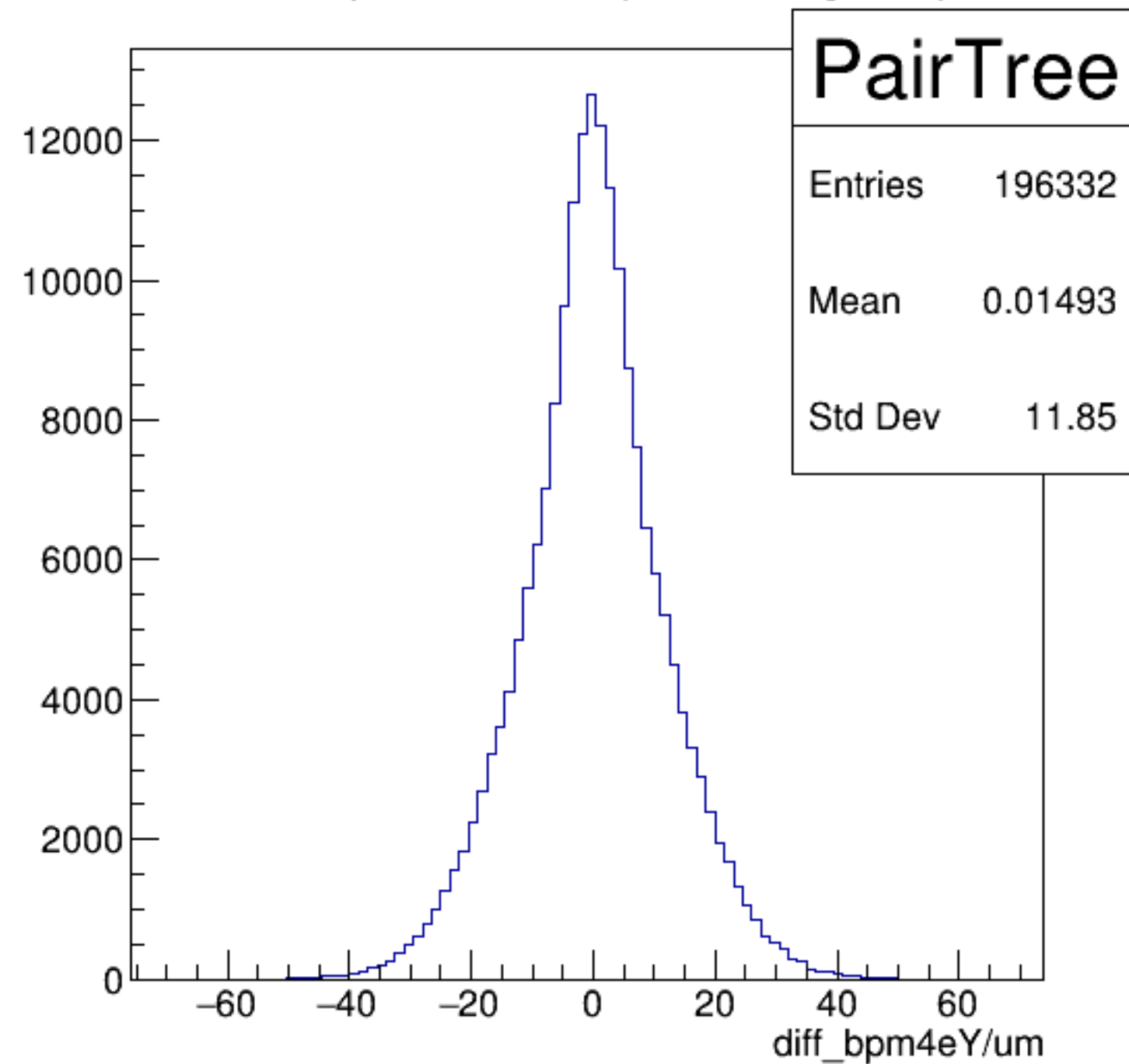
diff_bpm4eY/um {ErrorFlag==0}
