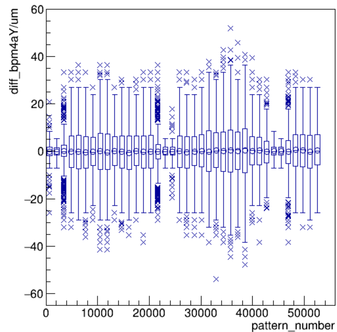
diff_bpm4aY/um:pattern_number {ErrorFlag==0}
