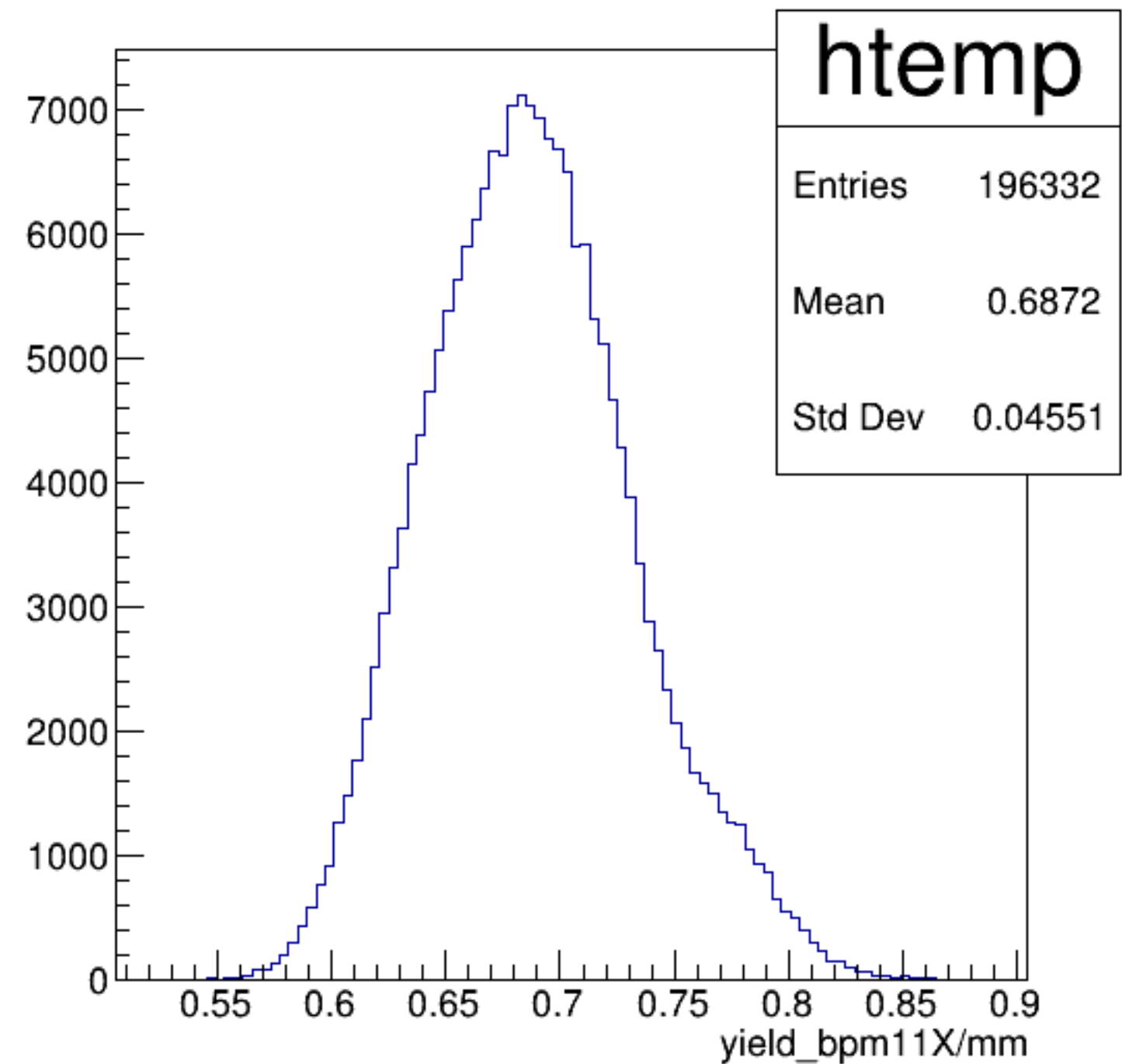
yield_bpm11X/mm {ErrorFlag==0}
