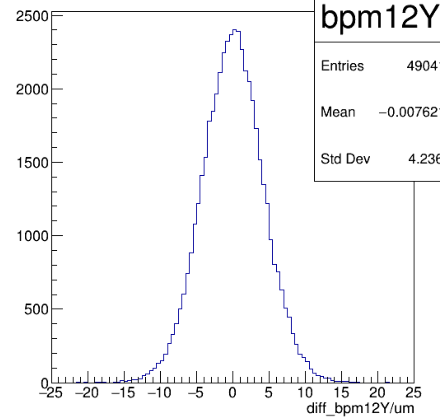
diff_bpm12Y/um {ErrorFlag==0}
