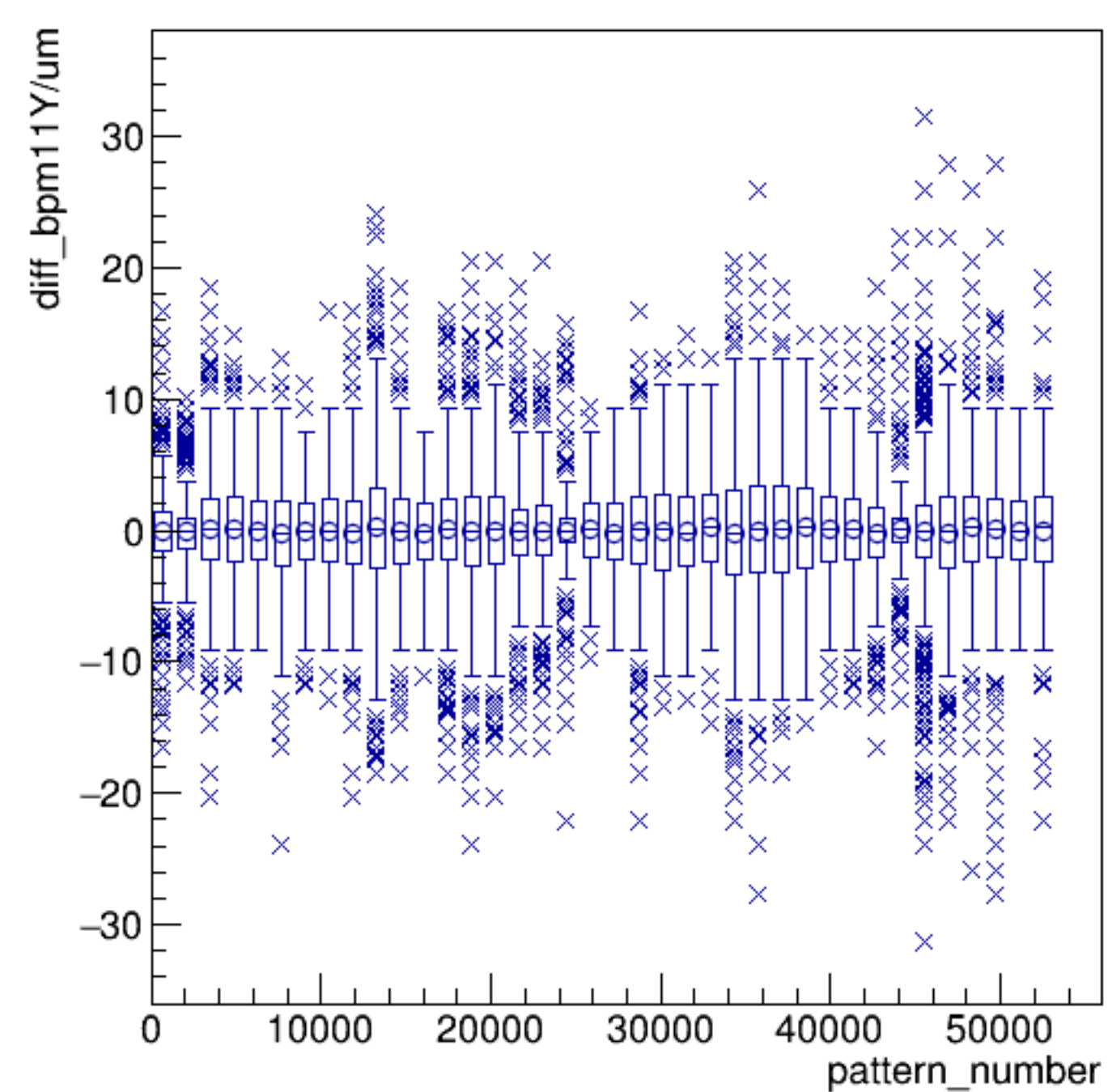
diff_bpm11Y/um:pattern_number {ErrorFlag==0}
