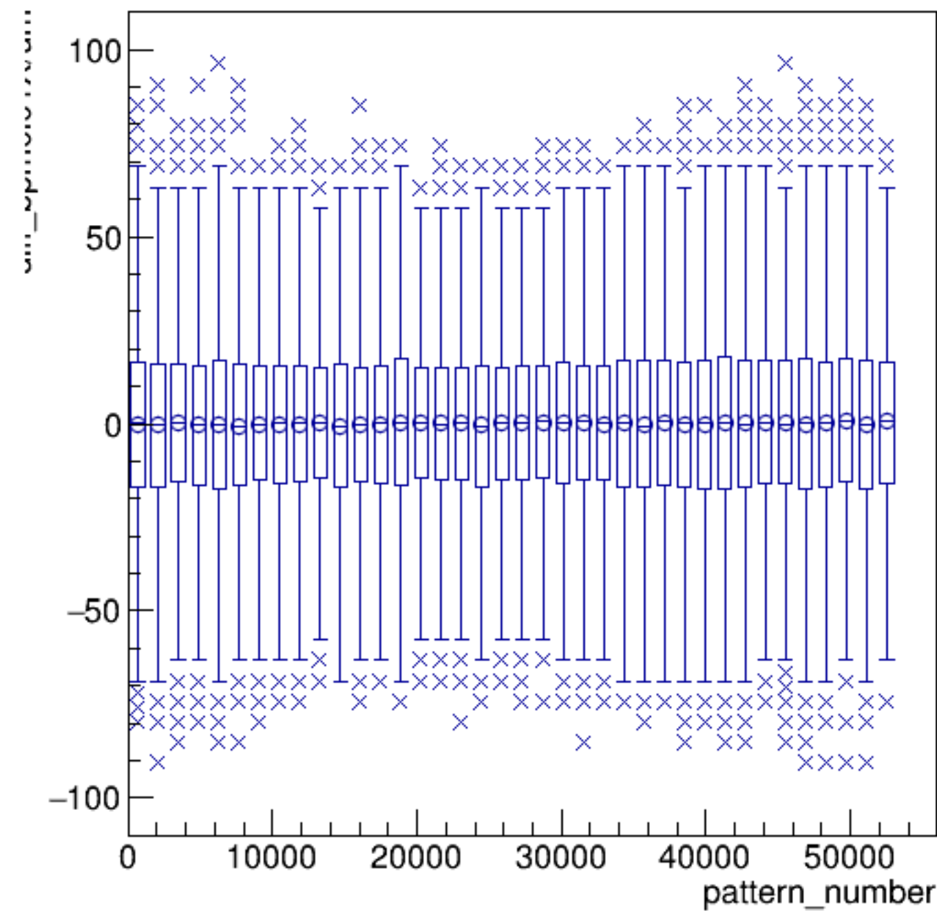
diff_bpm0l01X/um:pattern_number {ErrorFlag==0}
