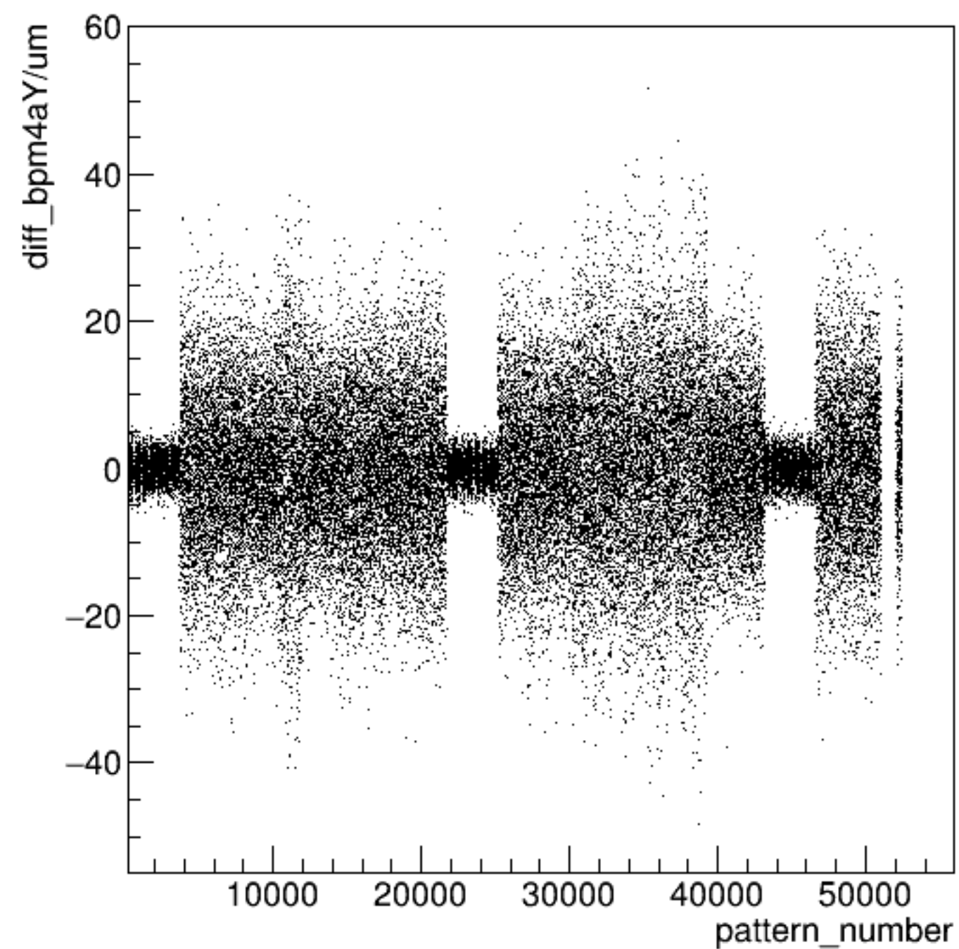
diff_bpm4aY/um:pattern_number {ErrorFlag==0}
