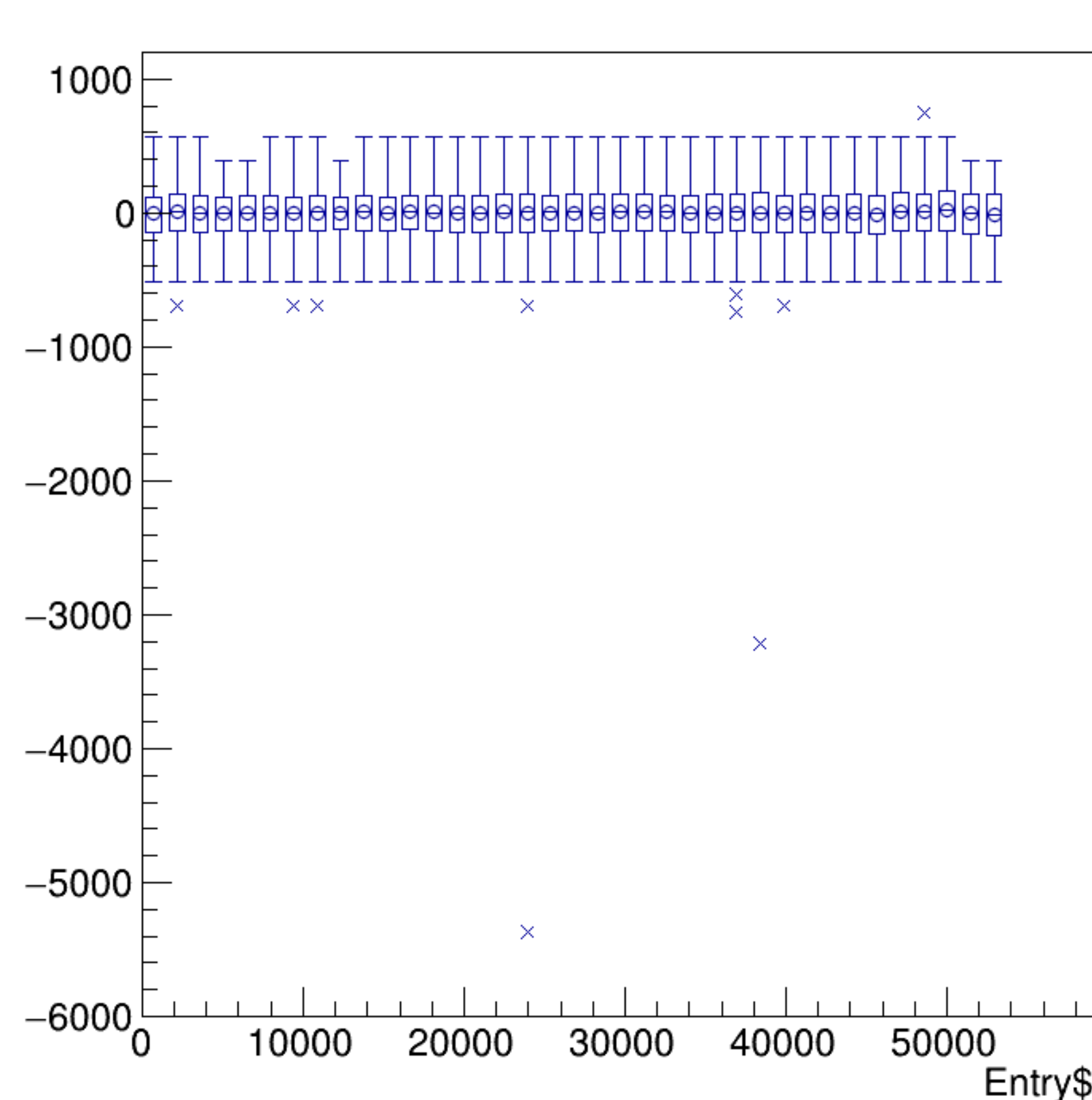
asym_bpm0l01WS/ppm:Entry$ {ErrorFlag==0}
