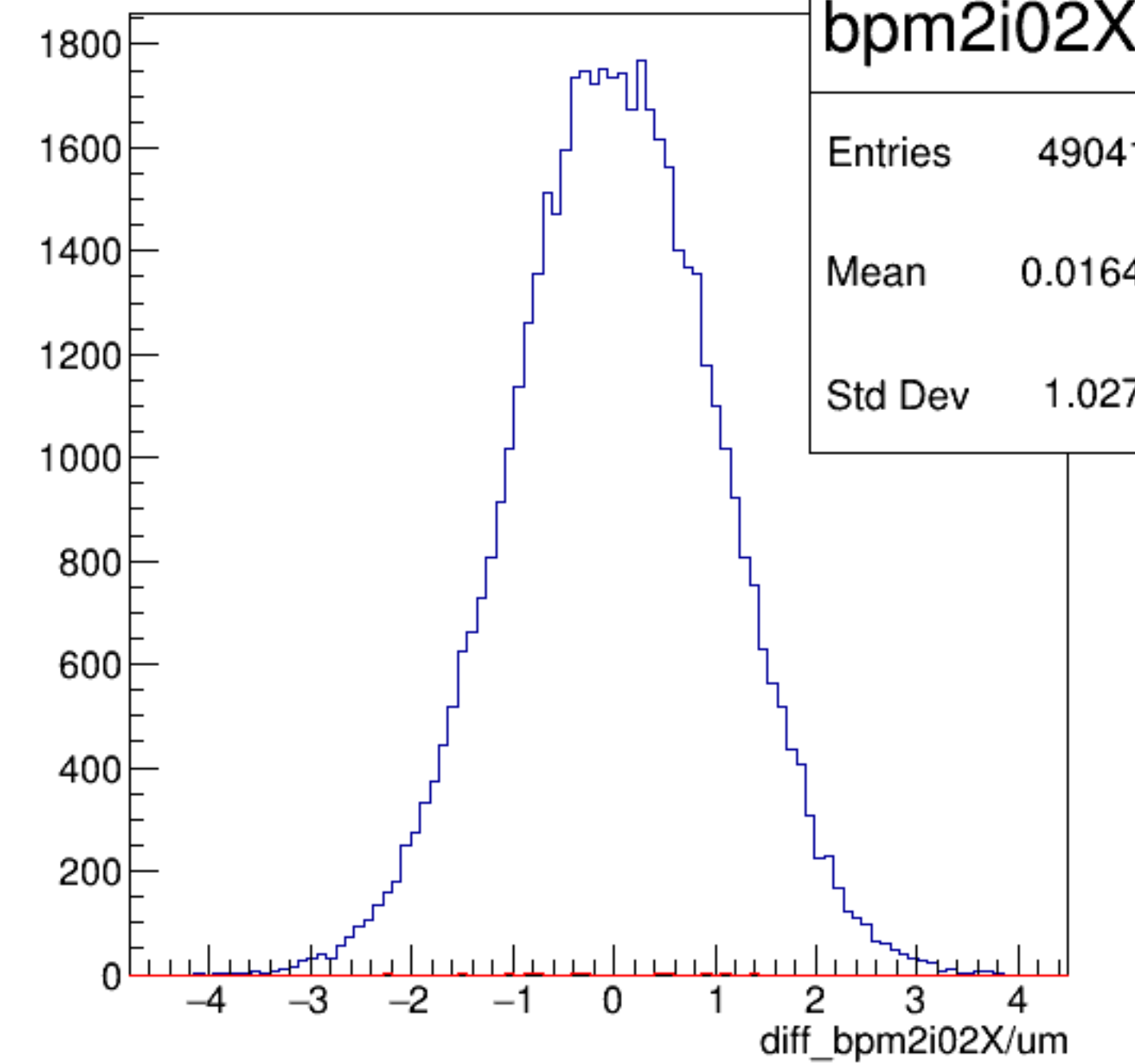
diff_bpm2i02X/um {ErrorFlag==0}
