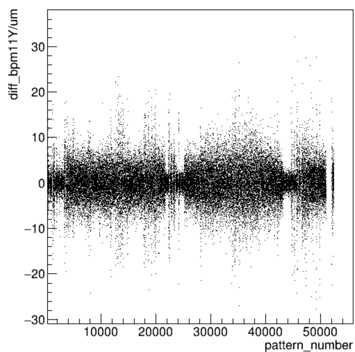
diff_bpm11Y/um:pattern_number {ErrorFlag==0}
