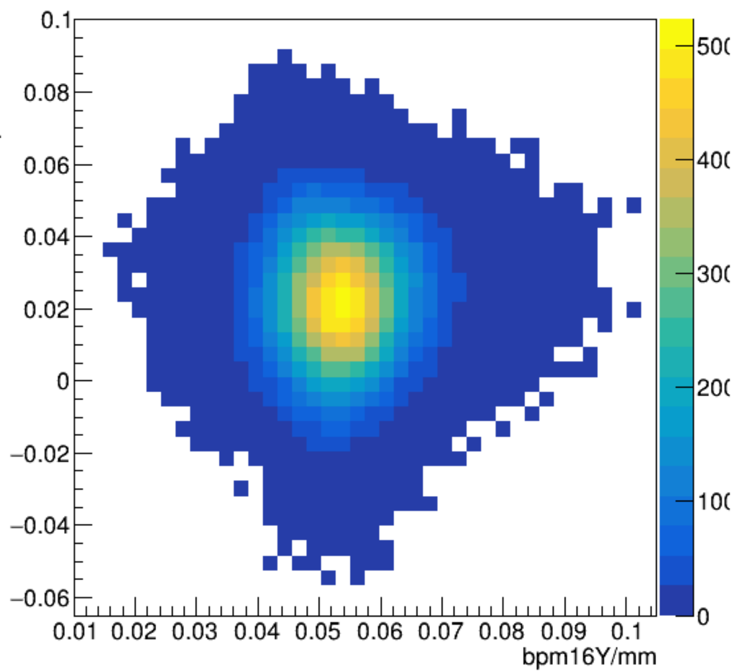
bpm16X/mm:bpm16Y/mm {ErrorFlag==0}
