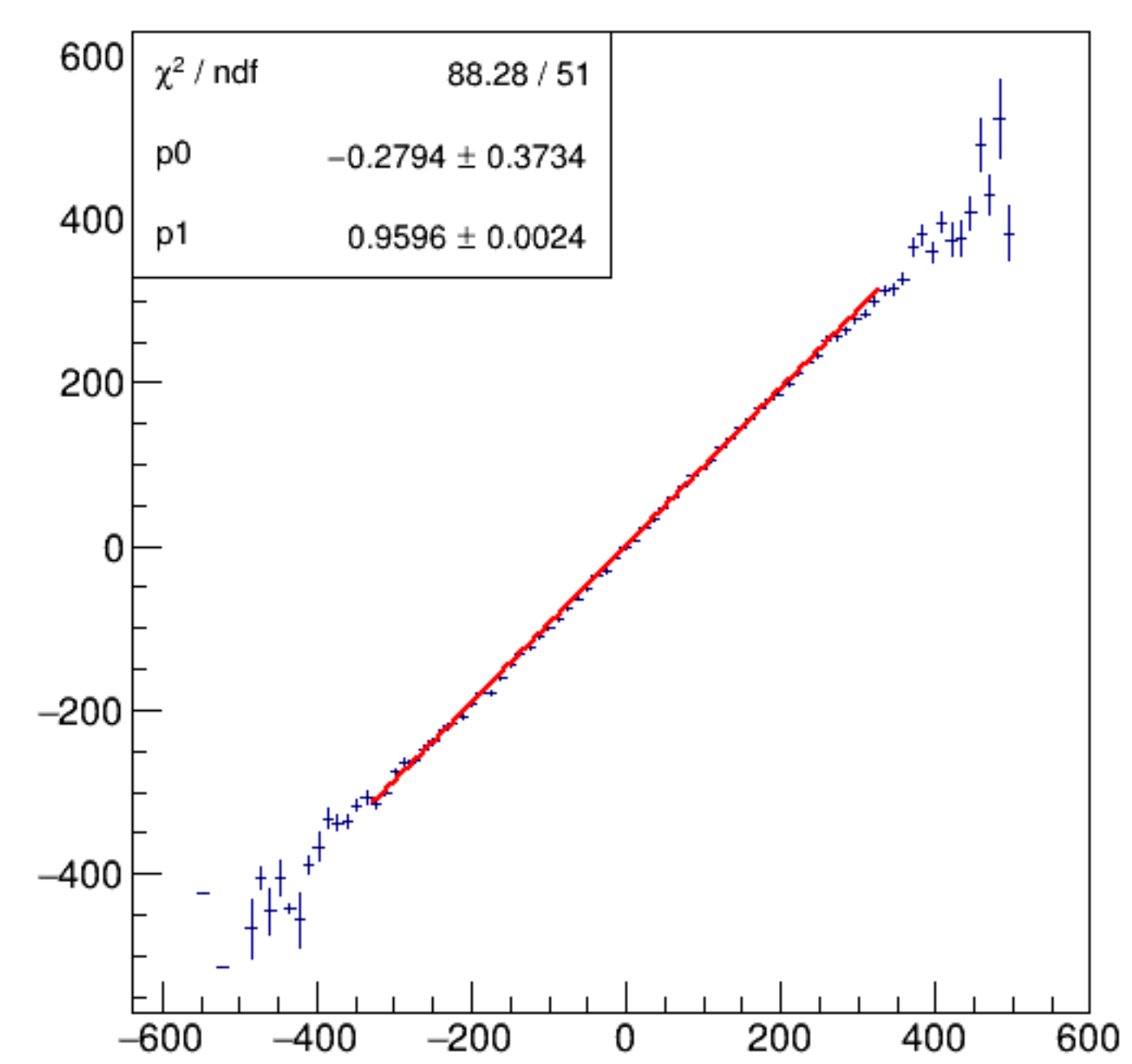
asym_bpm16WS/ppm:Aq/ppm {ErrorFlag==0}
