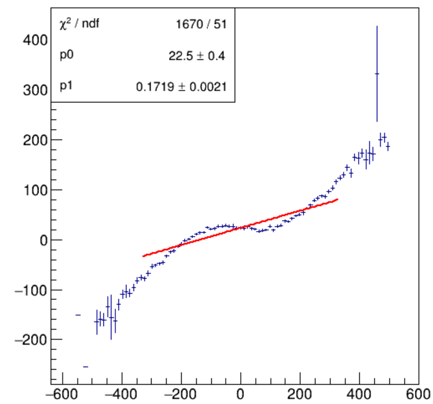
asym_bpm2i01WS/ppm:Aq/ppm {ErrorFlag==0}
