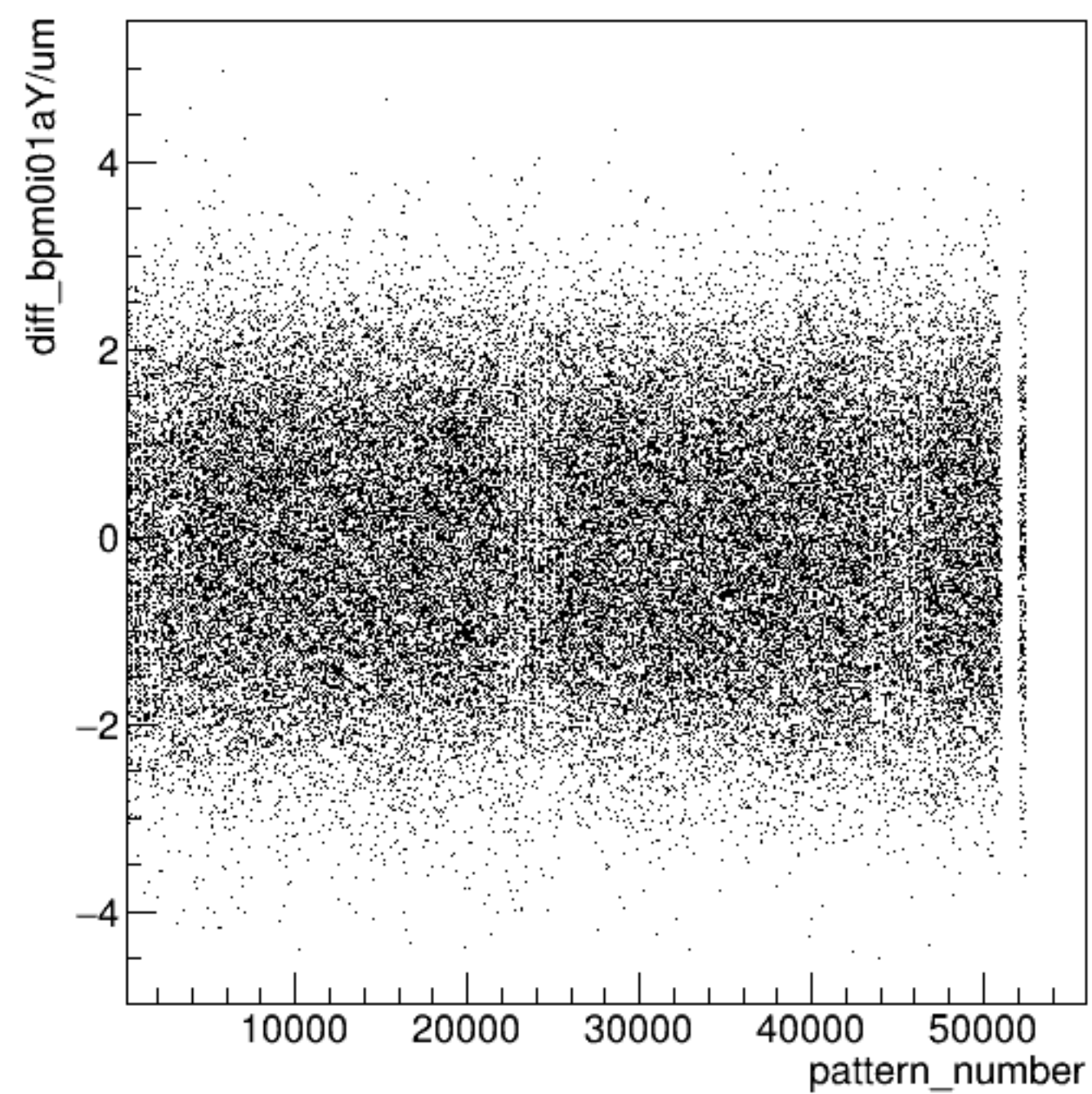
diff_bpm0i01aY/um:pattern_number {ErrorFlag==0}
