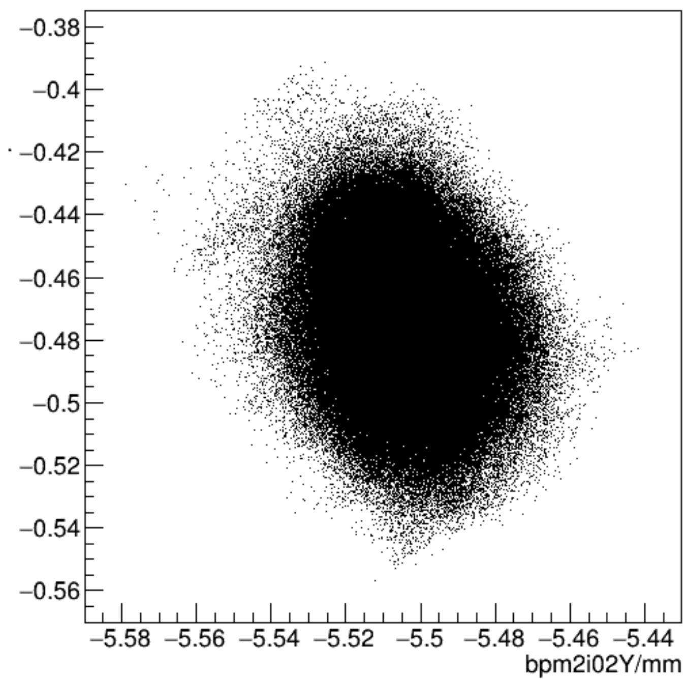
bpm2i02X/mm:bpm2i02Y/mm {ErrorFlag==0}
