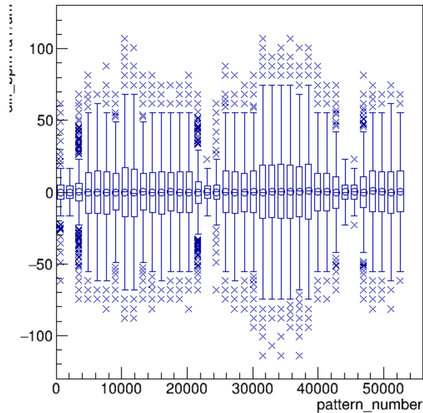
diff_bpm4aY/um:pattern_number {ErrorFlag==0}
