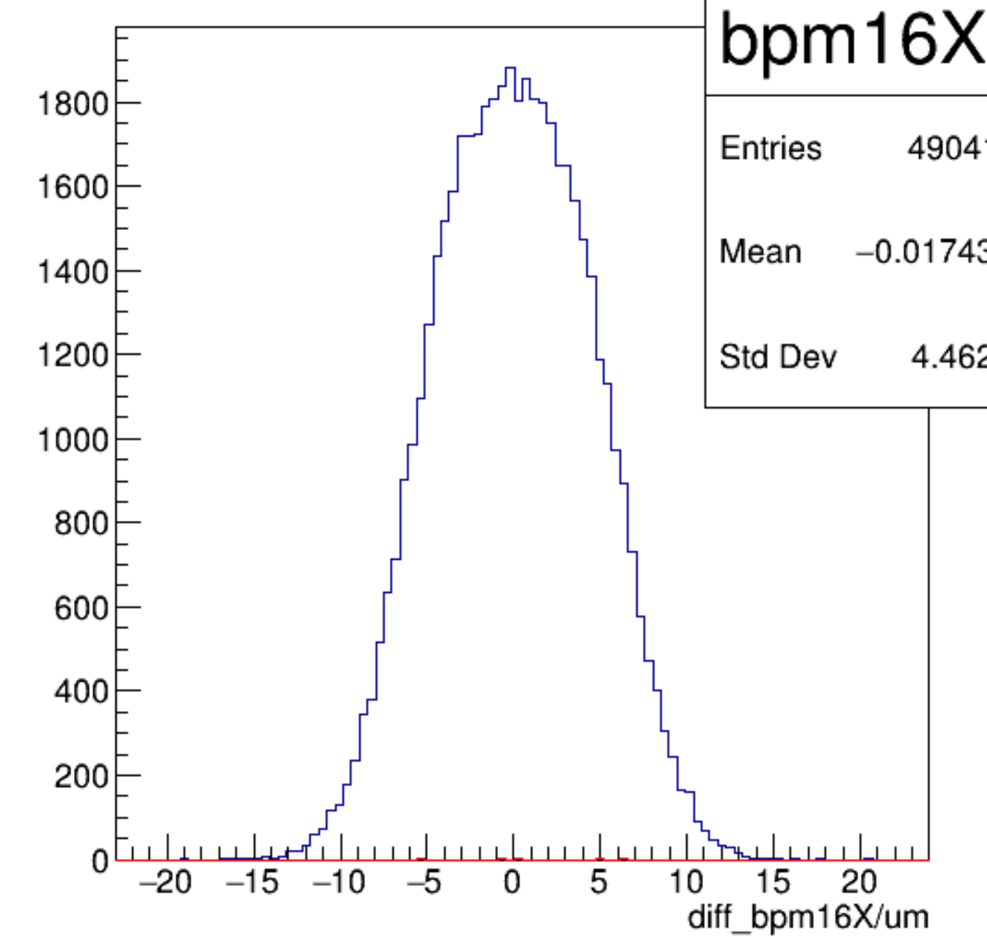
diff_bpm16X/um {ErrorFlag==0}
