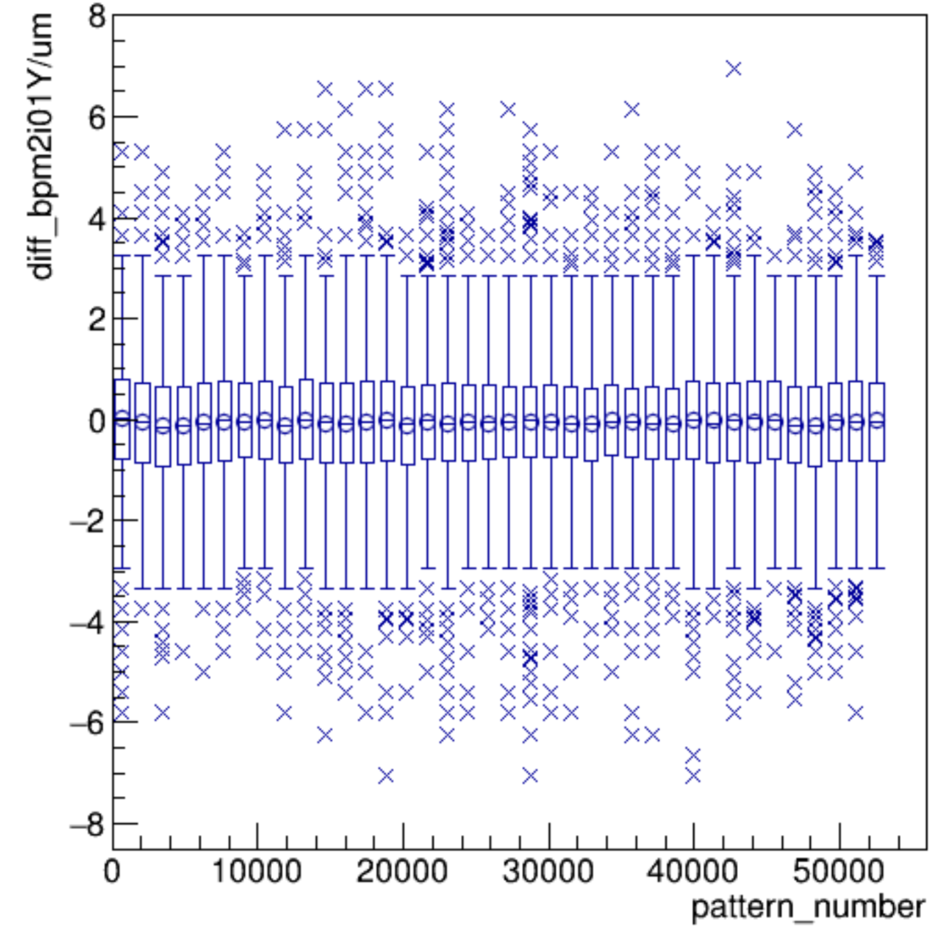
diff_bpm2i01Y/um:pattern_number {ErrorFlag==0}
