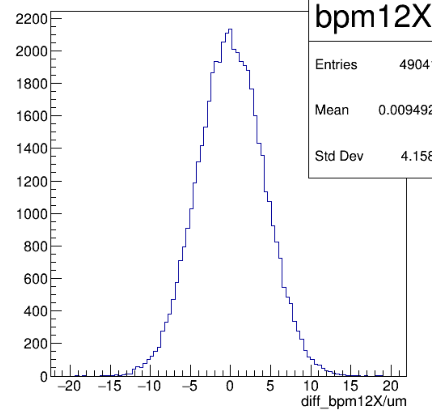
diff_bpm12X/um {ErrorFlag==0}
