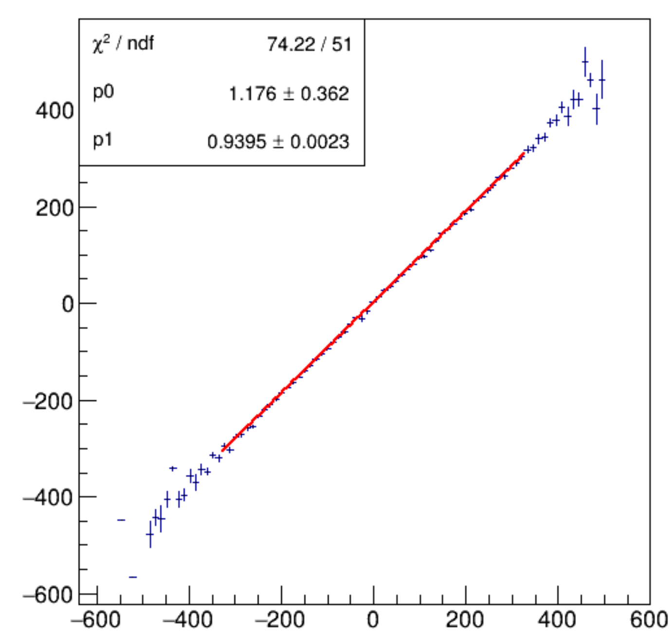
asym_bpm0l01WS/ppm:Aq/ppm {ErrorFlag==0}
