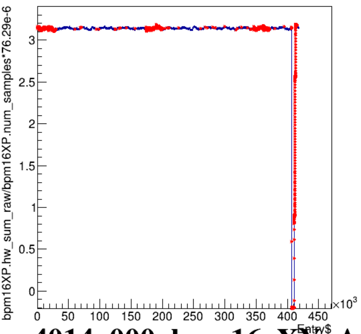
bpm16XP.hw_sum_raw/bpm16XP.num_samples*76.29e-6:Entry$
