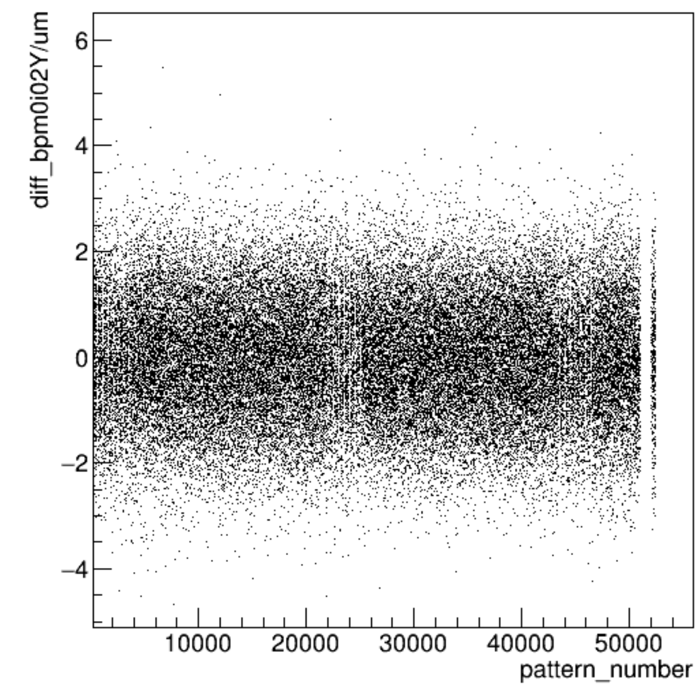
diff_bpm0i02Y/um:pattern_number {ErrorFlag==0}
