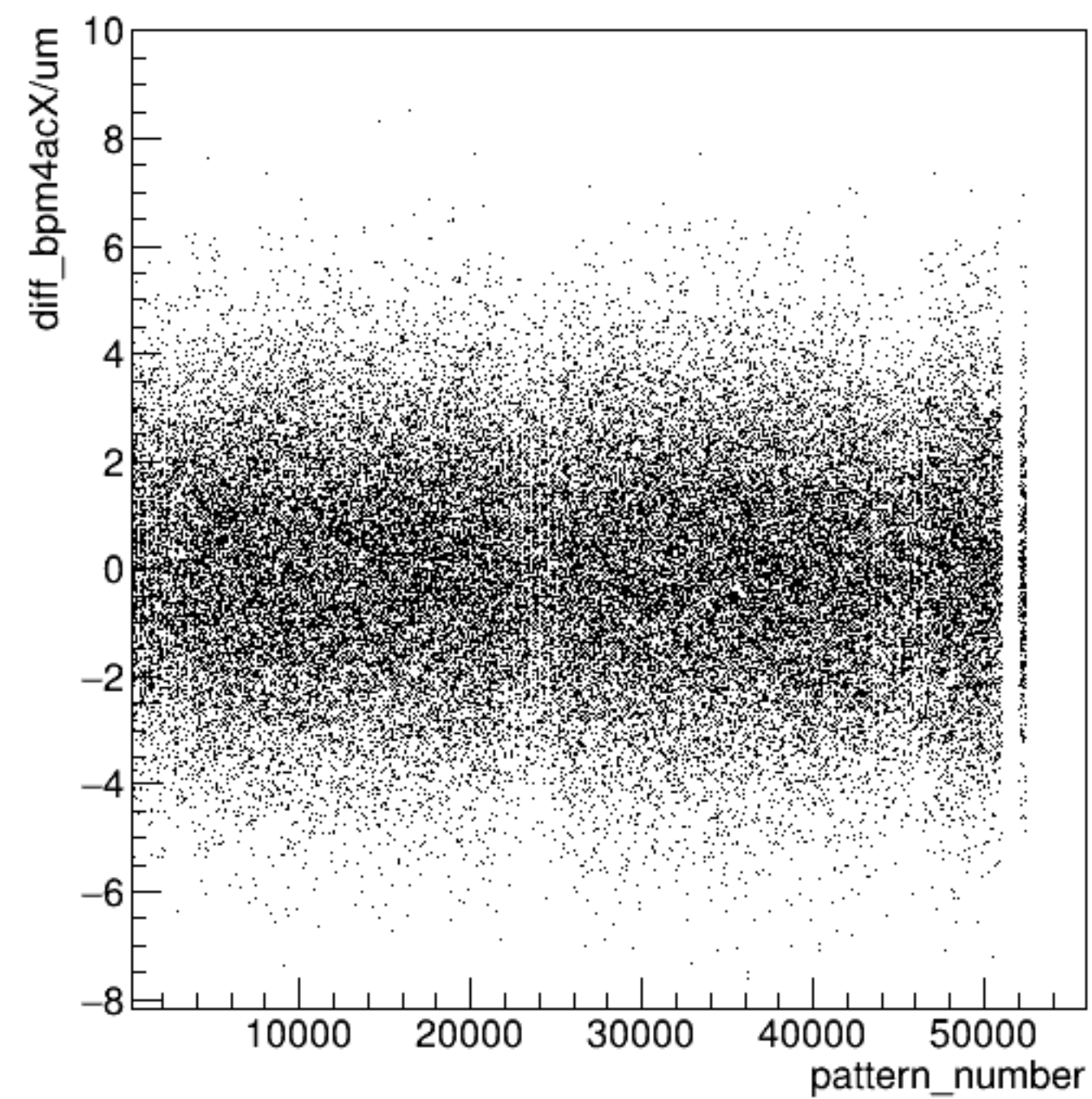
diff_bpm4acX/um:pattern_number {ErrorFlag==0}
