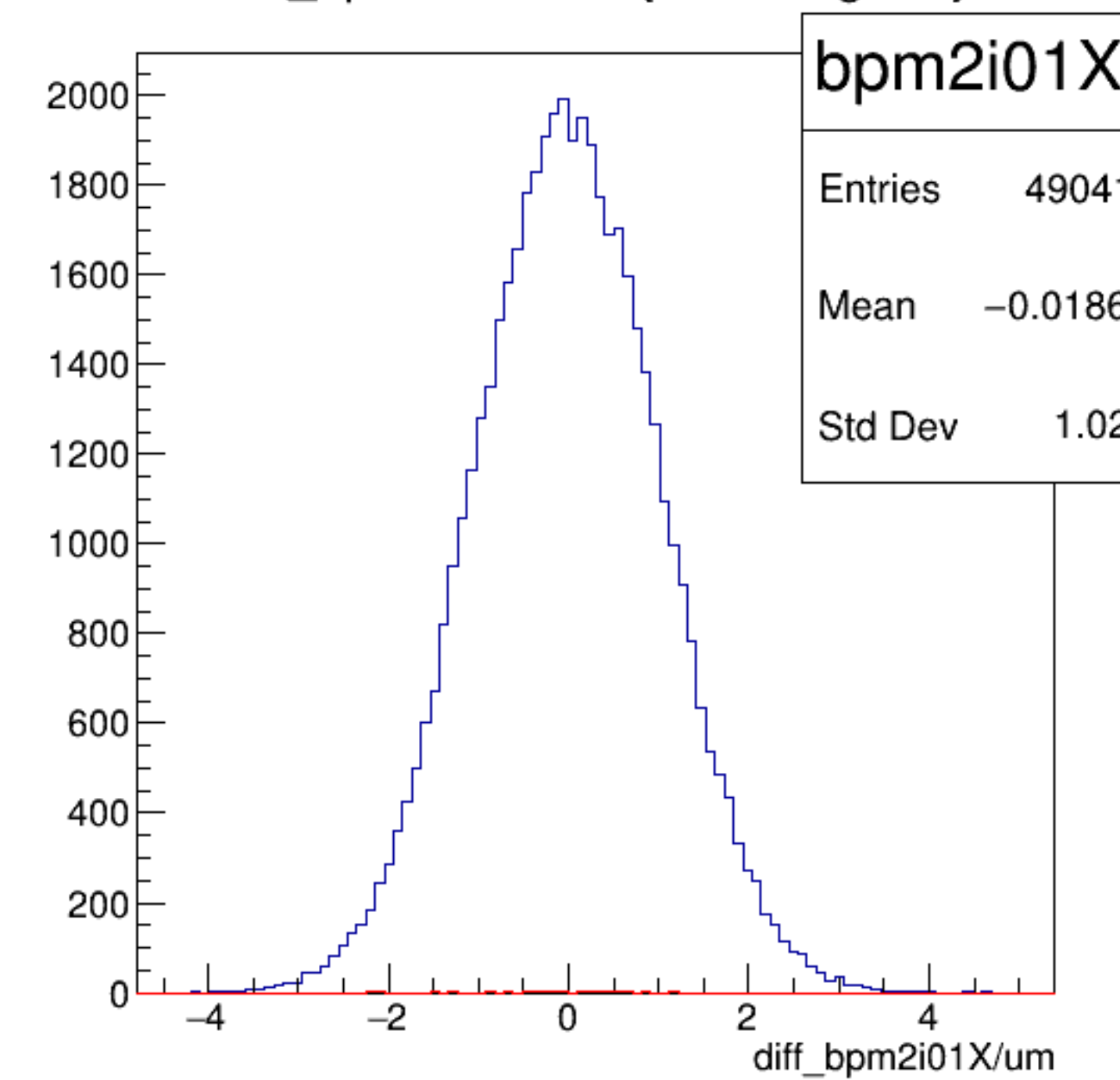
diff_bpm2i01X/um {ErrorFlag==0}
