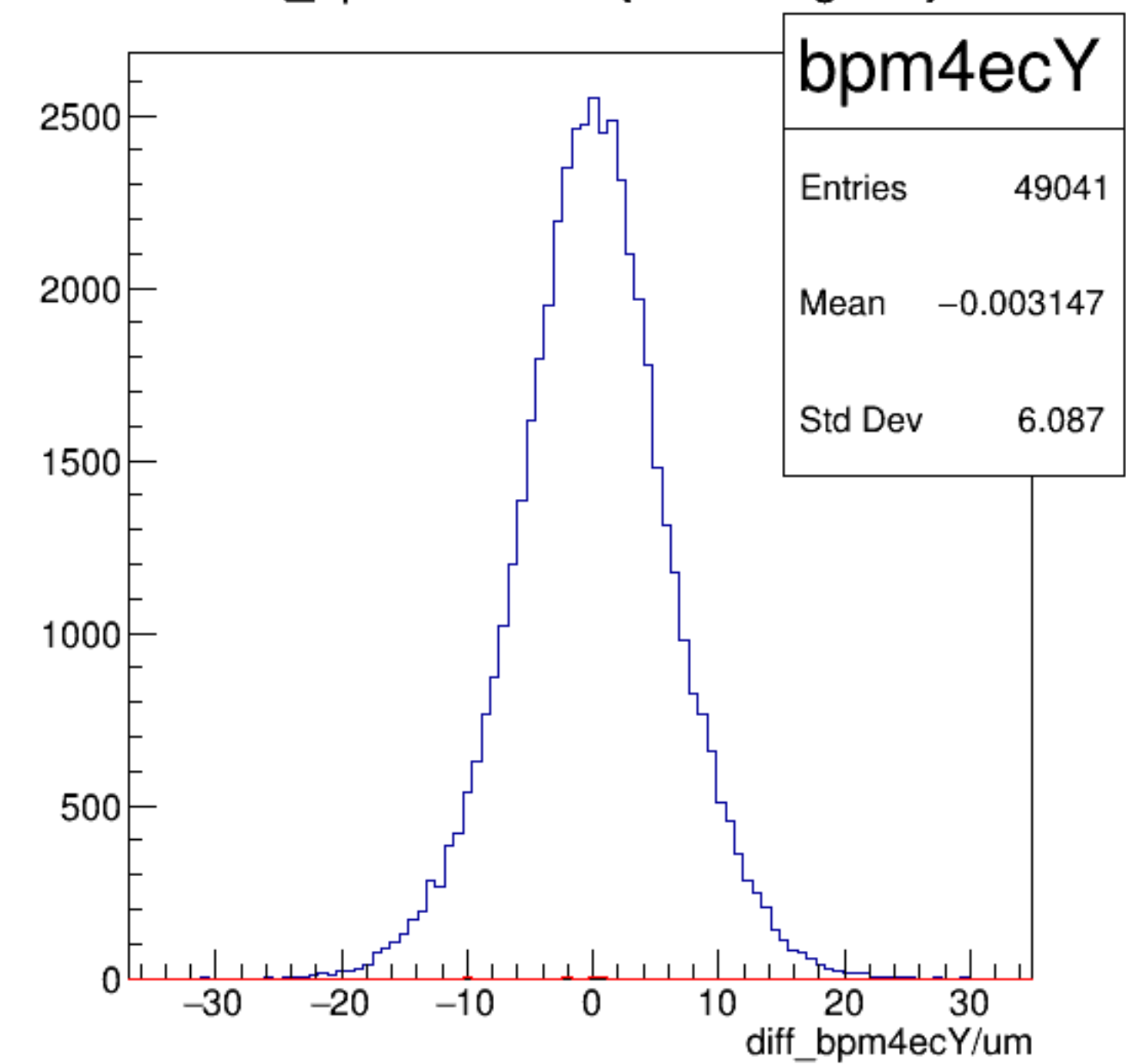
diff_bpm4ecY/um {ErrorFlag==0}
