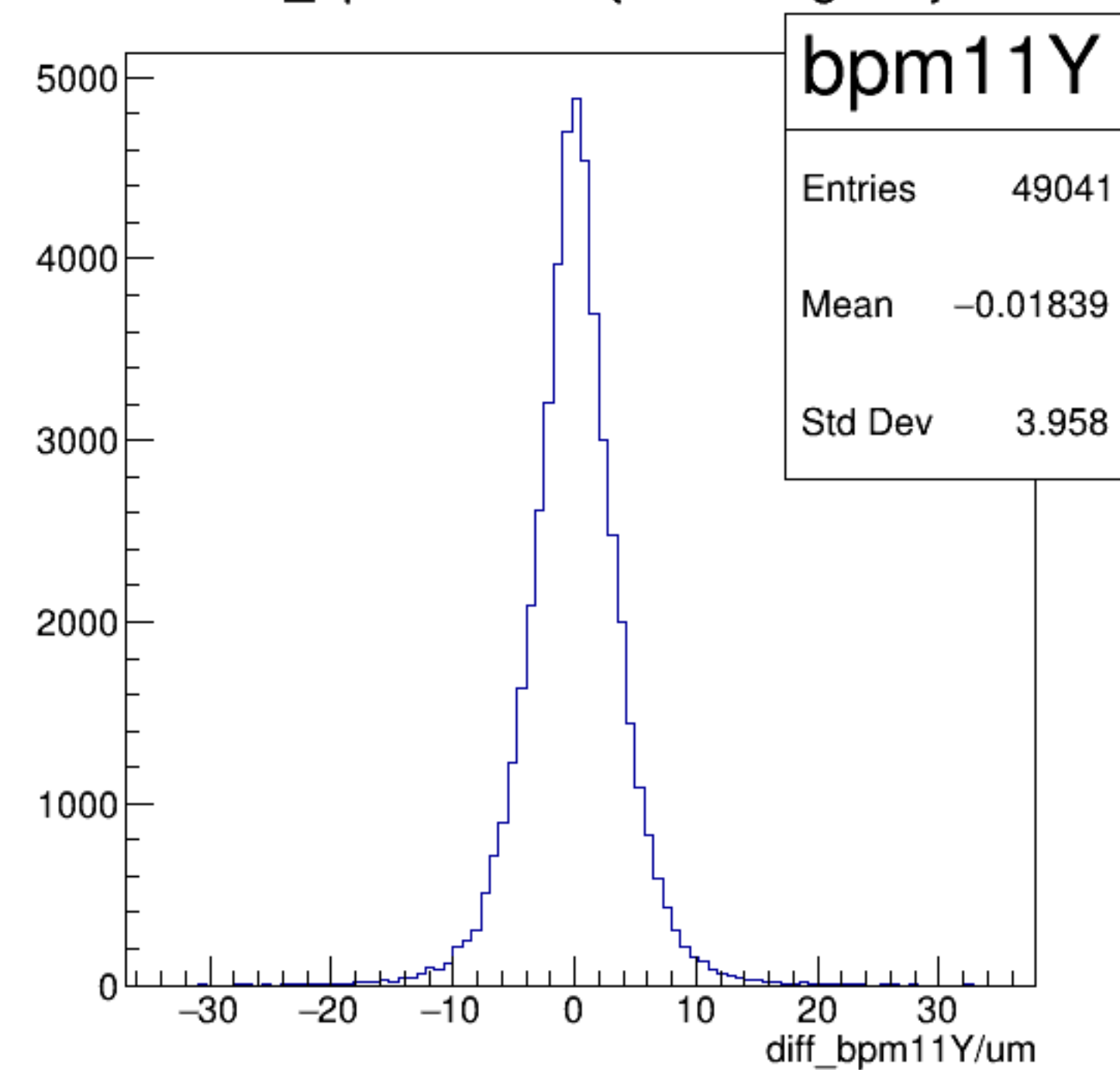
diff_bpm11Y/um {ErrorFlag==0}
