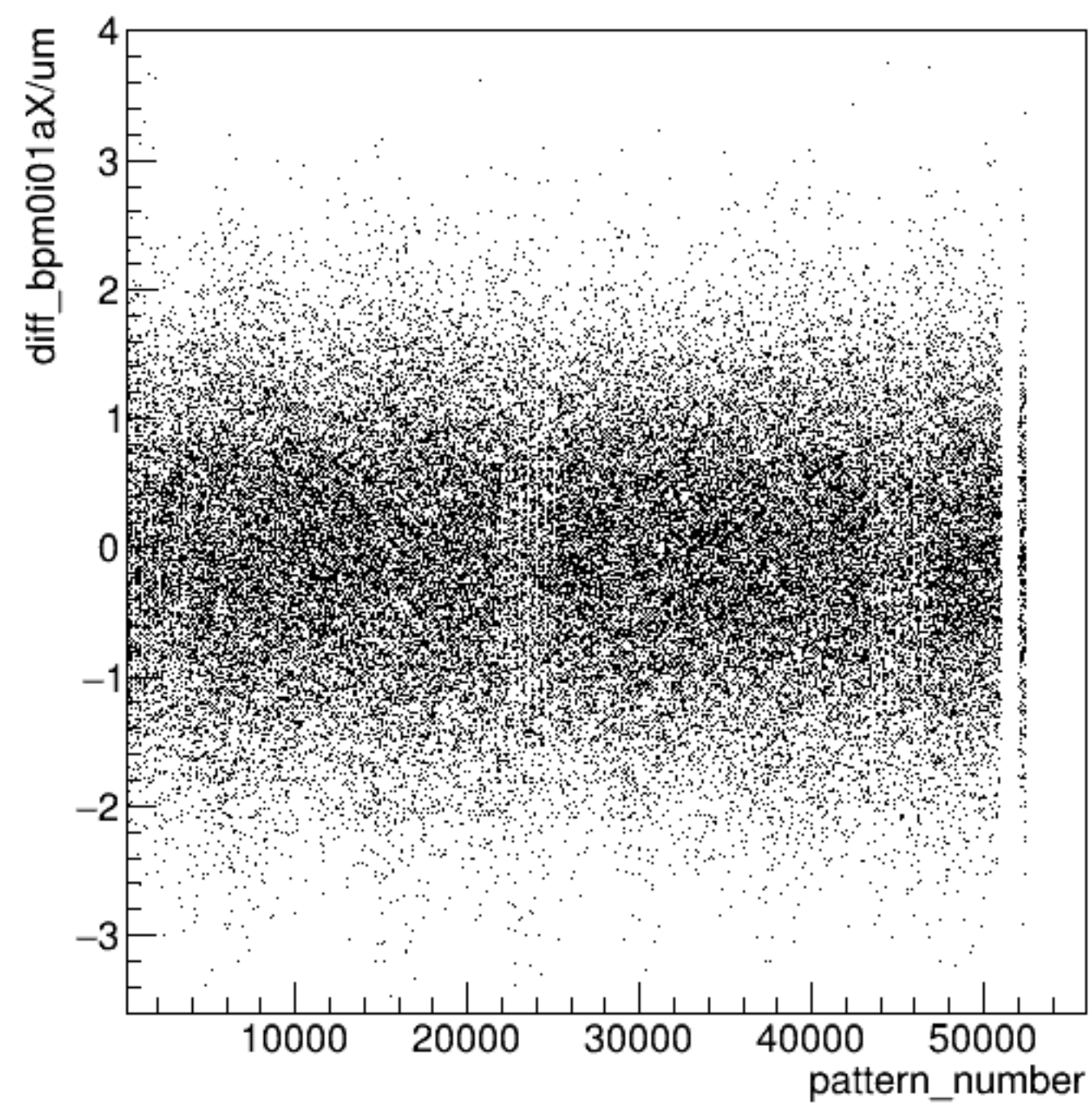
diff_bpm0i01aX/um:pattern_number {ErrorFlag==0}
