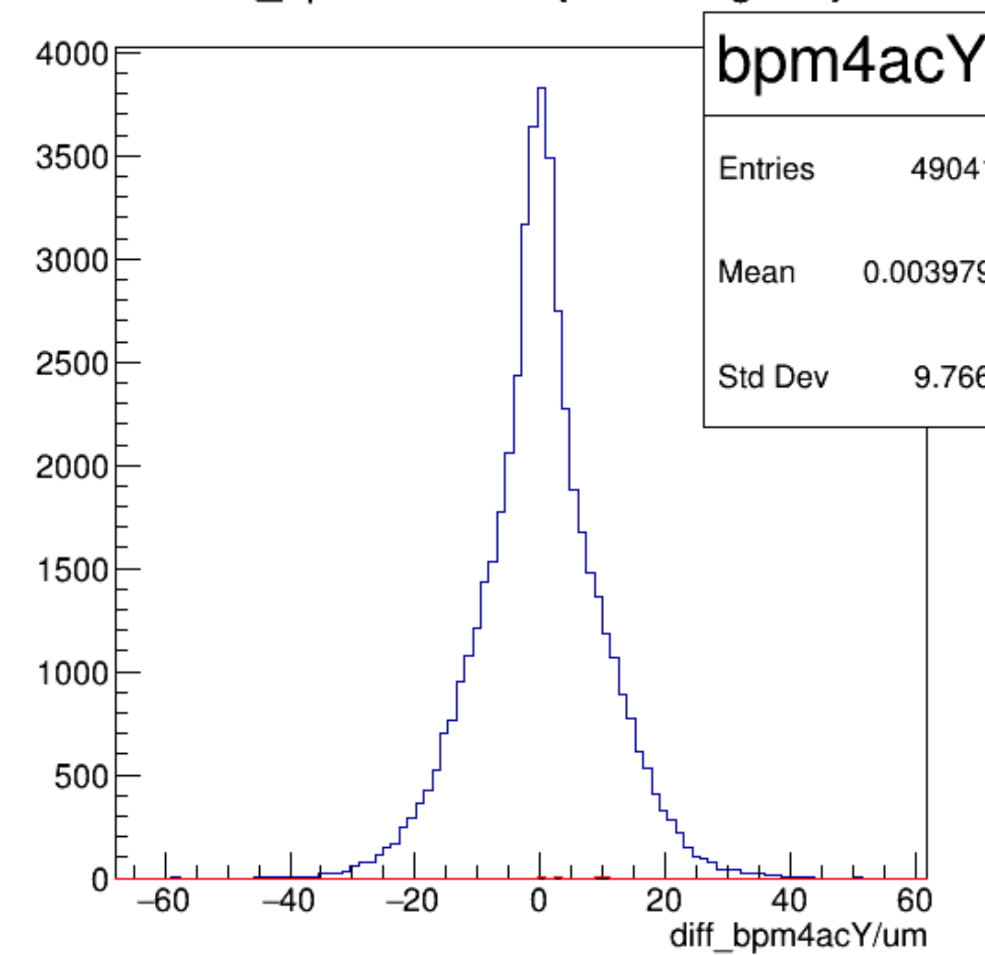
diff_bpm4acY/um {ErrorFlag==0}
