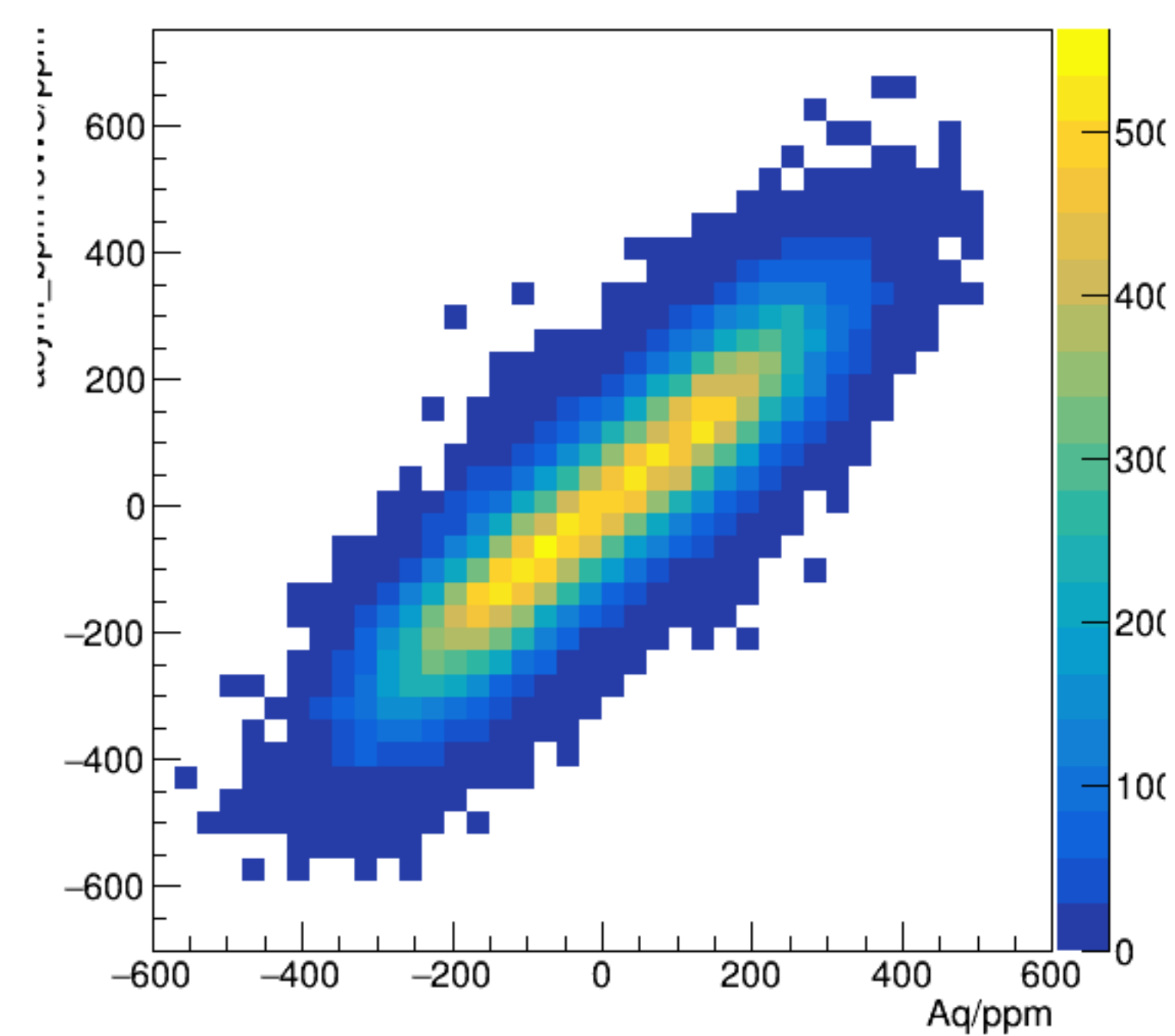
asym_bpm16WS/ppm:Aq/ppm {ErrorFlag==0}
