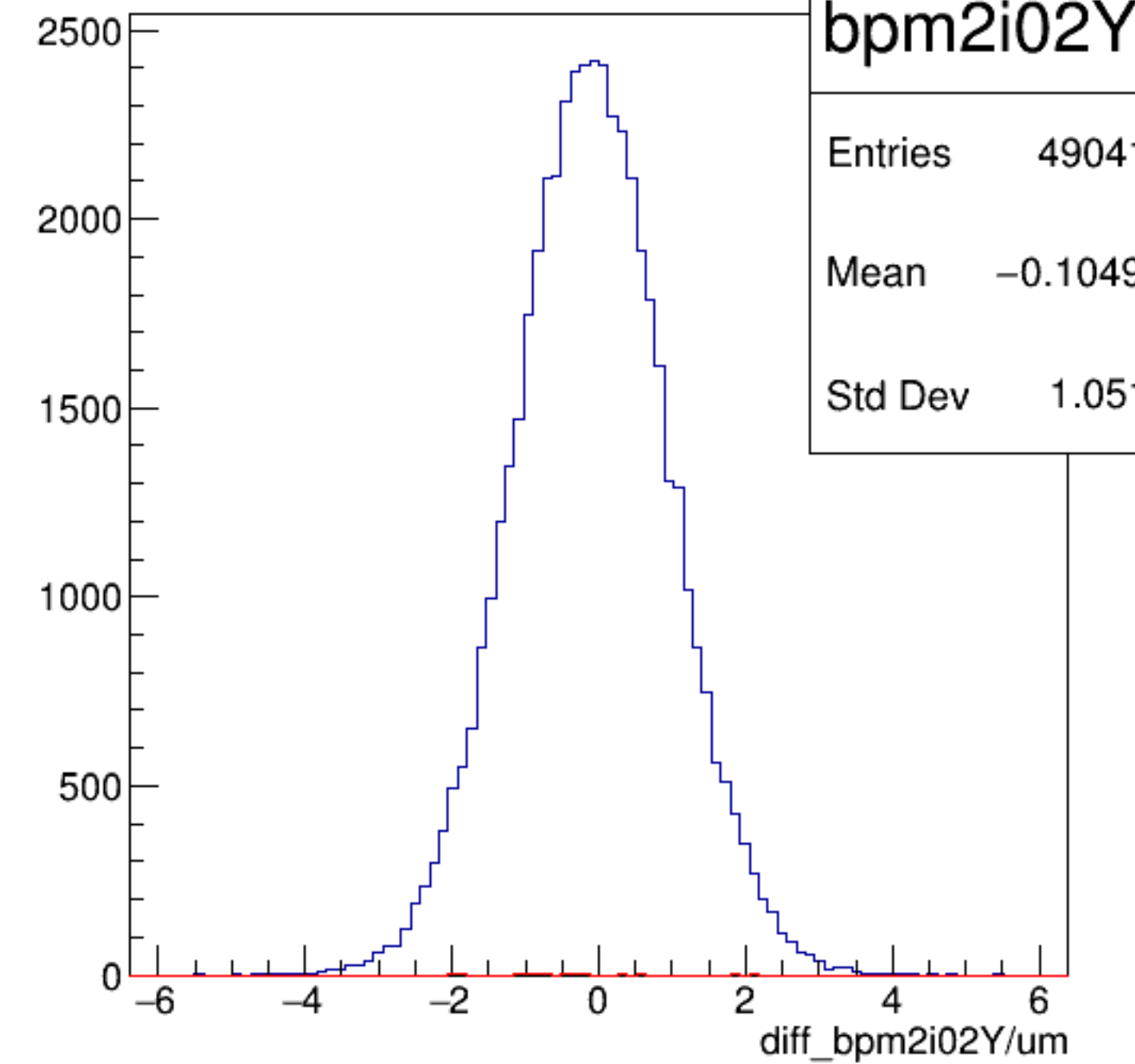
diff_bpm2i02Y/um {ErrorFlag==0}
