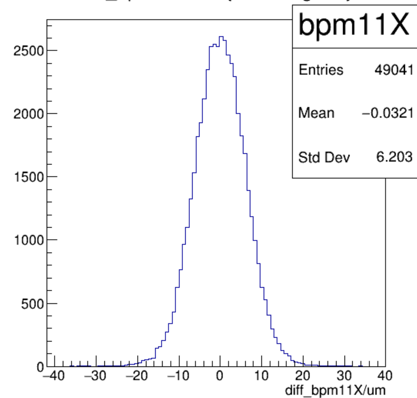
diff_bpm11X/um {ErrorFlag==0}
