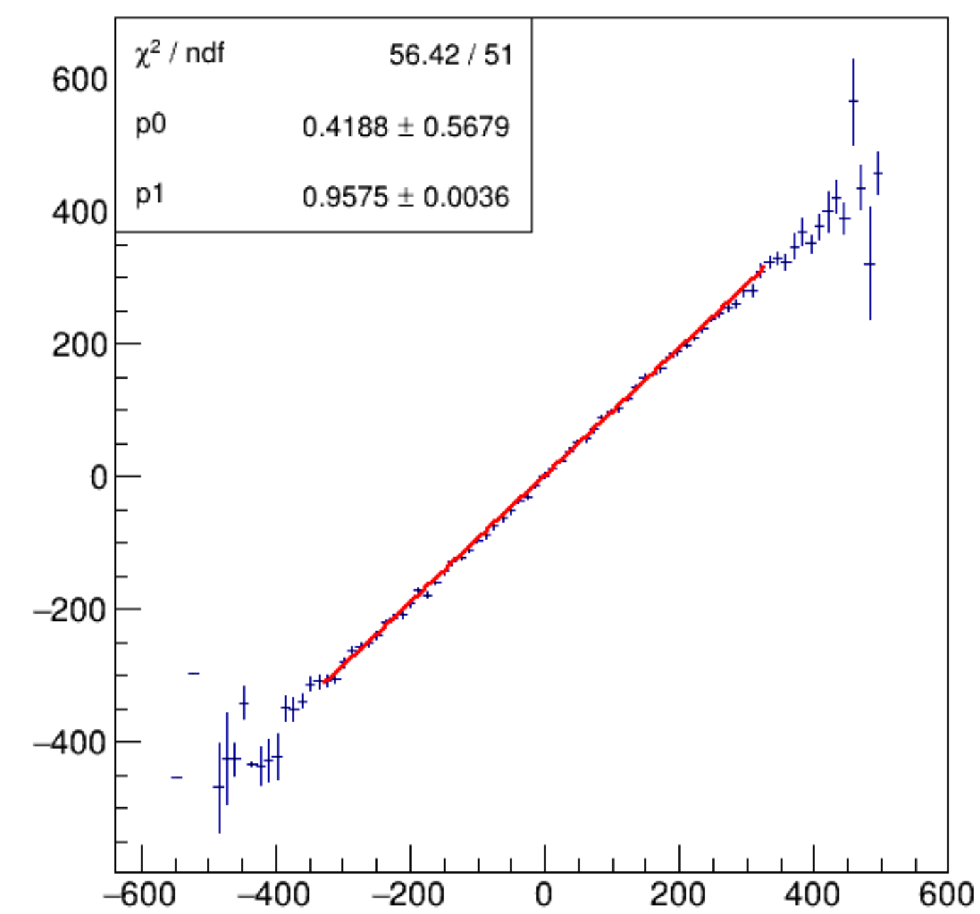
asym_bpm11WS/ppm:Aq/ppm {ErrorFlag==0}
