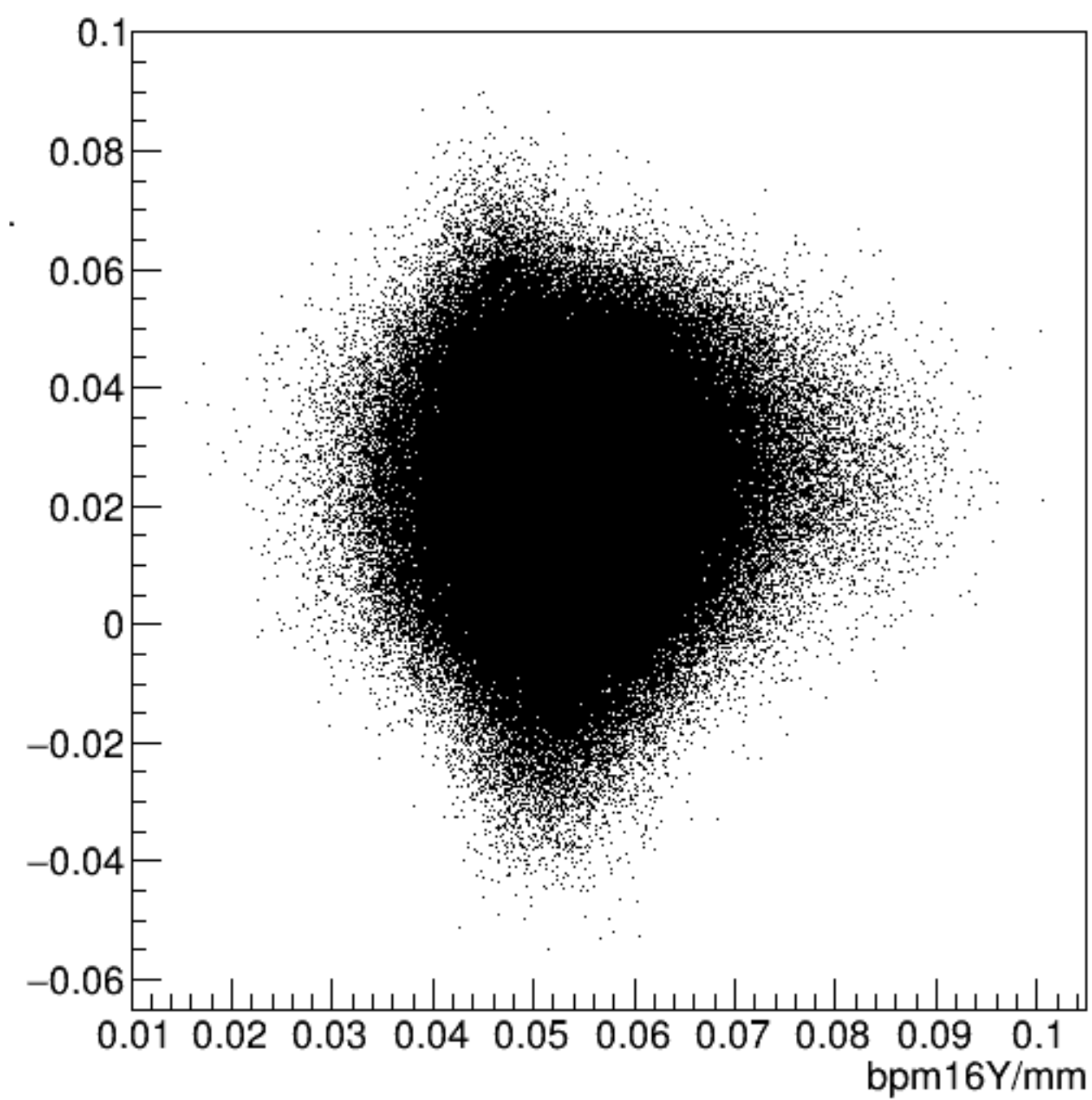
bpm16X/mm:bpm16Y/mm {ErrorFlag==0}
