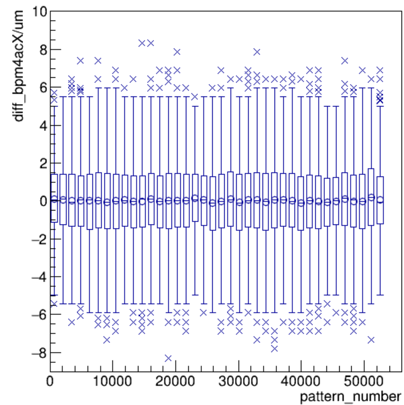
diff_bpm4acX/um:pattern_number {ErrorFlag==0}
