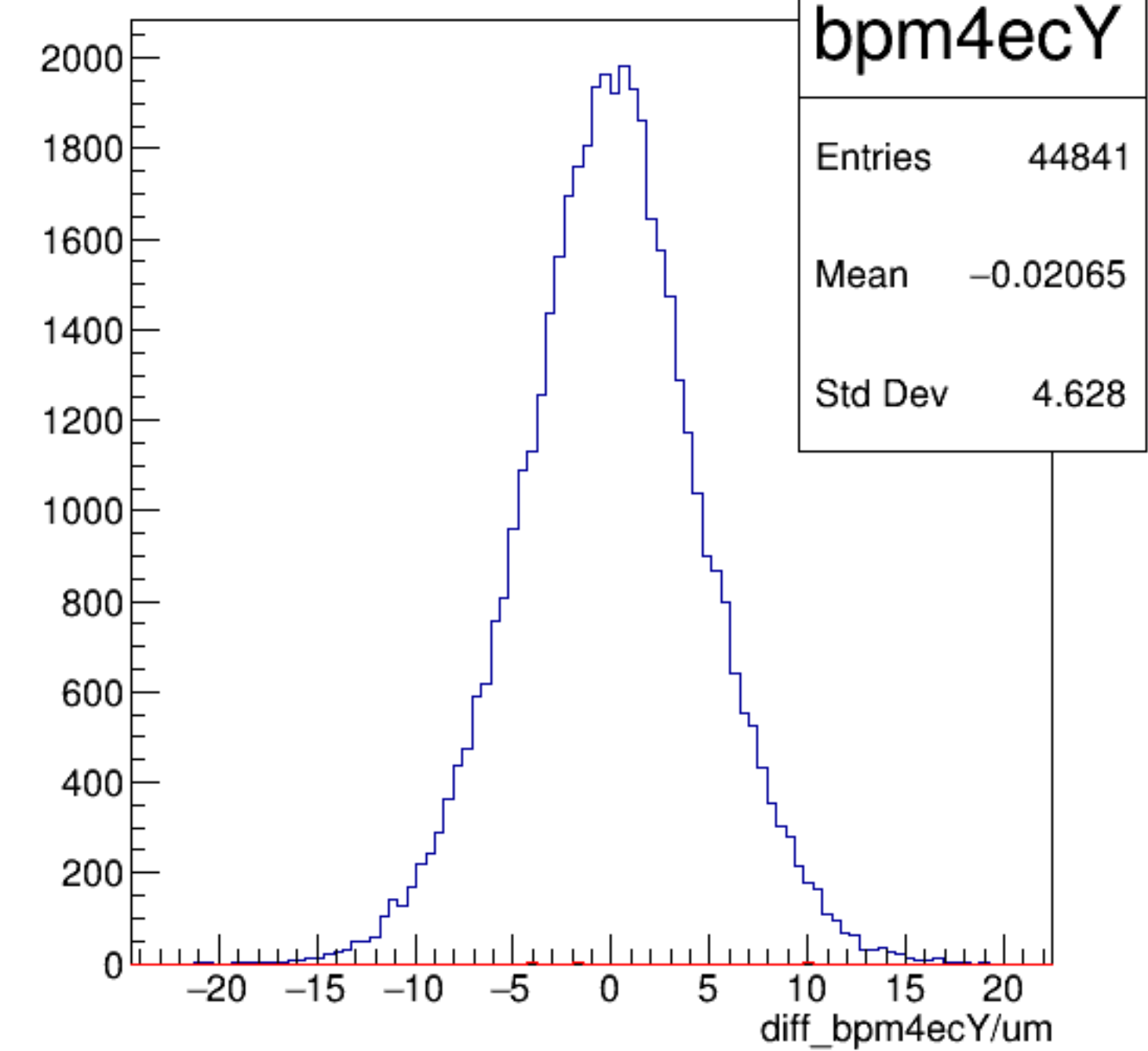
diff_bpm4ecY/um {ErrorFlag==0}
