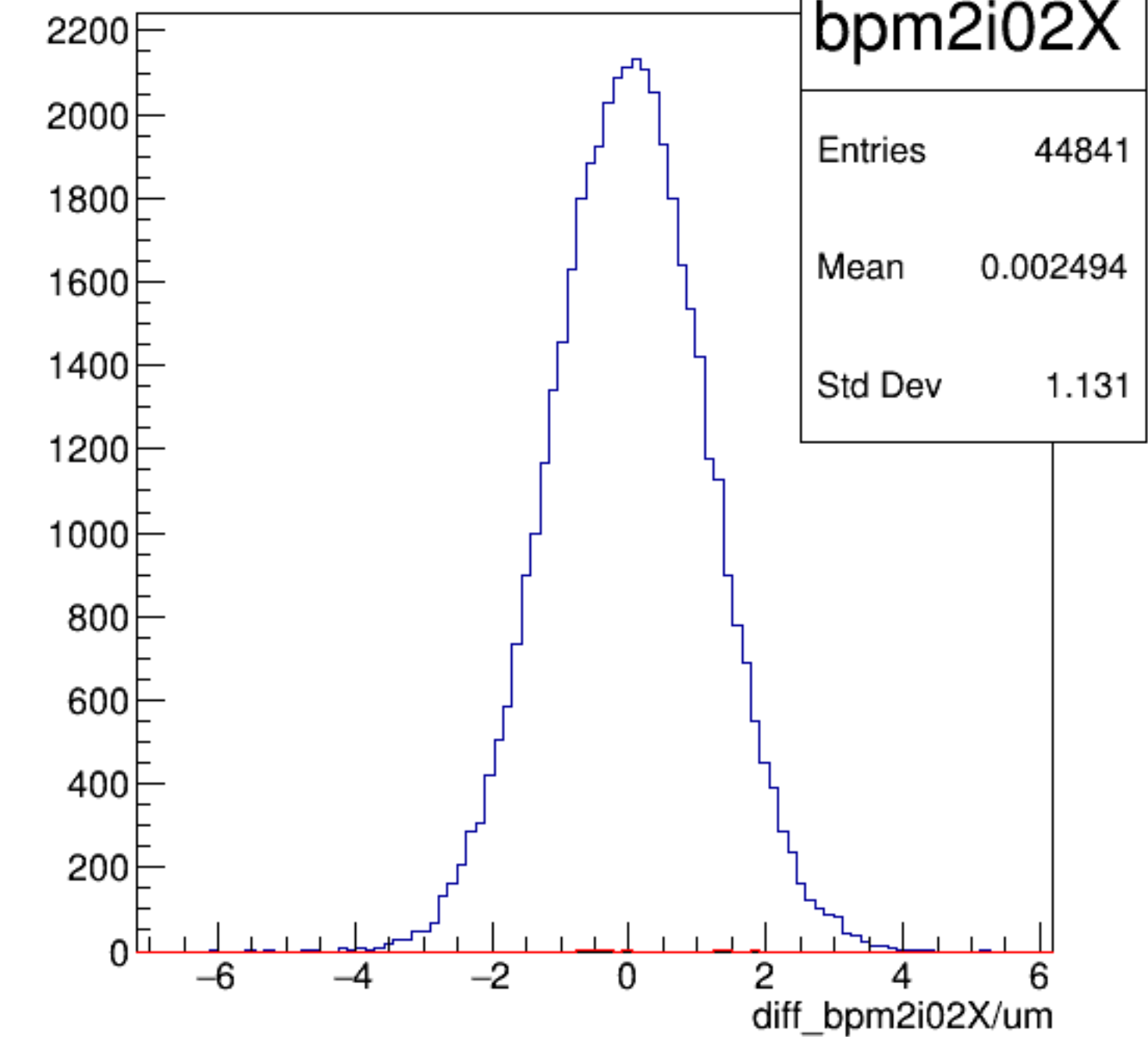
diff_bpm2i02X/um {ErrorFlag==0}
