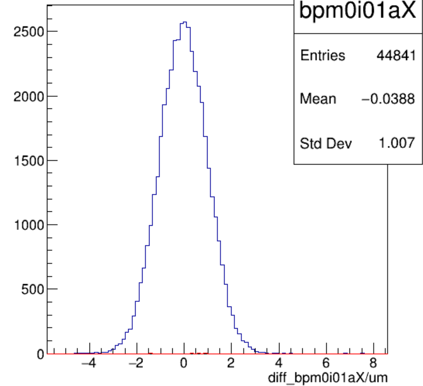
diff_bpm0i01aX/um {ErrorFlag==0}
