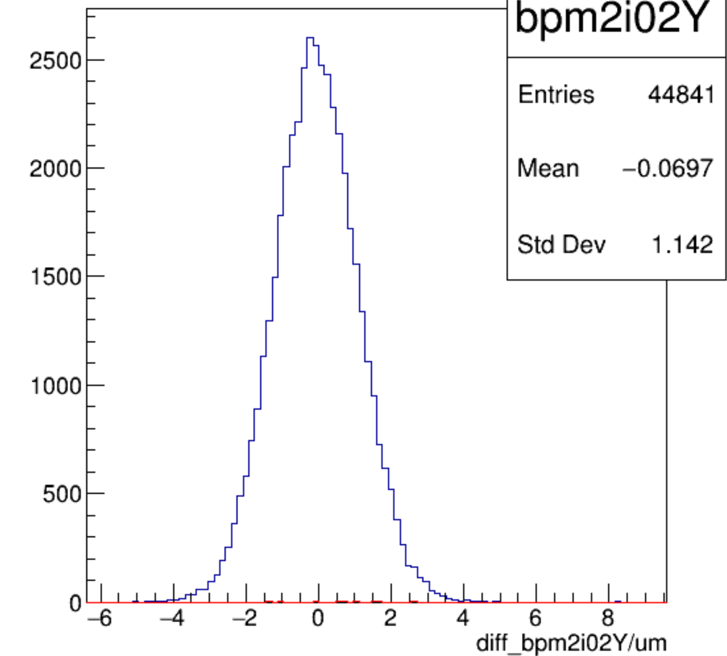
diff_bpm2i02Y/um {ErrorFlag==0}
