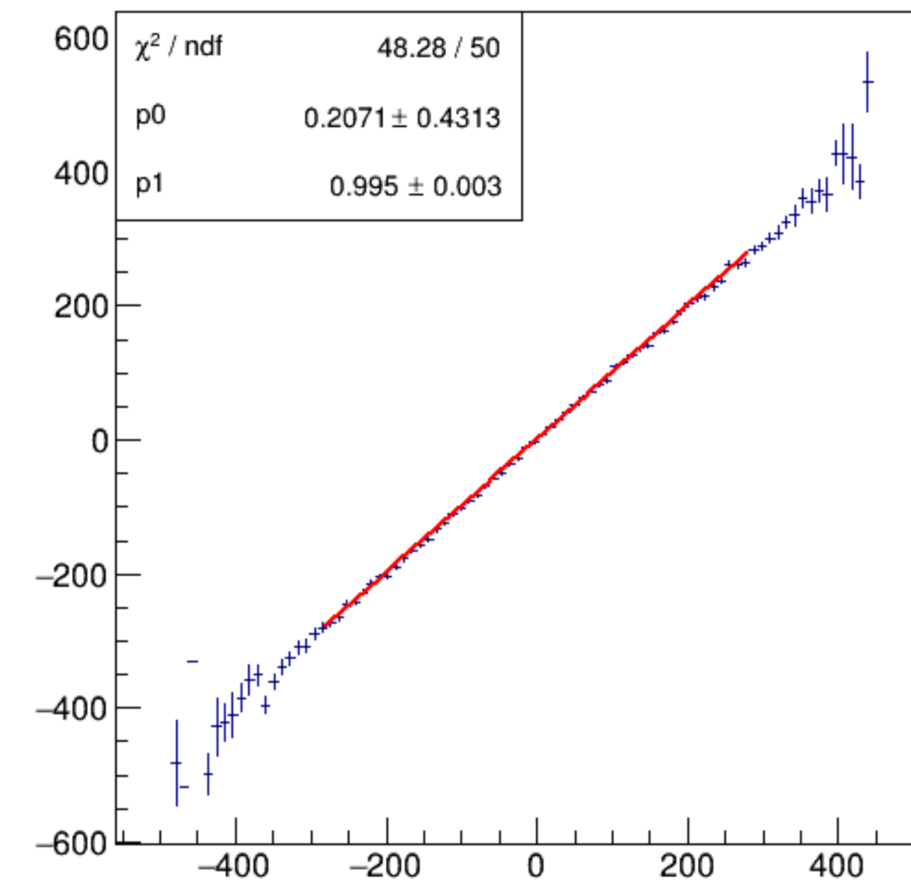
asym_bpm16WS/ppm:Aq/ppm {ErrorFlag==0}
