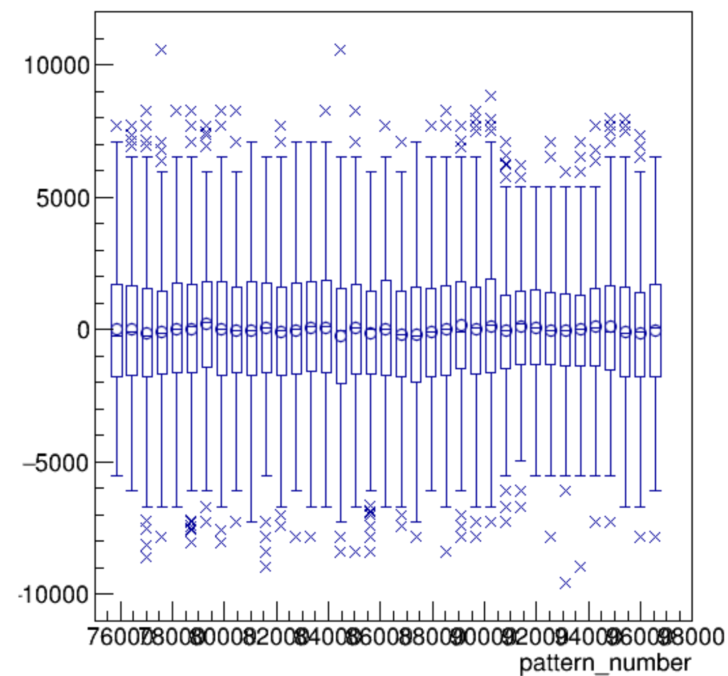
asym_atr2/ppm:pattern_number {ErrorFlag==0}
