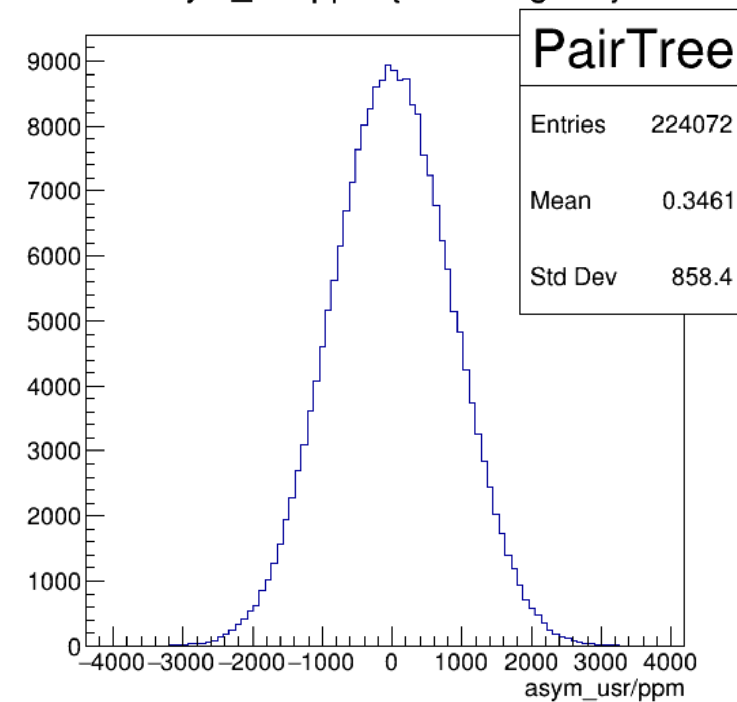
asym_usr/ppm {ErrorFlag==0}
