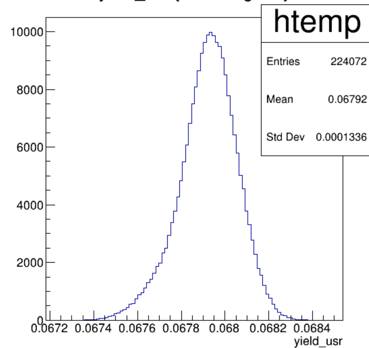
yield_usr {ErrorFlag==0}
