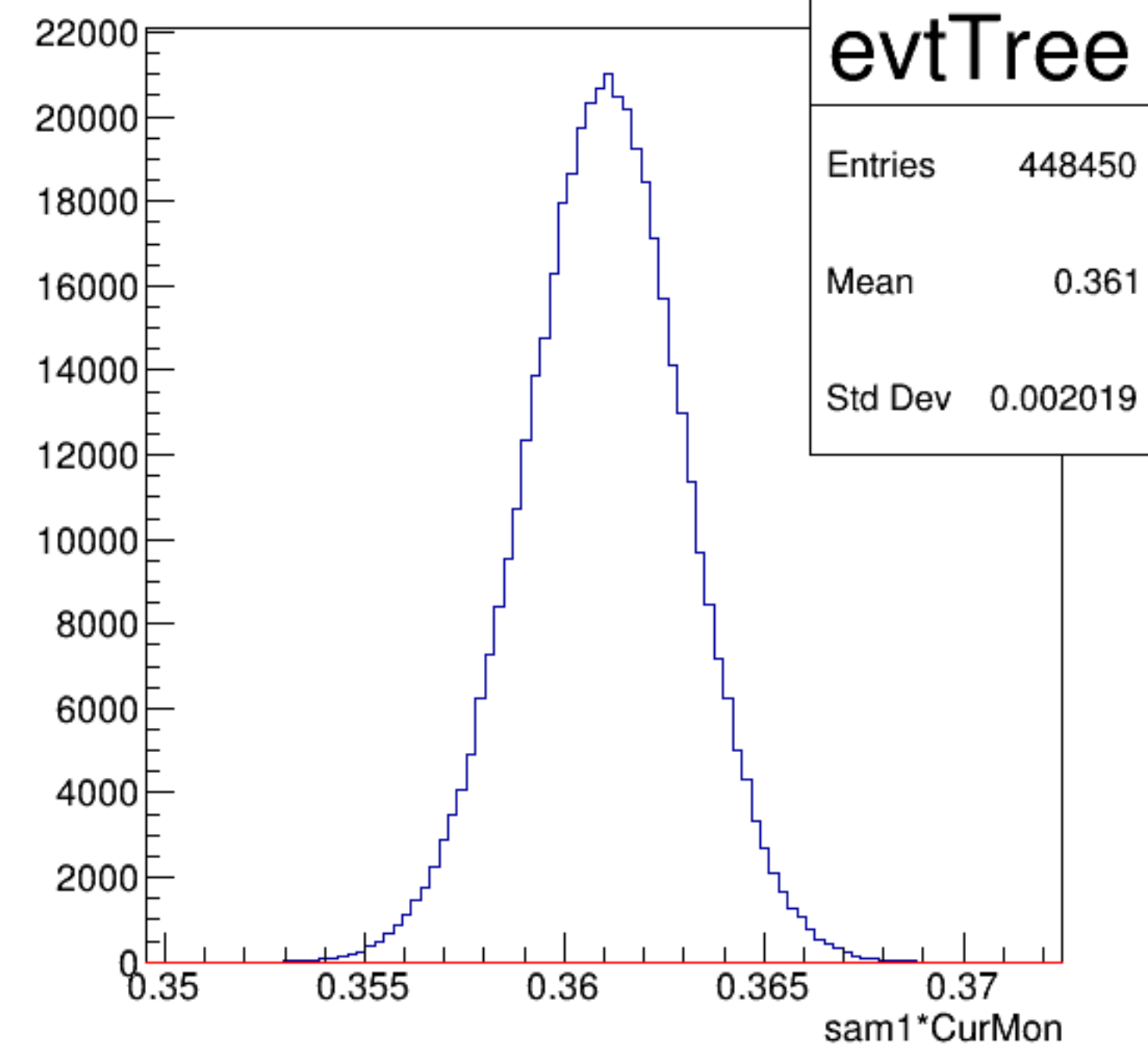
sam1*CurMon {ErrorFlag==0}
