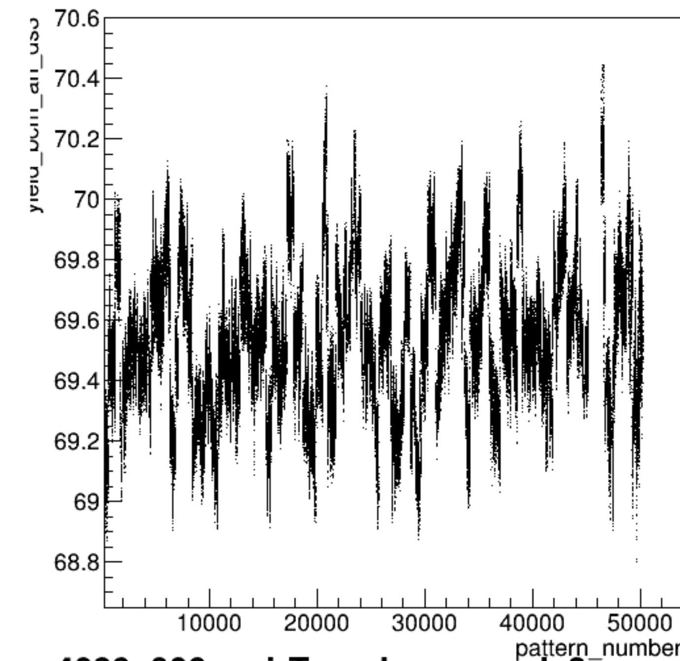
yield_bcm_an_ds3:pattern_number {ErrorFlag==0}
