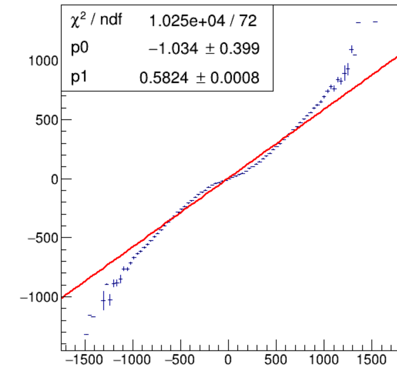
run4039_000_asym_bcm_dg_us_vs_asym_bcm_an_ds3_pr.png
