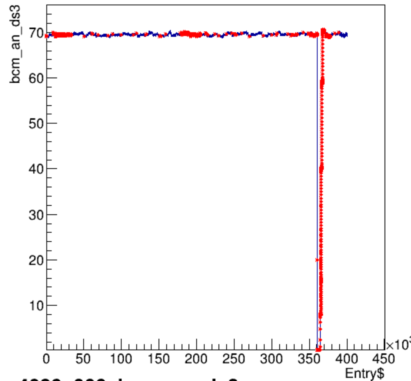
bcm_an_ds3:Entry$
