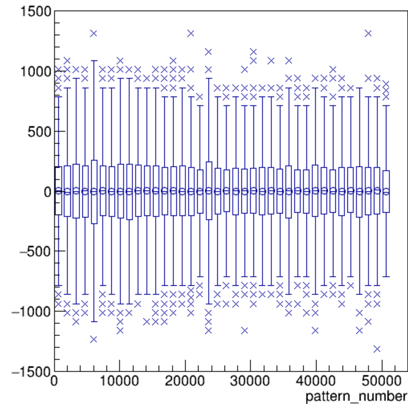
asym_bcm_dg_us/ppm:pattern_number {ErrorFlag==0}
