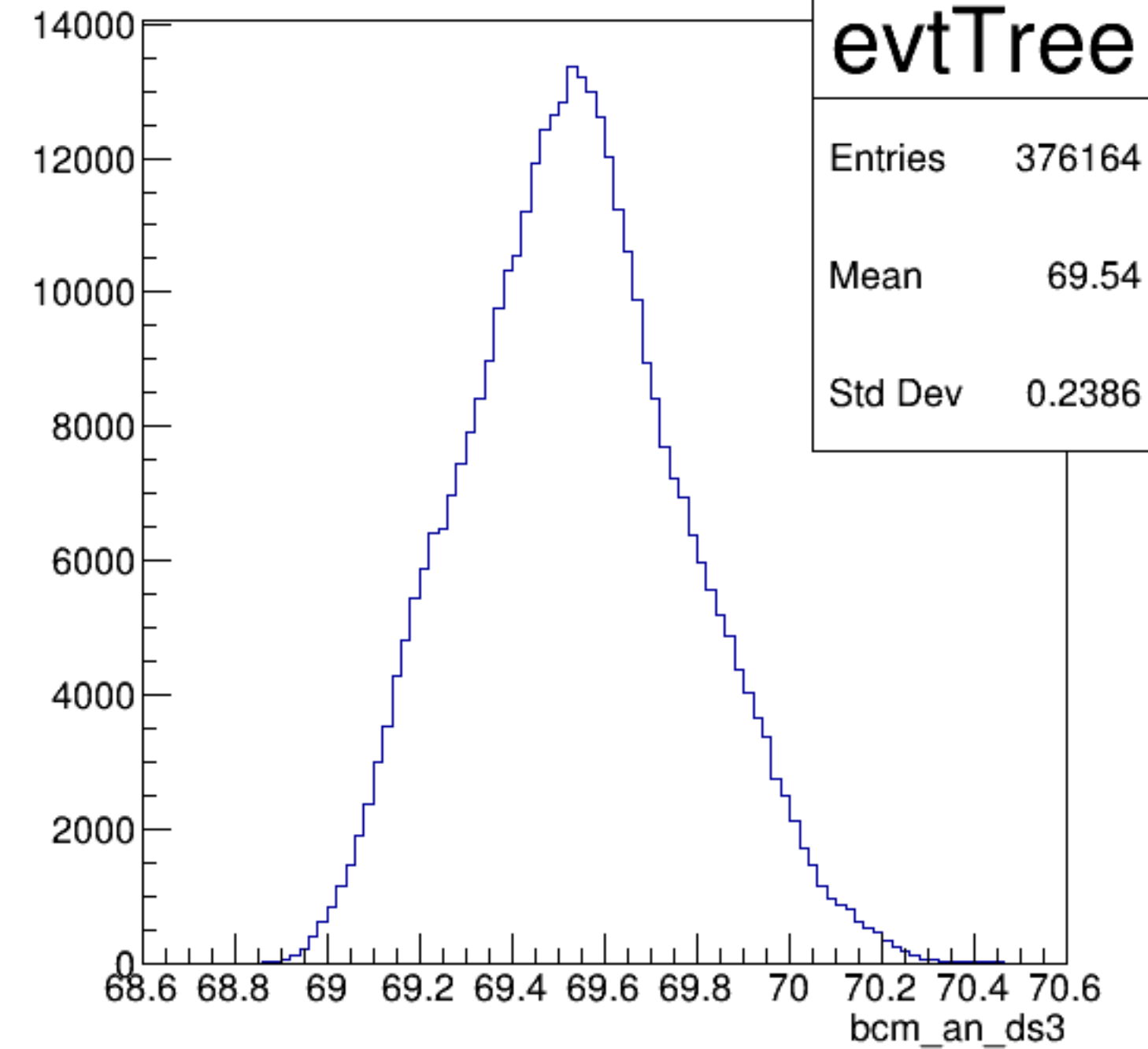
bcm_an_ds3 {ErrorFlag==0}
