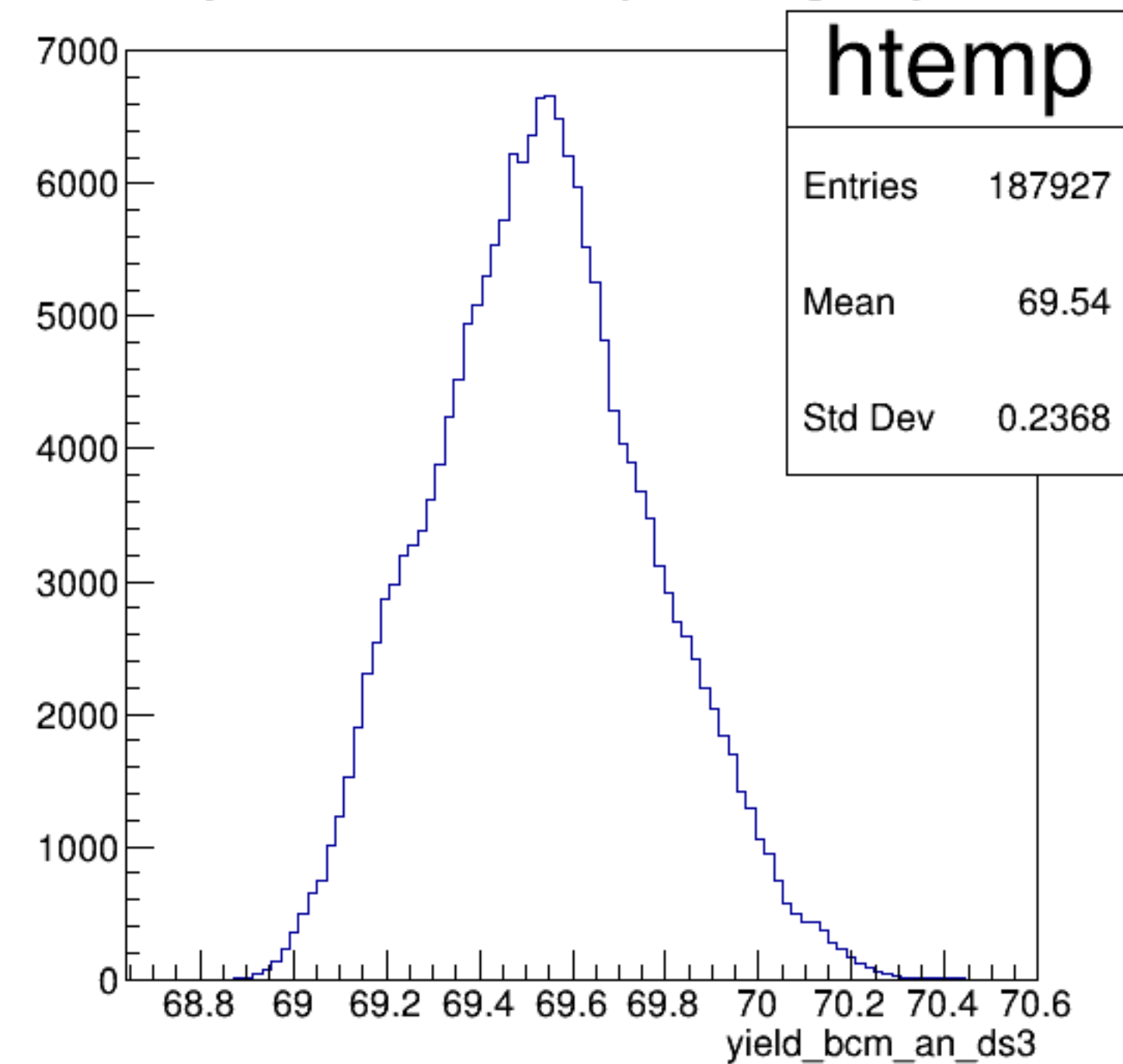
yield_bcm_an_ds3 {ErrorFlag==0}
