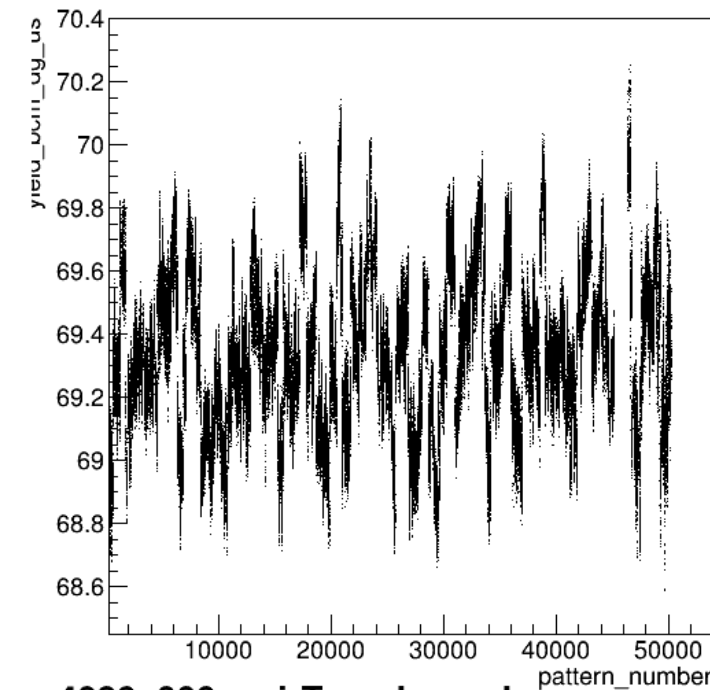
yield_bcm_dg_us:pattern_number {ErrorFlag==0}
