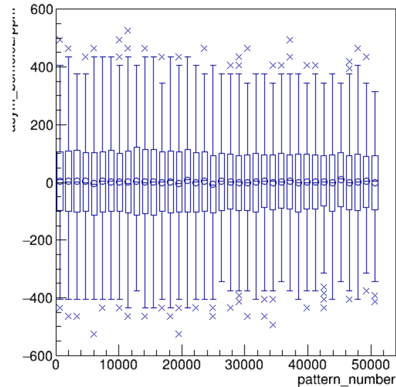
asym_bcm0l02/ppm:pattern_number {ErrorFlag==0}
