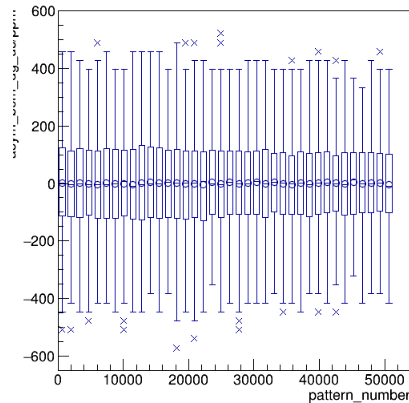
asym_bcm_dg_us/ppm:pattern_number {ErrorFlag==0}
