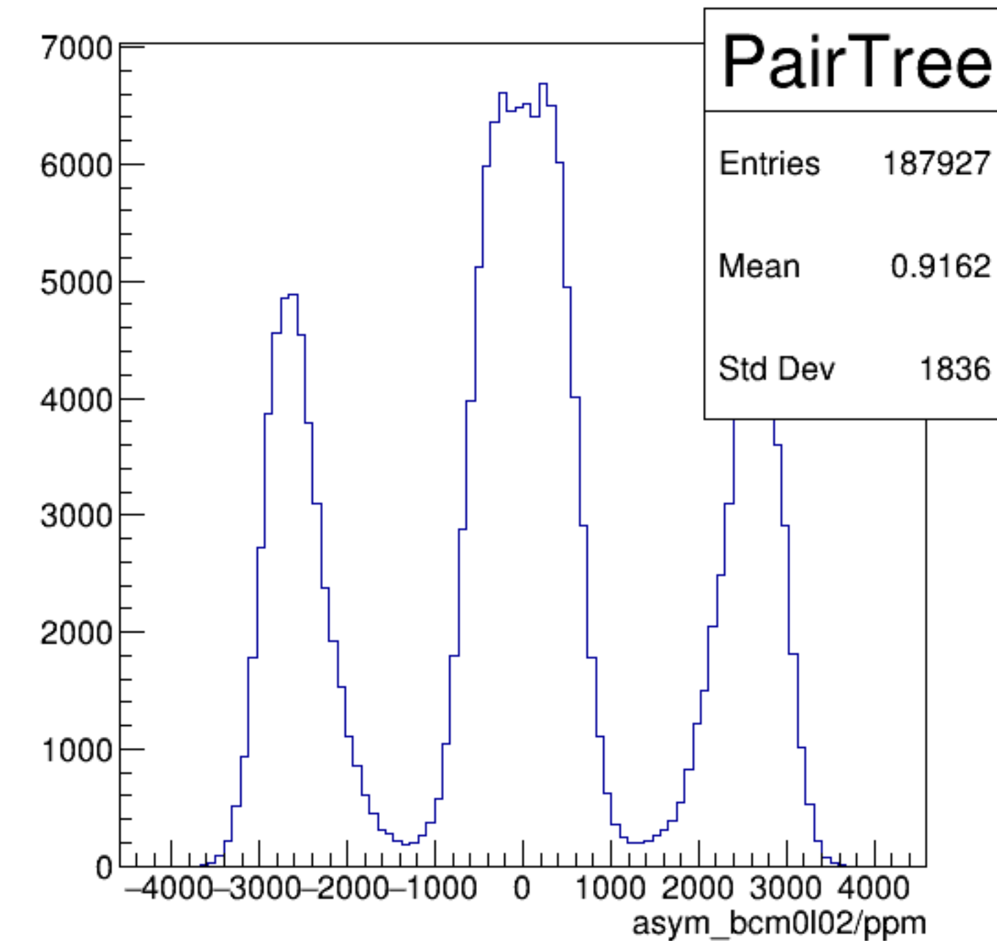
asym_bcm0l02/ppm {ErrorFlag==0}
