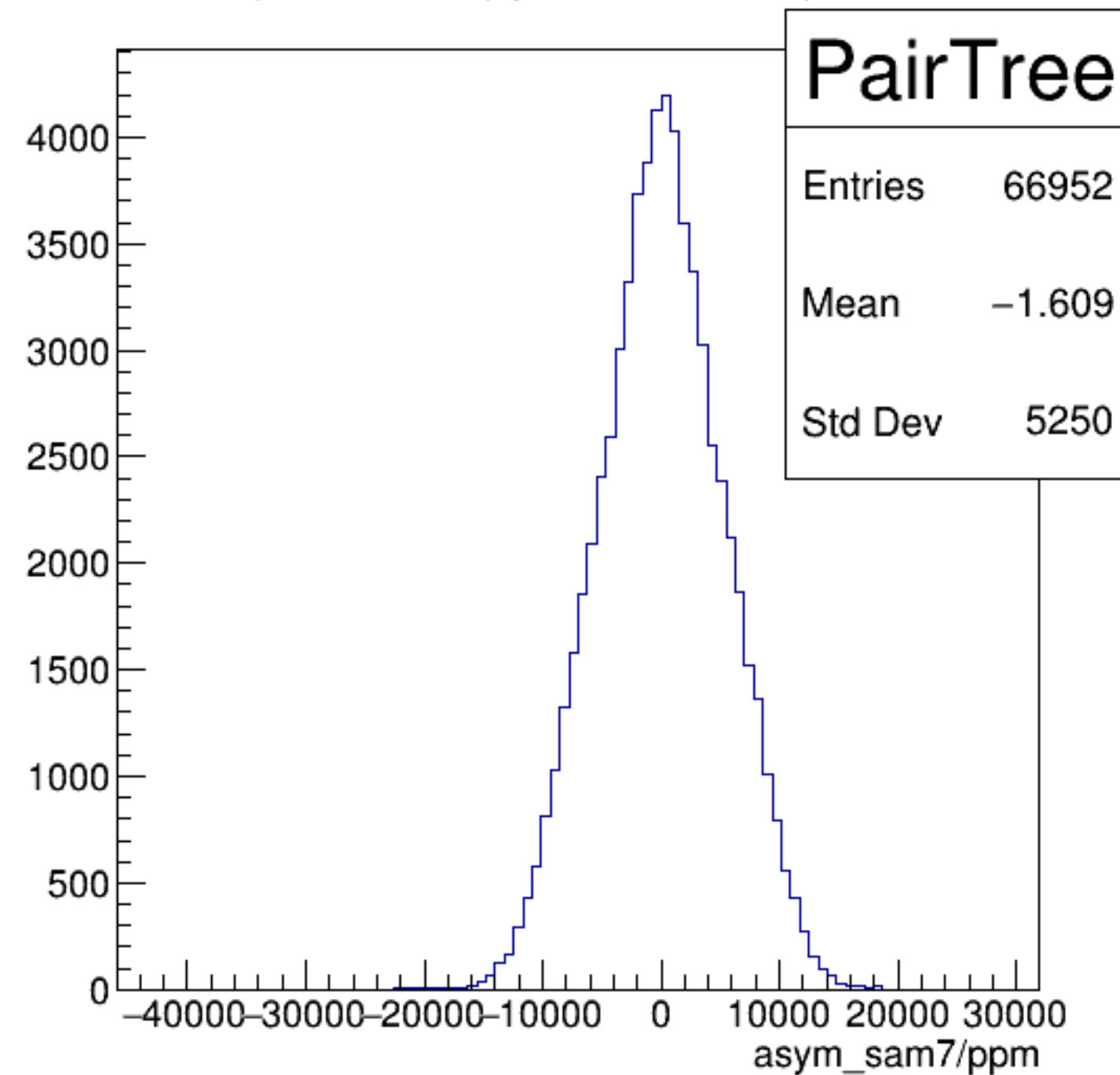
asym_sam7/ppm {ErrorFlag==0}
