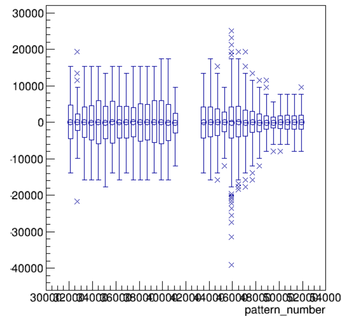
asym_sam7/ppm:pattern_number {ErrorFlag==0}
