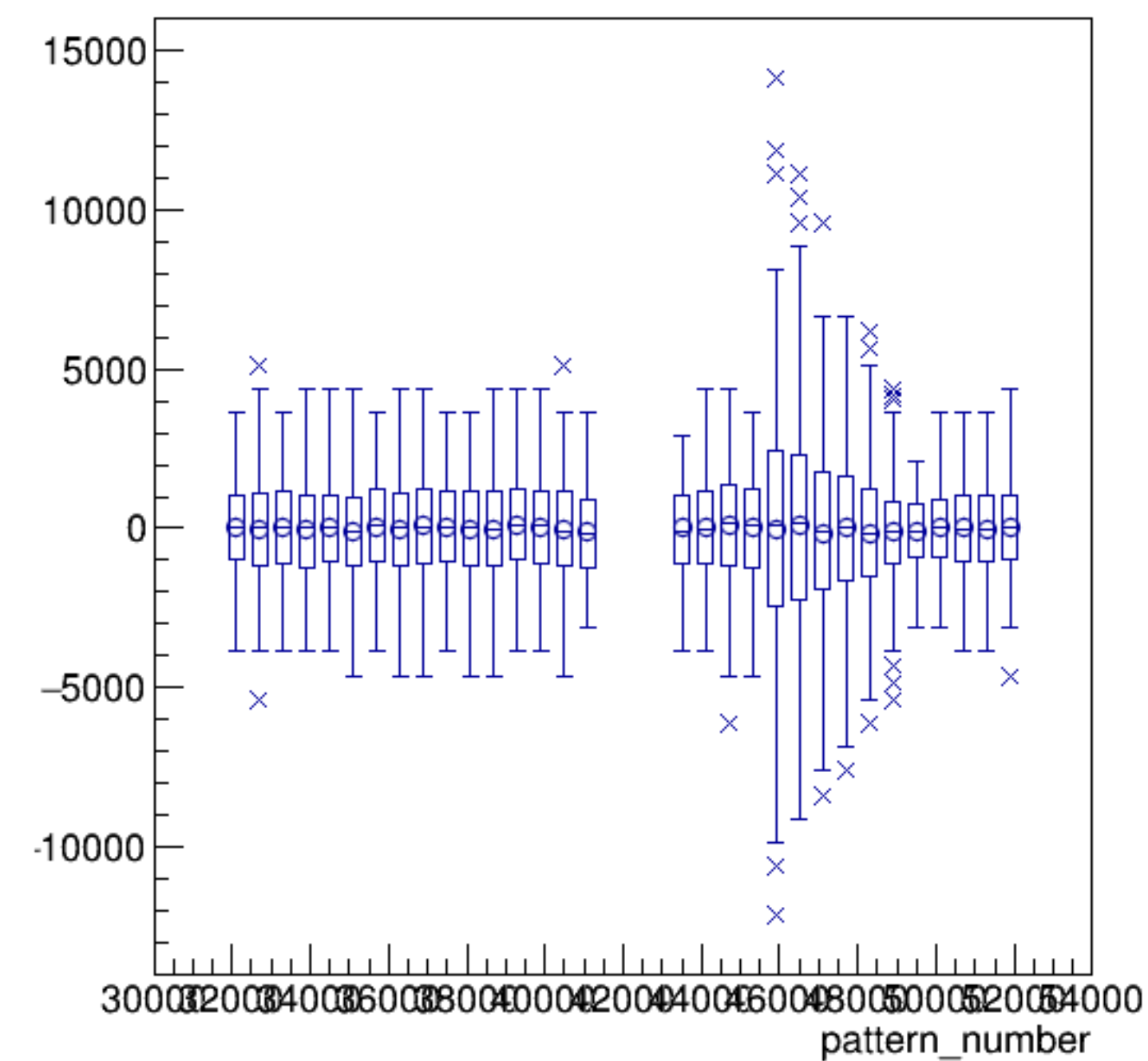
asym_sam7/ppm:pattern_number {ErrorFlag==0}
