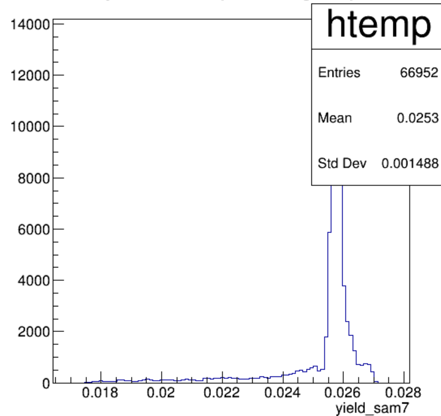
yield_sam7 {ErrorFlag==0}
