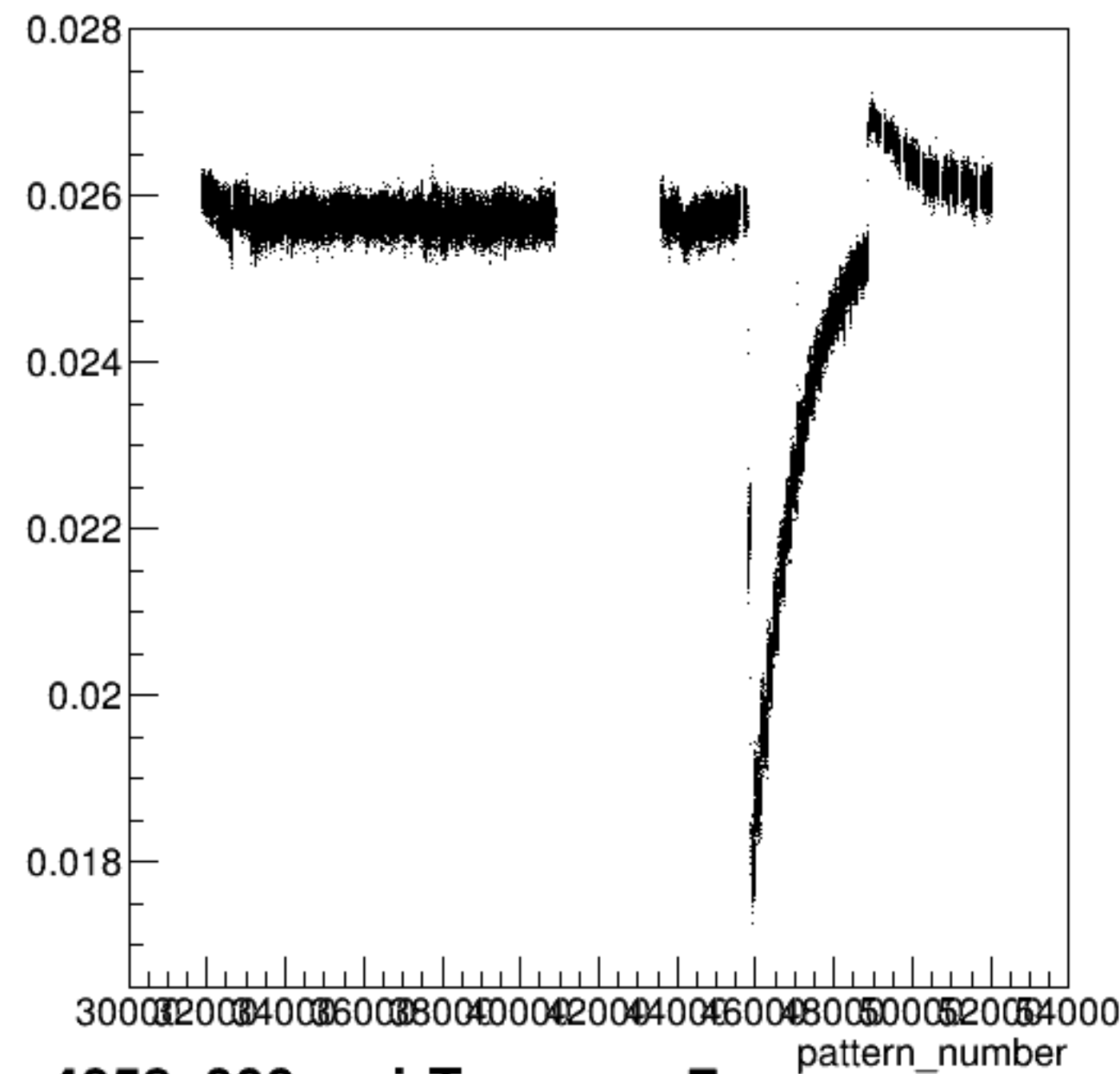
yield_sam7:pattern_number {ErrorFlag==0}
