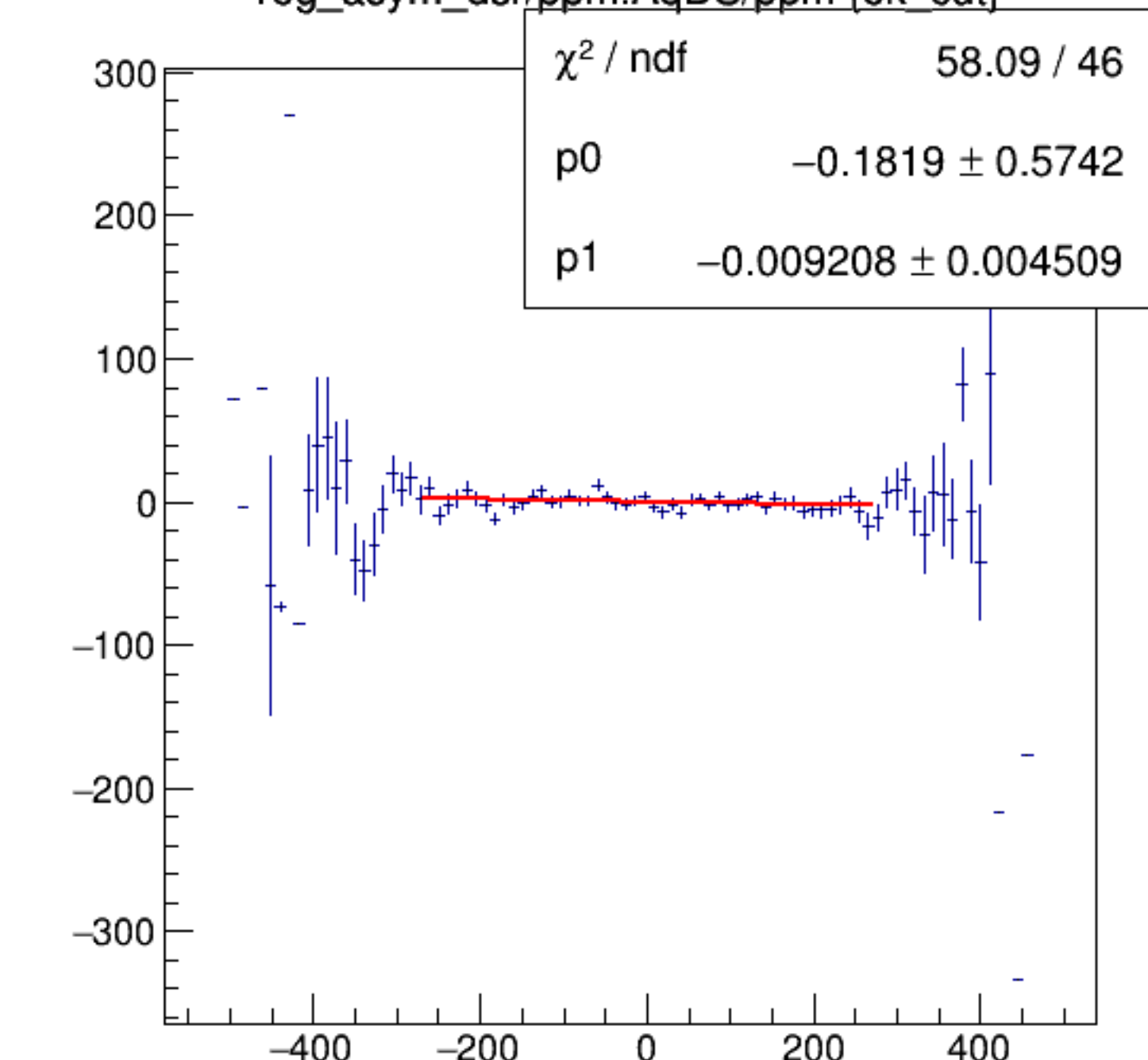
reg_asym_dsr/ppm:AqDS/ppm {ok_cut}
