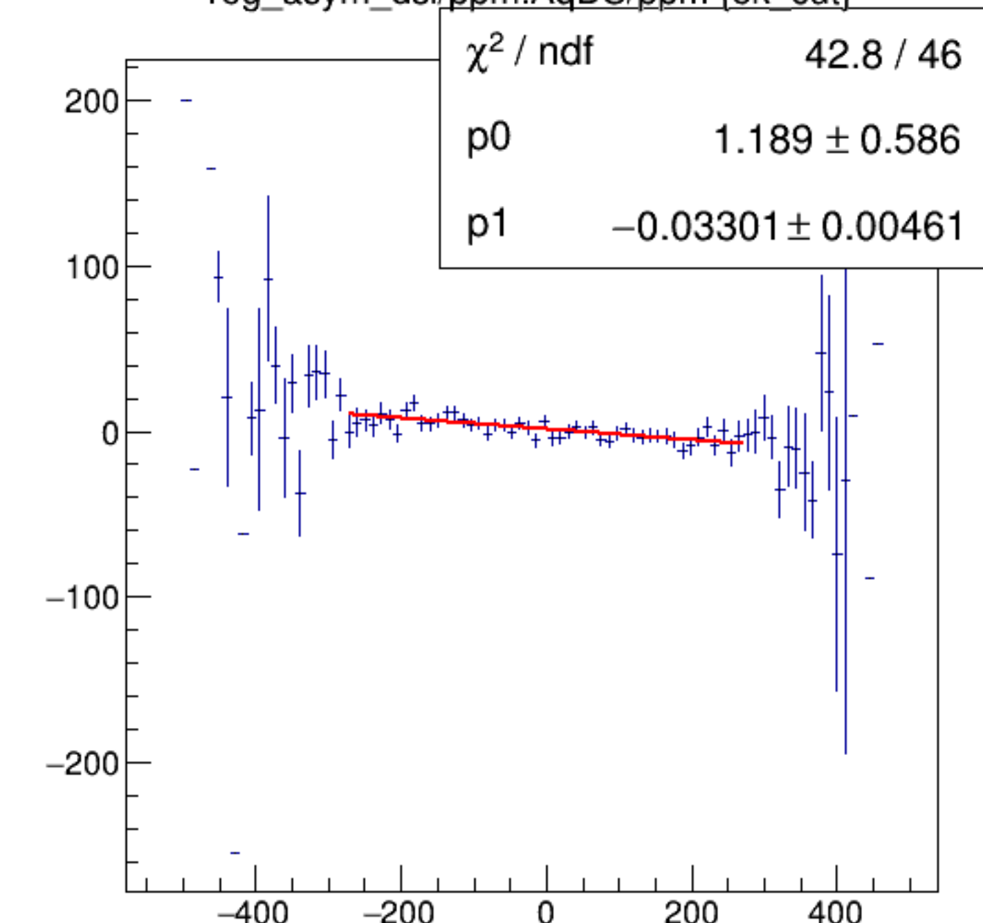
reg_asym_dsl/ppm:AqDS/ppm {ok_cut}
