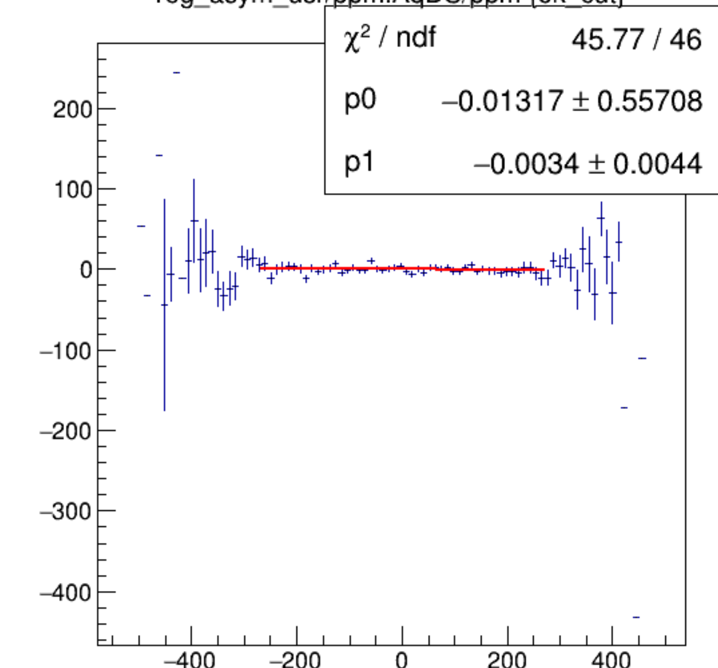
reg_asym_usr/ppm:AqDS/ppm {ok_cut}
