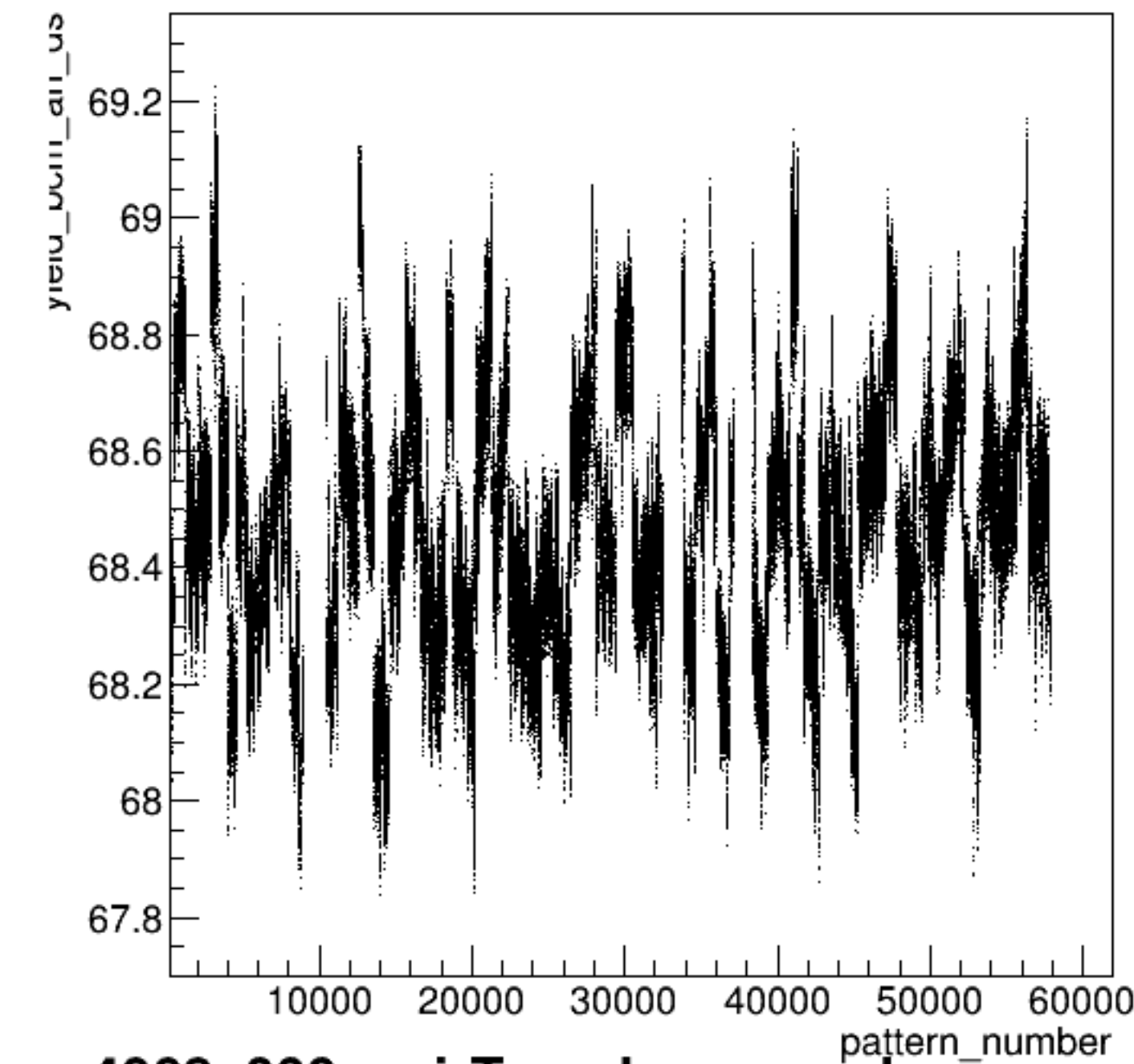
yield_bcm_an_ds:pattern_number {ErrorFlag==0}
