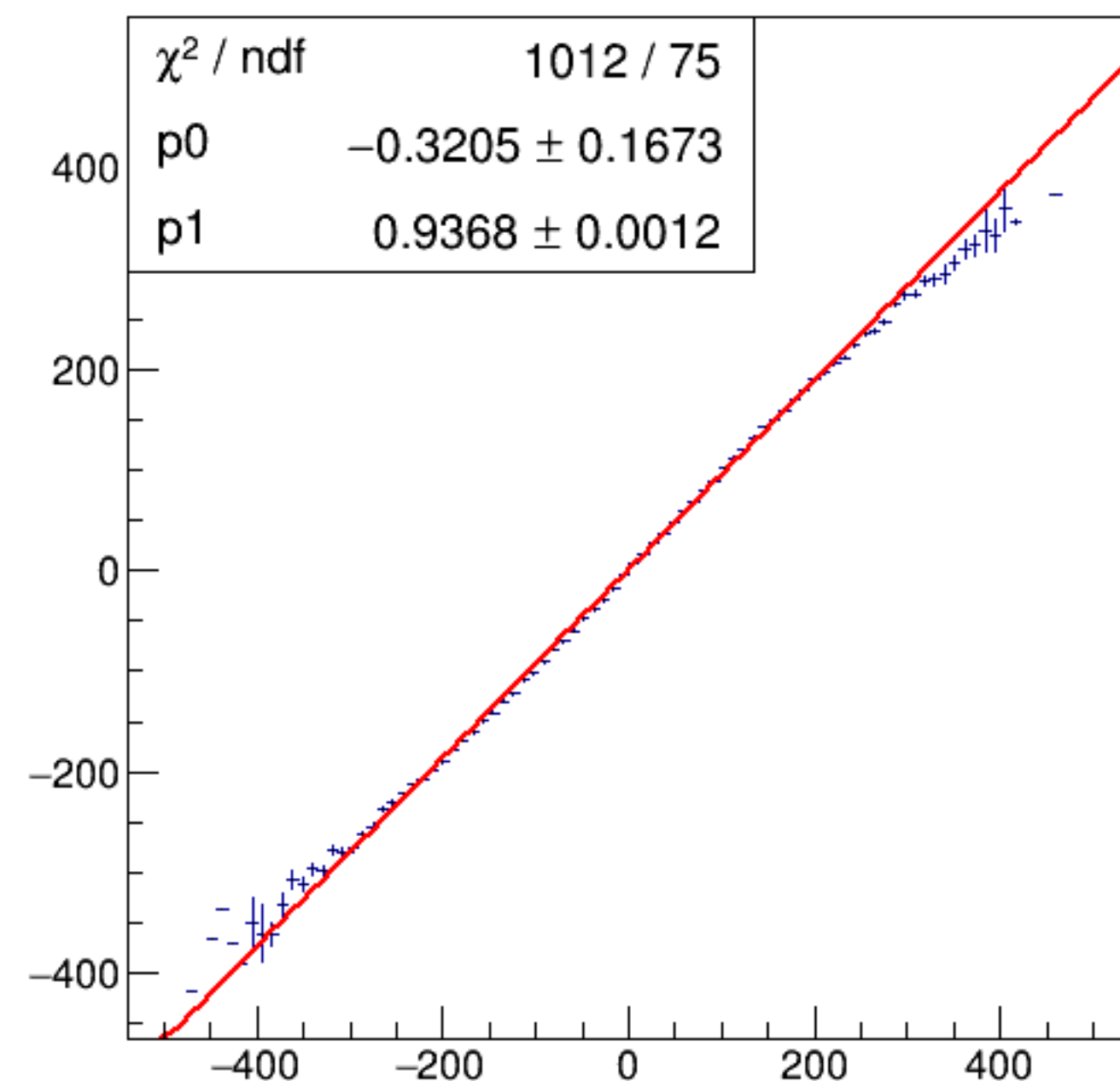
run4068_000_asym_bcm_an_us_vs_asym_bcm_an_ds3_mul.png
