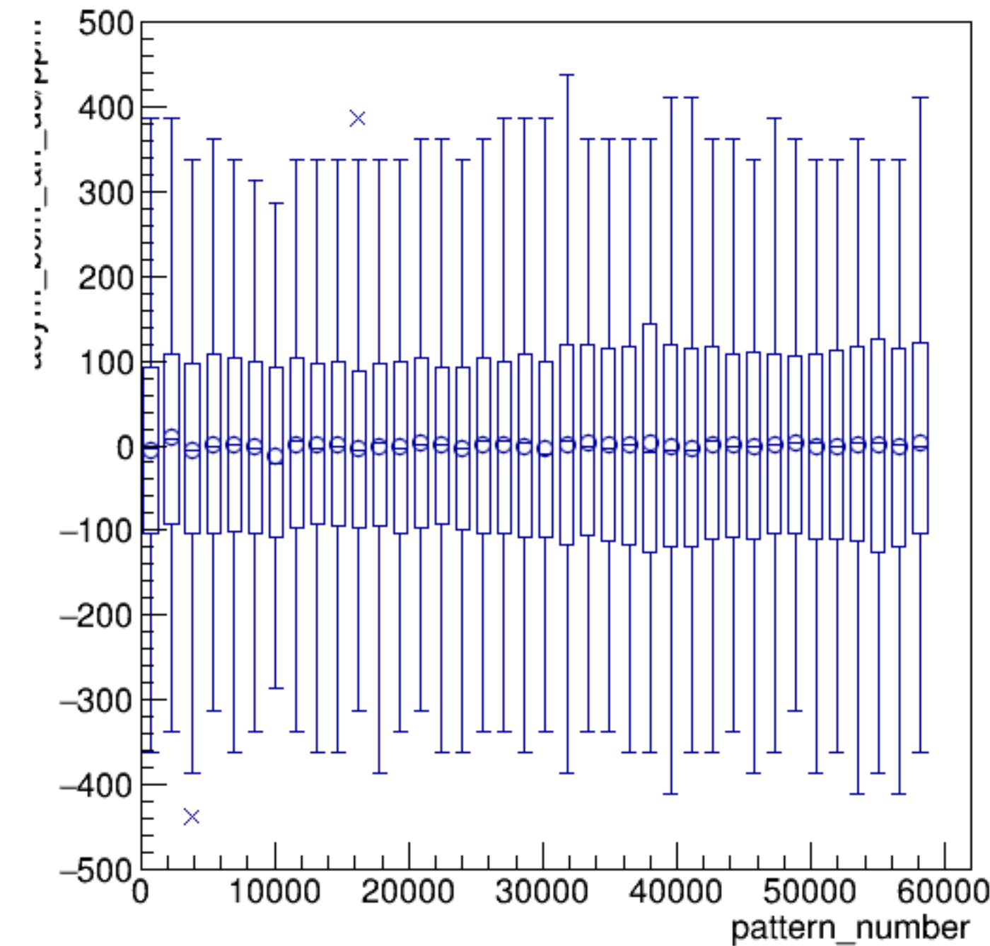
asym_bcm_an_us/ppm:pattern_number {ErrorFlag==0}
