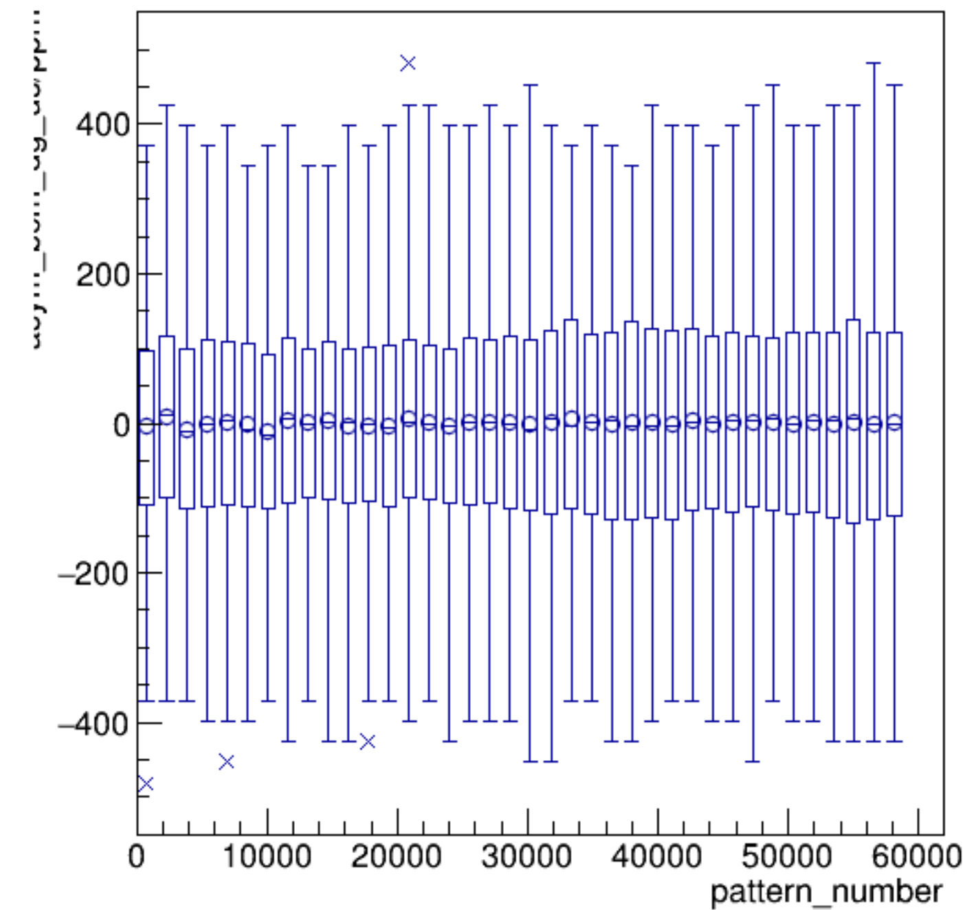
asym_bcm_dg_us/ppm:pattern_number {ErrorFlag==0}
