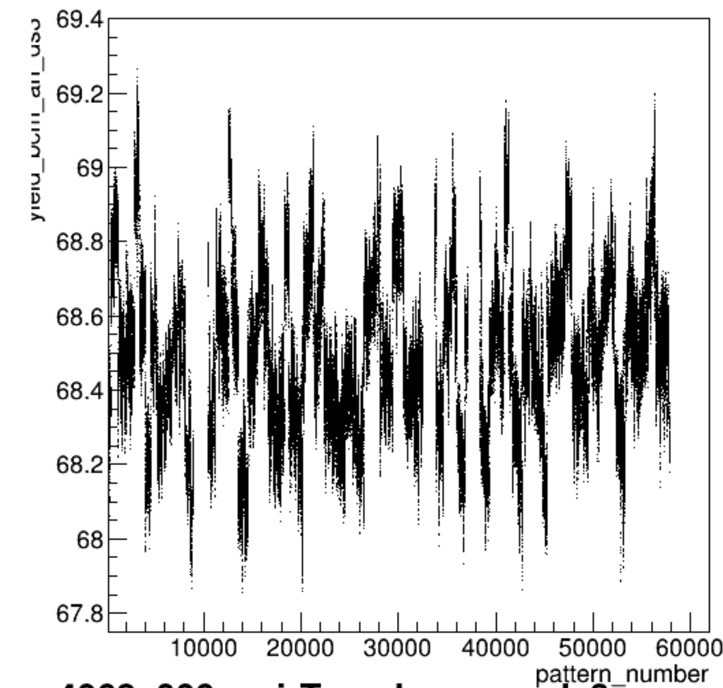
yield_bcm_an_ds3:pattern_number {ErrorFlag==0}
