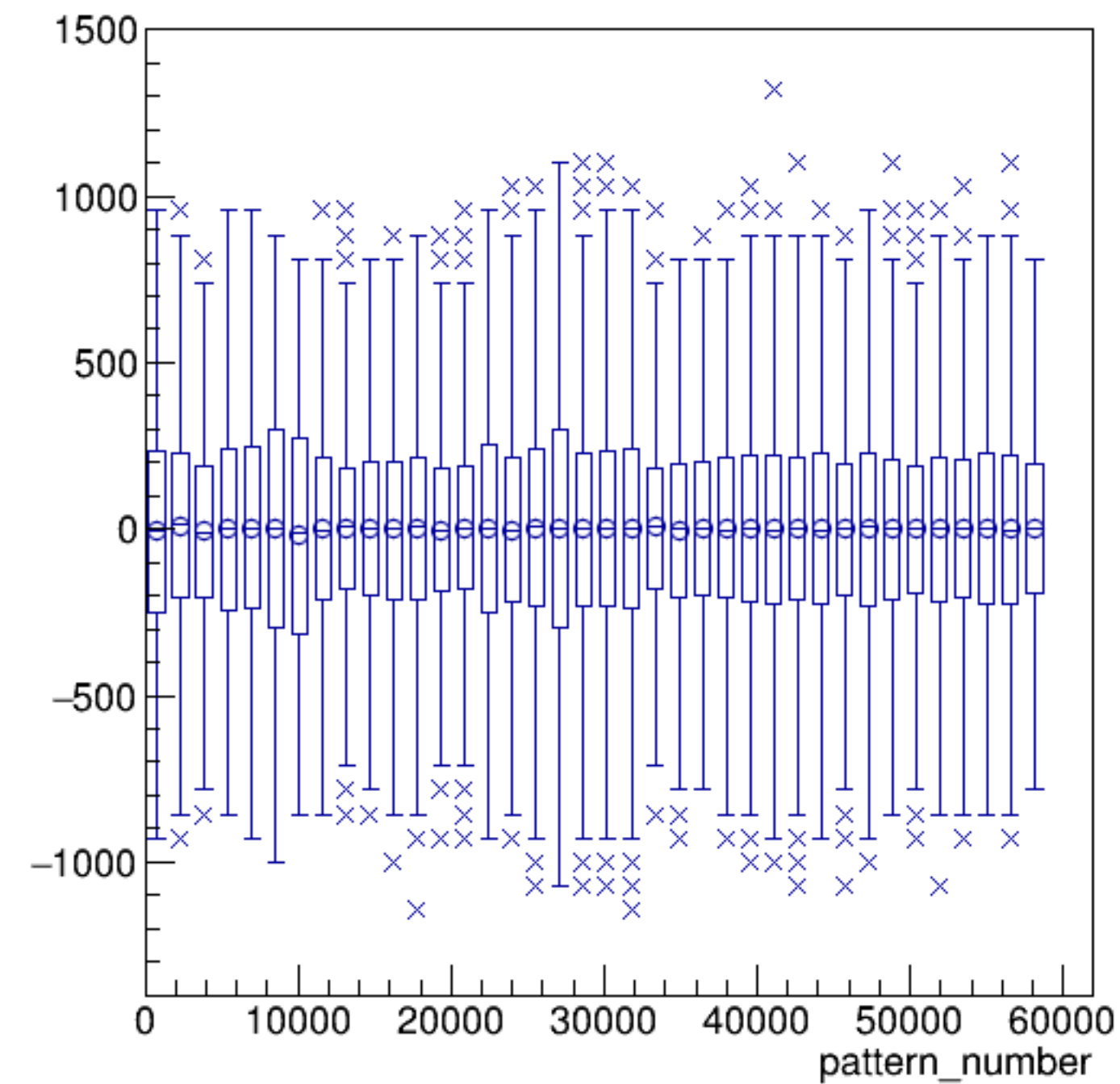
asym_bcm_an_ds3/ppm:pattern_number {ErrorFlag==0}
