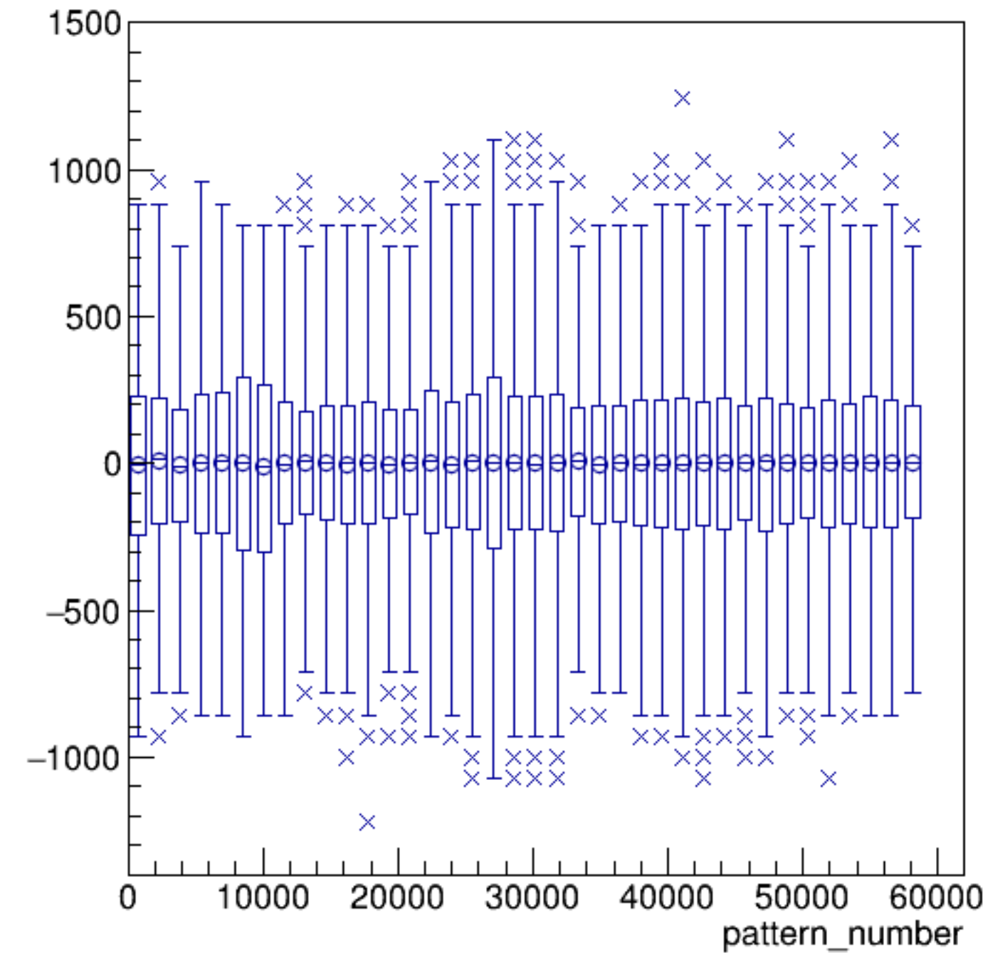
asym_bcm_an_ds/ppm:pattern_number {ErrorFlag==0}
