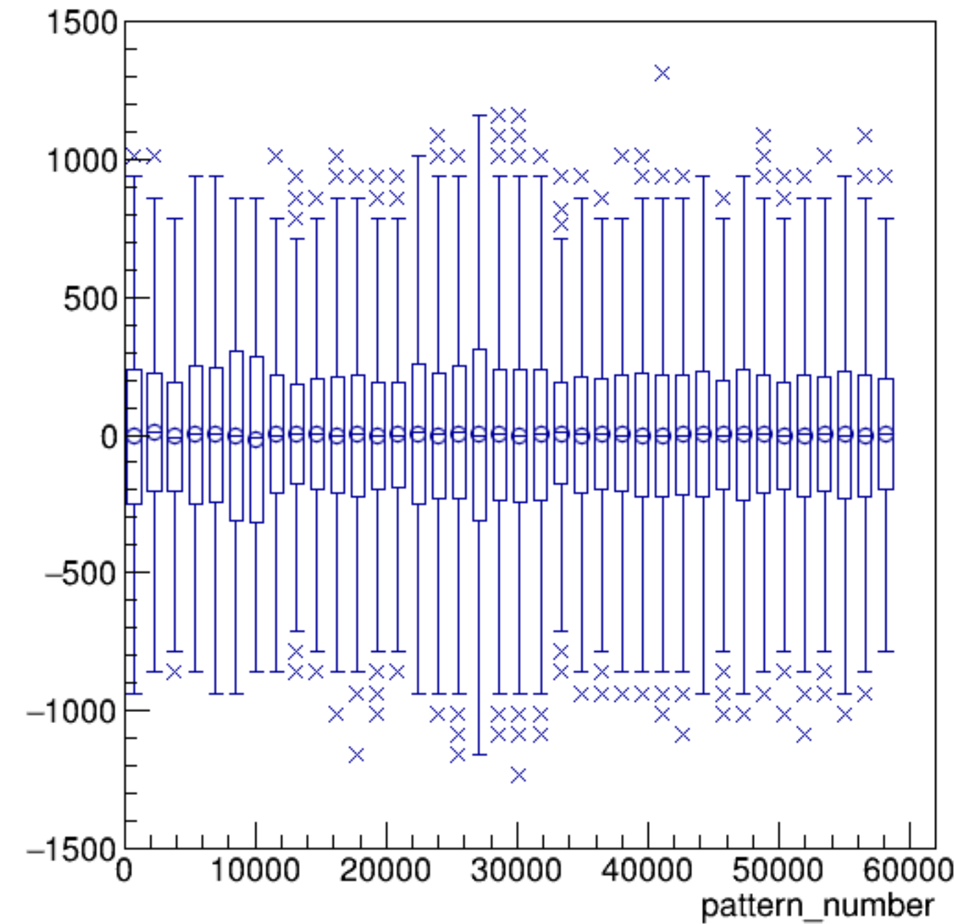
asym_bcm_dg_ds/ppm:pattern_number {ErrorFlag==0}
