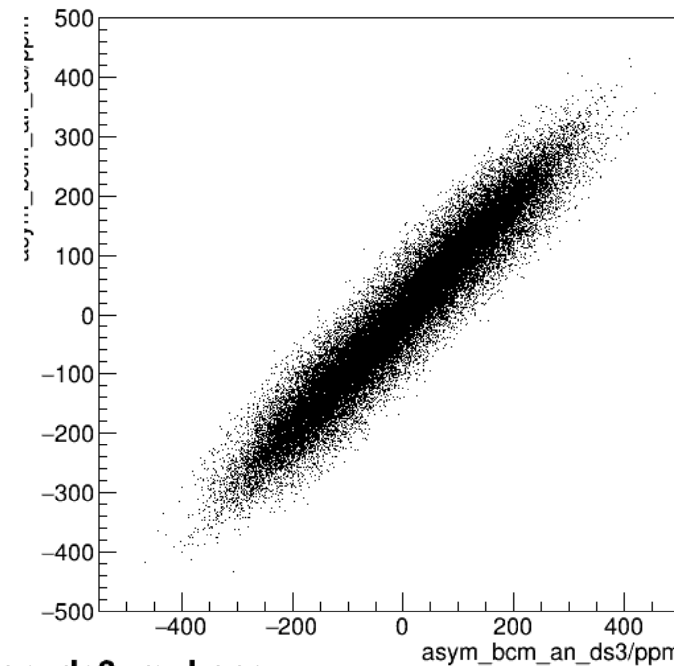
run4068_000_asym_bcm_an_us_vs_asym_bcm_an_ds3_mul.png
