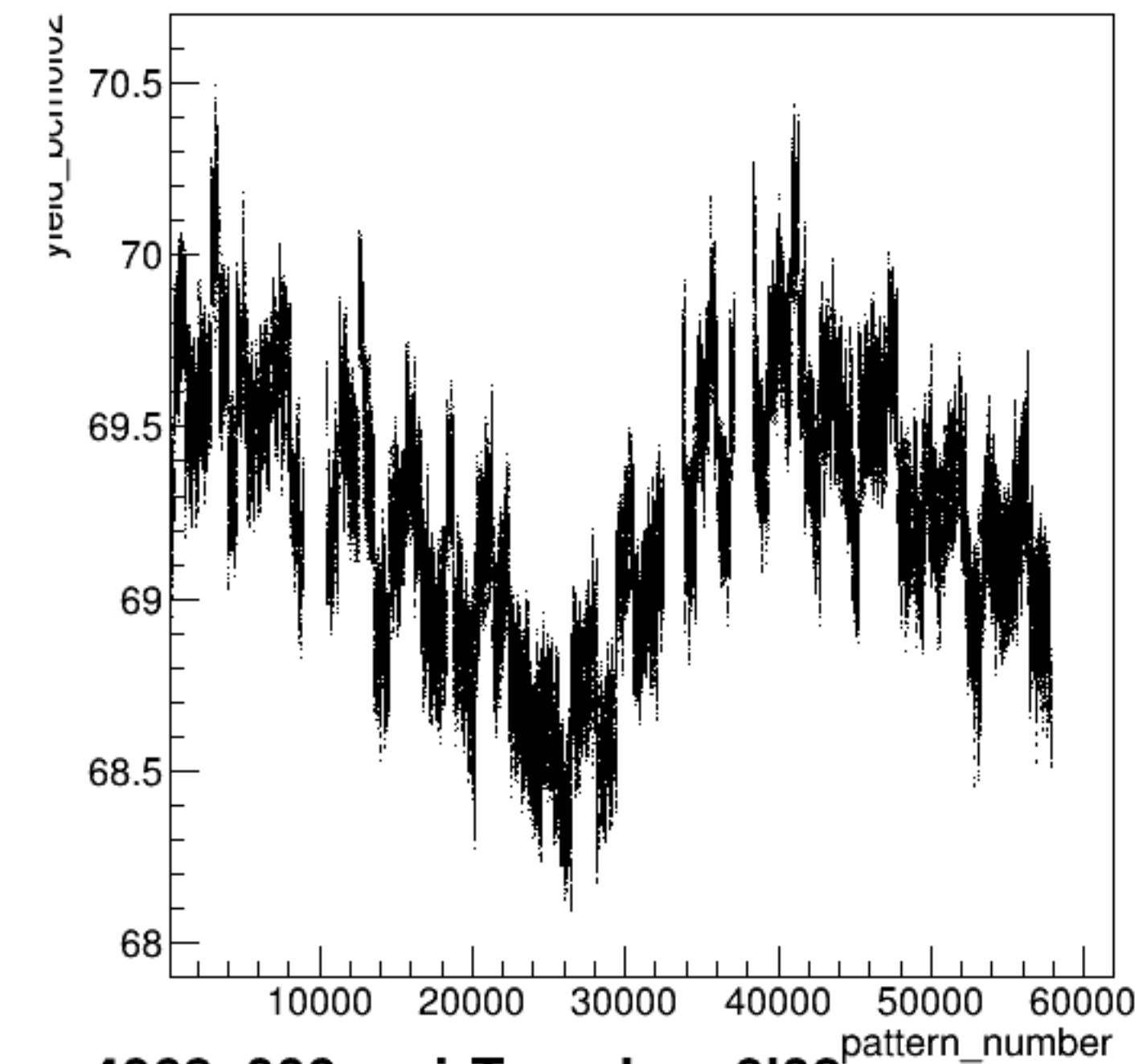
yield_bcm0l02:pattern_number {ErrorFlag==0}
