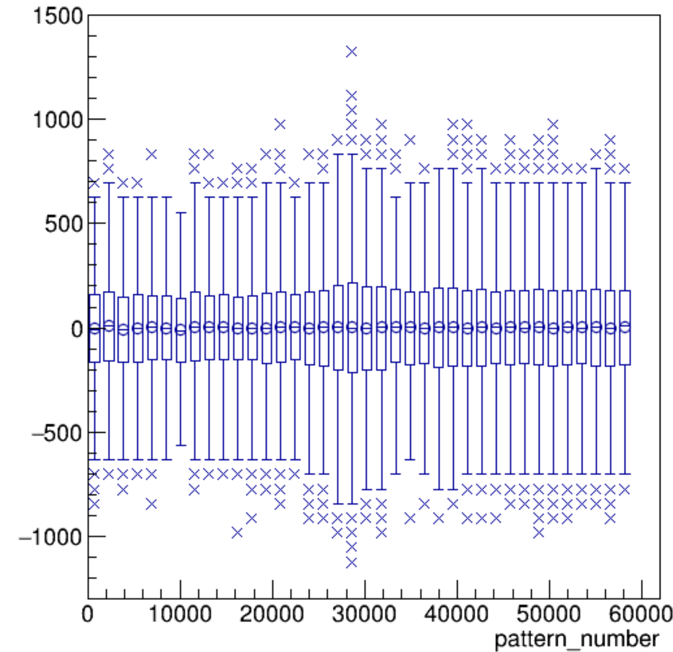
asym_bcm_dg_us/ppm:pattern_number {ErrorFlag==0}
