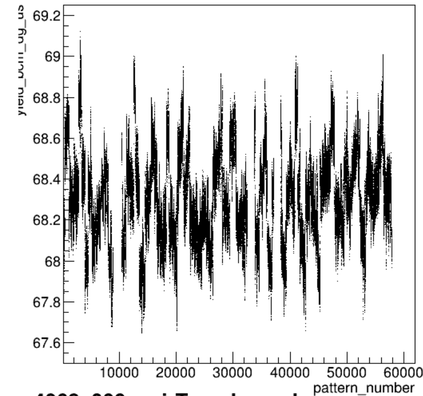
yield_bcm_dg_us:pattern_number {ErrorFlag==0}
