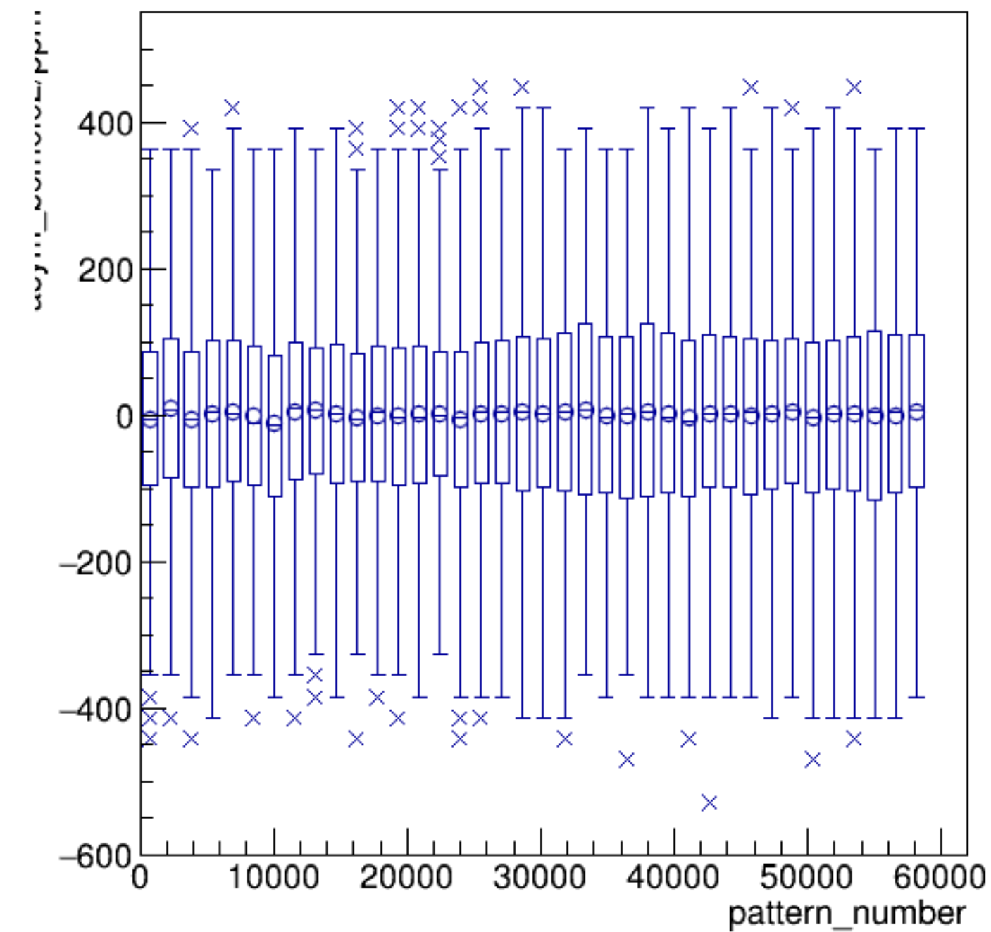
asym_bcm0l02/ppm:pattern_number {ErrorFlag==0}
