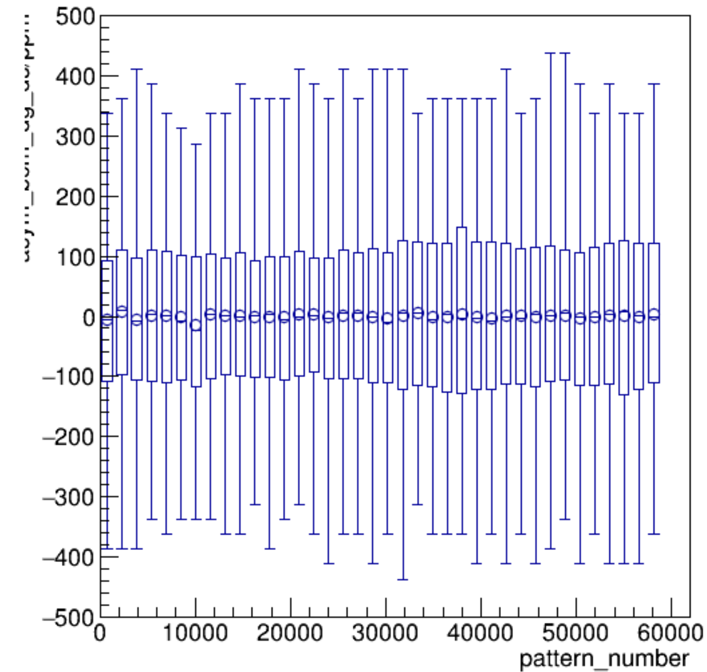
asym_bcm_dg_ds/ppm:pattern_number {ErrorFlag==0}
