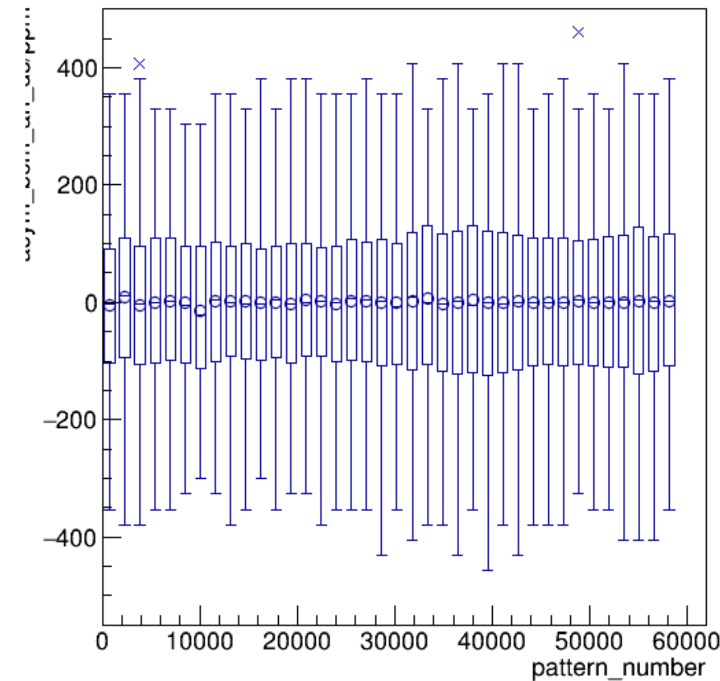
asym_bcm_an_ds/ppm:pattern_number {ErrorFlag==0}
