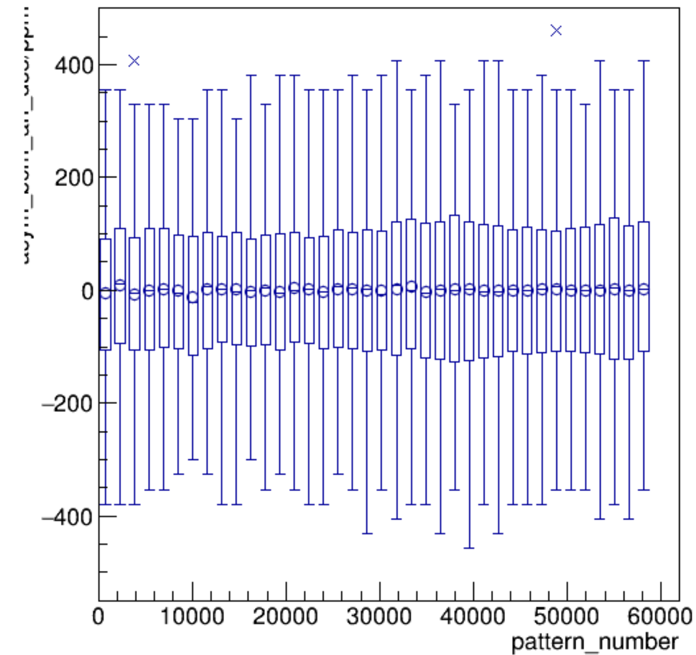
asym_bcm_an_ds3/ppm:pattern_number {ErrorFlag==0}
