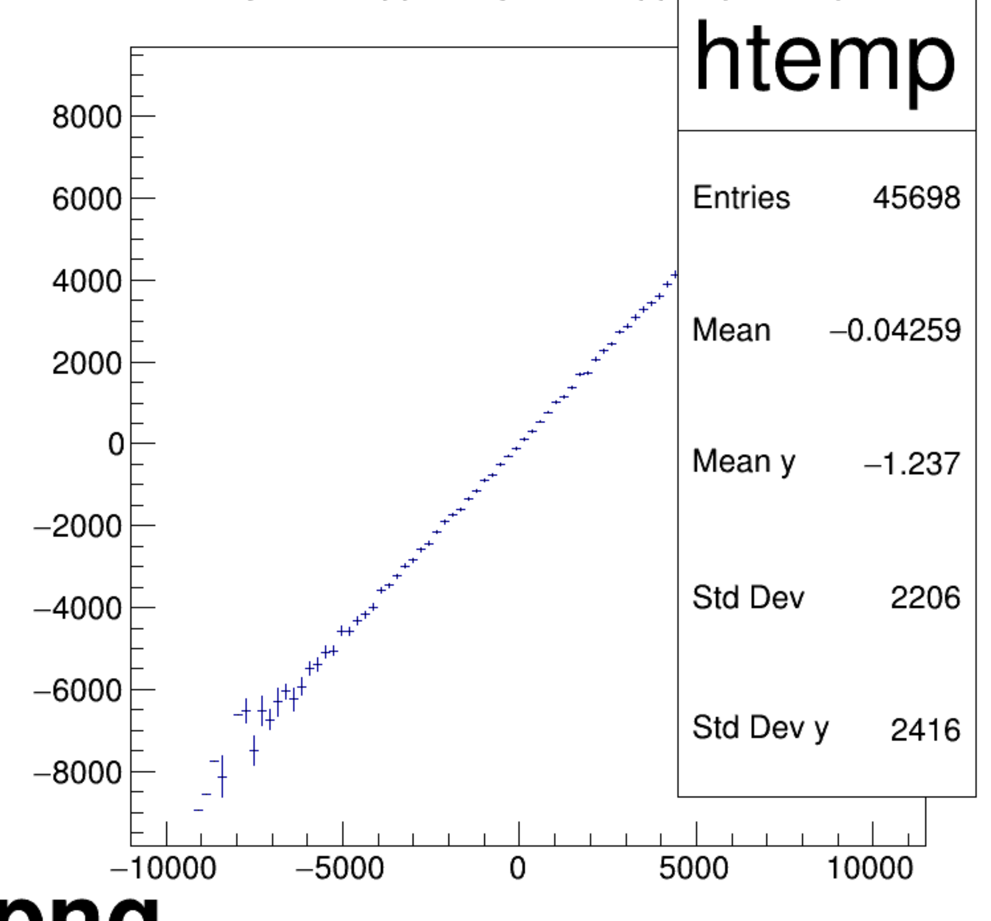
asym_atl2/ppm:asym_atr2/ppm {ok_cut}
