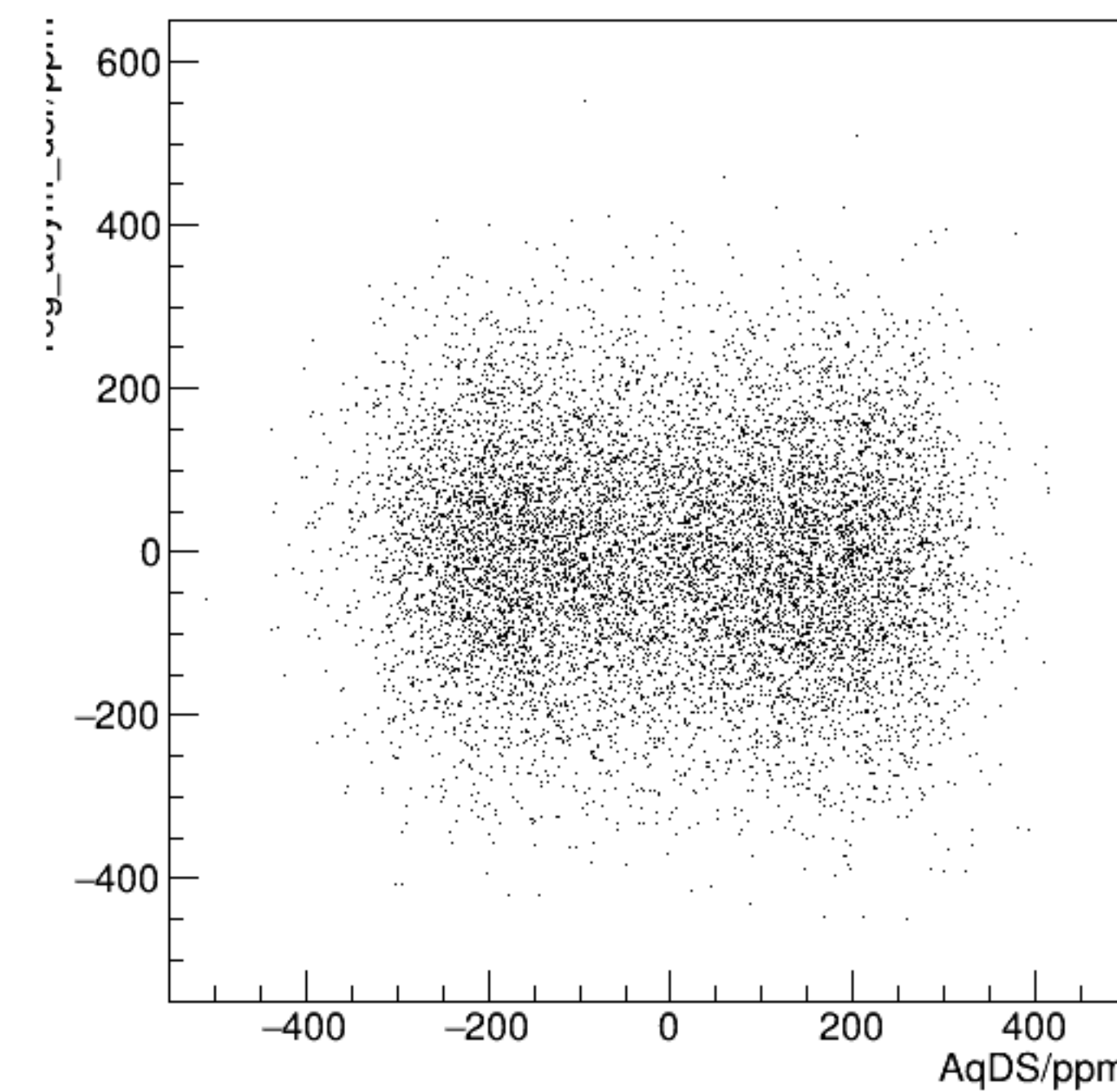
reg_asym_dsr/ppm:AqDS/ppm {ok_cut}
