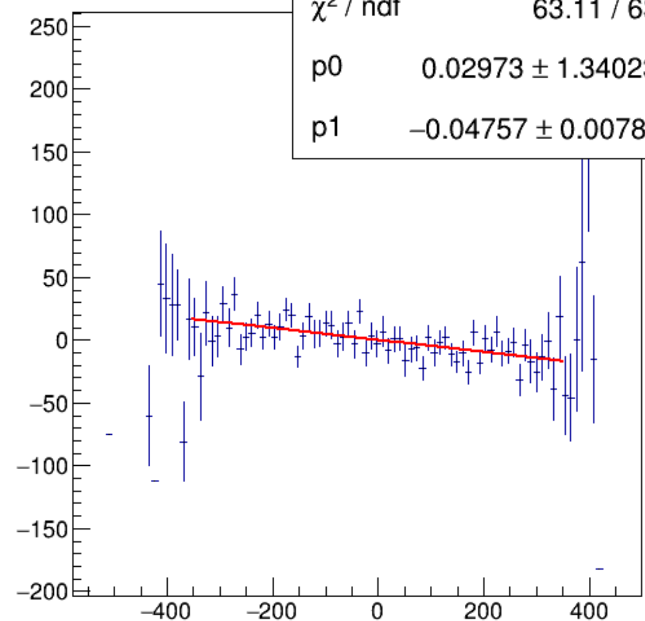
reg_asym_dsl/ppm:AqDS/ppm {ok_cut}
