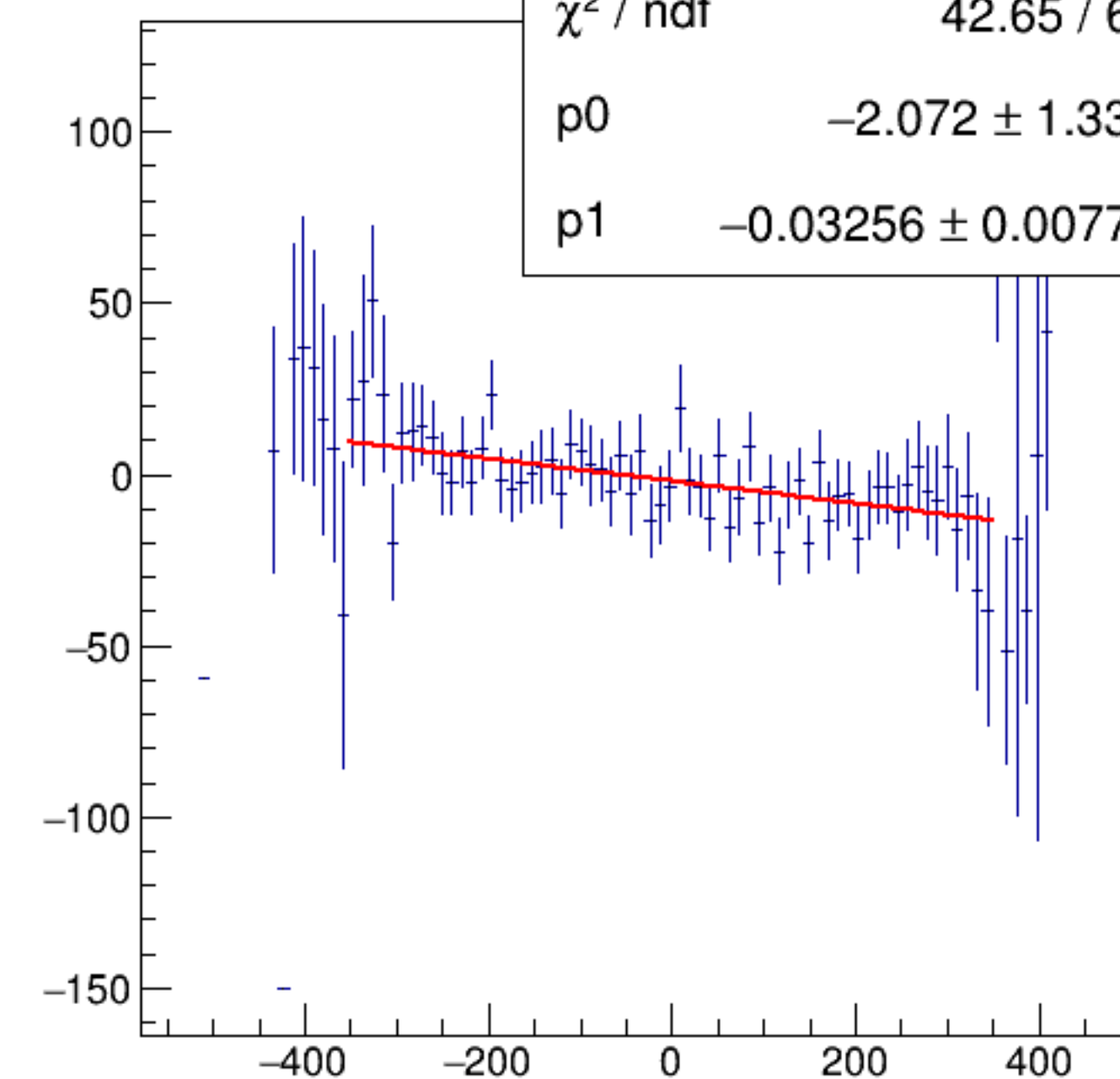
reg_asym_dsr/ppm:AqDS/ppm {ok_cut}
