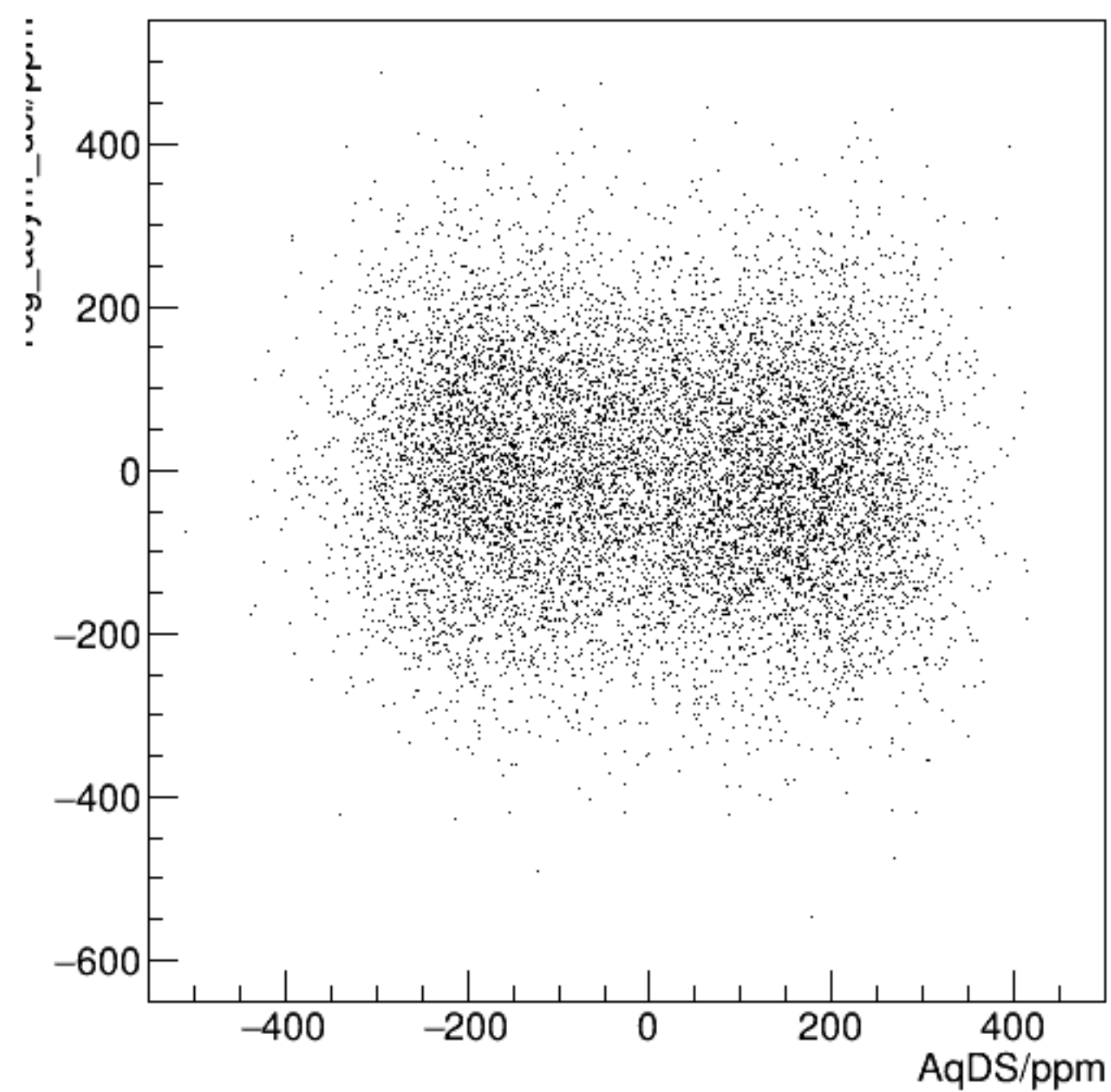
reg_asym_dsl/ppm:AqDS/ppm {ok_cut}
