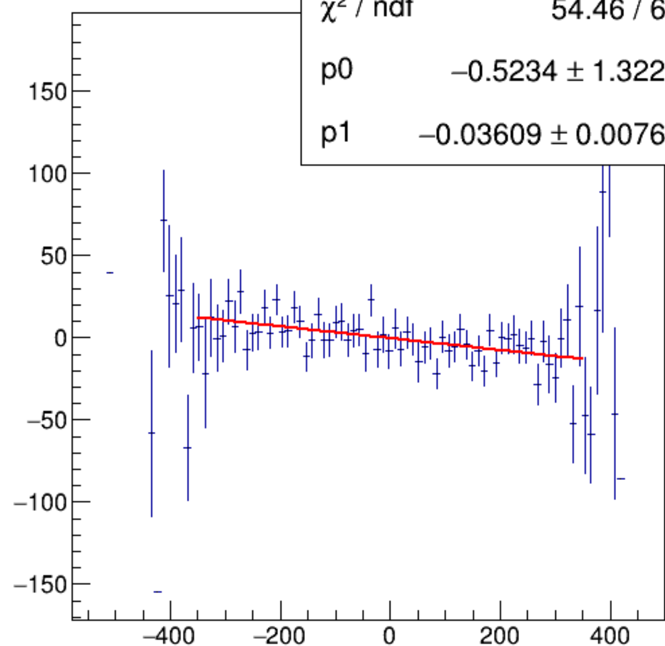
reg_asym_usl/ppm:AqDS/ppm {ok_cut}
