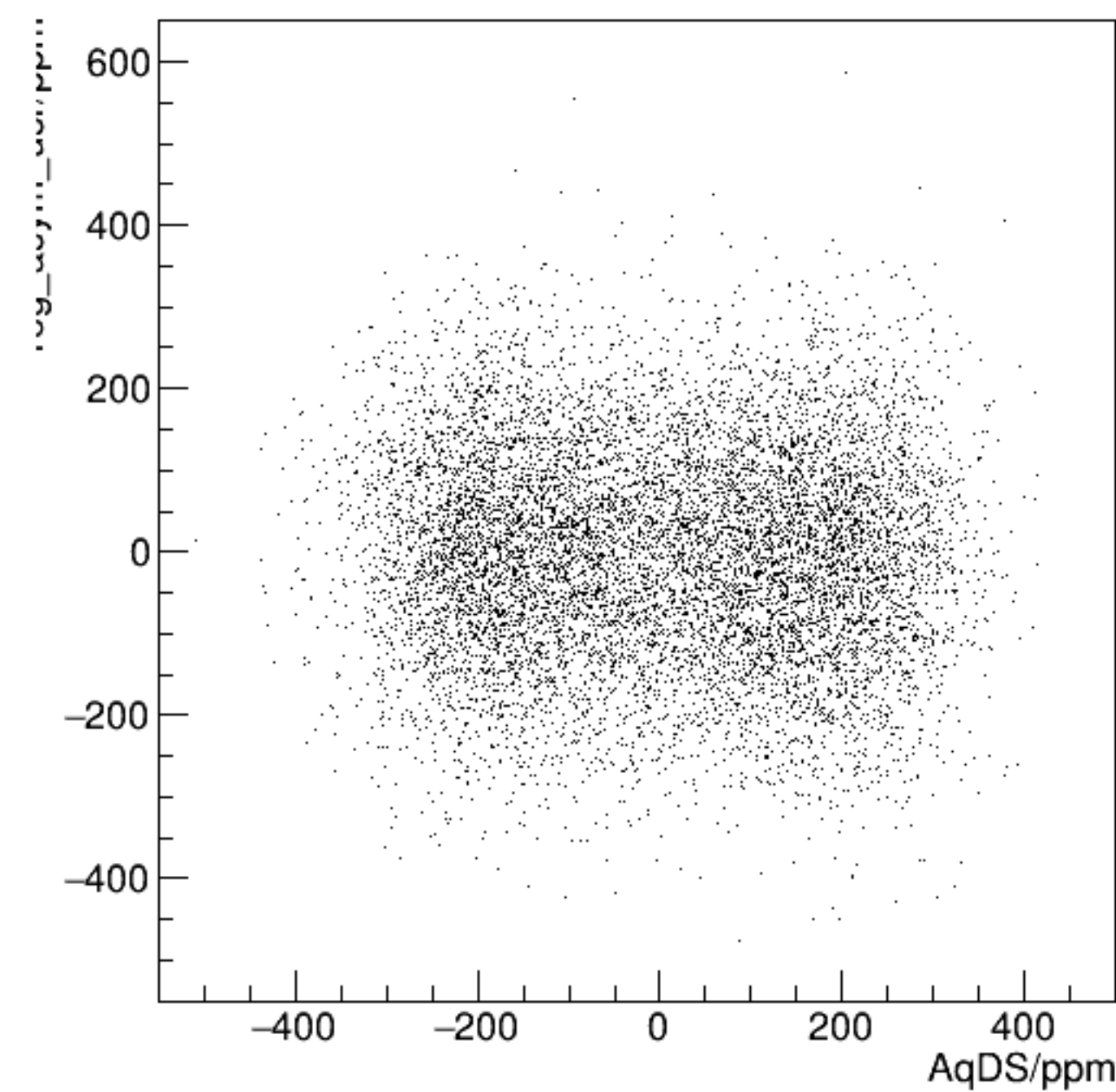
reg_asym_usr/ppm:AqDS/ppm {ok_cut}
