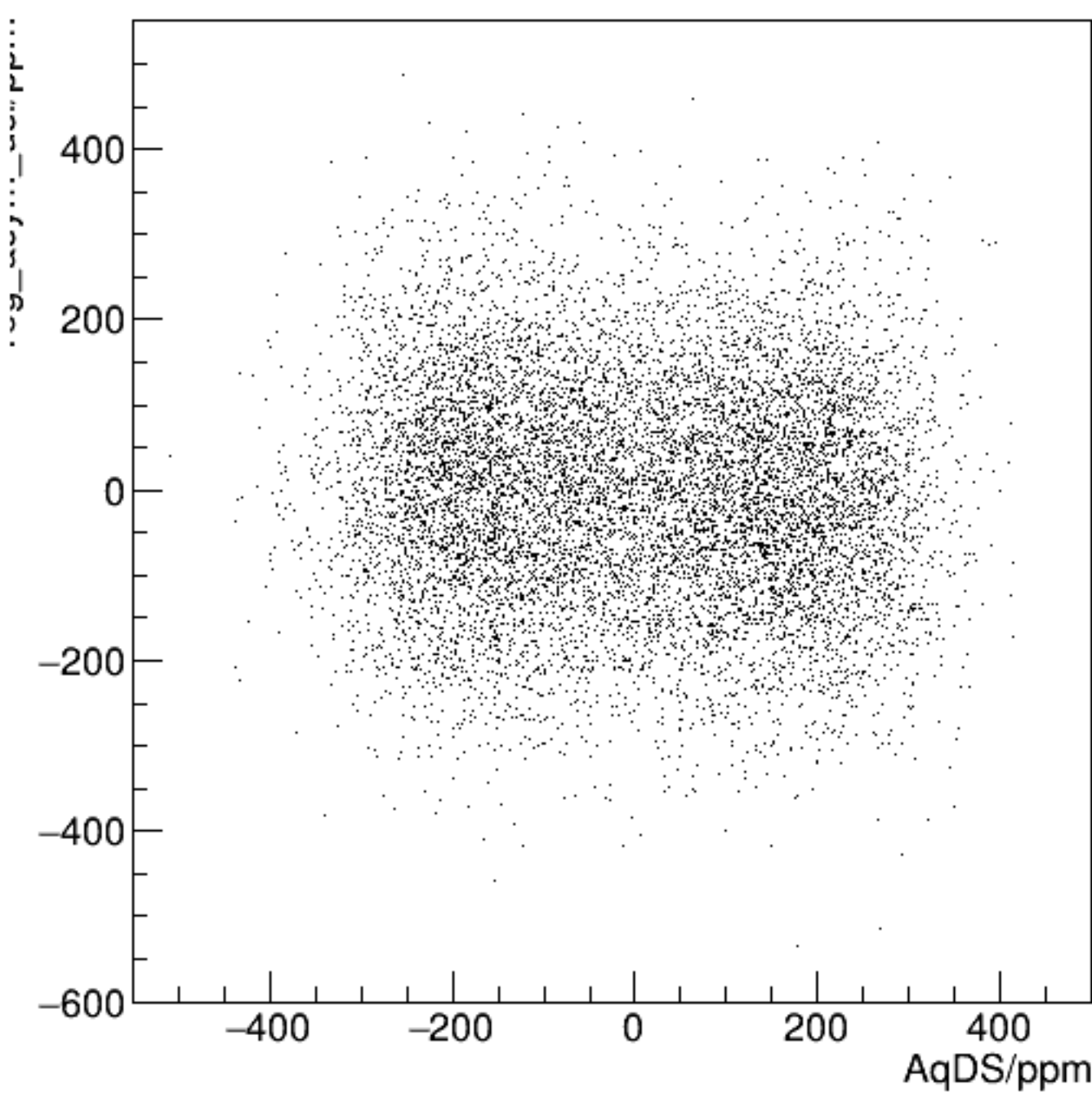
reg_asym_usl/ppm:AqDS/ppm {ok_cut}
