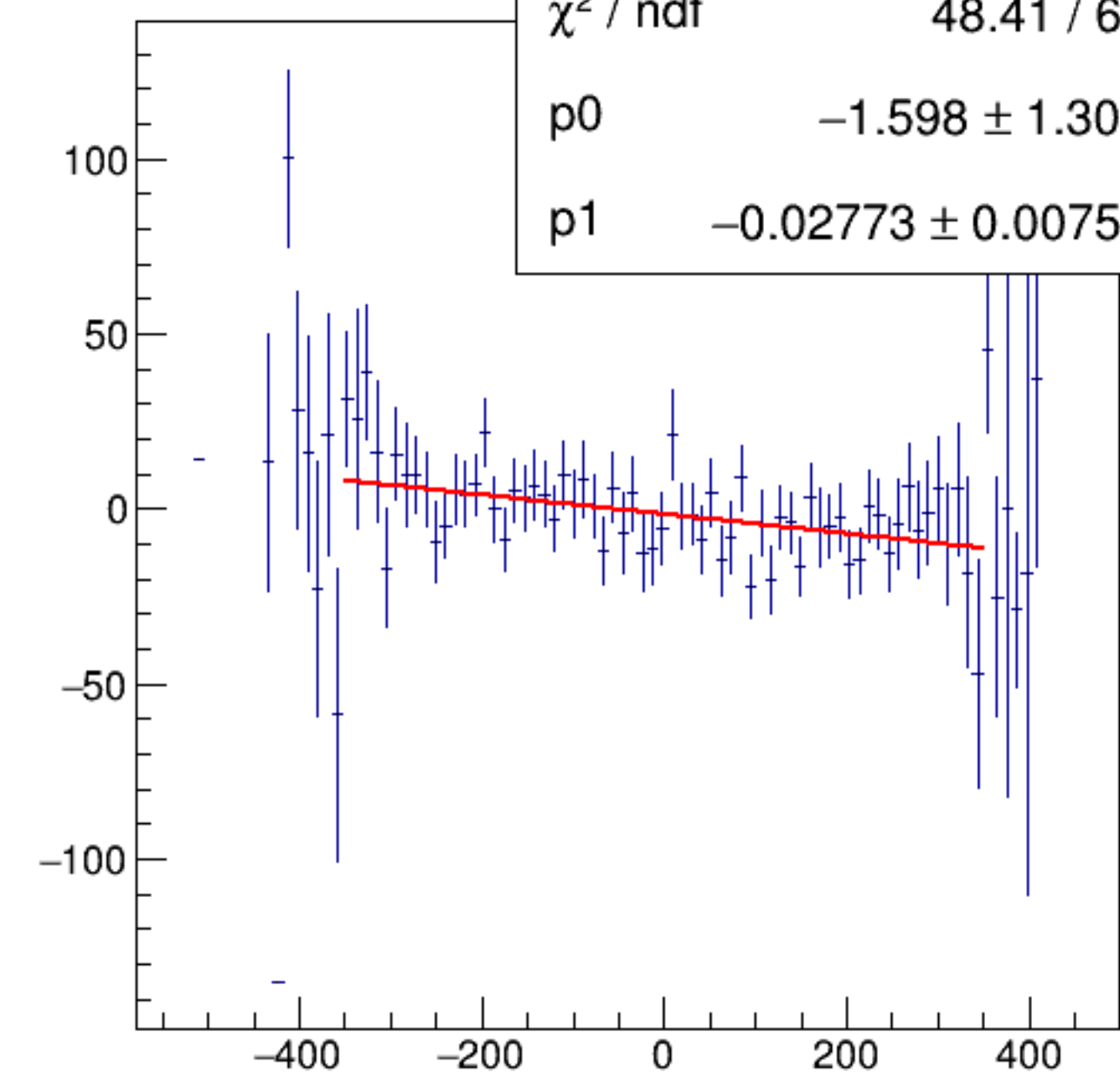
reg_asym_usr/ppm:AqDS/ppm {ok_cut}
