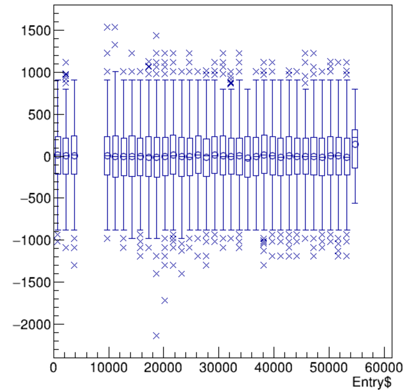
(reg_asym_atl1/ppm+reg_asym_atr1/ppm)/2:Entry$ {ok_cut}
