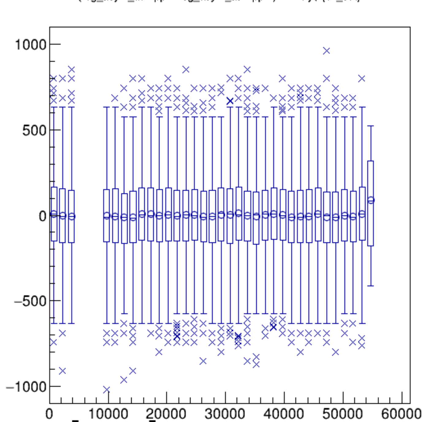
(reg_asym_atl2/ppm-reg_asym_atr2/ppm)/2:Entry$ {ok_cut}
