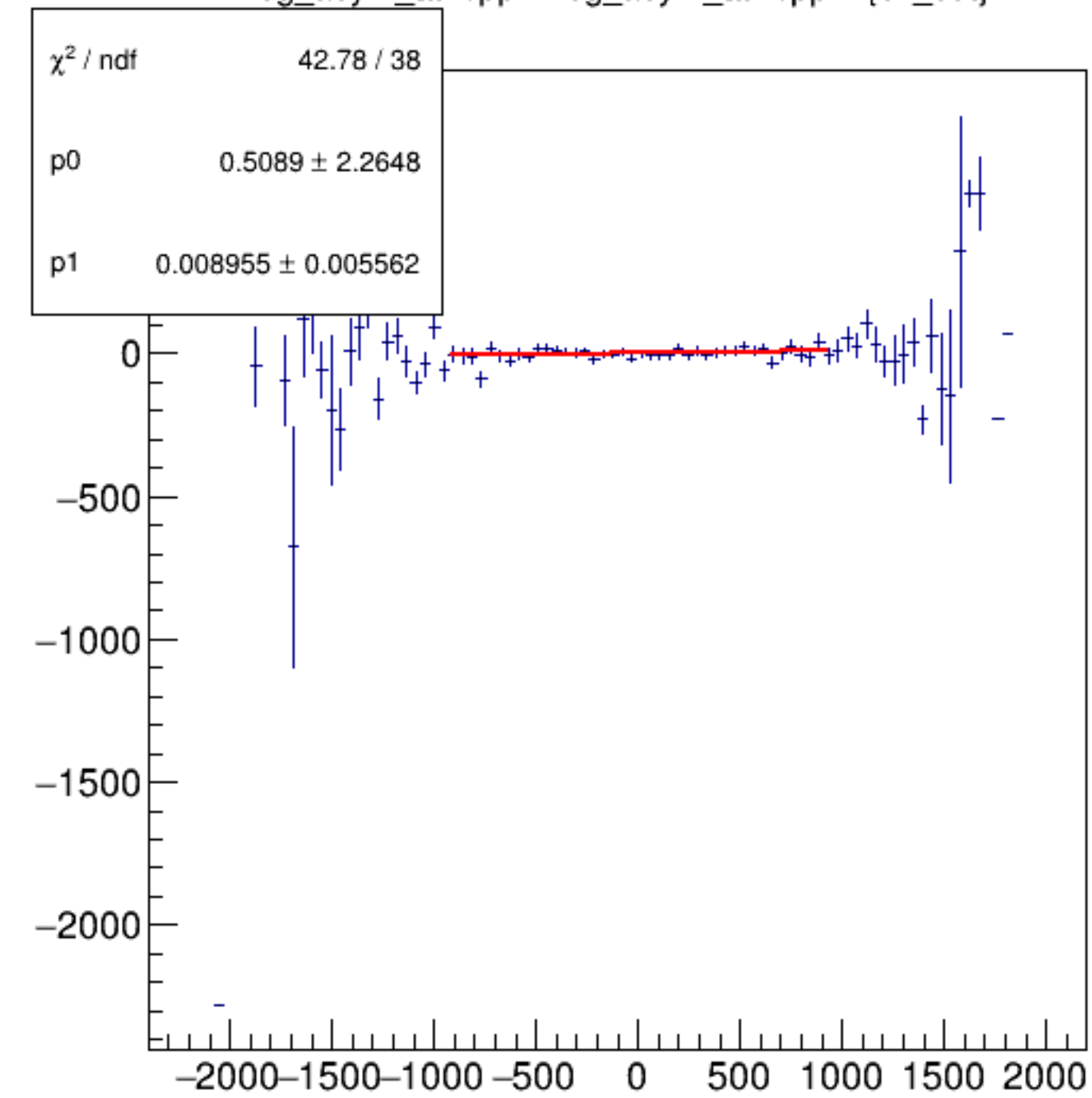
reg_asym_atl1/ppm:reg_asym_atr1/ppm {ok_cut}
