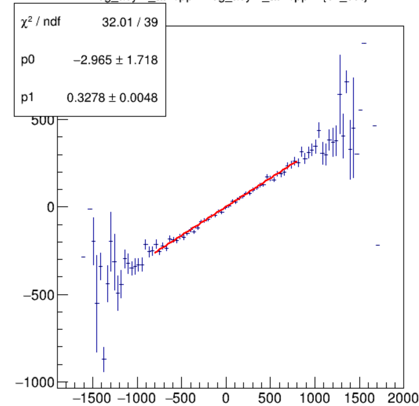
reg_asym_atl2/ppm:reg_asym_atr2/ppm {ok_cut}
