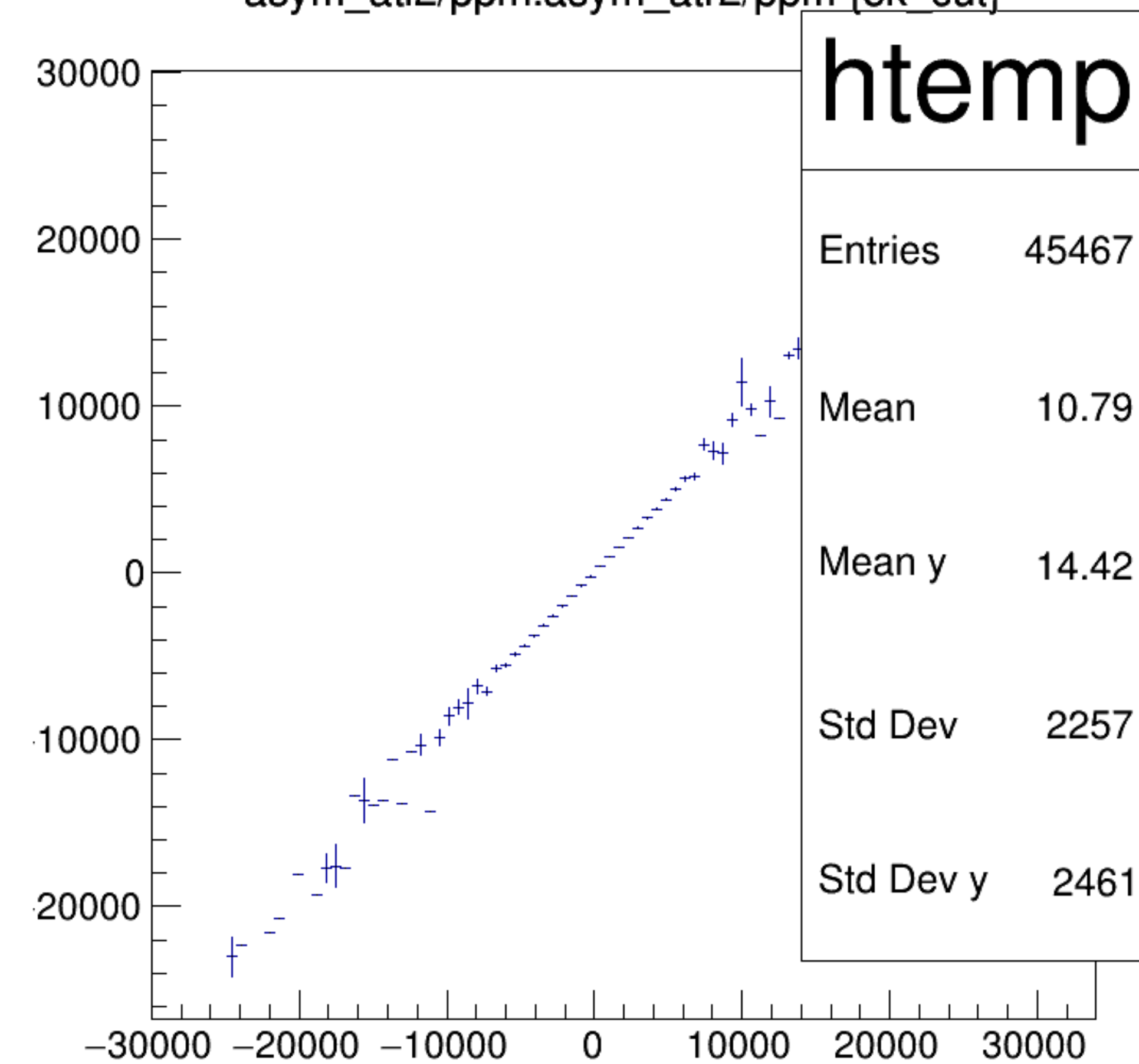
asym_atl2/ppm:asym_atr2/ppm {ok_cut}
