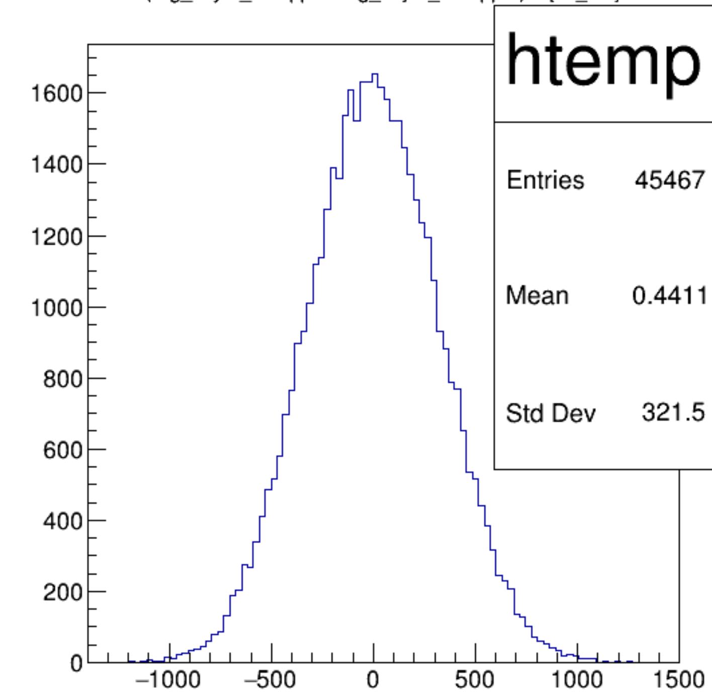
(reg_asym_atl2/ppm+reg_asym_atr2/ppm)/2 {ok_cut}
