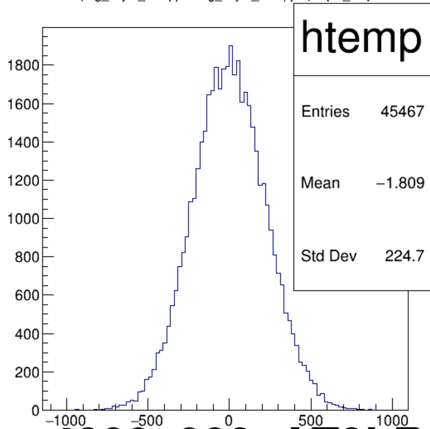
(reg_asym_atl2/ppm-reg_asym_atr2/ppm)/2 {ok_cut}
