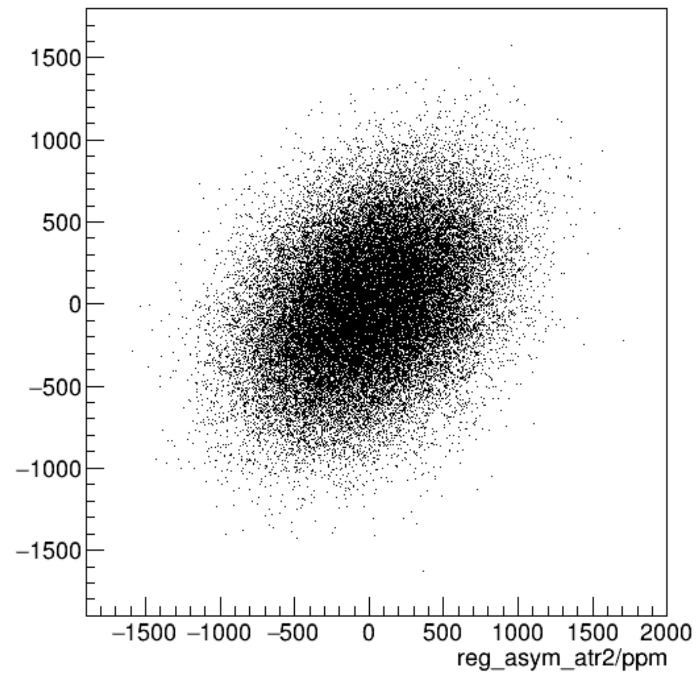
reg_asym_atl2/ppm:reg_asym_atr2/ppm {ok_cut}
