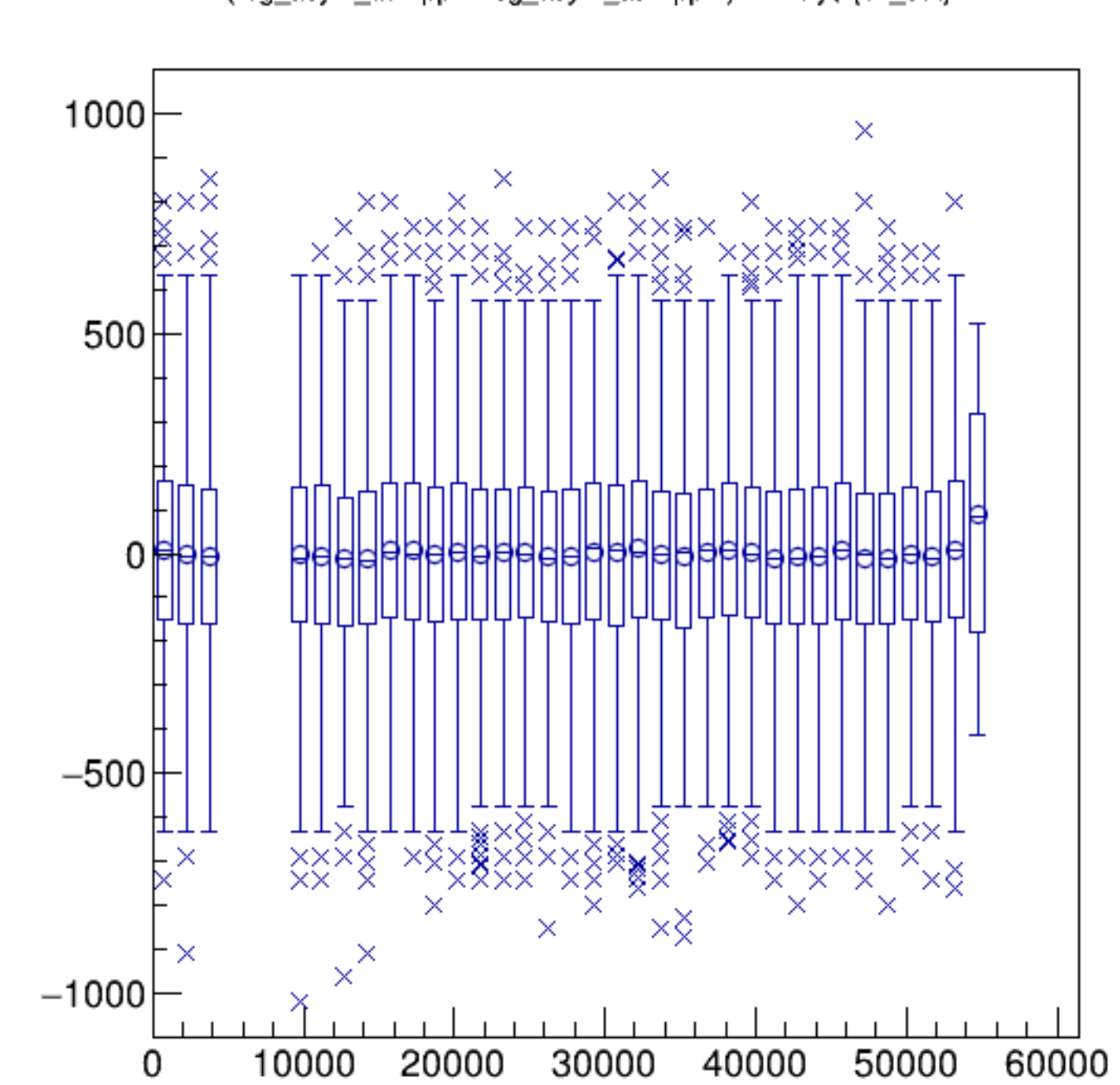
(reg_asym_atl2/ppm-reg_asym_atr2/ppm)/2:Entry$ {ok_cut}
