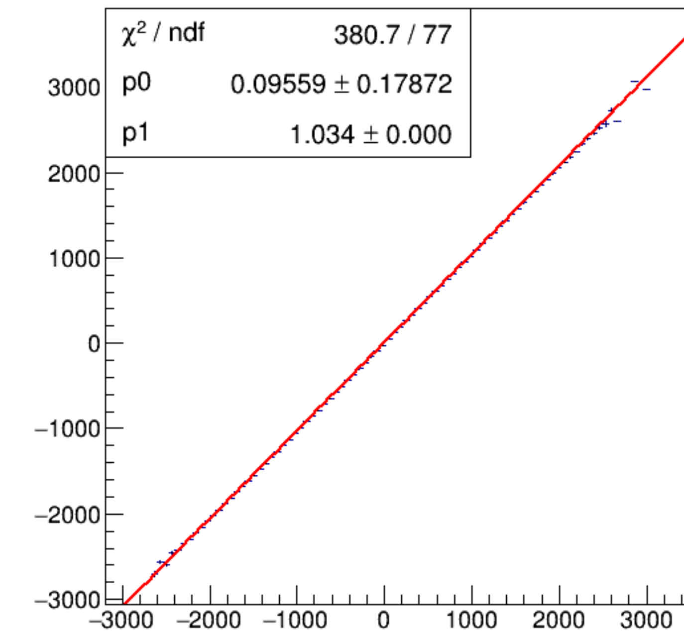
run4144_000_asym_bcm_dg_ds_vs_asym_bcm_an_us_pr.png
