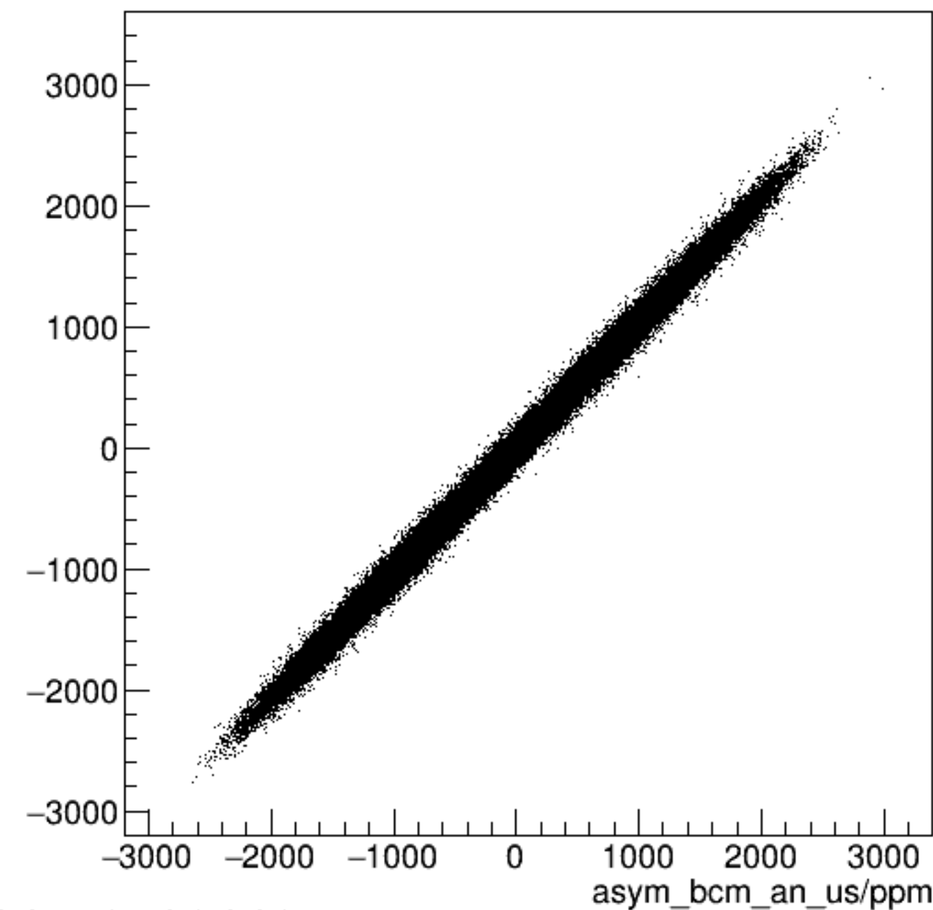
run4144_000_asym_bcm_dg_ds_vs_asym_bcm_an_us_pr.png
