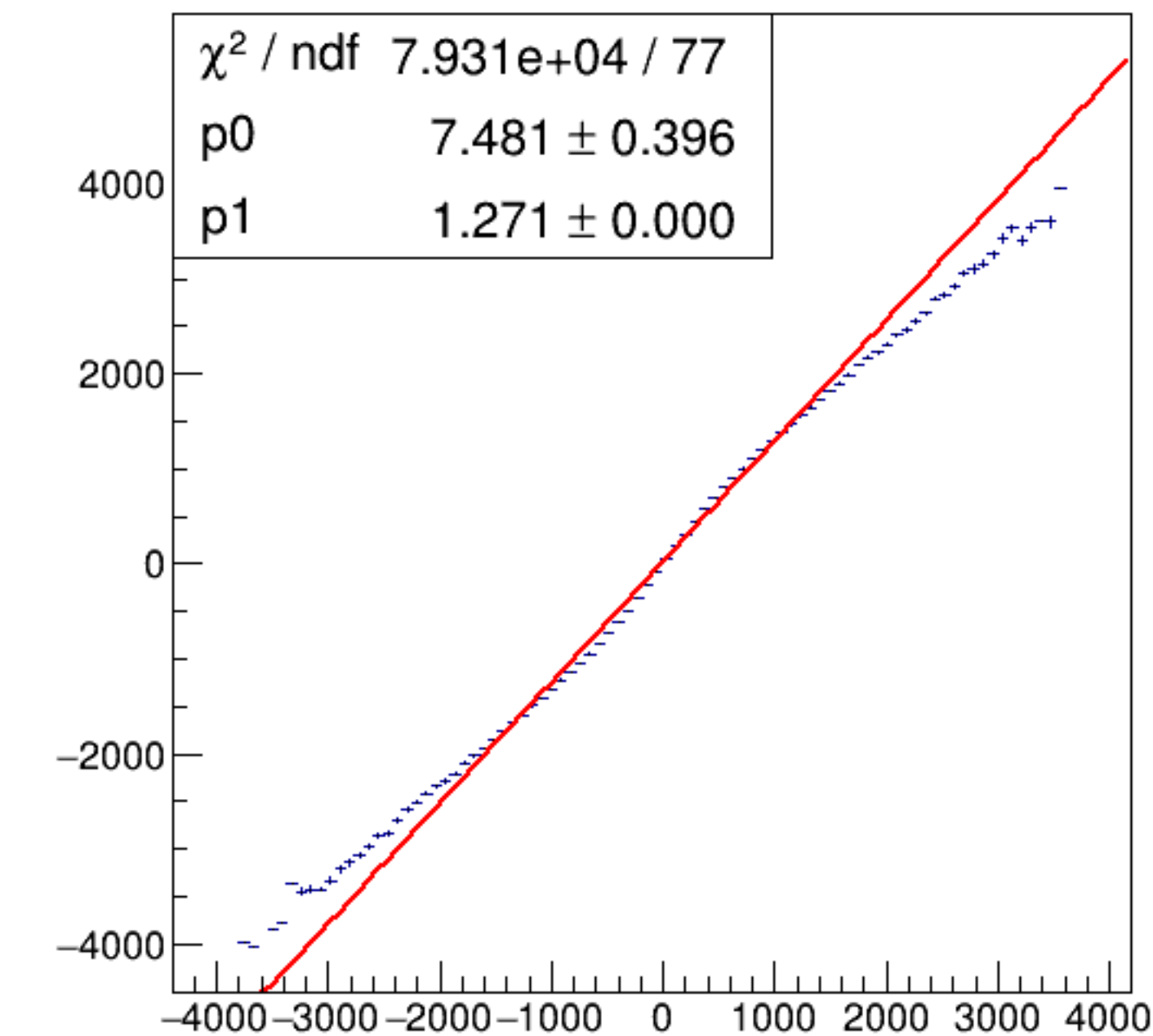
run4149_000_asym_bcm_dg_us_vs_asym_bcm_an_ds3_pr.png
