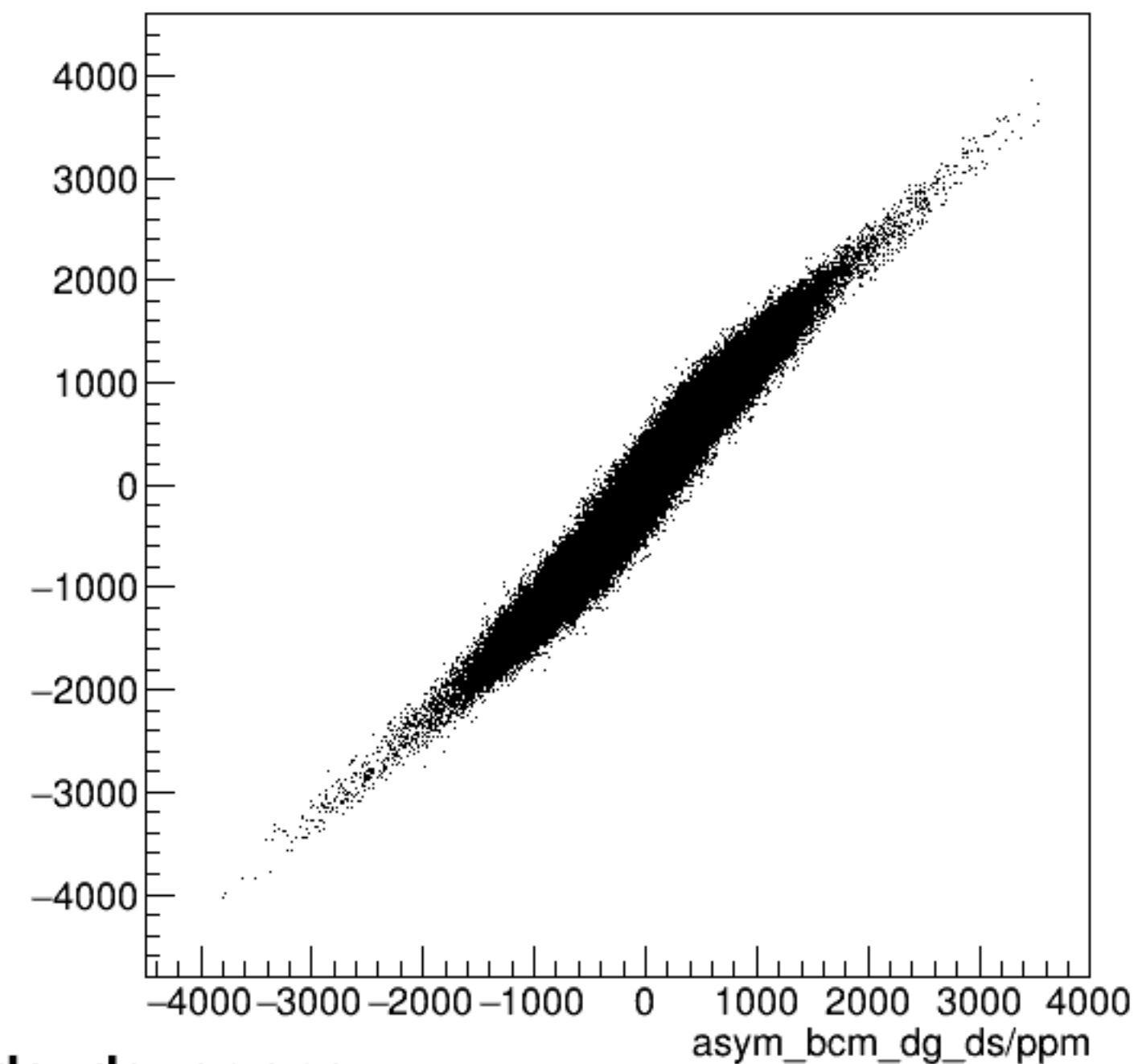
run4149_000_asym_bcm_dg_us_vs_asym_bcm_dg_ds_pr.png
