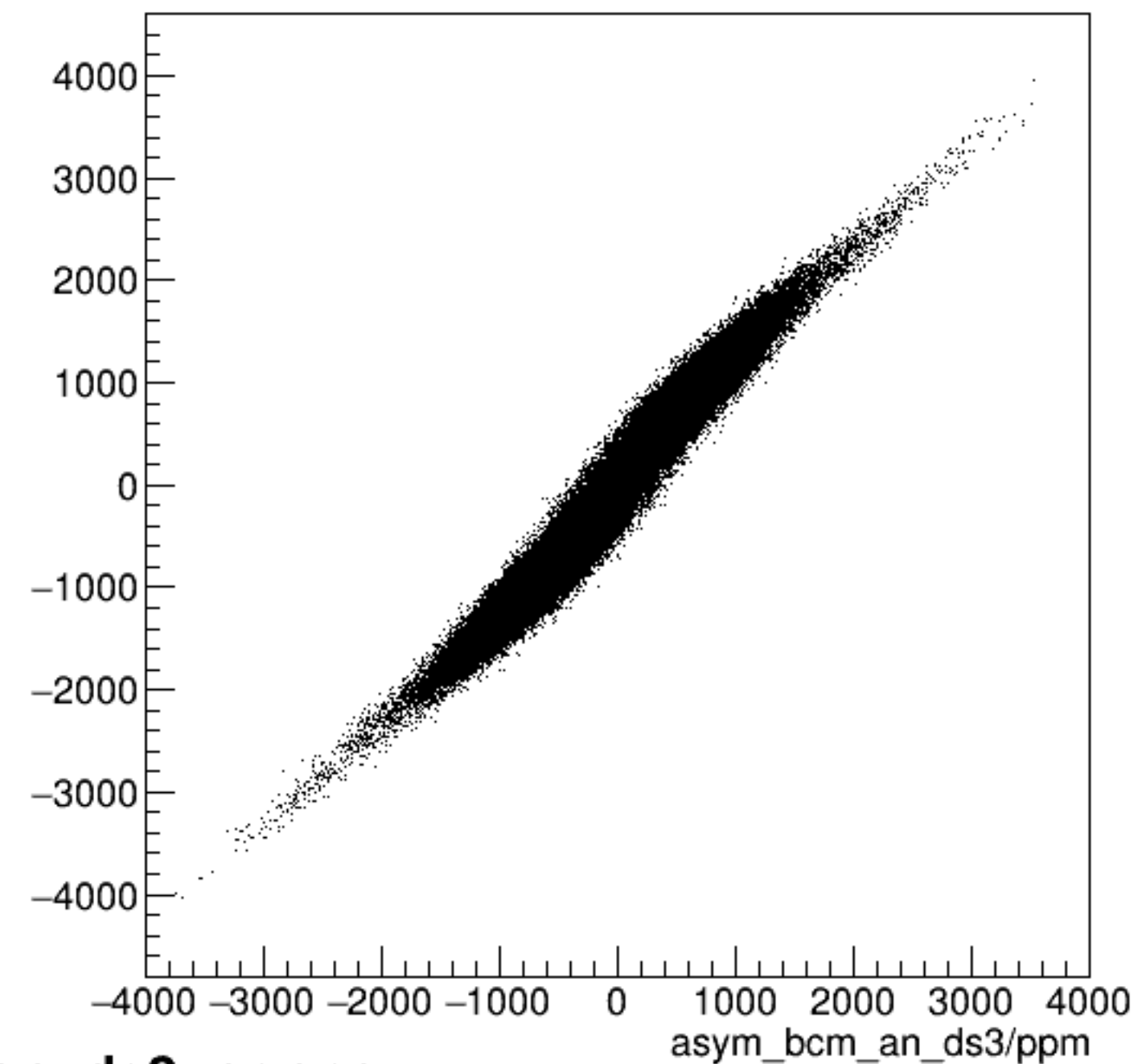
run4149_000_asym_bcm_dg_us_vs_asym_bcm_an_ds3_pr.png
