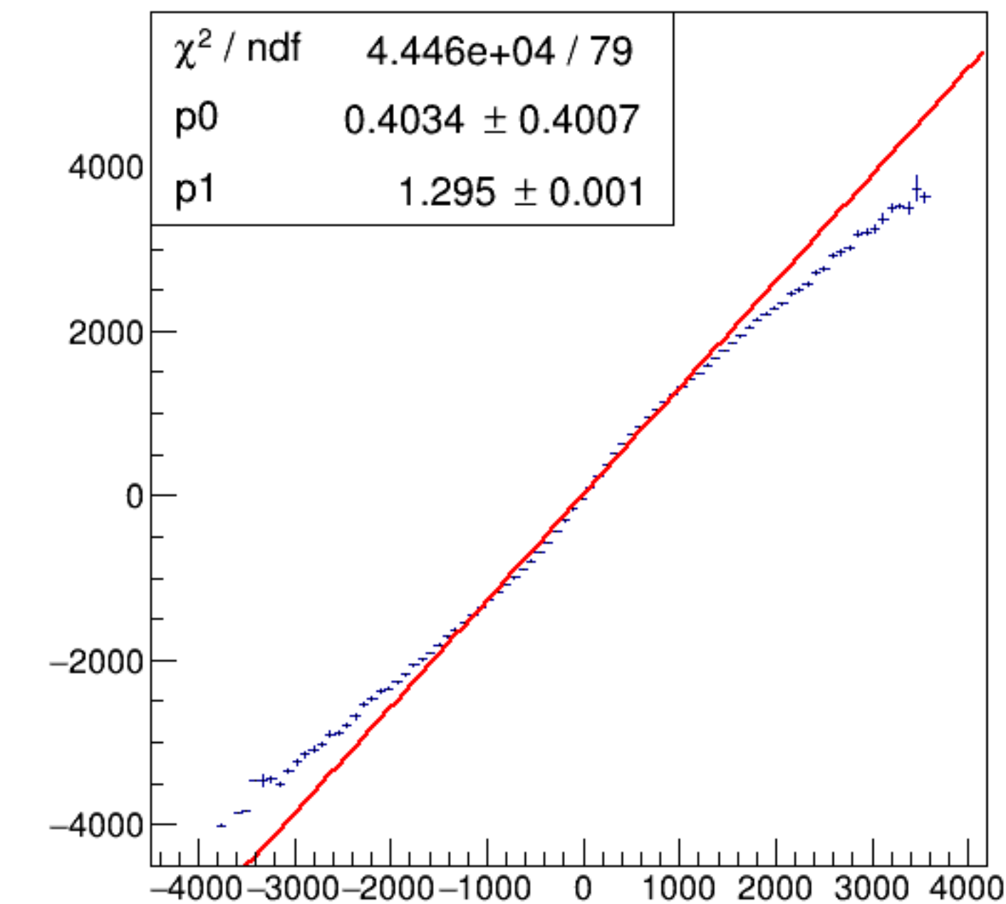
run4149_000_asym_bcm_dg_us_vs_asym_bcm_dg_ds_pr.png
