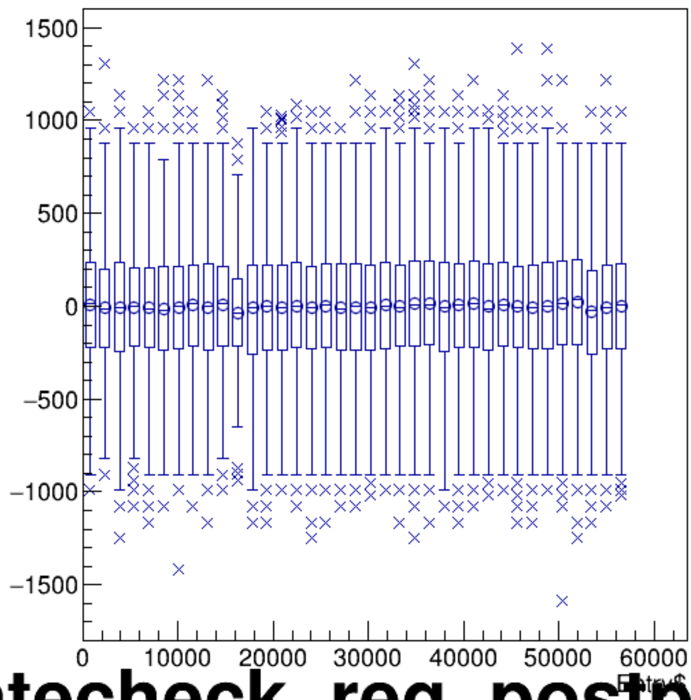
(reg_asym_atl1/ppm-reg_asym_atr1/ppm)/2:Entry$ {ok_cut}
