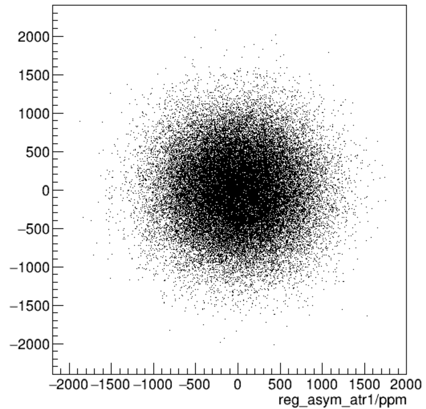
reg_asym_atl1/ppm:reg_asym_atr1/ppm {ok_cut}
