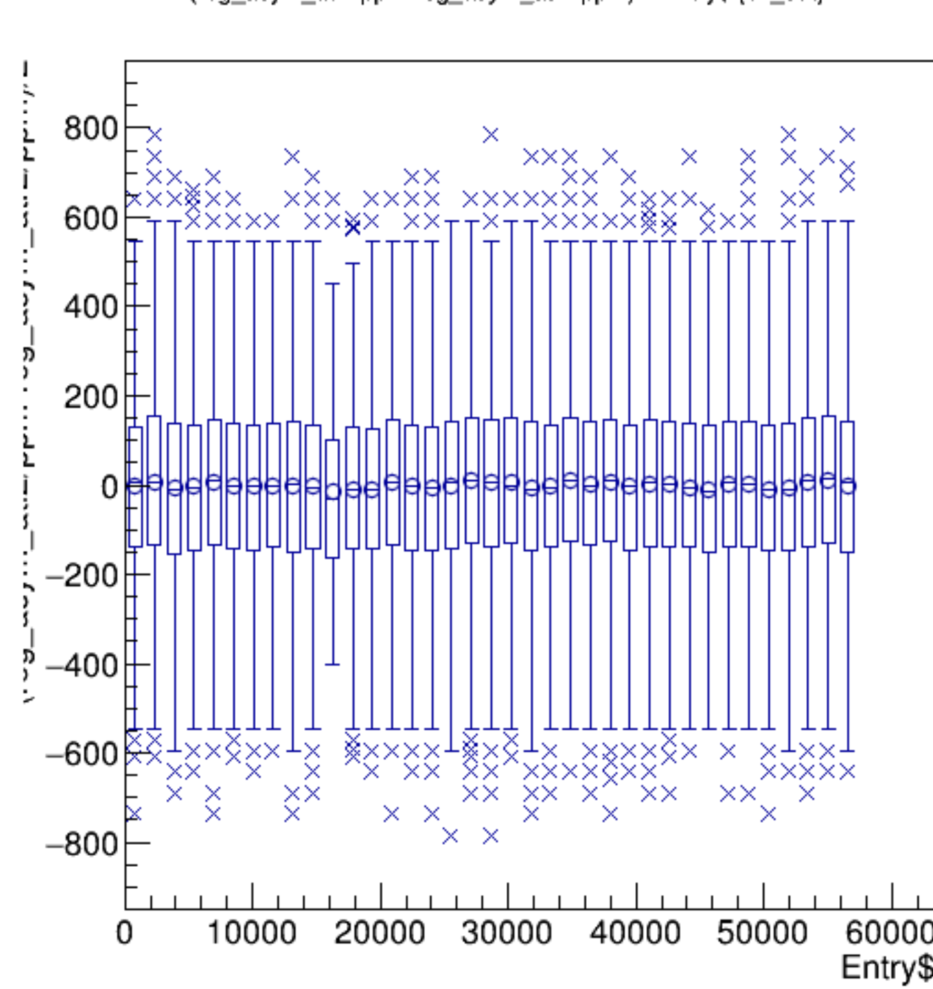
(reg_asym_atl2/ppm-reg_asym_atr2/ppm)/2:Entry$ {ok_cut}
