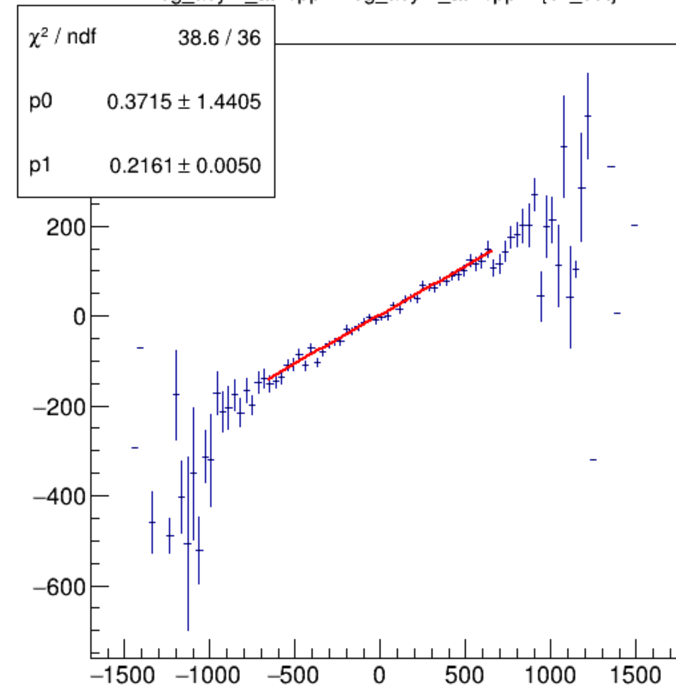
reg_asym_atl2/ppm:reg_asym_atr2/ppm {ok_cut}
