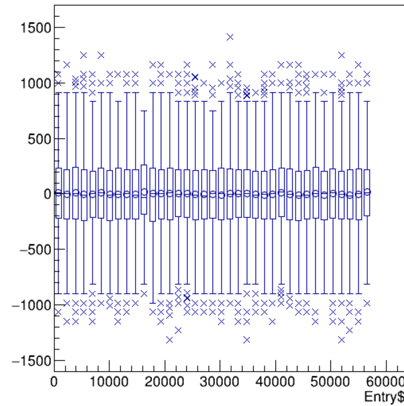
(reg_asym_atl1/ppm+reg_asym_atr1/ppm)/2:Entry$ {ok_cut}
