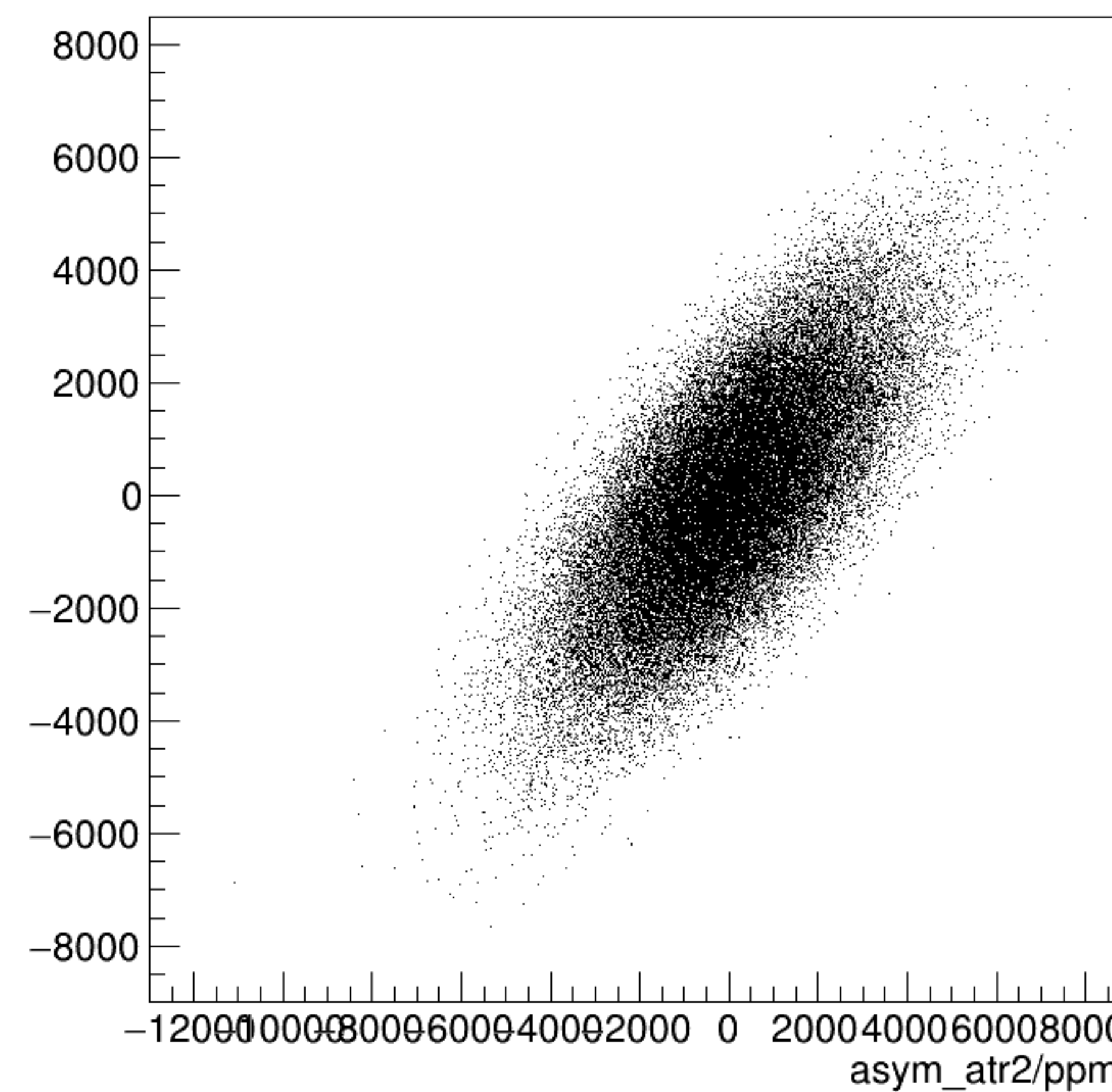
asym_atl2/ppm:asym_atr2/ppm {ok_cut}
