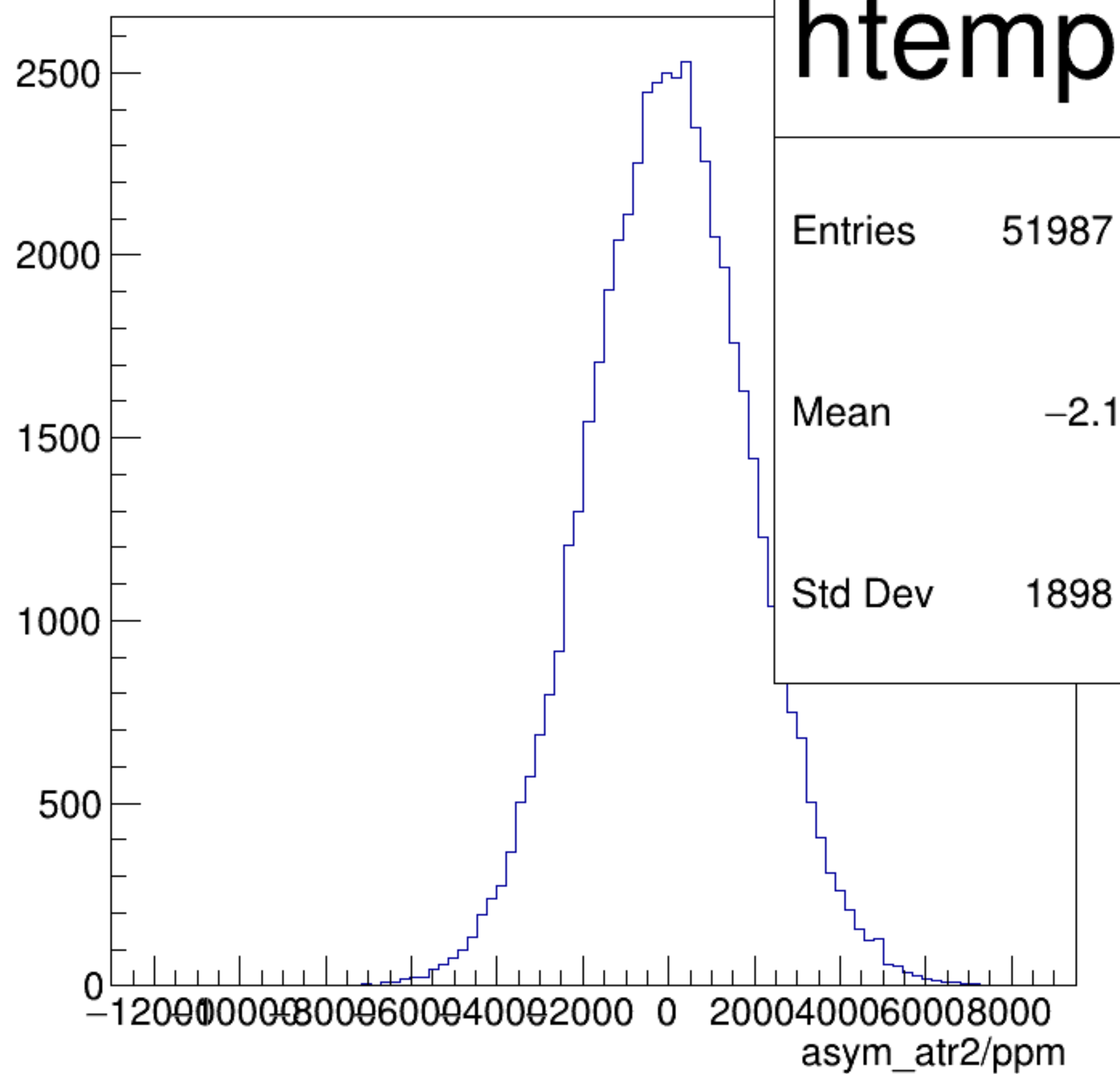
asym_atr2/ppm {ok_cut}
