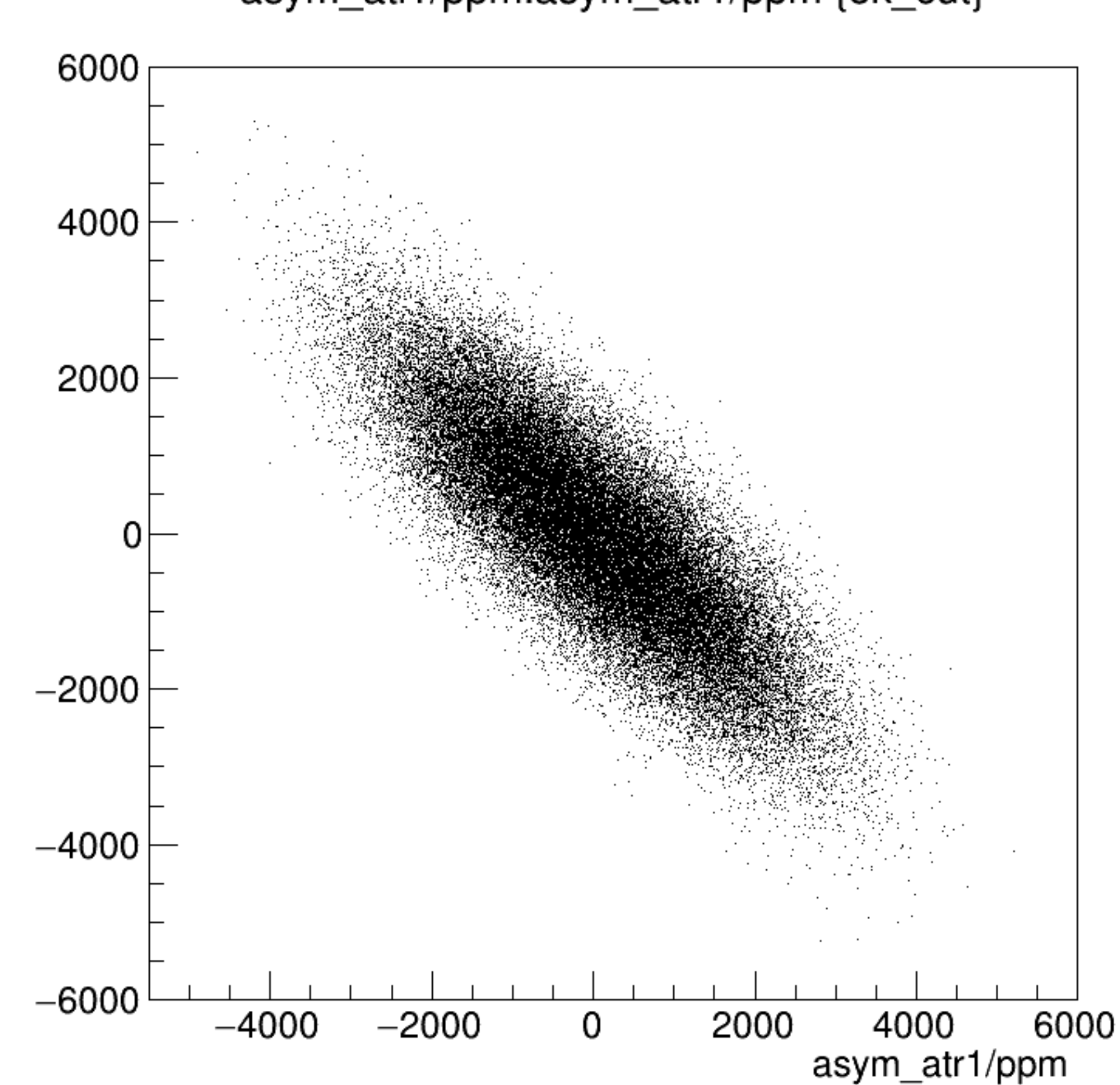
asym_atl1/ppm:asym_atr1/ppm {ok_cut}
