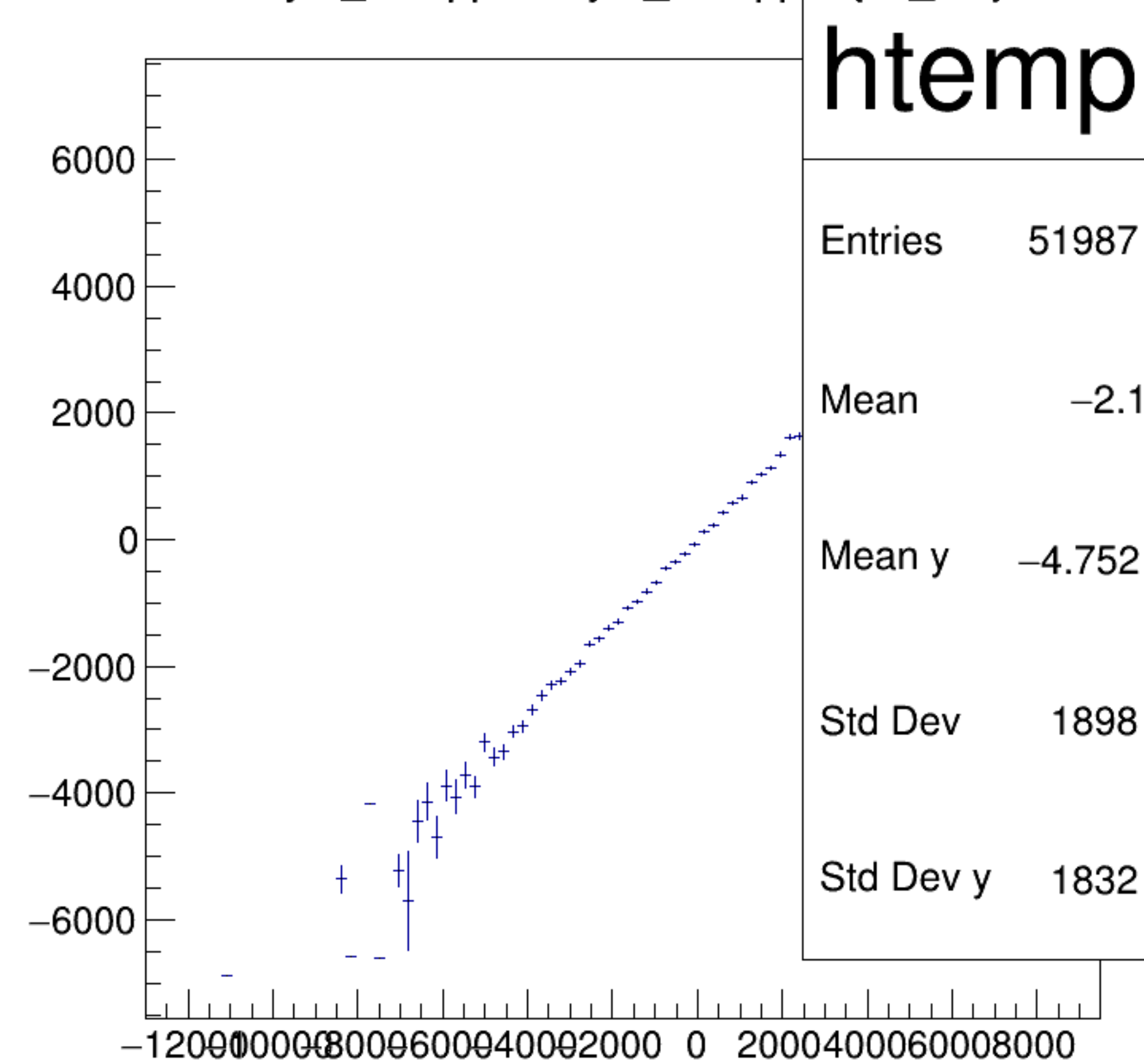
asym_atl2/ppm:asym_atr2/ppm {ok_cut}
