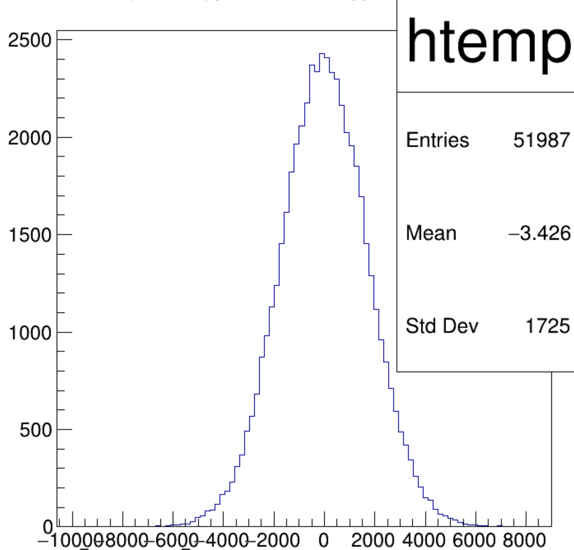
(asym_atl2/ppm+asym_atr2/ppm)/2 {ok_cut}
