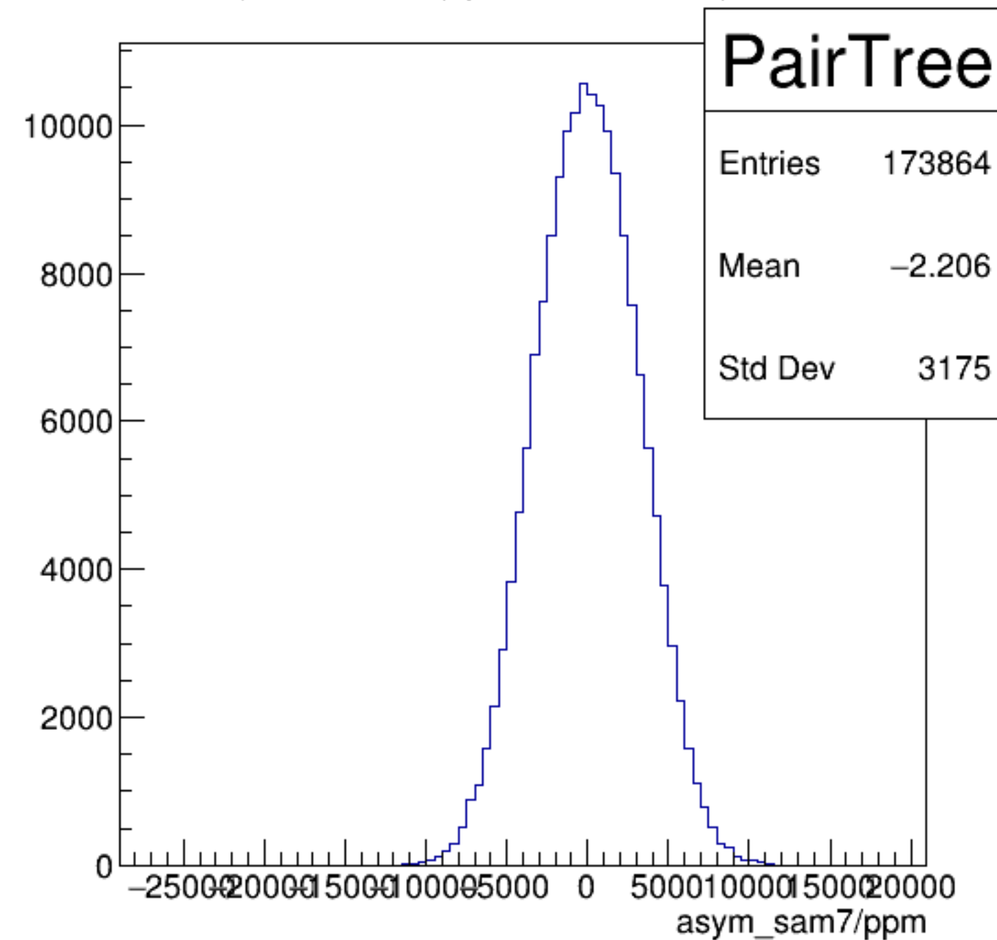
asym_sam7/ppm {ErrorFlag==0}
