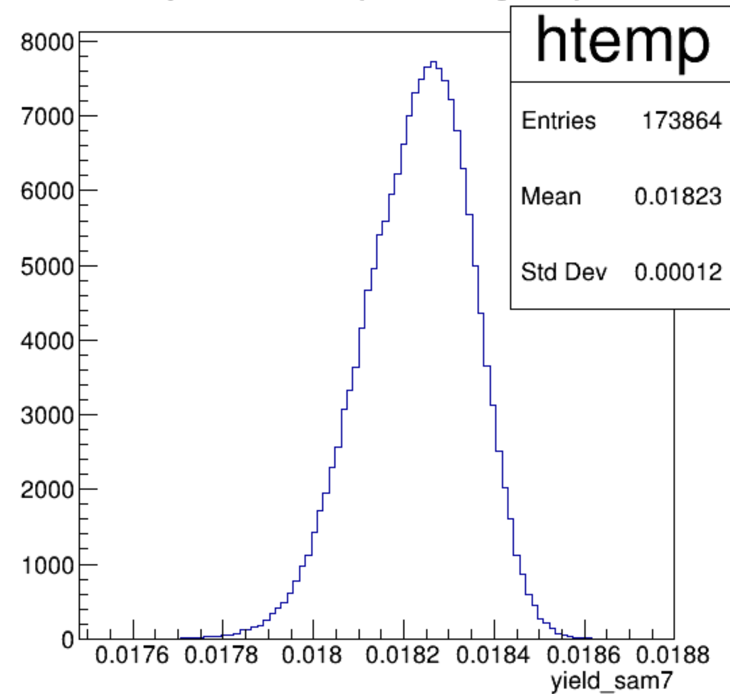
yield_sam7 {ErrorFlag==0}
