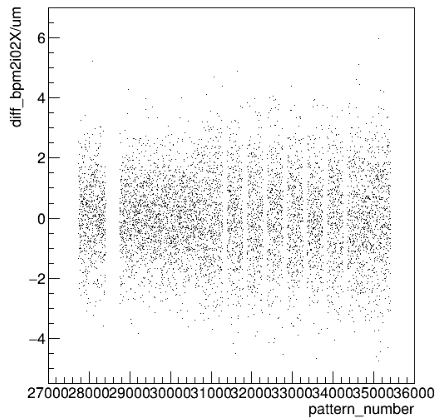
diff_bpm2i02X/um:pattern_number {ErrorFlag==0}
