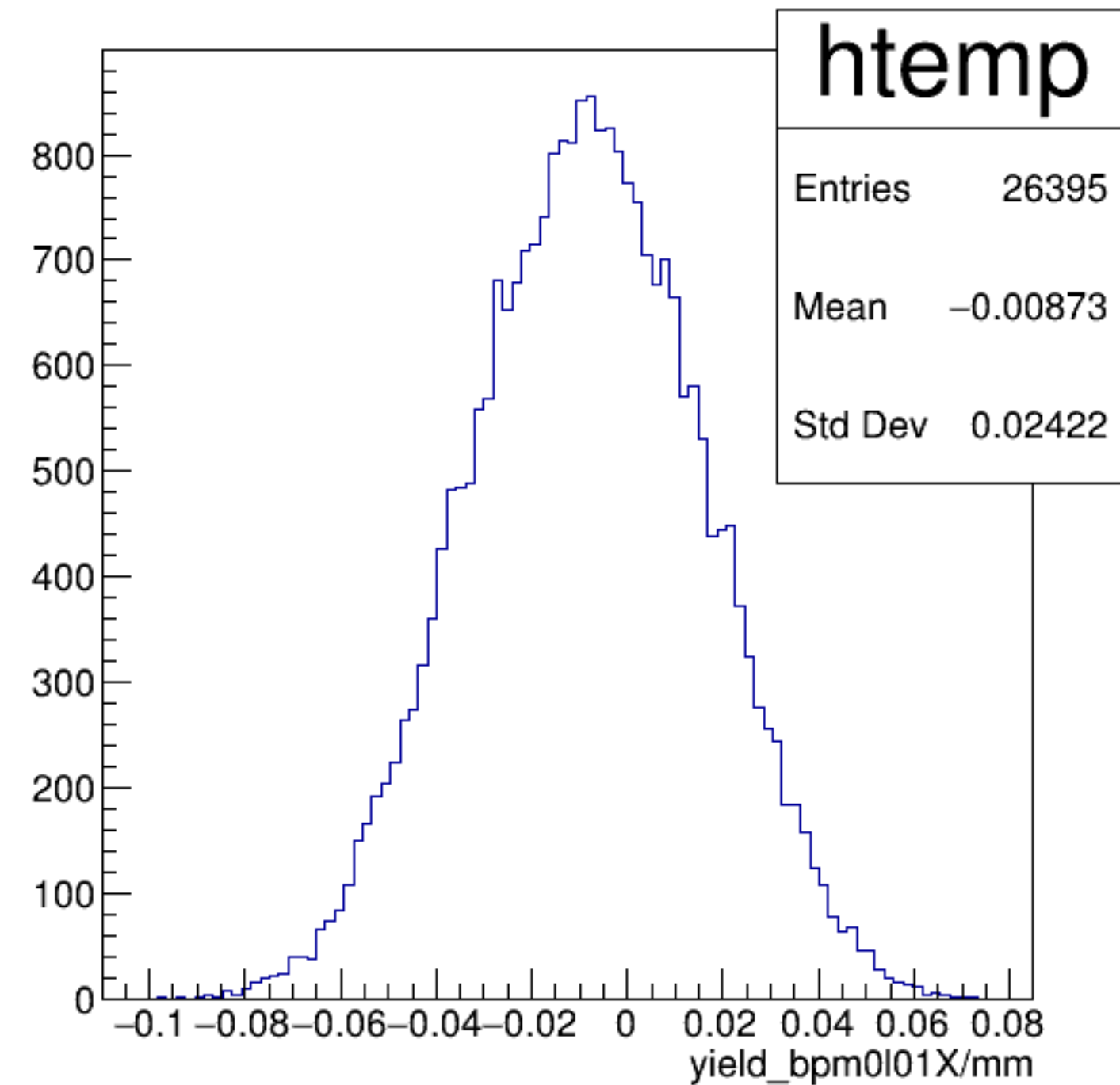
yield_bpm0l01X/mm {ErrorFlag==0}
