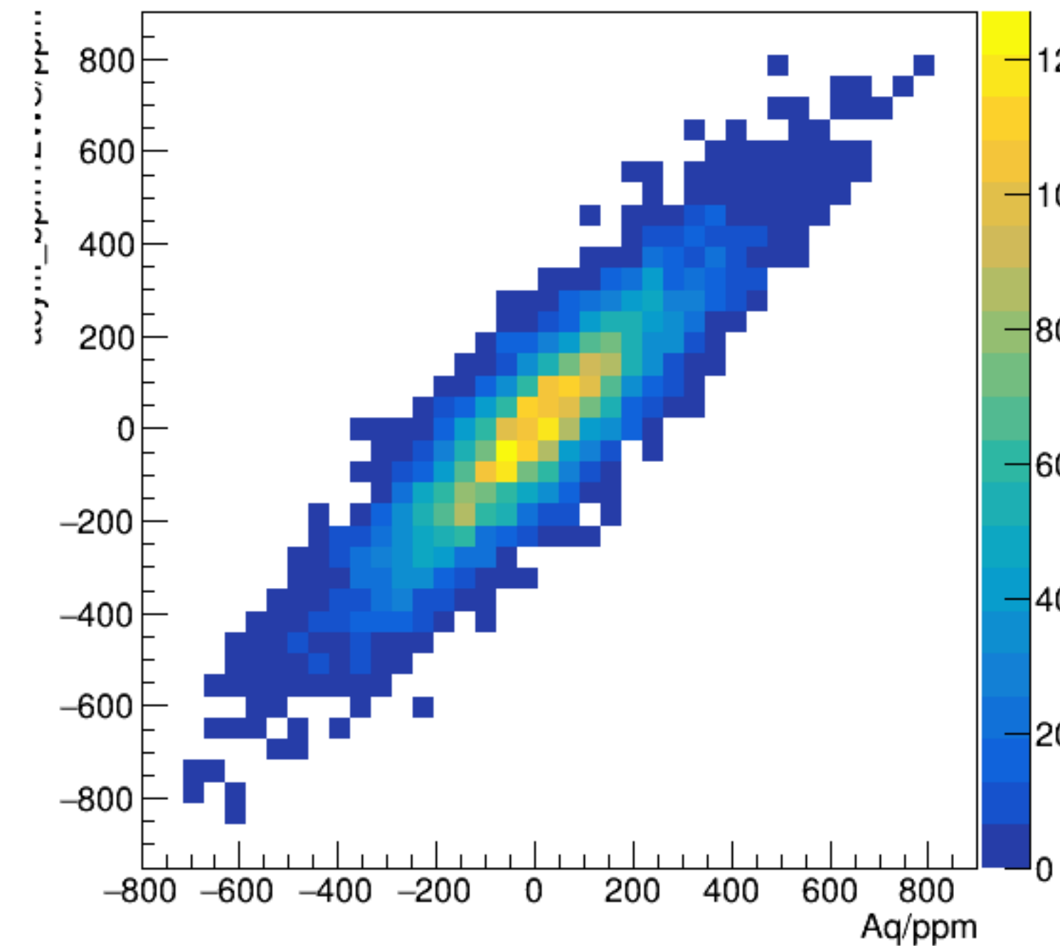
asym_bpm12WS/ppm:Aq/ppm {ErrorFlag==0}
