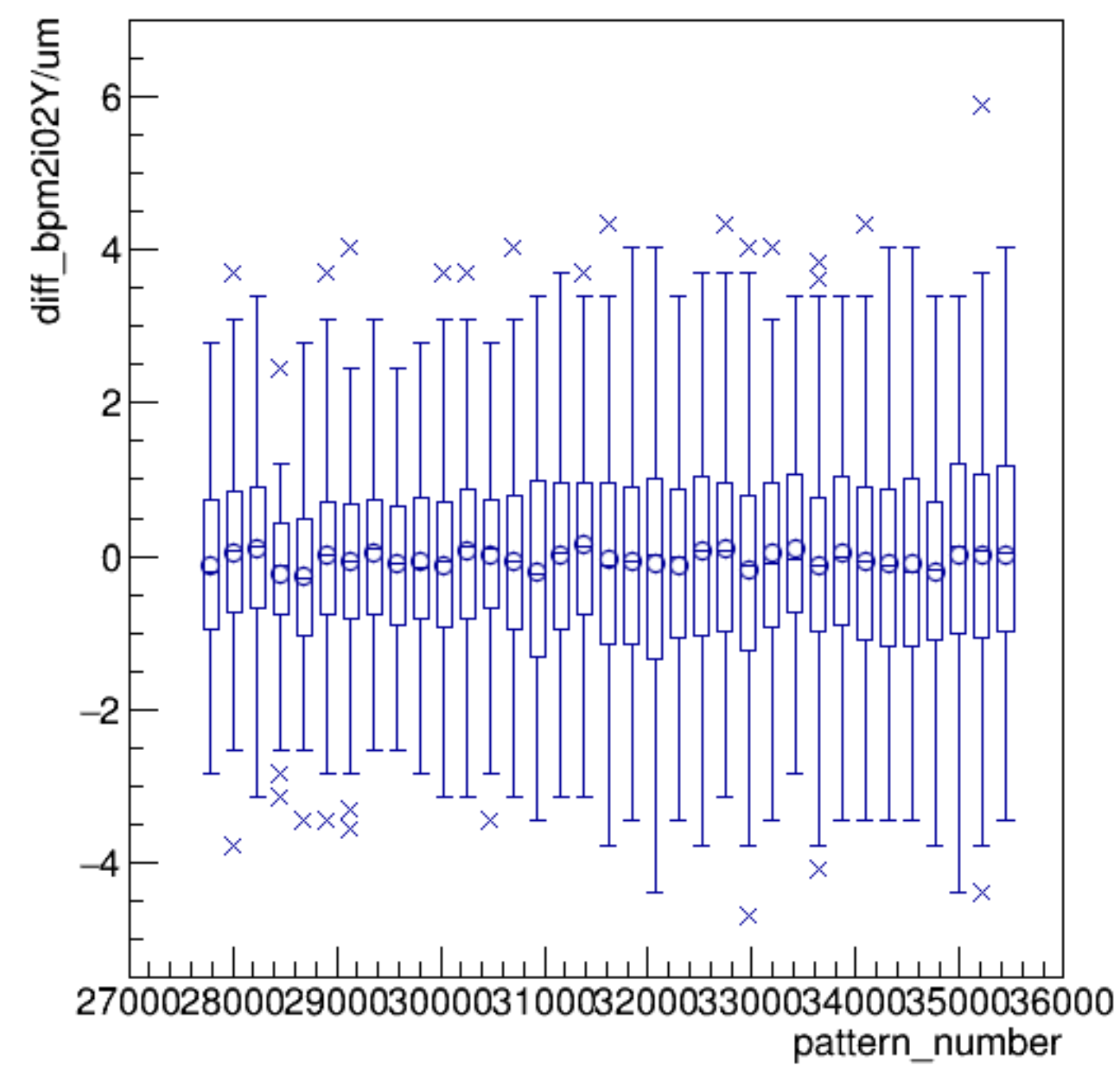
diff_bpm2i02Y/um:pattern_number {ErrorFlag==0}
