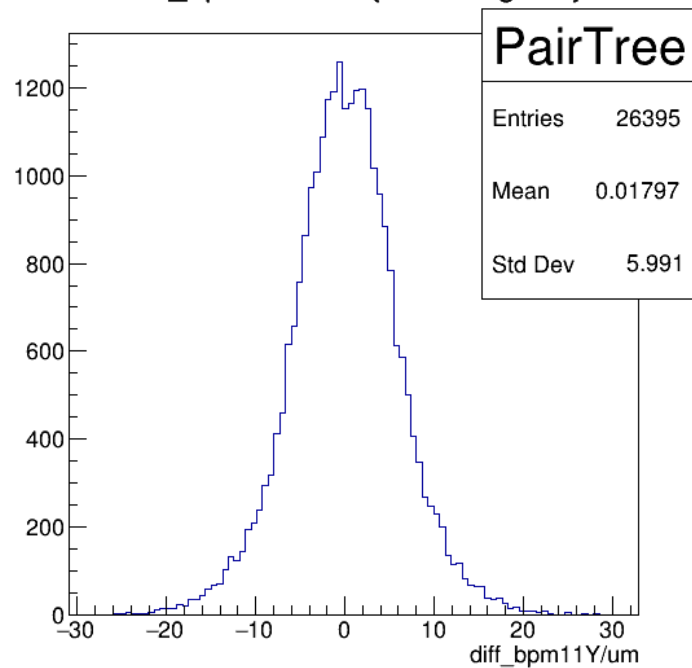
diff_bpm11Y/um {ErrorFlag==0}
