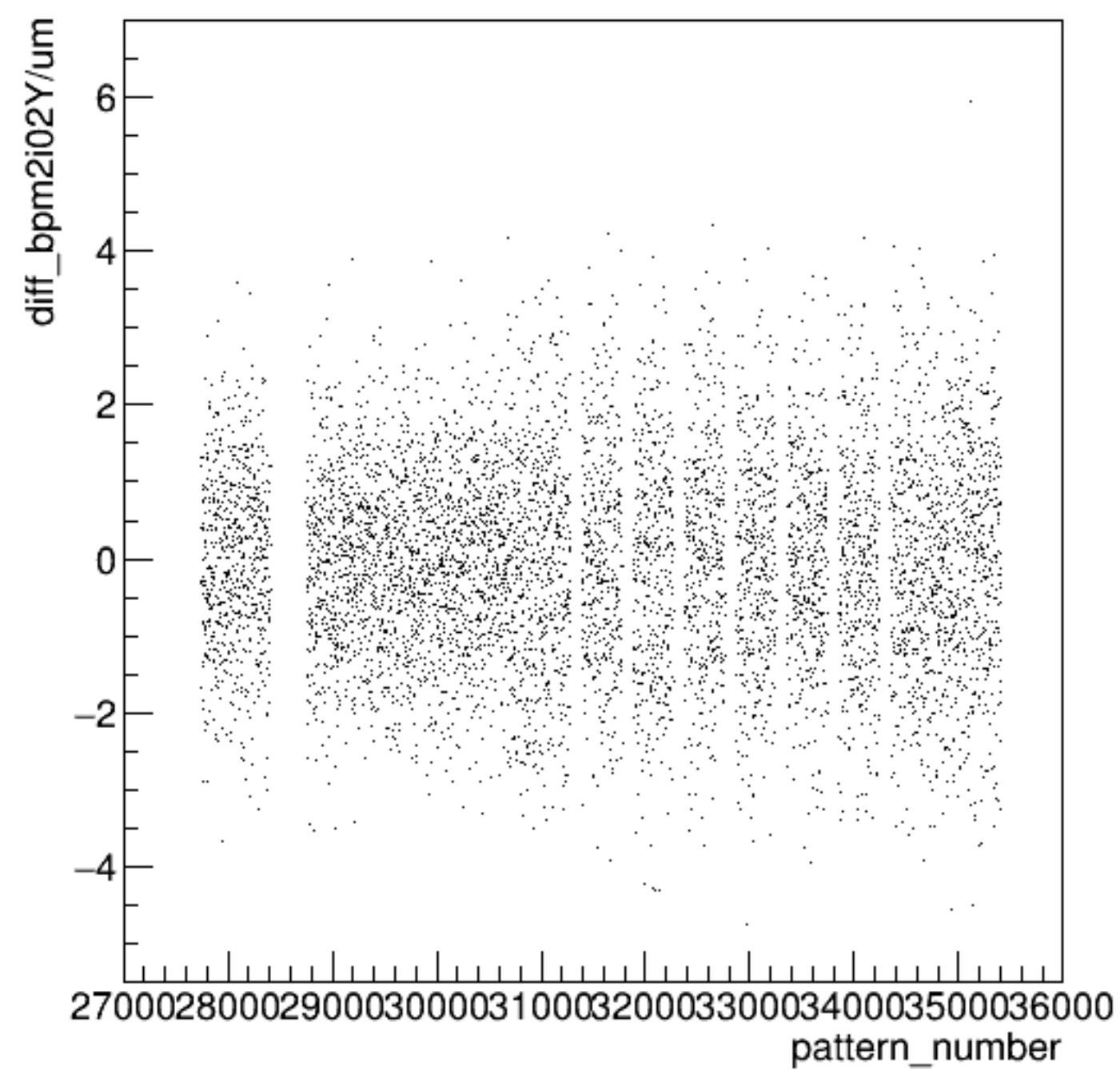
diff_bpm2i02Y/um:pattern_number {ErrorFlag==0}
