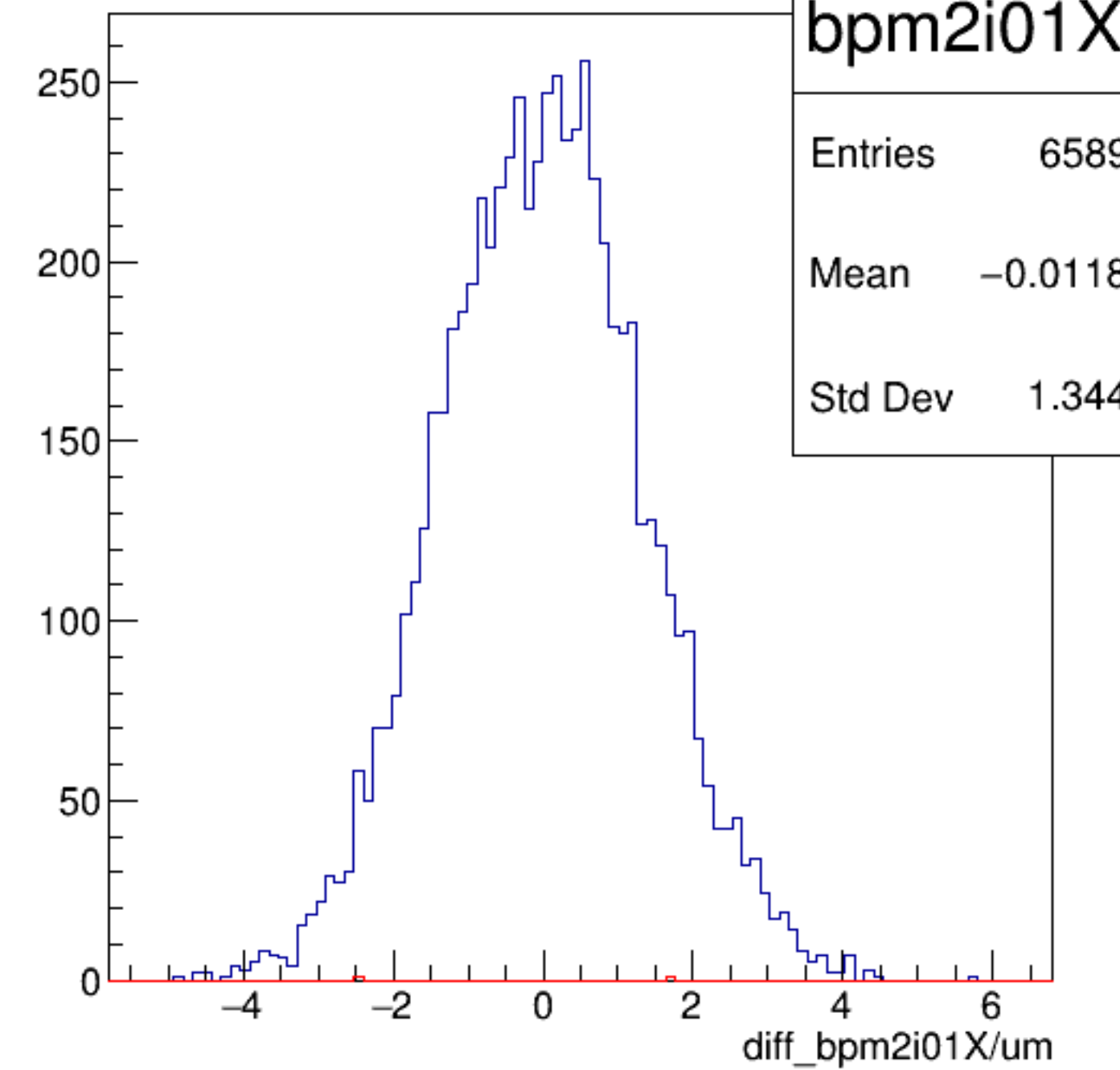
diff_bpm2i01X/um {ErrorFlag==0}
