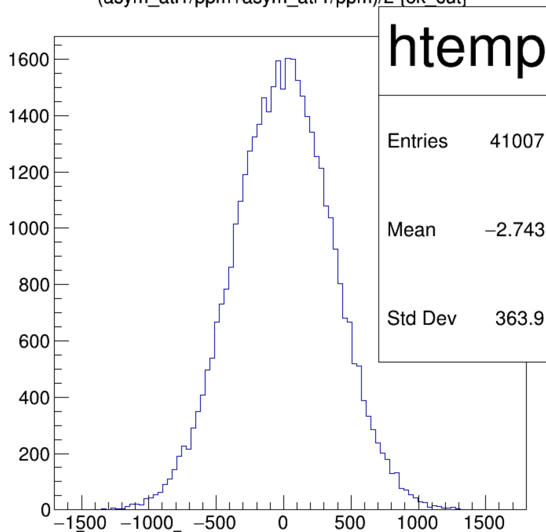
(asym_atl1/ppm+asym_atr1/ppm)/2 {ok_cut}
