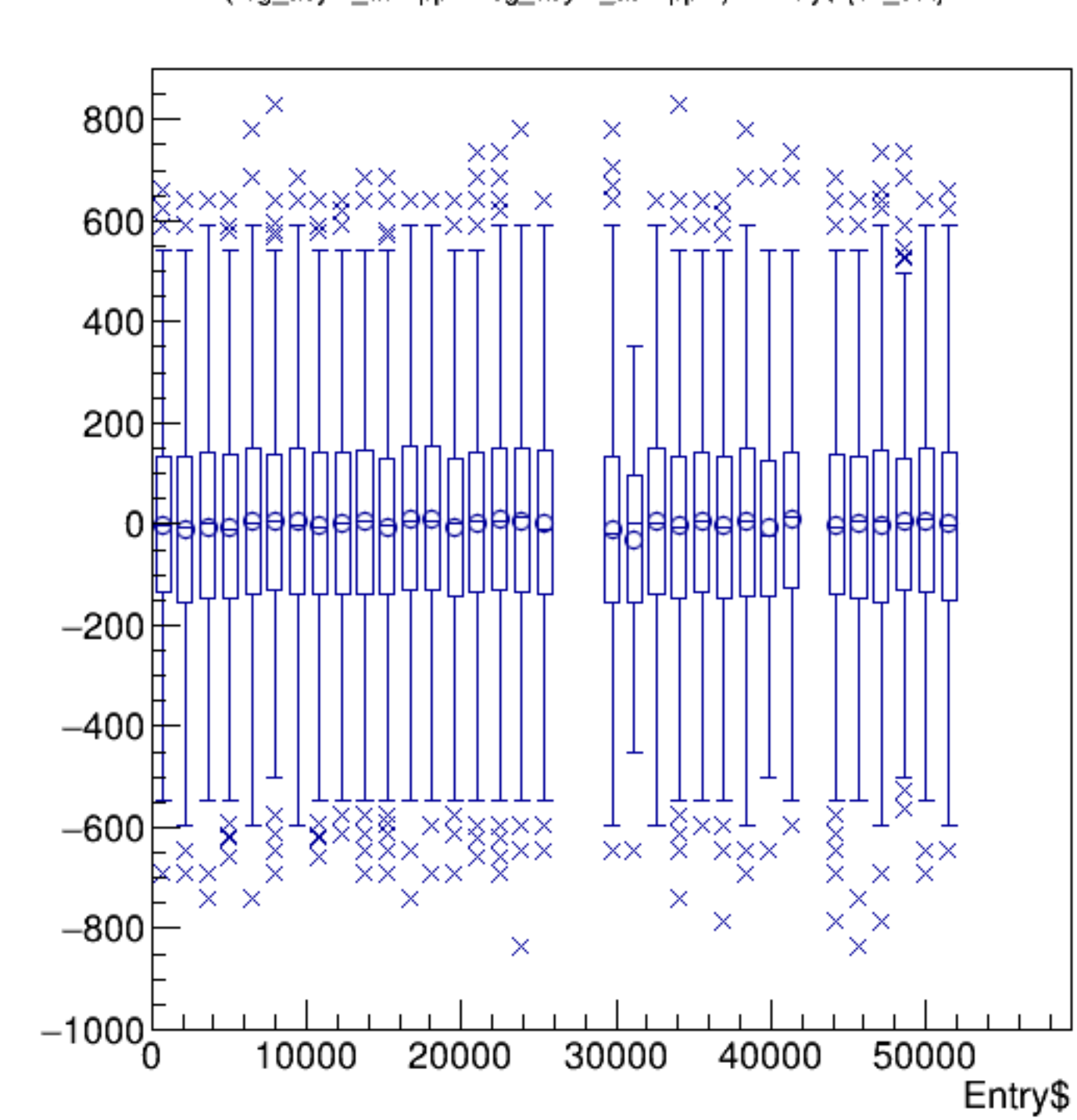
(reg_asym_atl2/ppm-reg_asym_atr2/ppm)/2:Entry$ {ok_cut}
