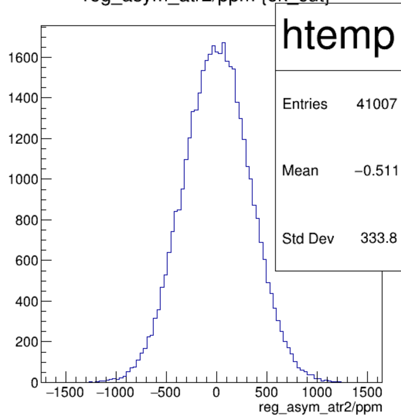
reg_asym_atr2/ppm {ok_cut}
