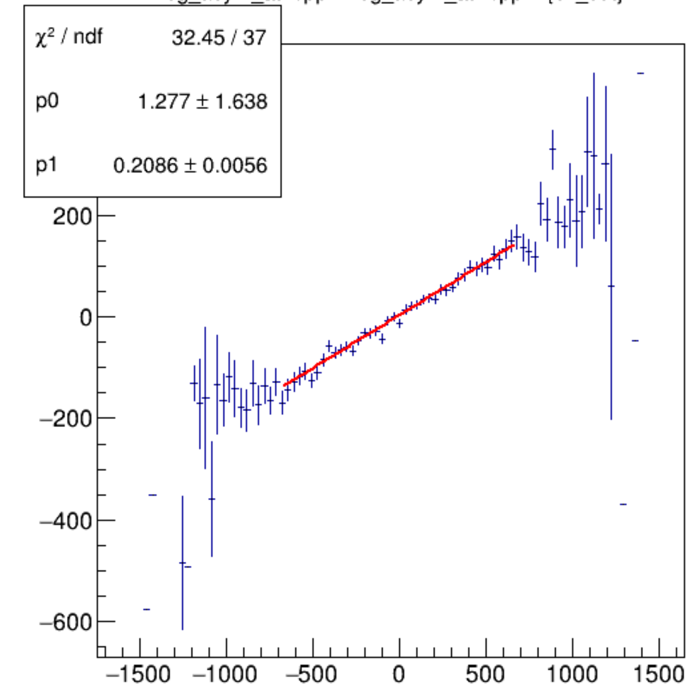
reg_asym_atl2/ppm:reg_asym_atr2/ppm {ok_cut}
