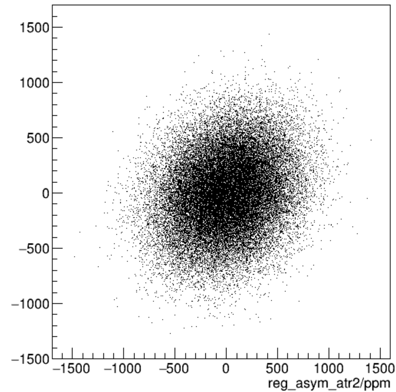
reg_asym_atl2/ppm:reg_asym_atr2/ppm {ok_cut}
