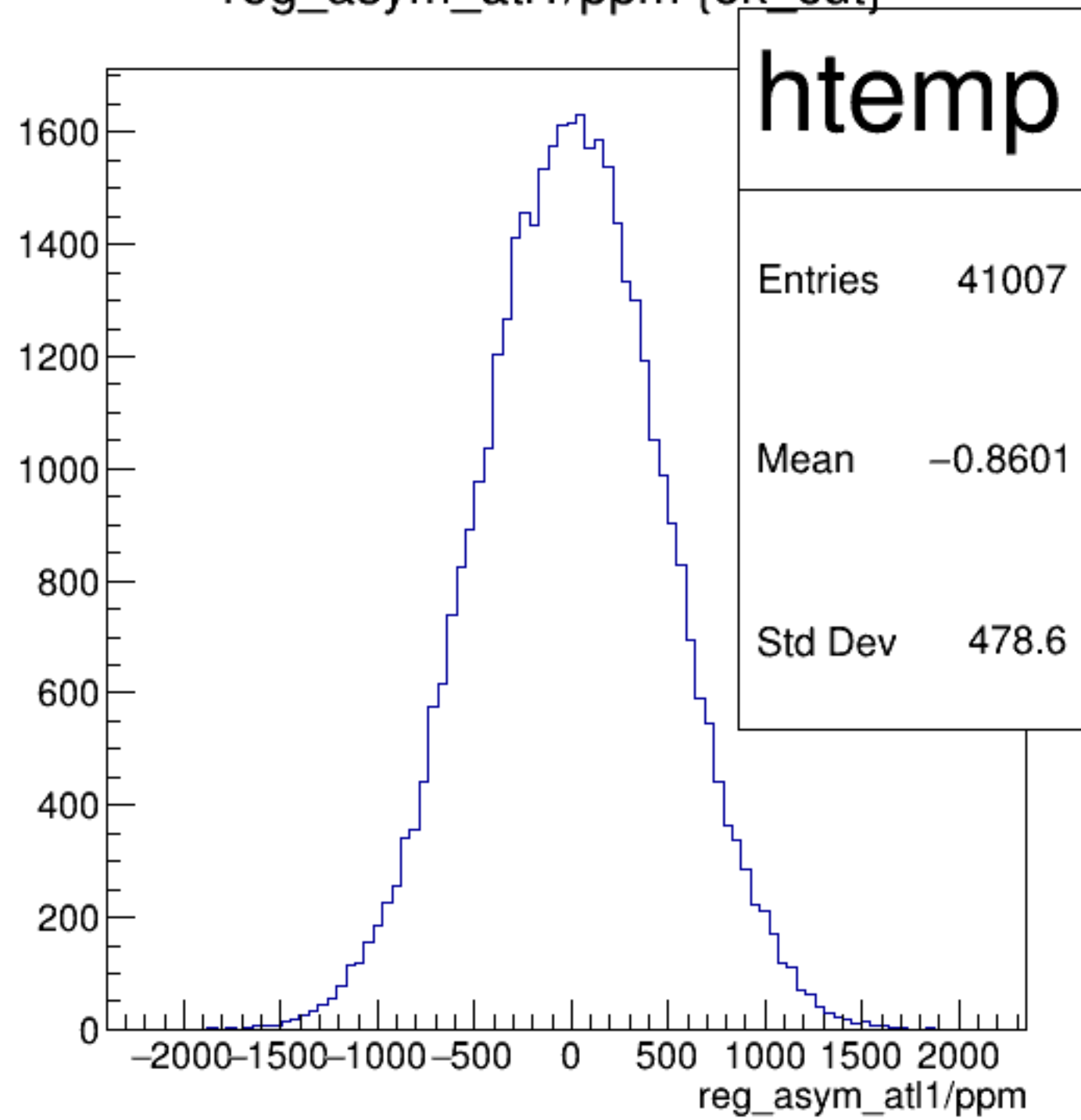
reg_asym_atl1/ppm {ok_cut}
