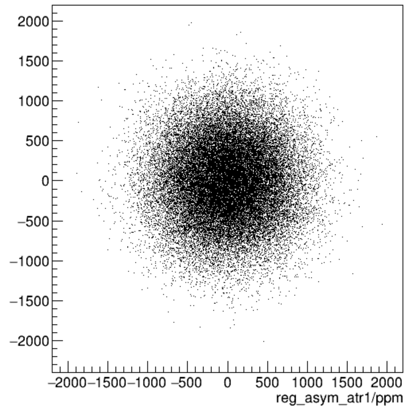
reg_asym_atl1/ppm:reg_asym_atr1/ppm {ok_cut}
