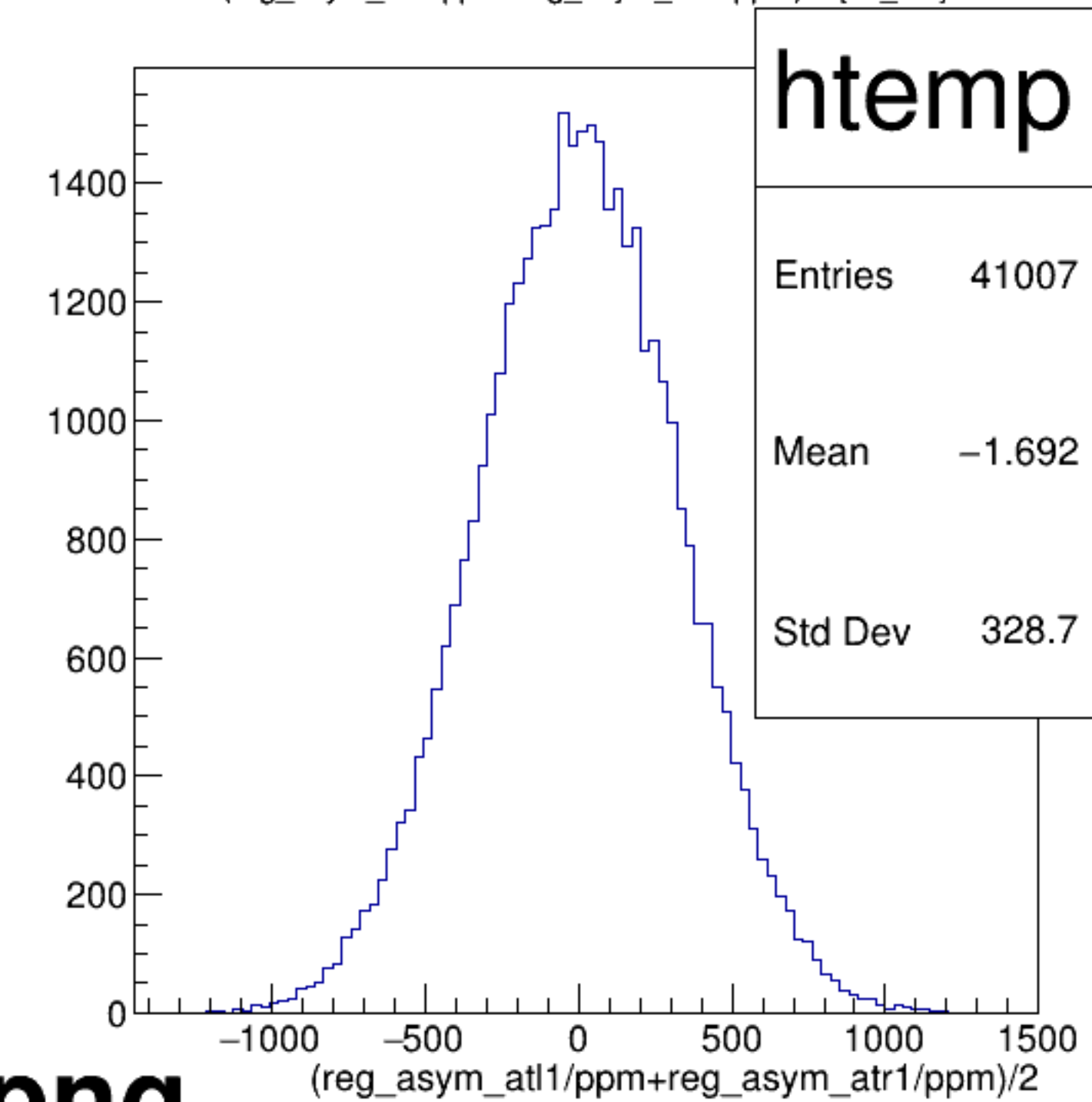
(reg_asym_atl1/ppm+reg_asym_atr1/ppm)/2 {ok_cut}
