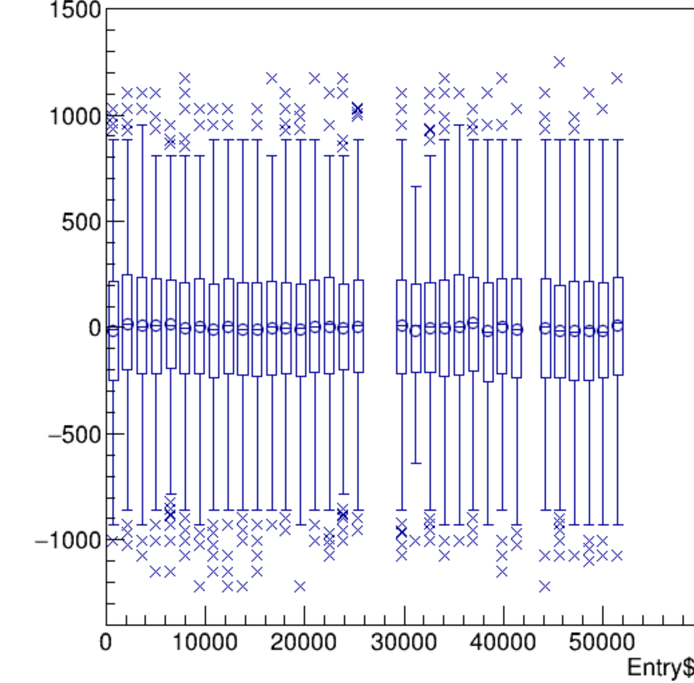
(reg_asym_atl1/ppm+reg_asym_atr1/ppm)/2:Entry$ {ok_cut}
