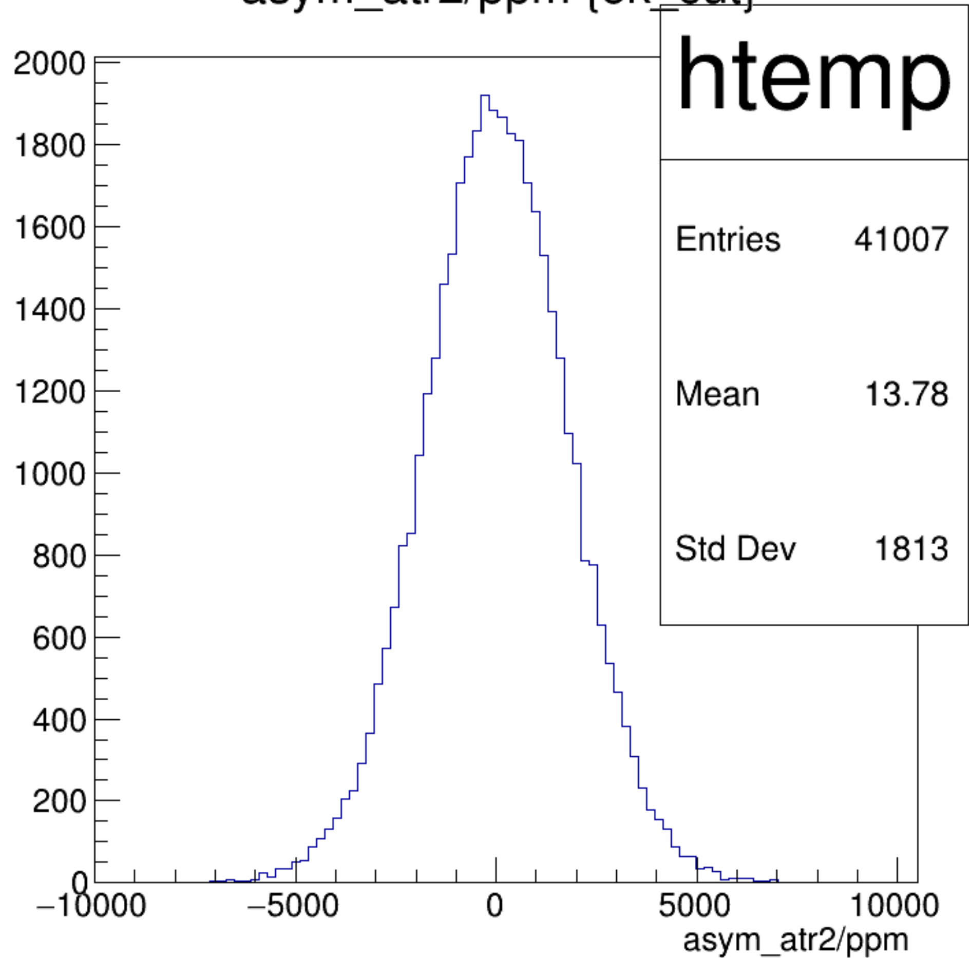
asym_atr2/ppm {ok_cut}
