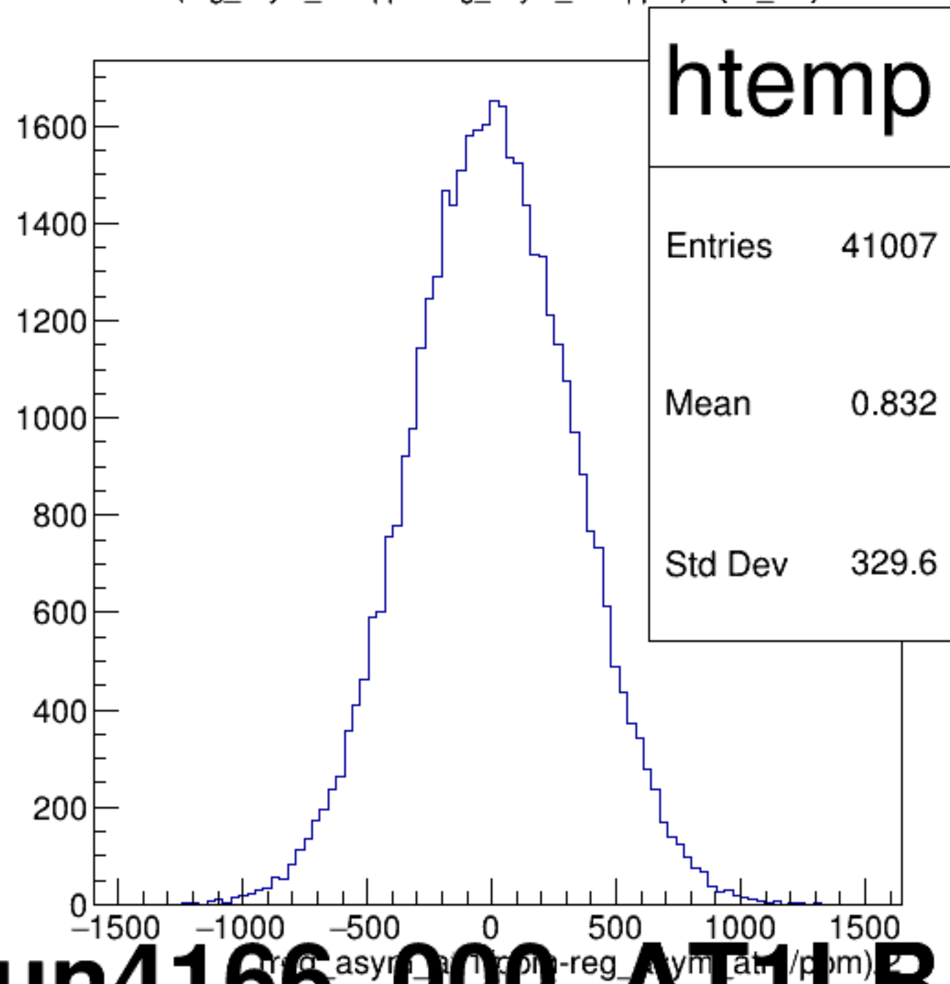
(reg_asym_atl1/ppm-reg_asym_atr1/ppm)/2 {ok_cut}
