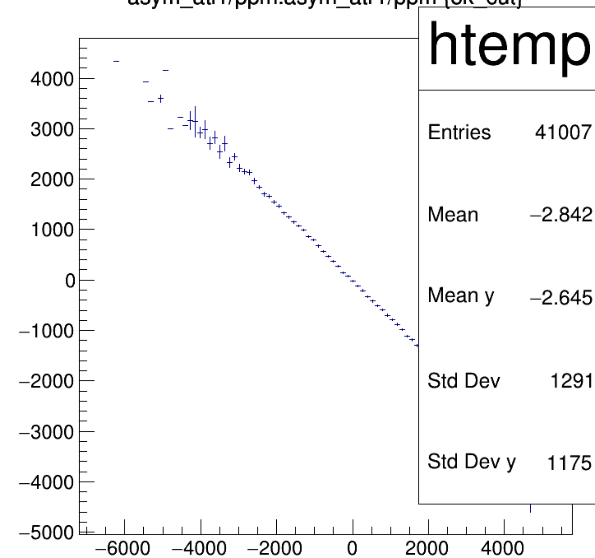
asym_atl1/ppm:asym_atr1/ppm {ok_cut}
