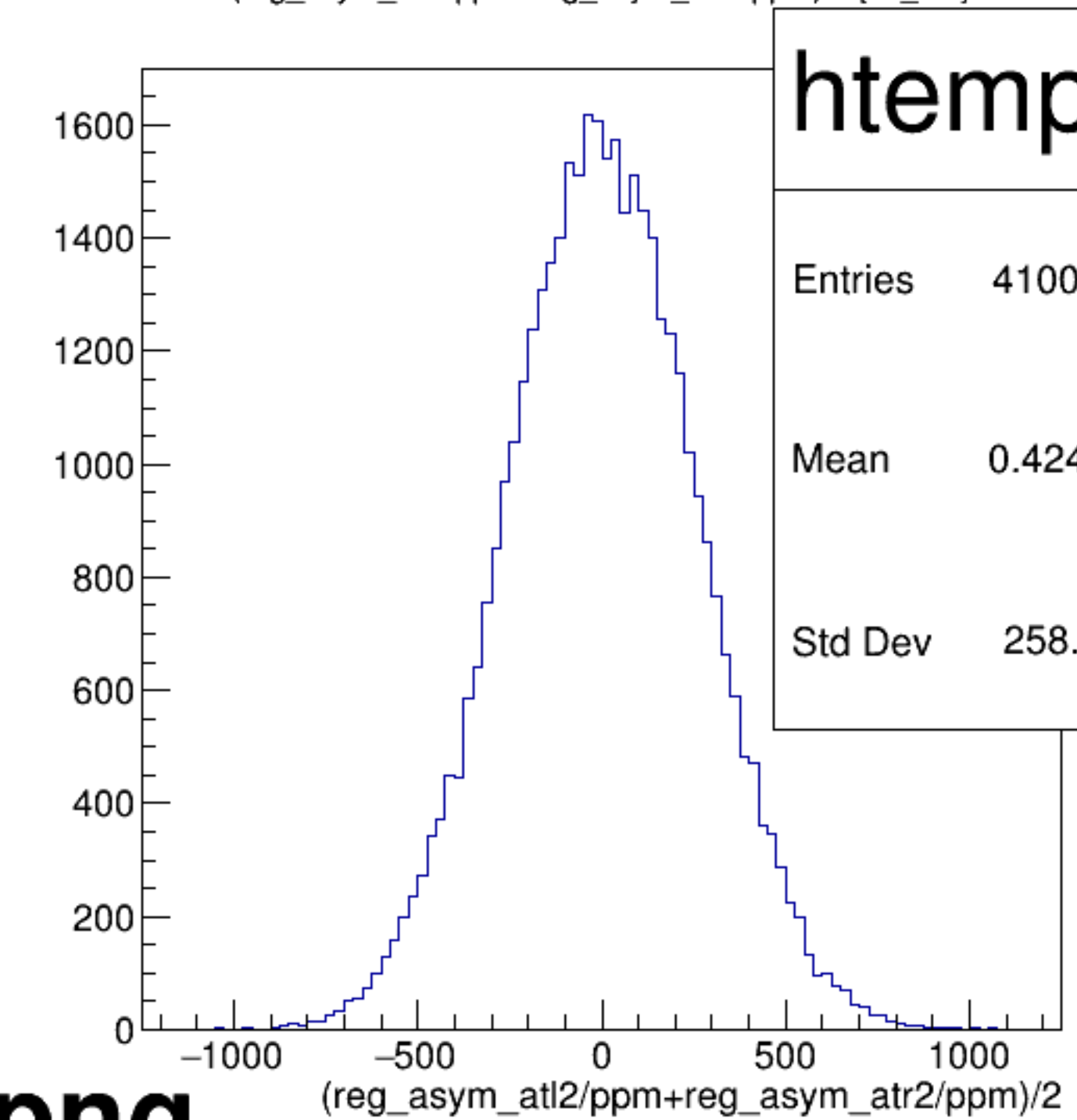
(reg_asym_atl2/ppm+reg_asym_atr2/ppm)/2 {ok_cut}
