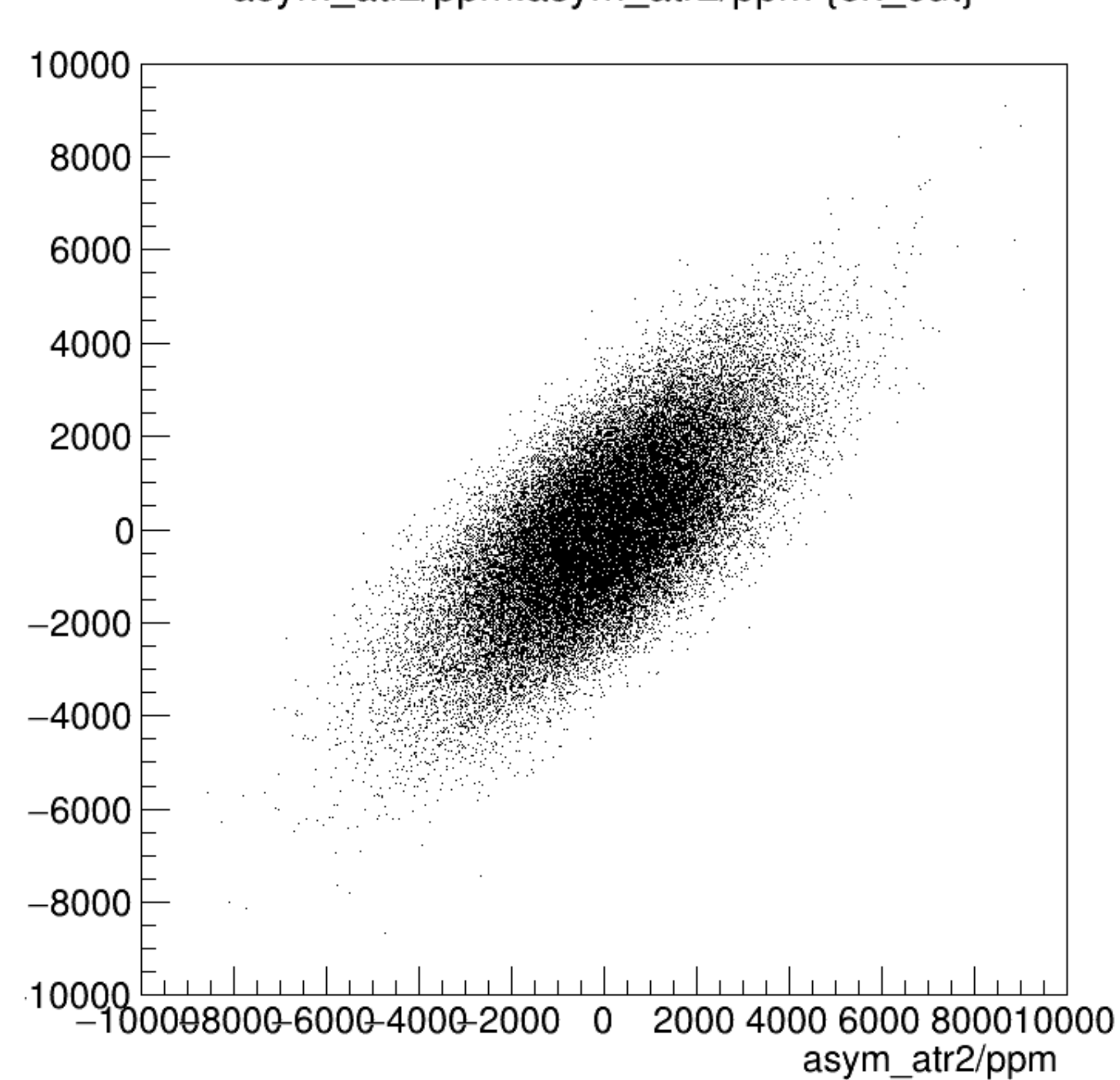
asym_atl2/ppm:asym_atr2/ppm {ok_cut}
