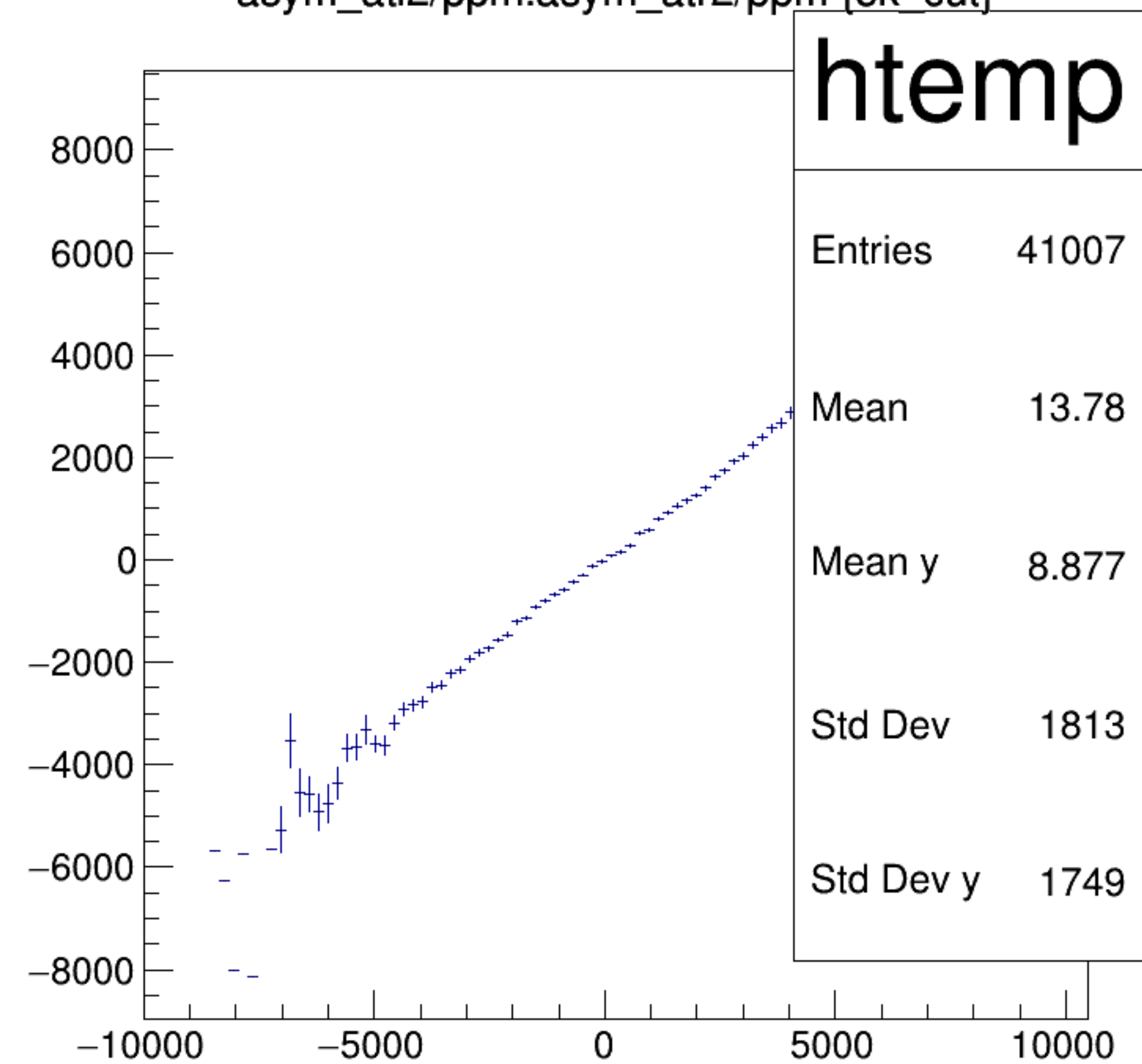
asym_atl2/ppm:asym_atr2/ppm {ok_cut}
