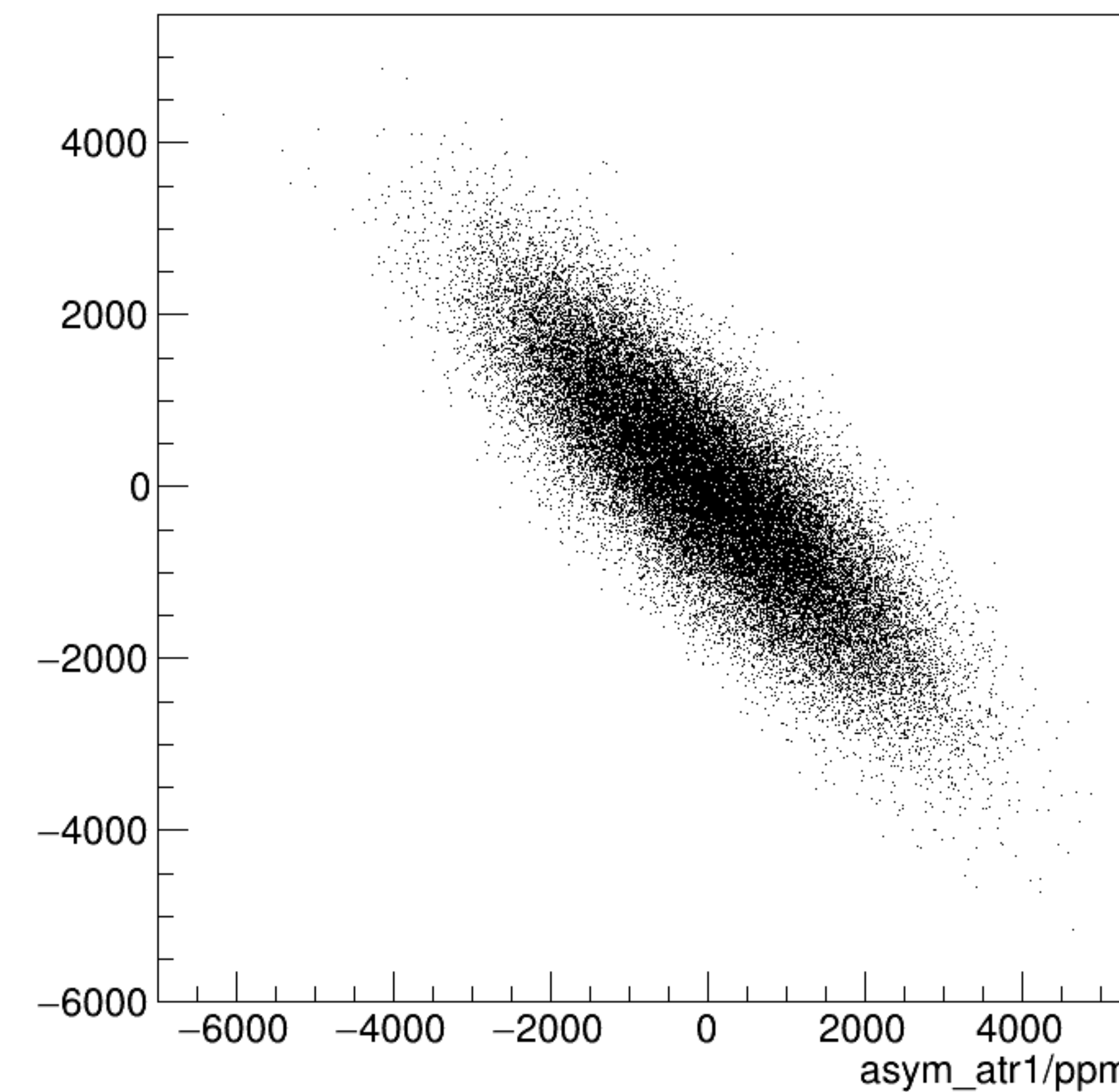
asym_atl1/ppm:asym_atr1/ppm {ok_cut}
