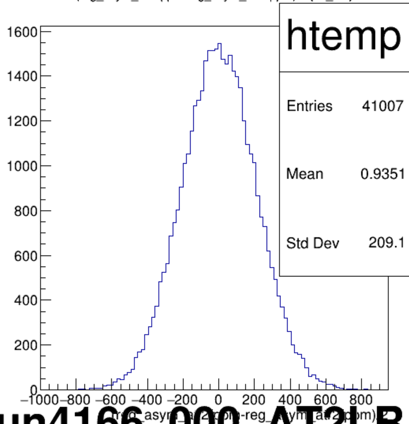
(reg_asym_atl2/ppm-reg_asym_atr2/ppm)/2 {ok_cut}
