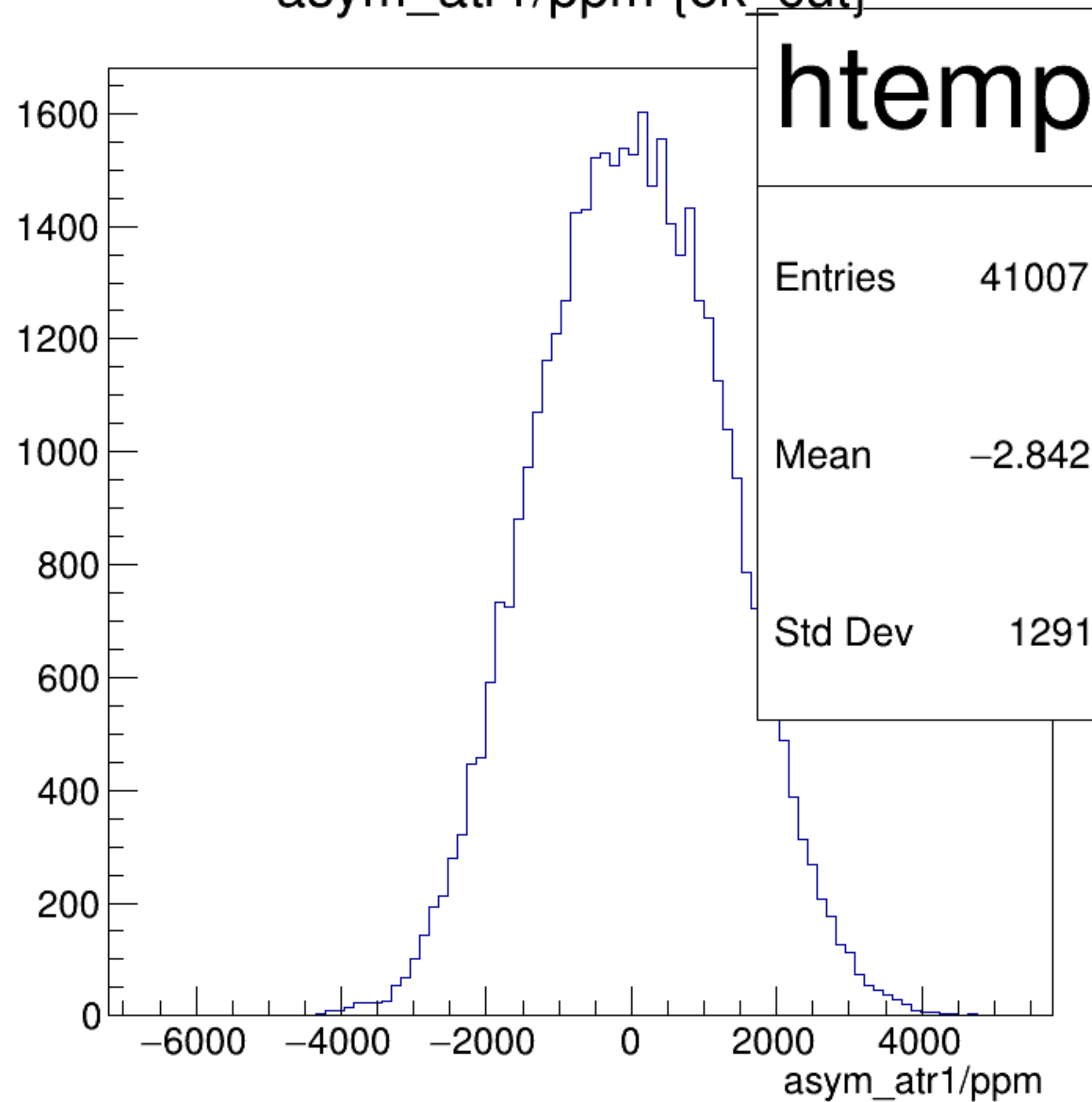
asym_atr1/ppm {ok_cut}
