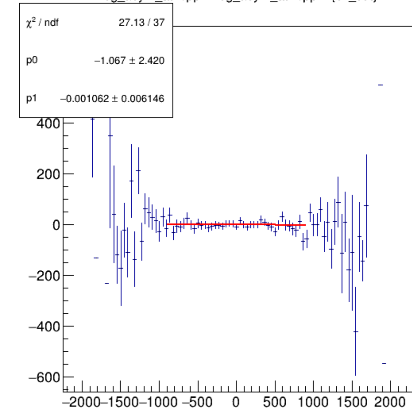
reg_asym_atl1/ppm:reg_asym_atr1/ppm {ok_cut}
