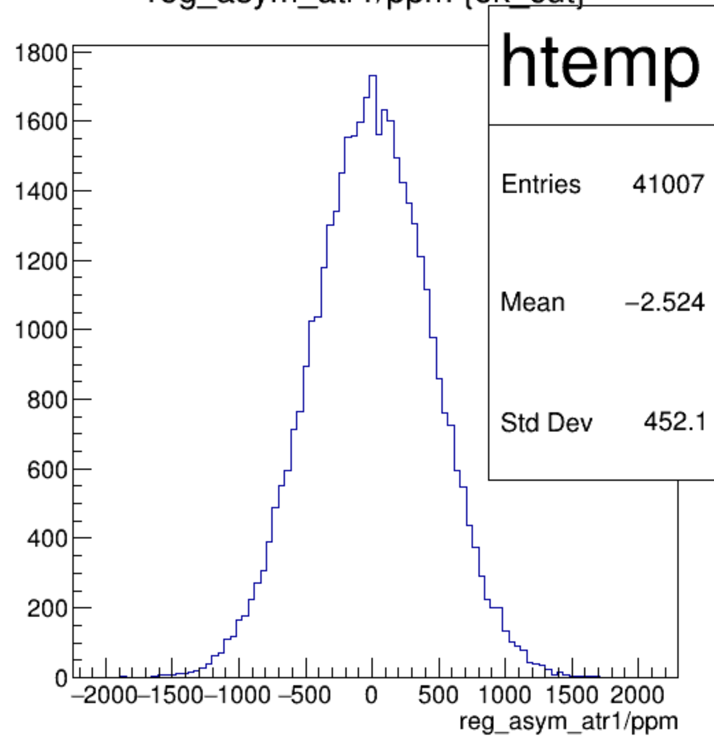
reg_asym_atr1/ppm {ok_cut}
