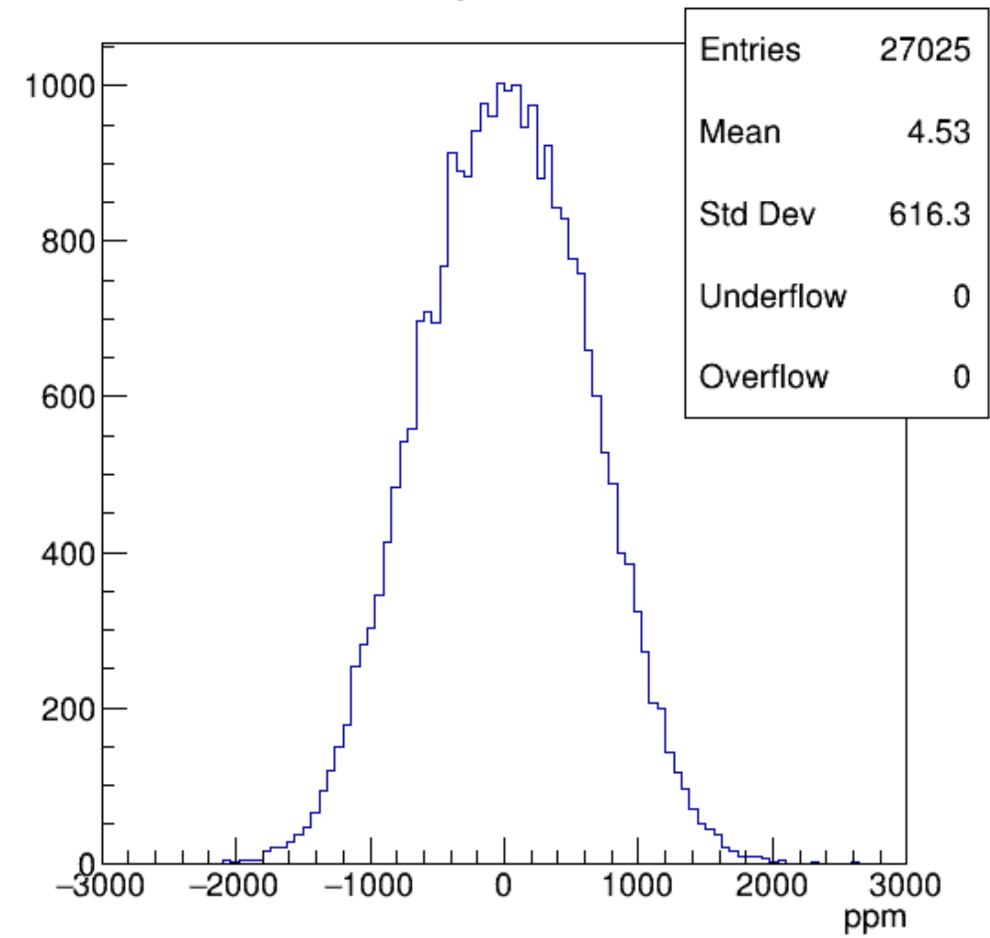
asym_dsl
