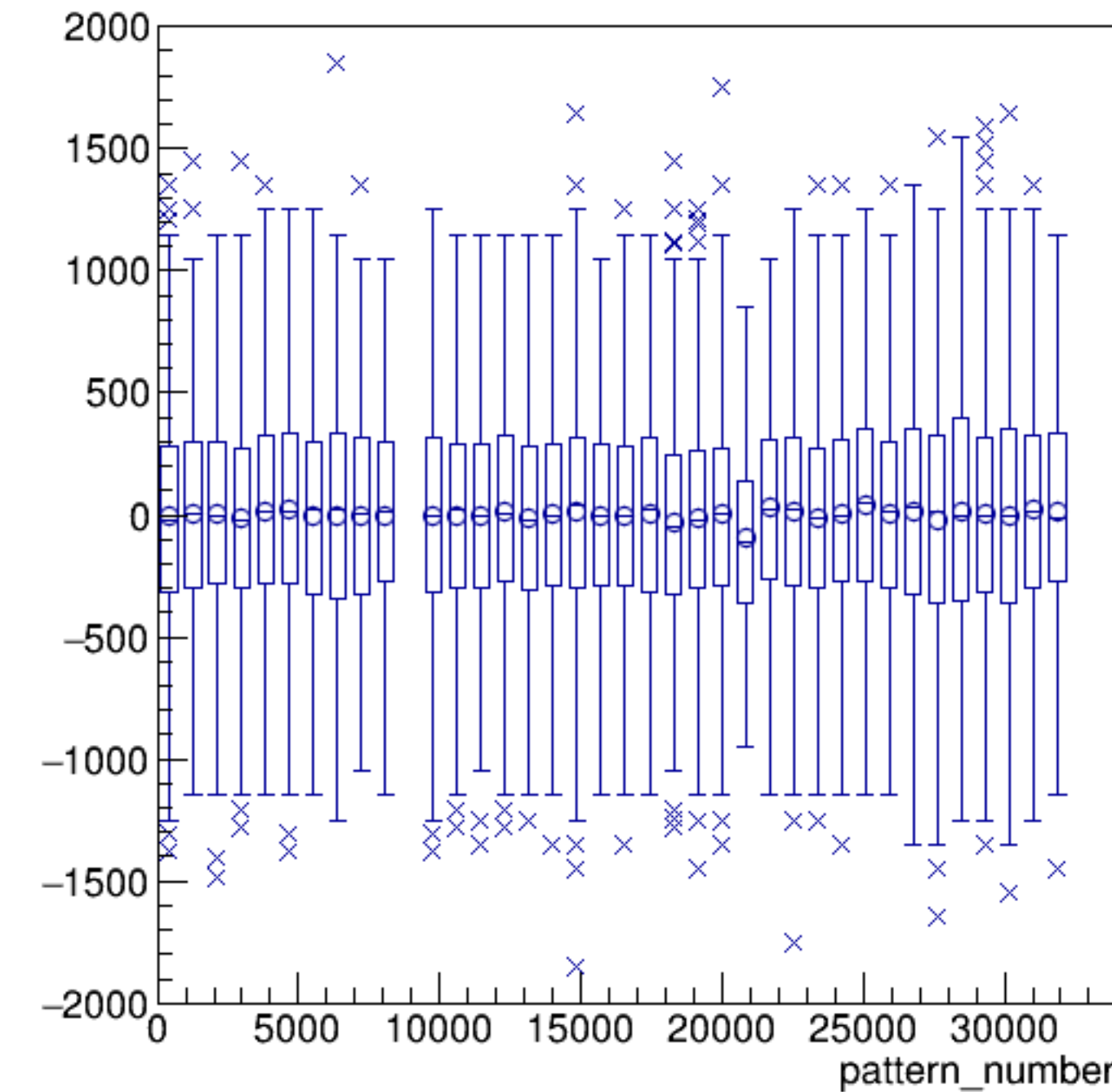
asym_dsr/ppm:pattern_number {ErrorFlag==0}
