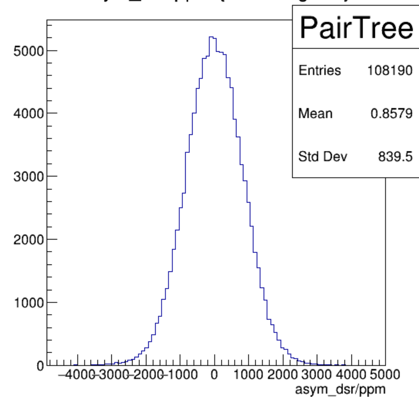
asym_dsr/ppm {ErrorFlag==0}
