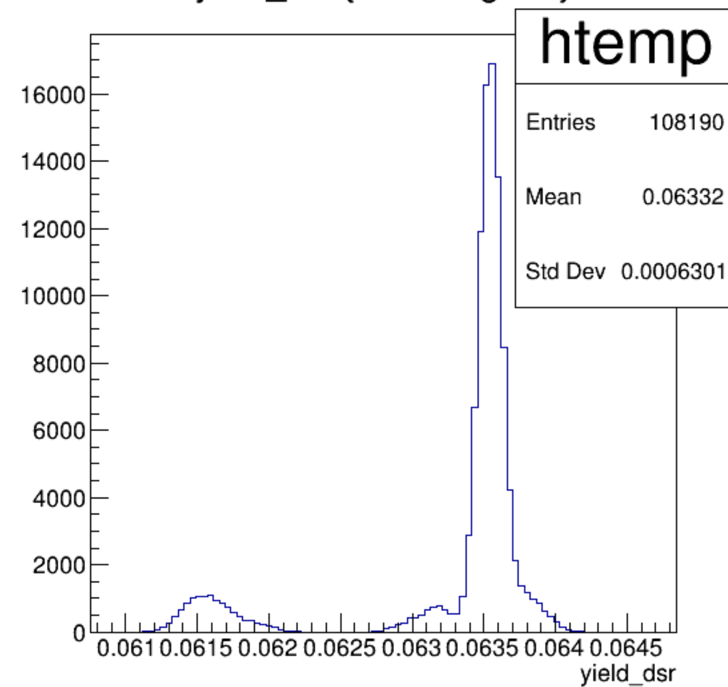
yield_dsr {ErrorFlag==0}
