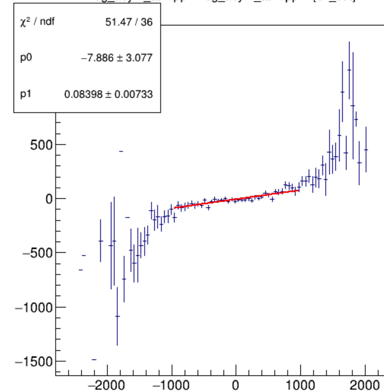
reg_asym_atl1/ppm:reg_asym_atr1/ppm {ok_cut}
