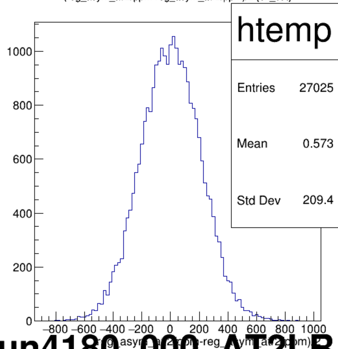
(reg_asym_atl2/ppm-reg_asym_atr2/ppm)/2 {ok_cut}
