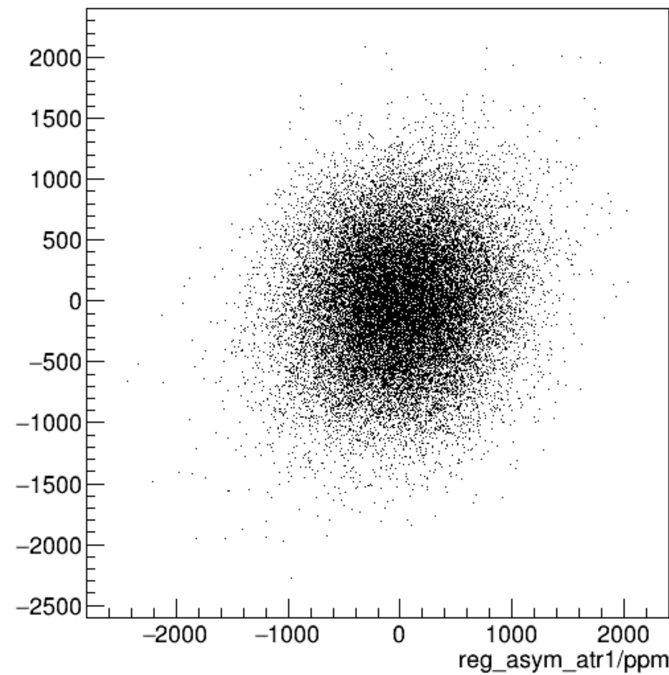
reg_asym_atl1/ppm:reg_asym_atr1/ppm {ok_cut}
