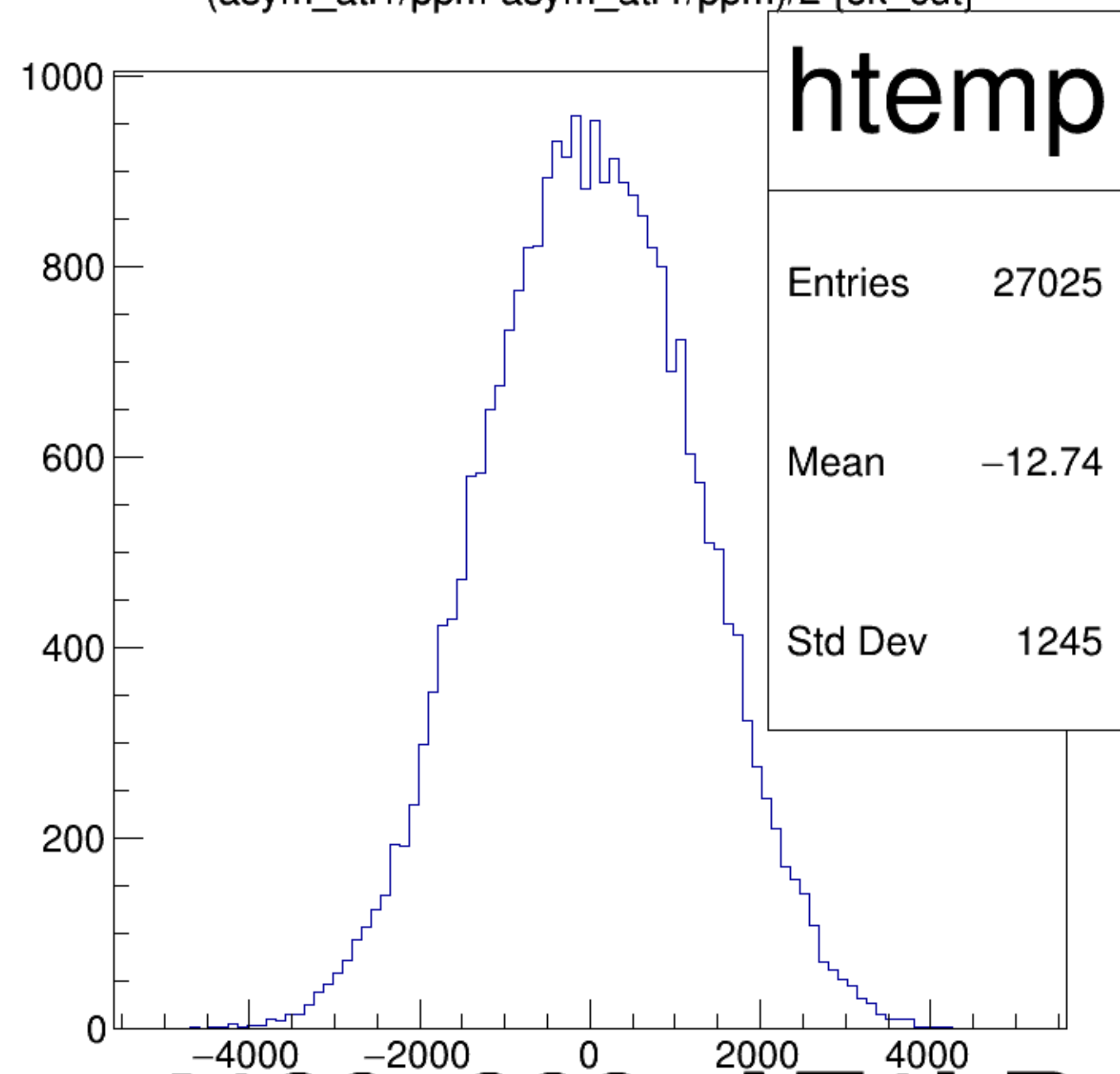
(asym_atl1/ppm-asym_atr1/ppm)/2 {ok_cut}
