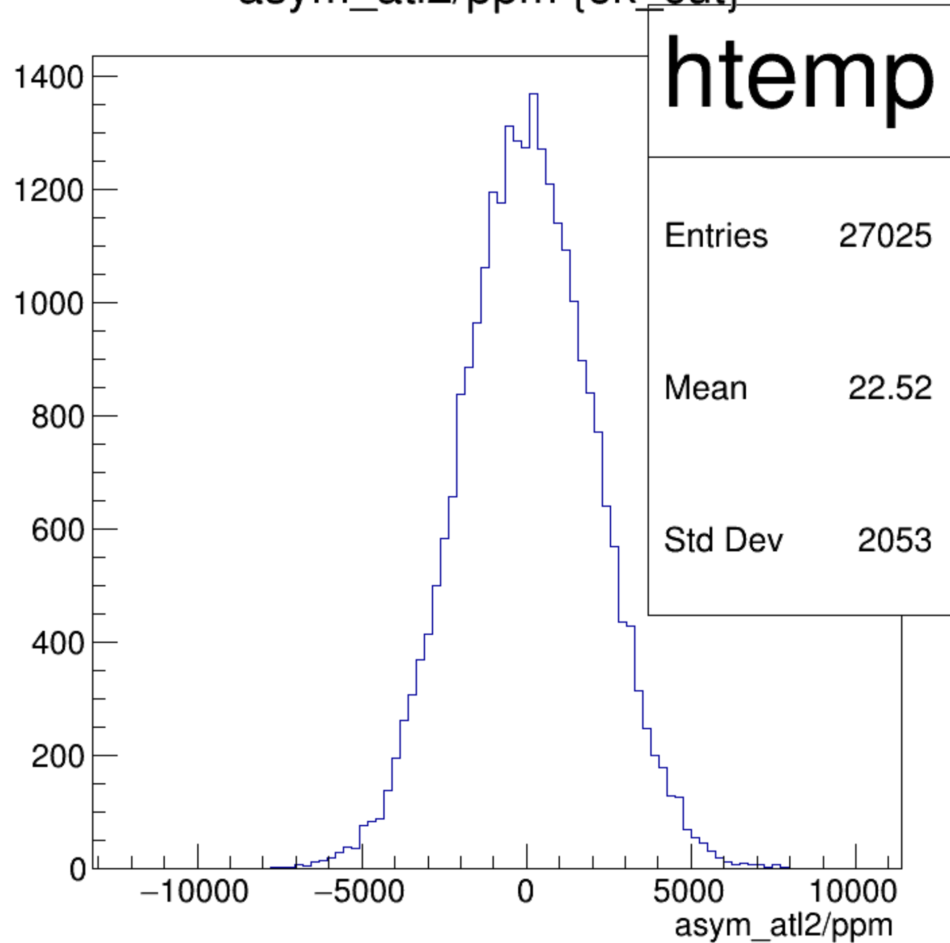
asym_atl2/ppm {ok_cut}
