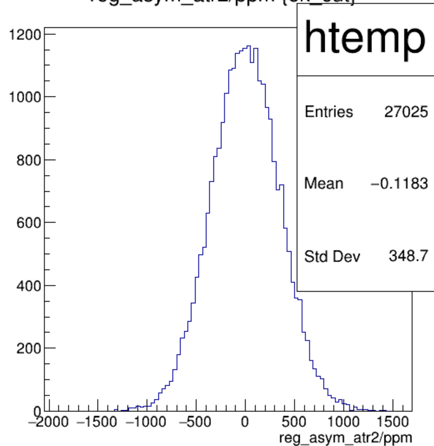
reg_asym_atr2/ppm {ok_cut}
