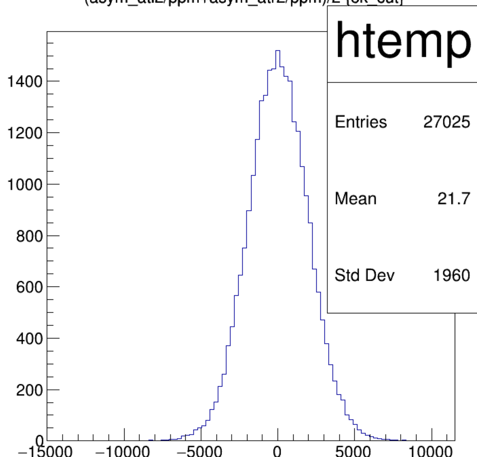
(asym_atl2/ppm+asym_atr2/ppm)/2 {ok_cut}
