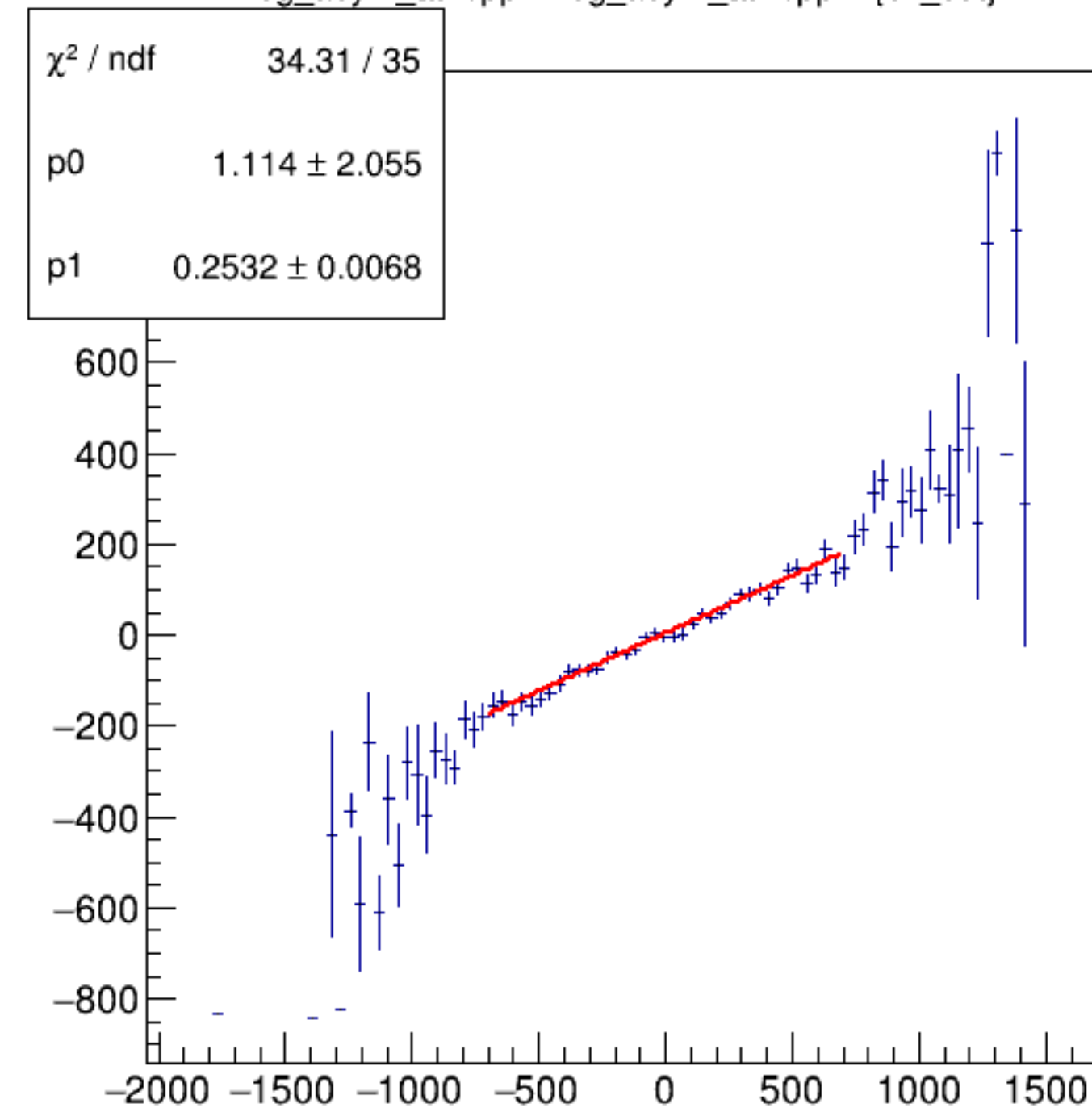
reg_asym_atl2/ppm:reg_asym_atr2/ppm {ok_cut}
