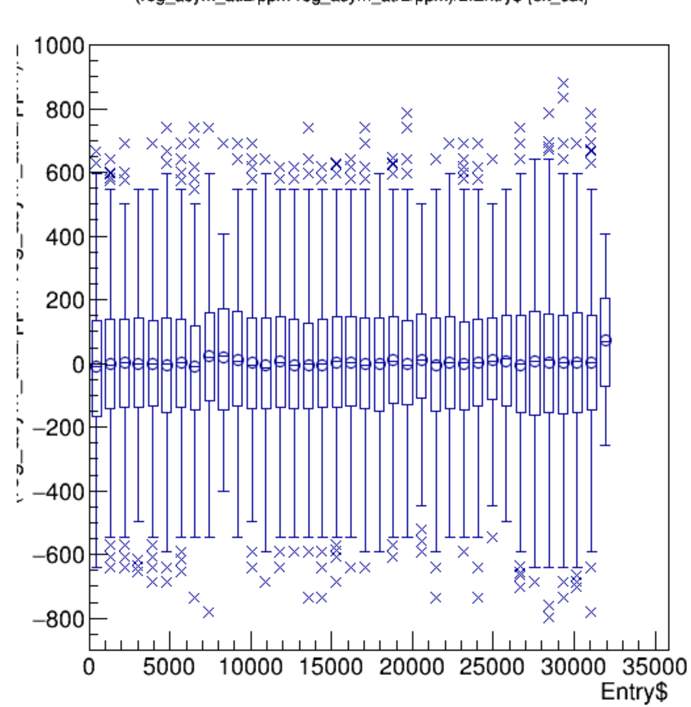
(reg_asym_atl2/ppm-reg_asym_atr2/ppm)/2:Entry$ {ok_cut}
