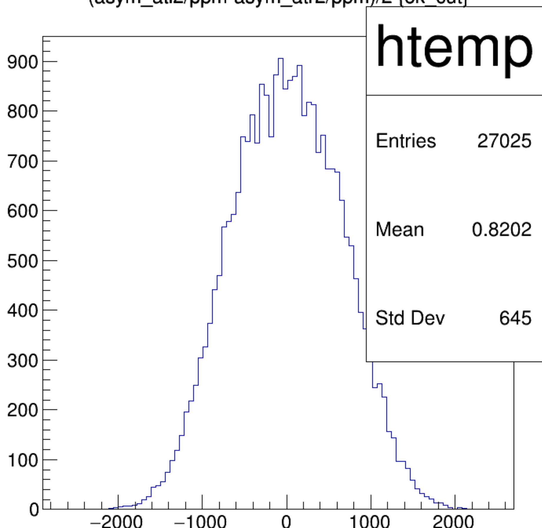
(asym_atl2/ppm-asym_atr2/ppm)/2 {ok_cut}
