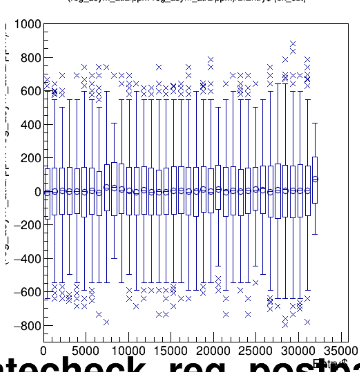
(reg_asym_atl2/ppm-reg_asym_atr2/ppm)/2:Entry$ {ok_cut}
