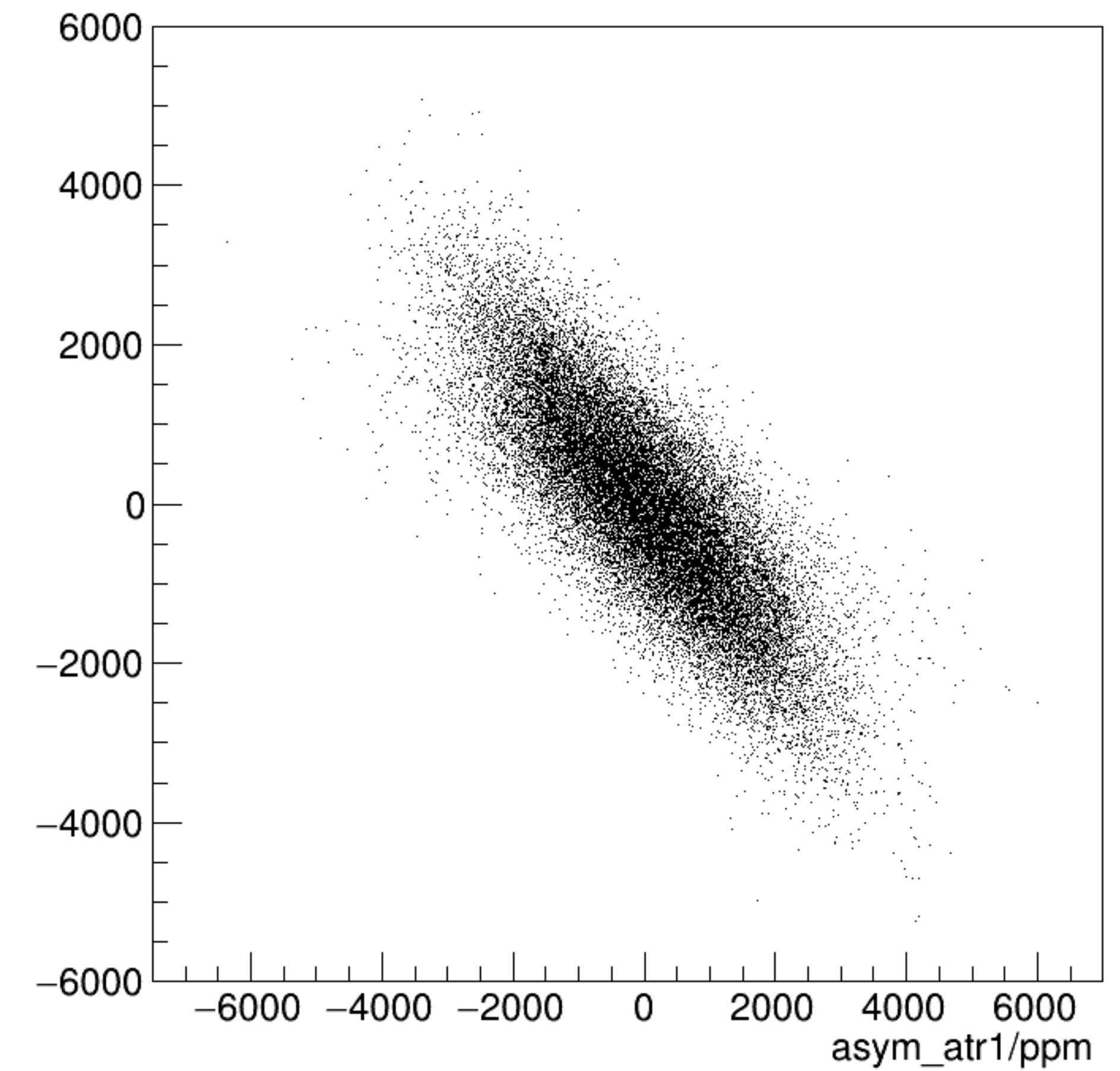
asym_atl1/ppm:asym_atr1/ppm {ok_cut}
