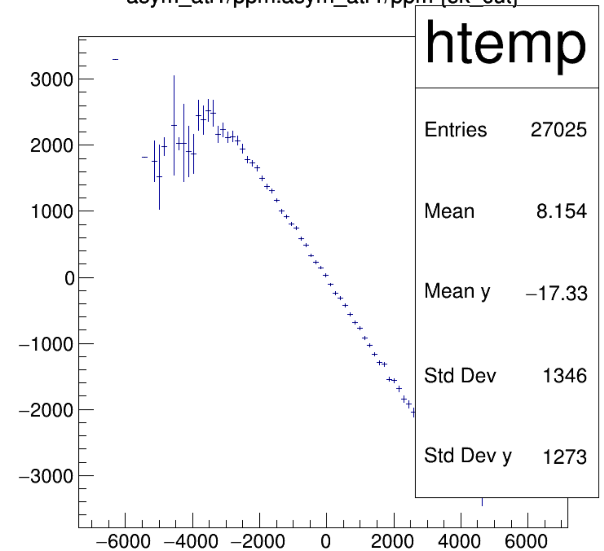
asym_atl1/ppm:asym_atr1/ppm {ok_cut}
