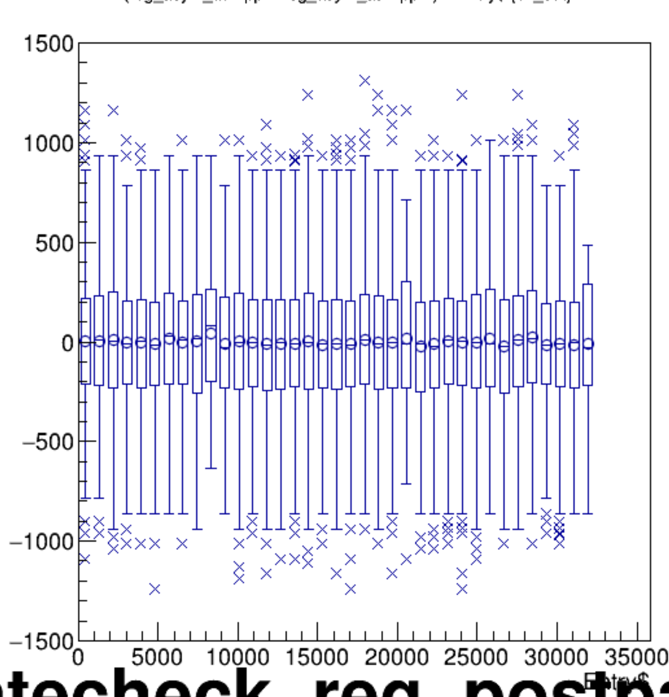
(reg_asym_atl1/ppm-reg_asym_atr1/ppm)/2:Entry$ {ok_cut}
