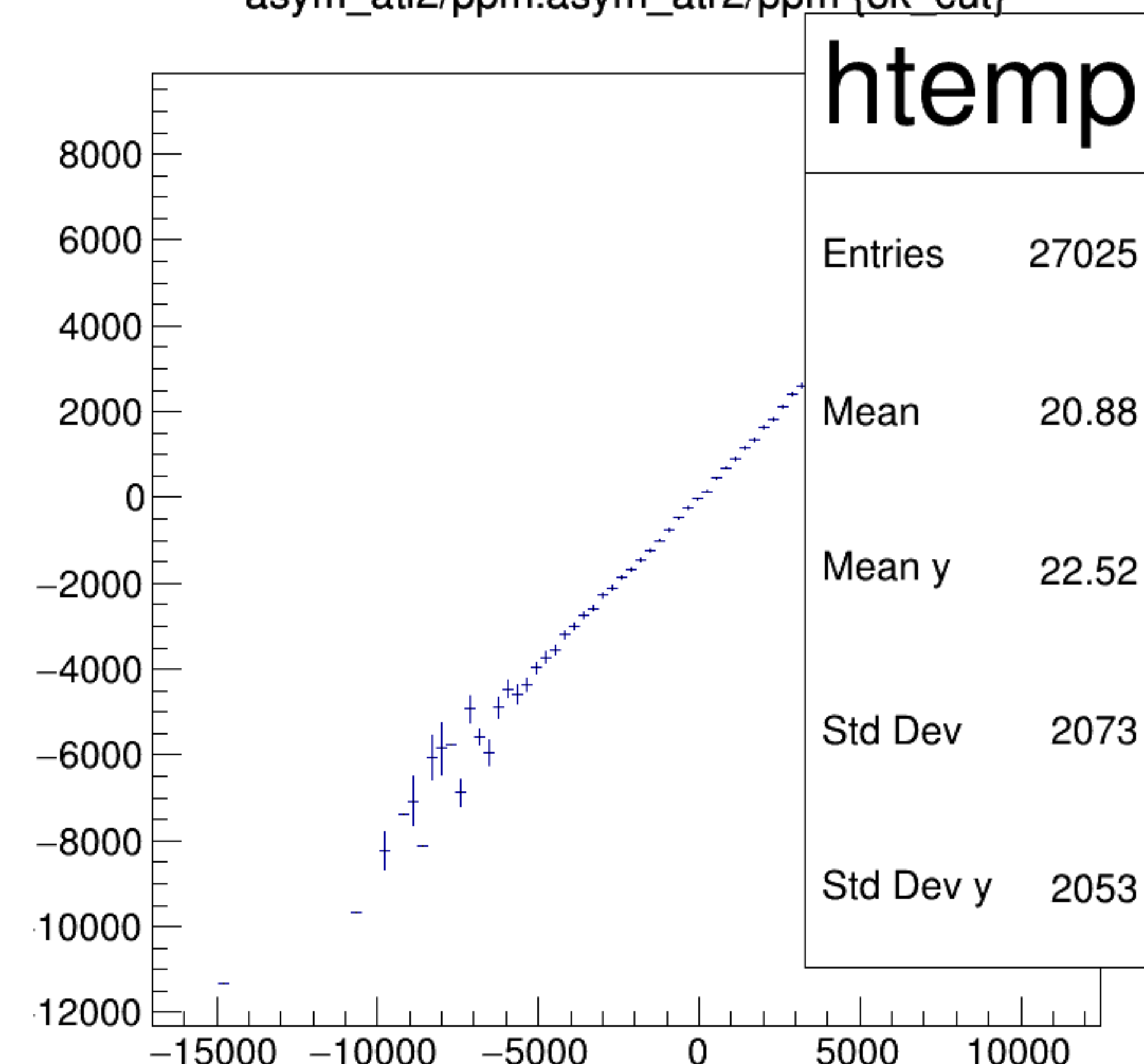
asym_atl2/ppm:asym_atr2/ppm {ok_cut}
