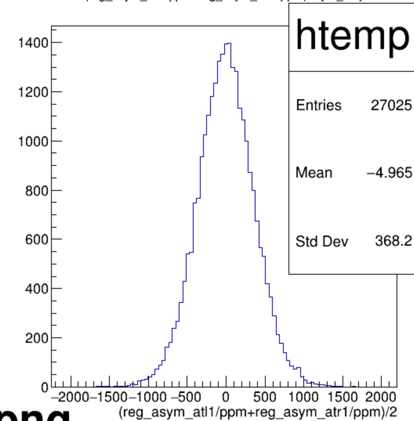
(reg_asym_atl1/ppm+reg_asym_atr1/ppm)/2 {ok_cut}
