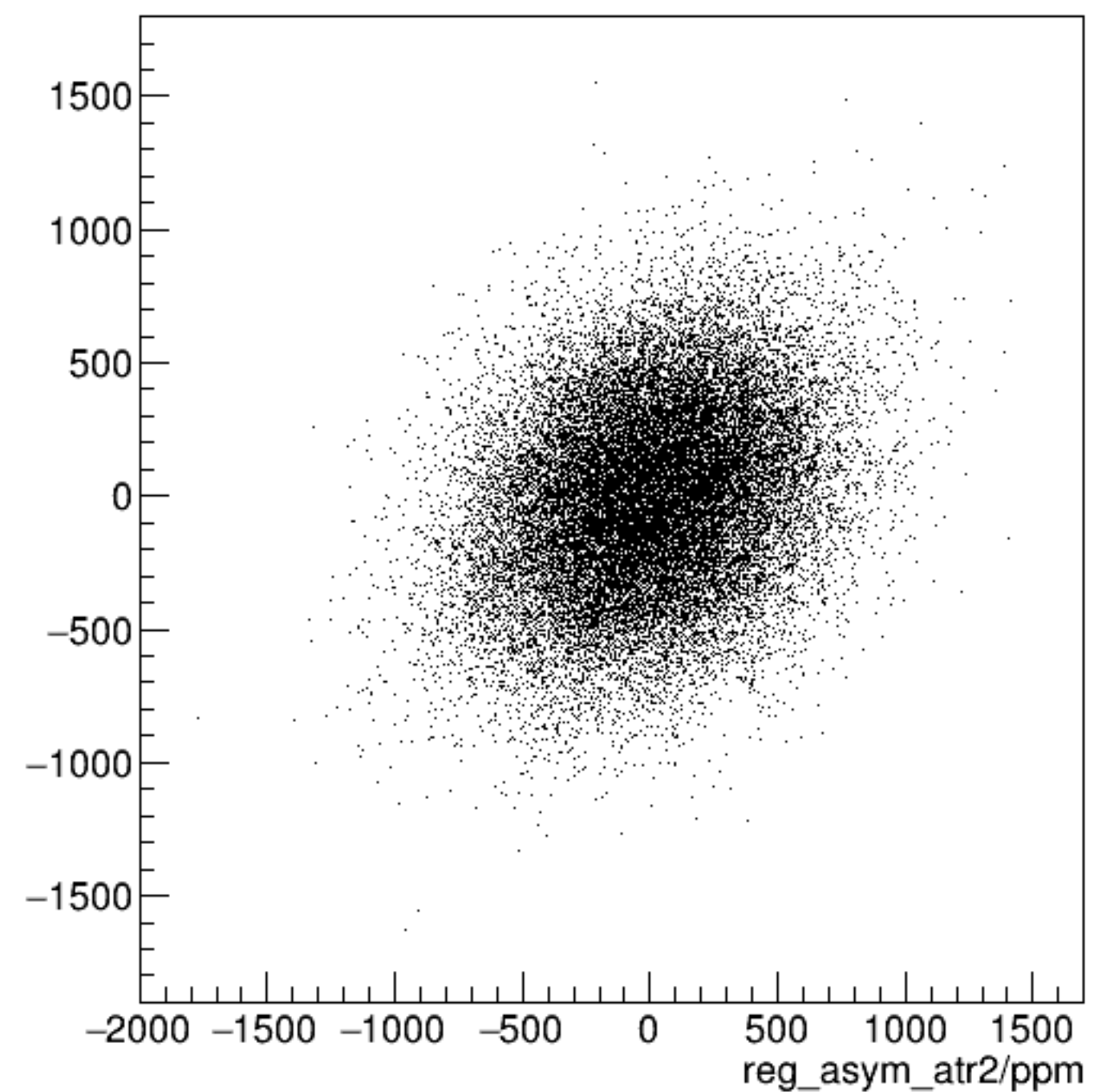
reg_asym_atl2/ppm:reg_asym_atr2/ppm {ok_cut}
