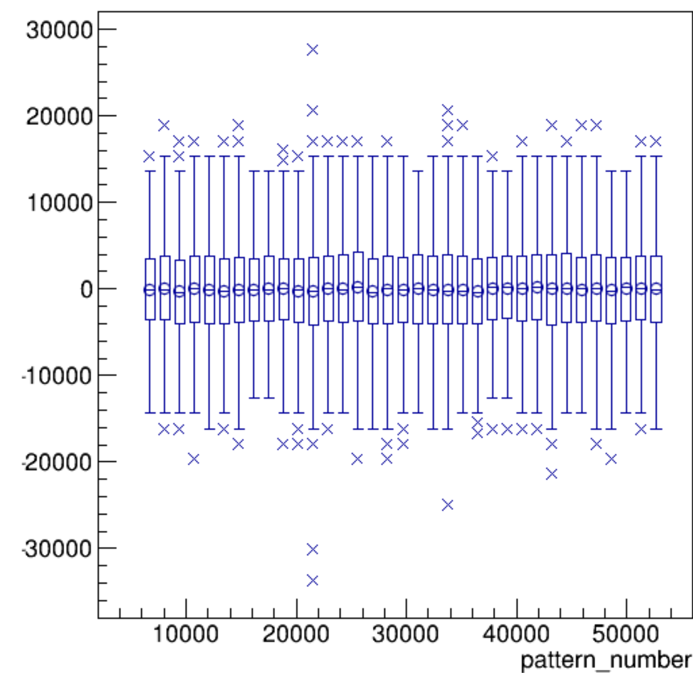
asym_sam4/ppm:pattern_number {ErrorFlag==0}
