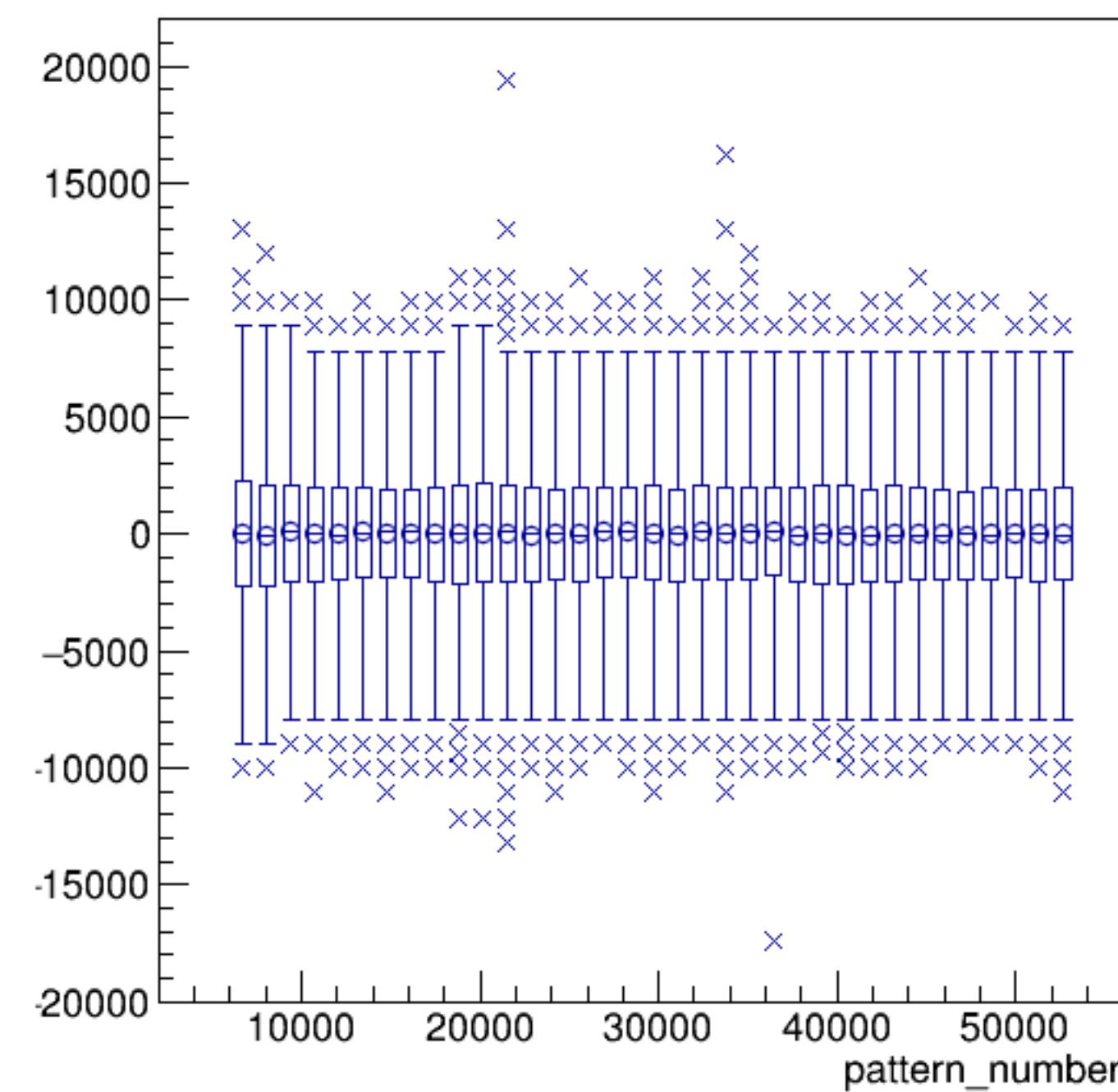
asym_sam7/ppm:pattern_number {ErrorFlag==0}
