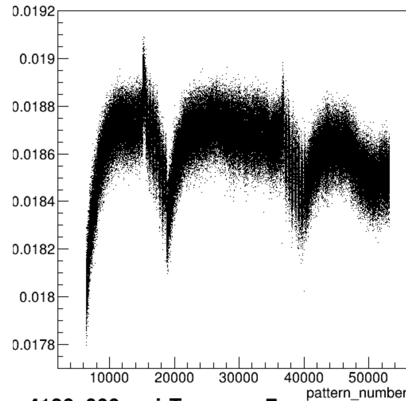
yield_sam7:pattern_number {ErrorFlag==0}
