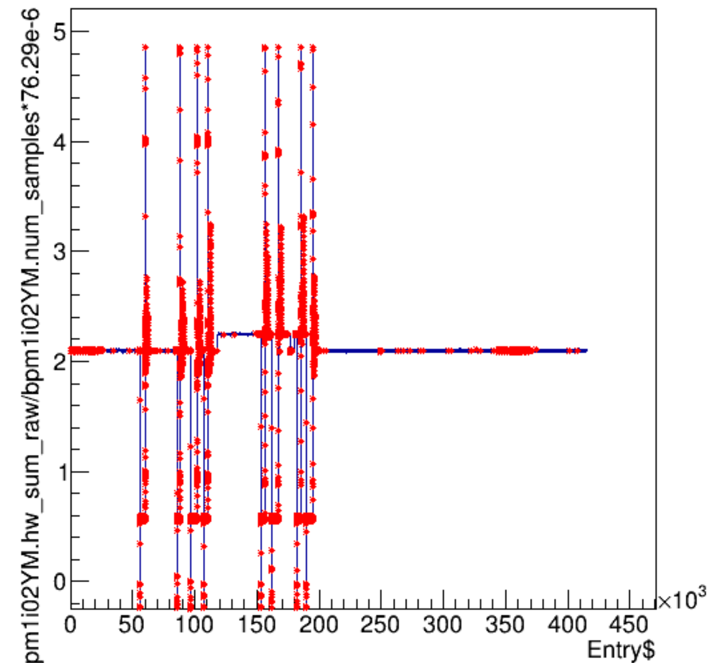
bpm1i02YM.hw_sum_raw/bpm1i02YM.num_samples*76.29e-6:Entry$
