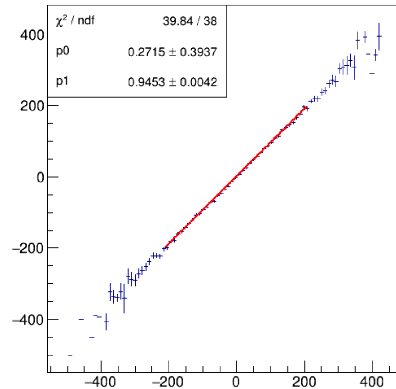
asym_bpm16WS/ppm:Aq/ppm {ErrorFlag==0}
