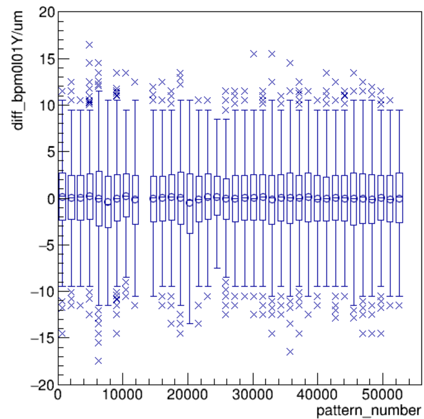
diff_bpm0l01Y/um:pattern_number {ErrorFlag==0}
