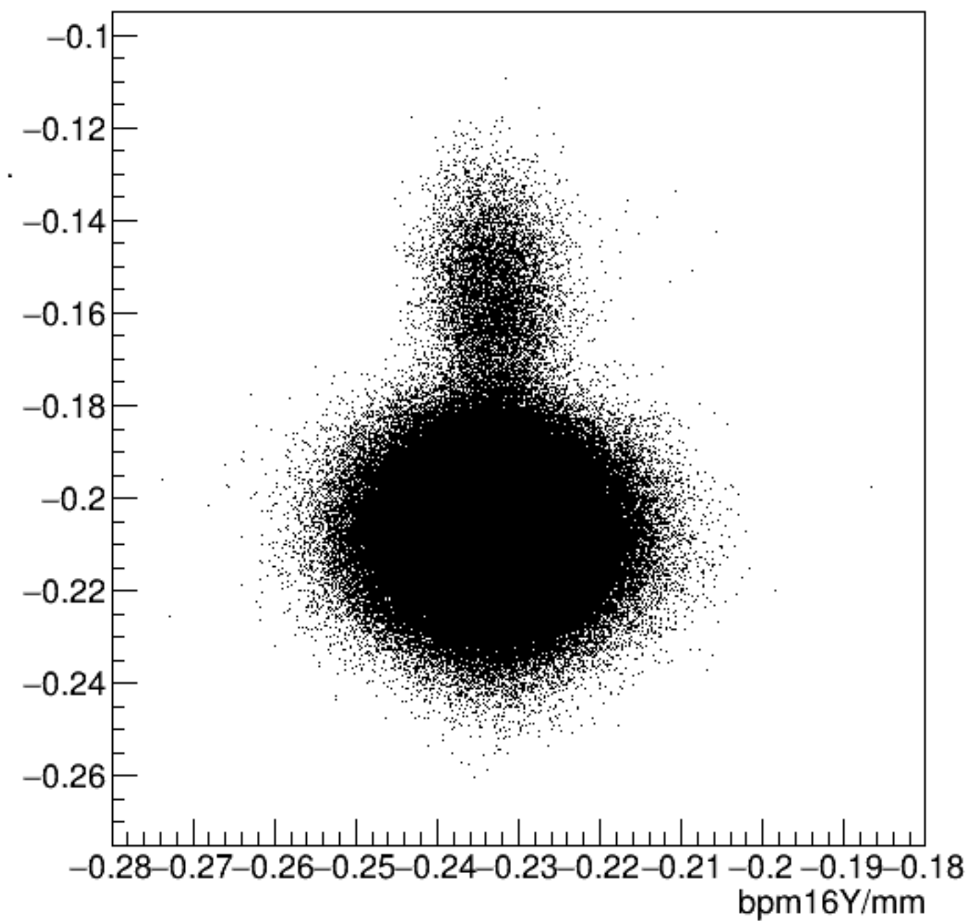
bpm16X/mm:bpm16Y/mm {ErrorFlag==0}
