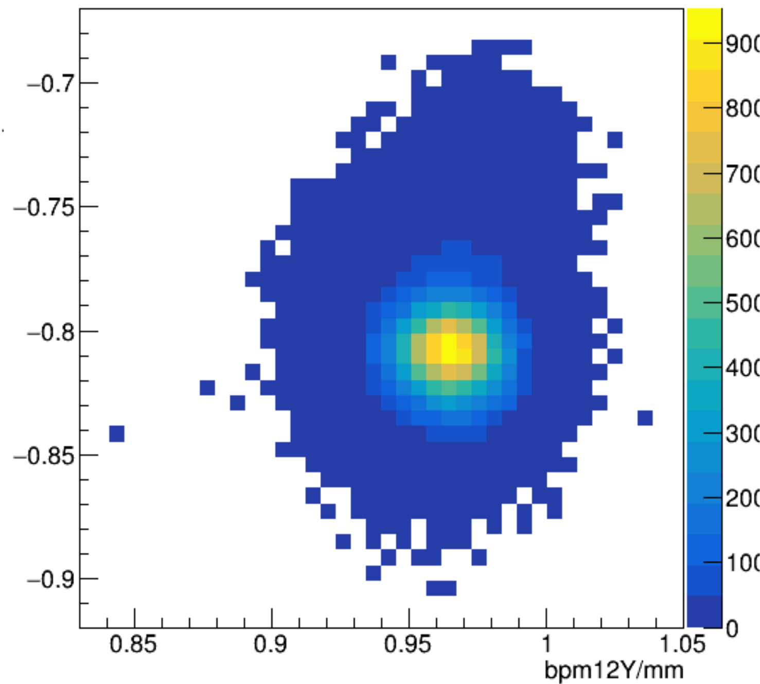
bpm12X/mm:bpm12Y/mm {ErrorFlag==0}
