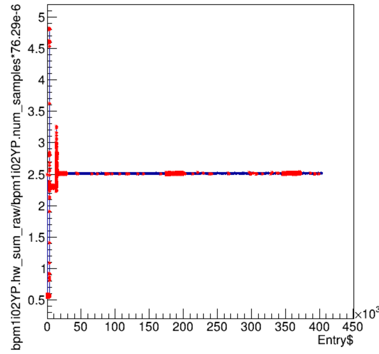
bpm1i02YP.hw_sum_raw/bpm1i02YP.num_samples*76.29e-6:Entry$
