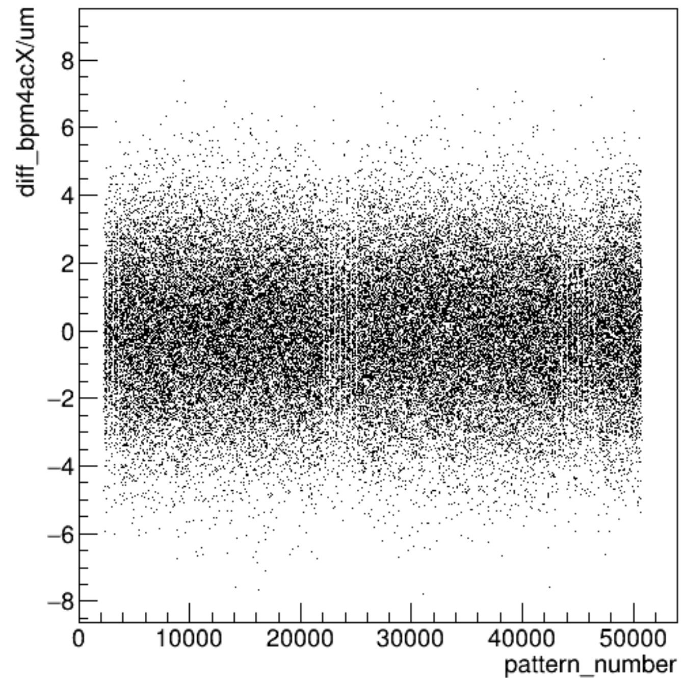
diff_bpm4acX/um:pattern_number {ErrorFlag==0}
