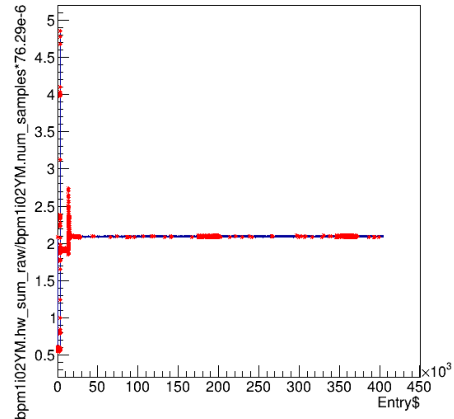
bpm1i02YM.hw_sum_raw/bpm1i02YM.num_samples*76.29e-6:Entry$
