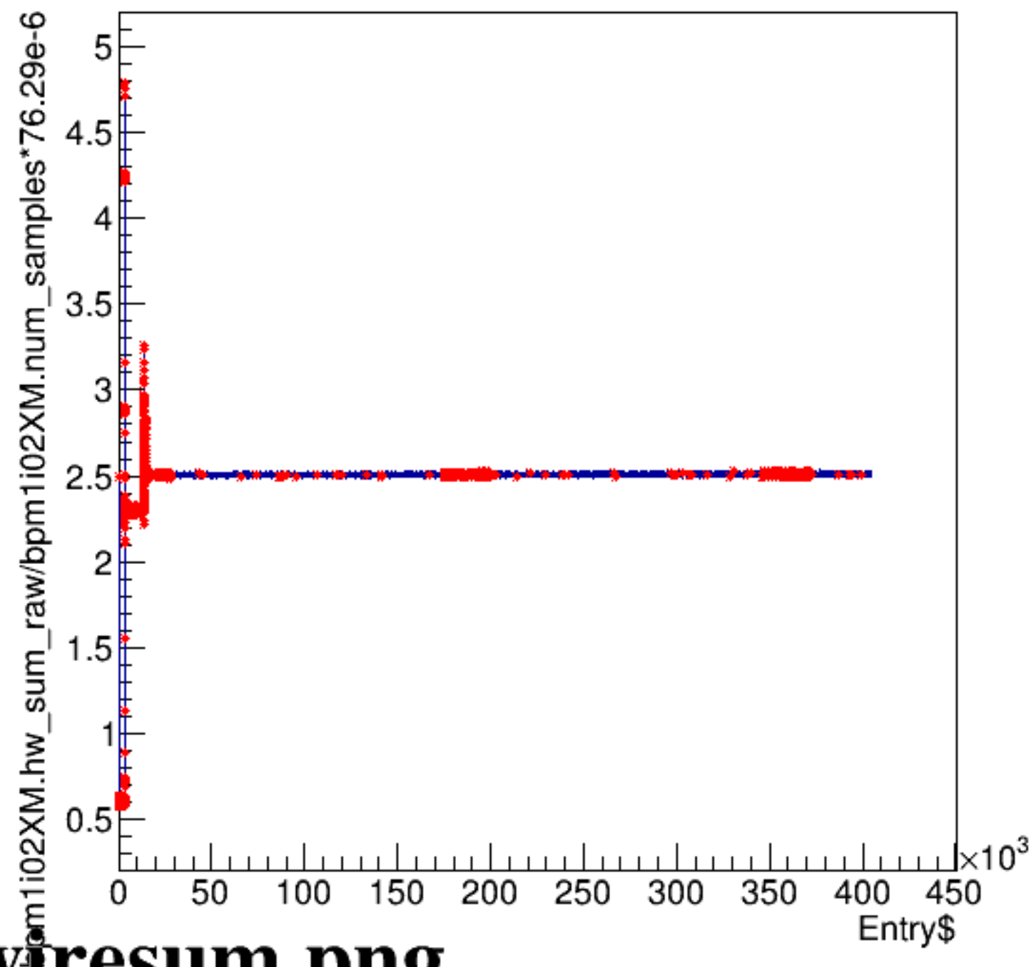
bpm1i02XM.hw_sum_raw/bpm1i02XM.num_samples*76.29e-6:Entry$
