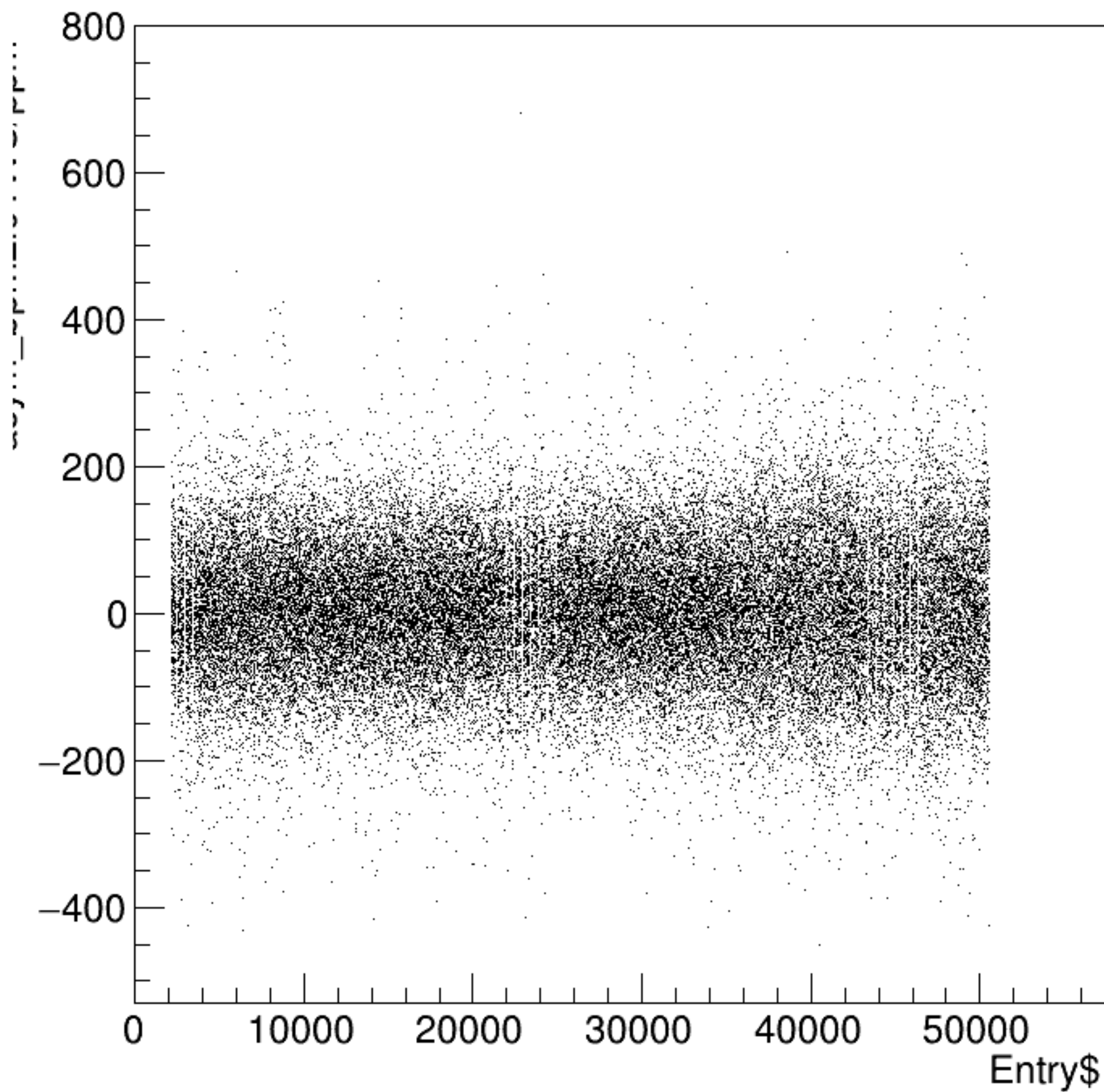
asym_bpm2i01WS/ppm:Entry$ {ErrorFlag==0}
