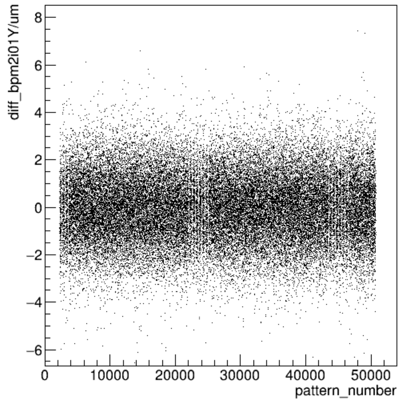
diff_bpm2i01Y/um:pattern_number {ErrorFlag==0}
