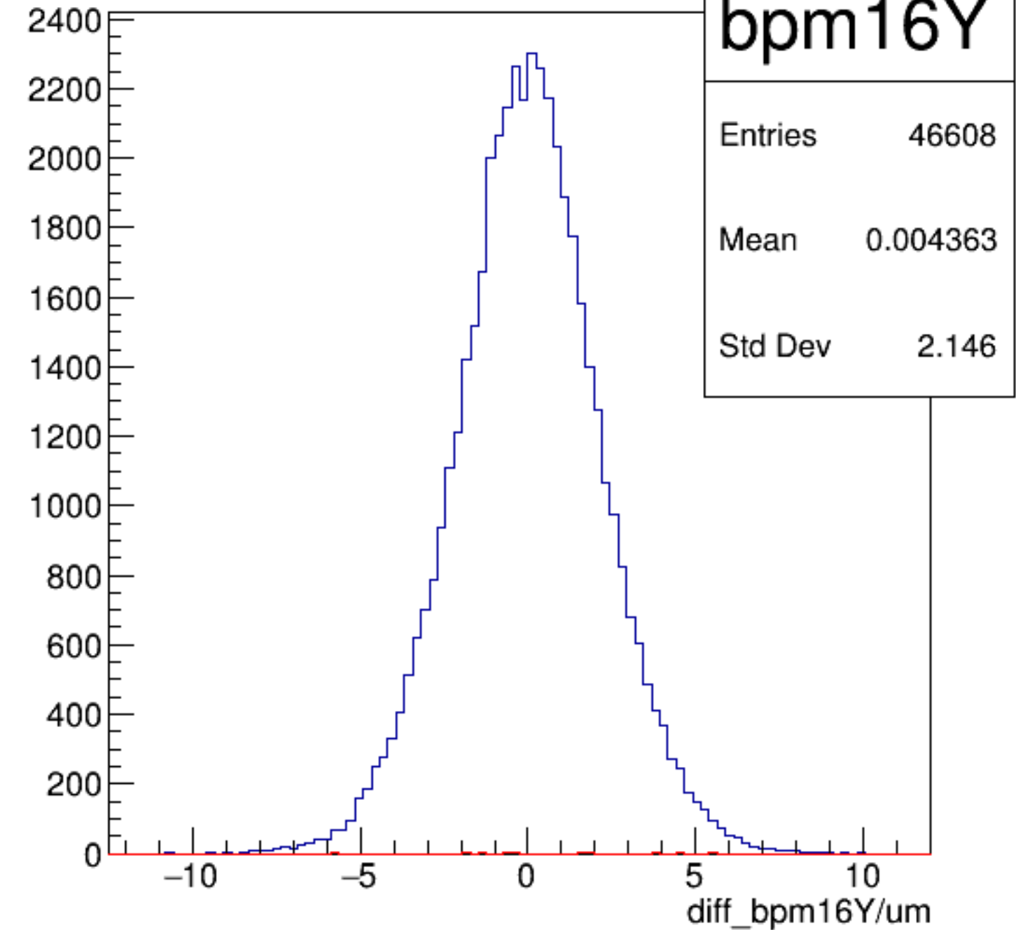
diff_bpm16Y/um {ErrorFlag==0}
