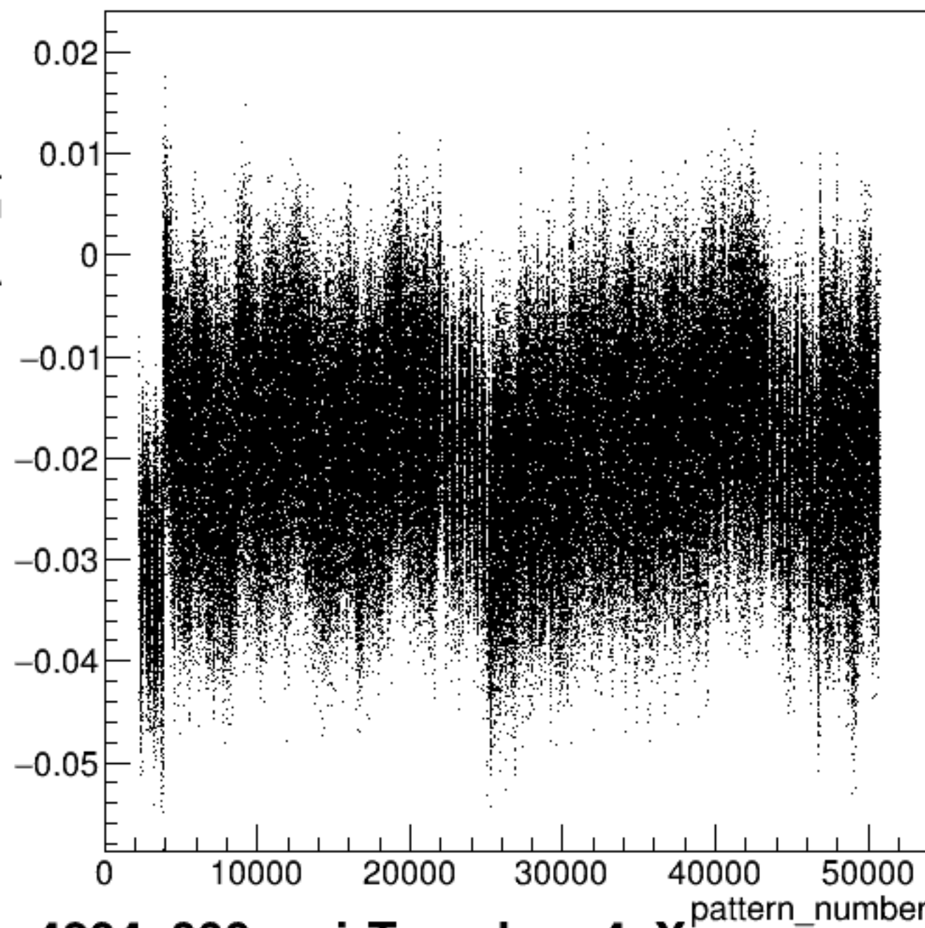
yield_bpm4aX/mm:pattern_number {ErrorFlag==0}
