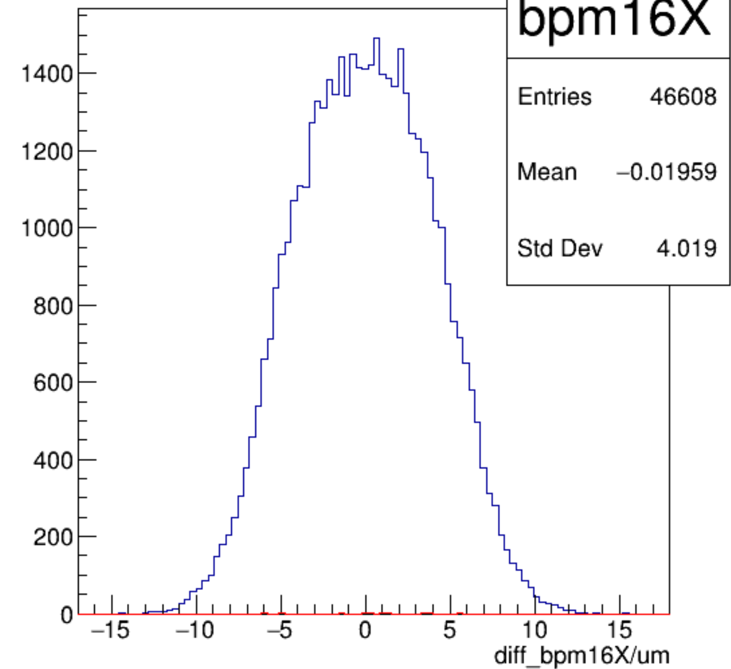
diff_bpm16X/um {ErrorFlag==0}
