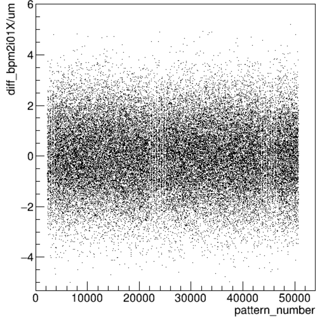
diff_bpm2i01X/um:pattern_number {ErrorFlag==0}
