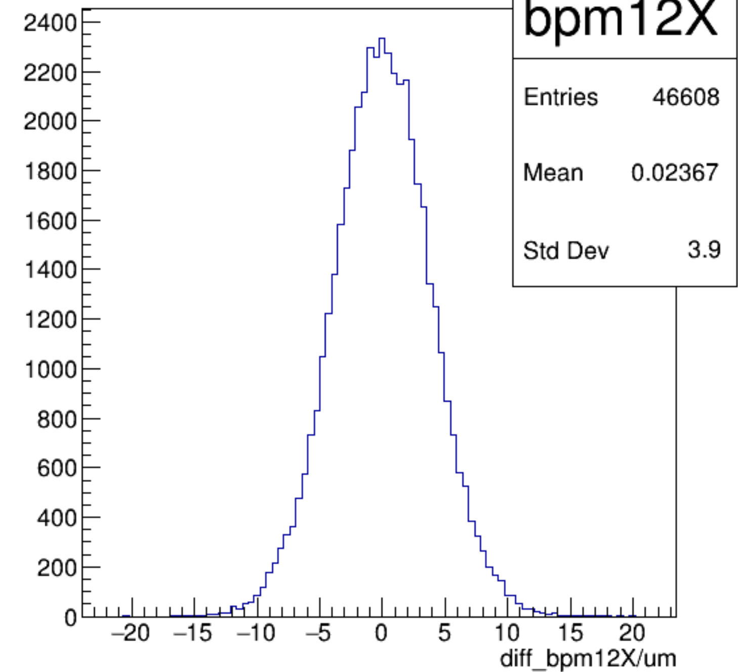
diff_bpm12X/um {ErrorFlag==0}
