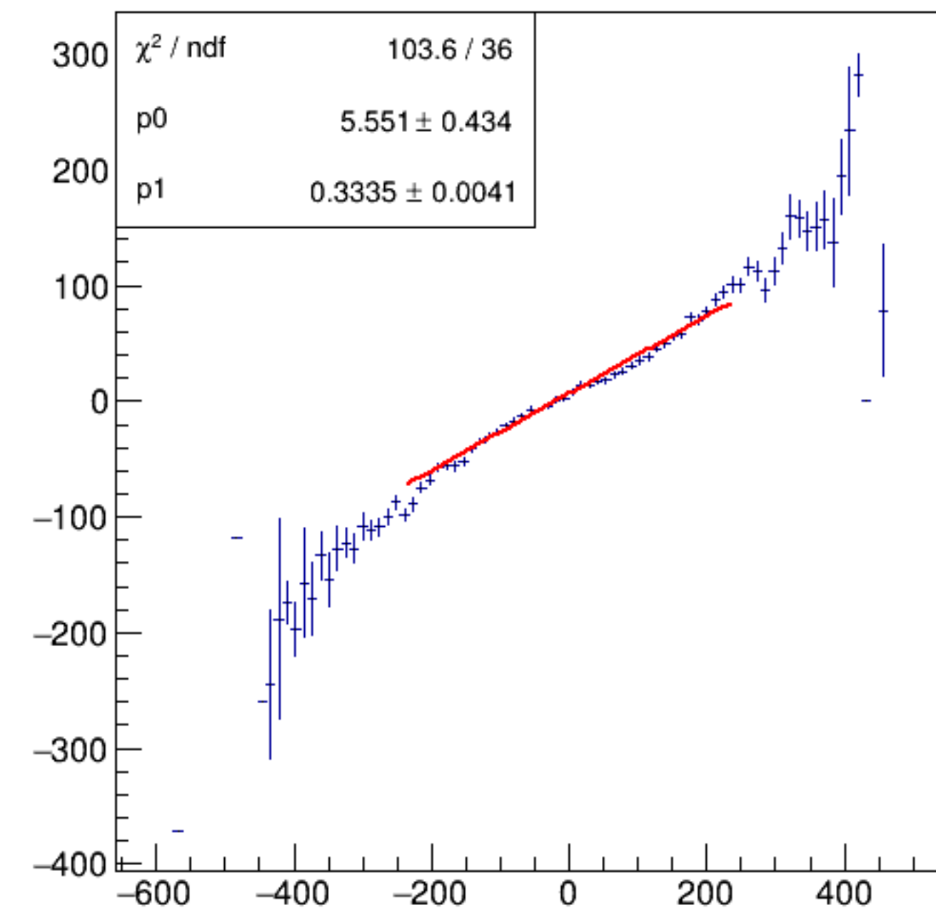
asym_bpm1i02WS/ppm:Aq/ppm {ErrorFlag==0}
