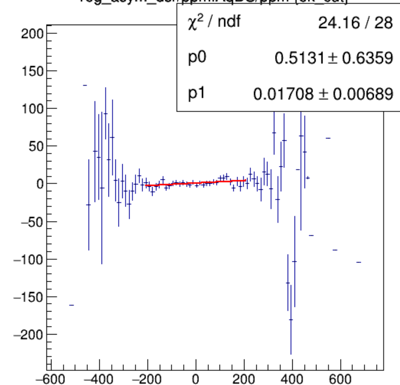
reg_asym_dsr/ppm:AqDS/ppm {ok_cut}
