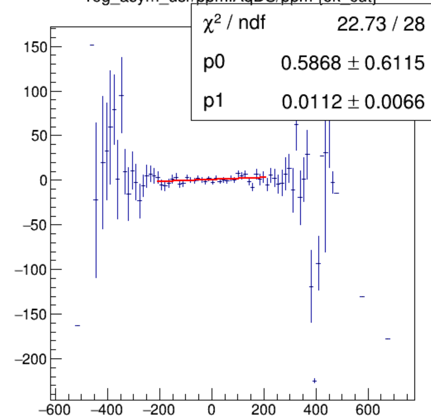
reg_asym_usr/ppm:AqDS/ppm {ok_cut}
