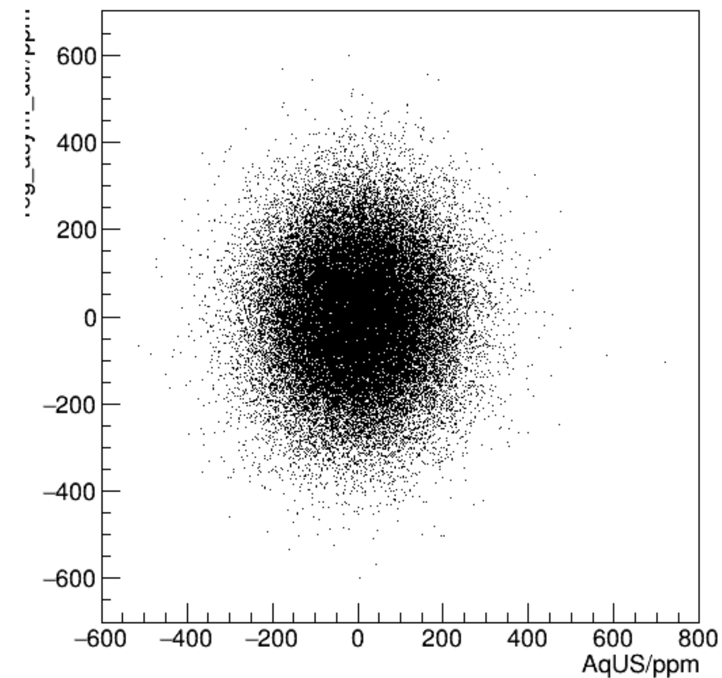
reg_asym_dsr/ppm:AqUS/ppm {ok_cut}
