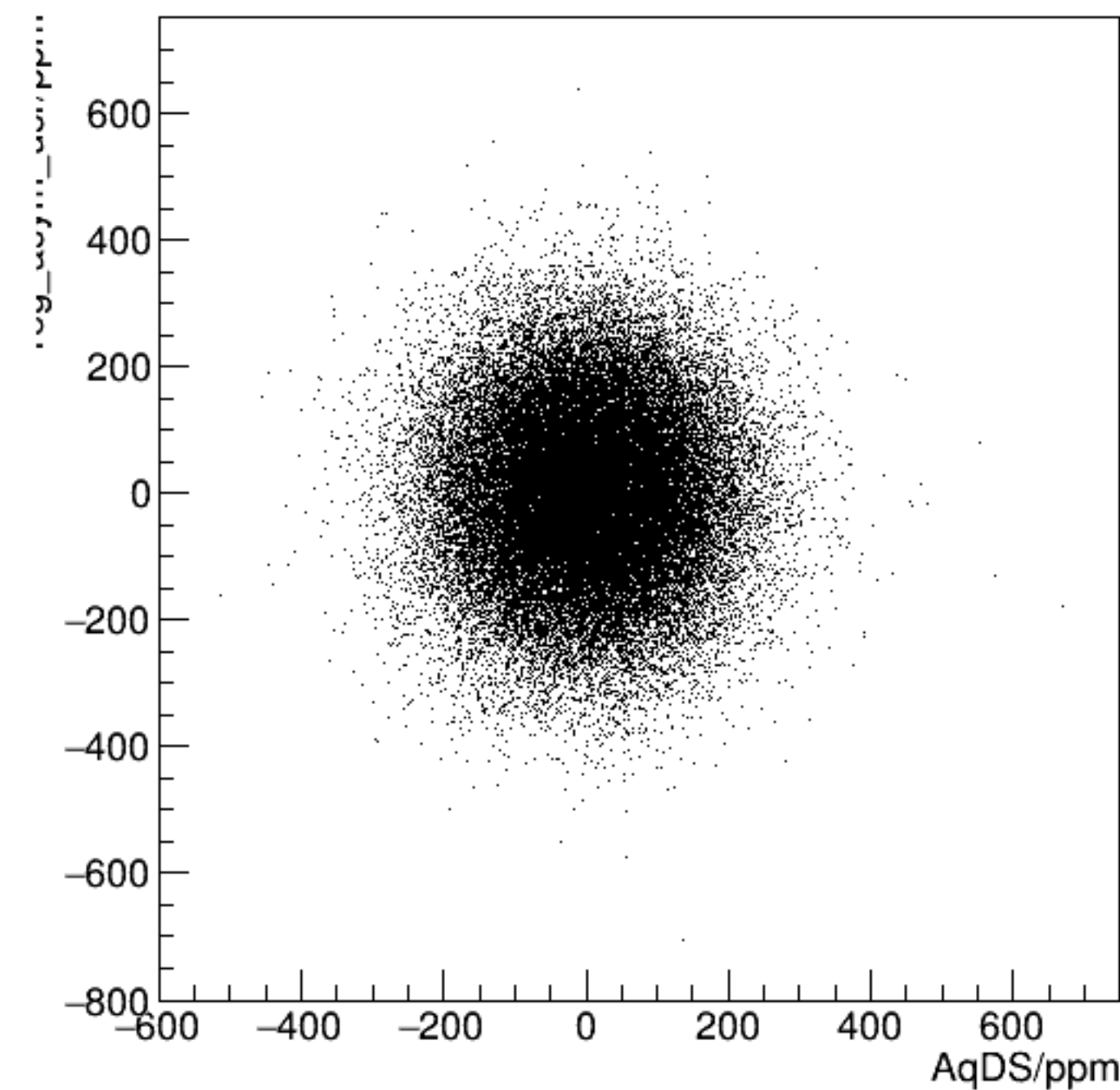
reg_asym_usr/ppm:AqDS/ppm {ok_cut}
