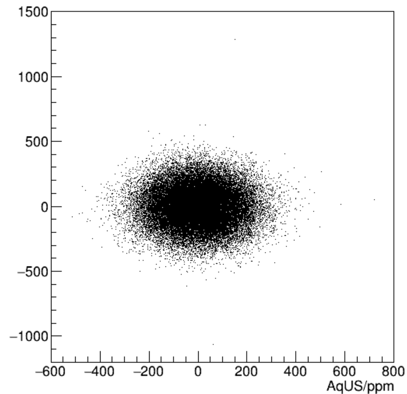
reg_asym_dsl/ppm:AqUS/ppm {ok_cut}
