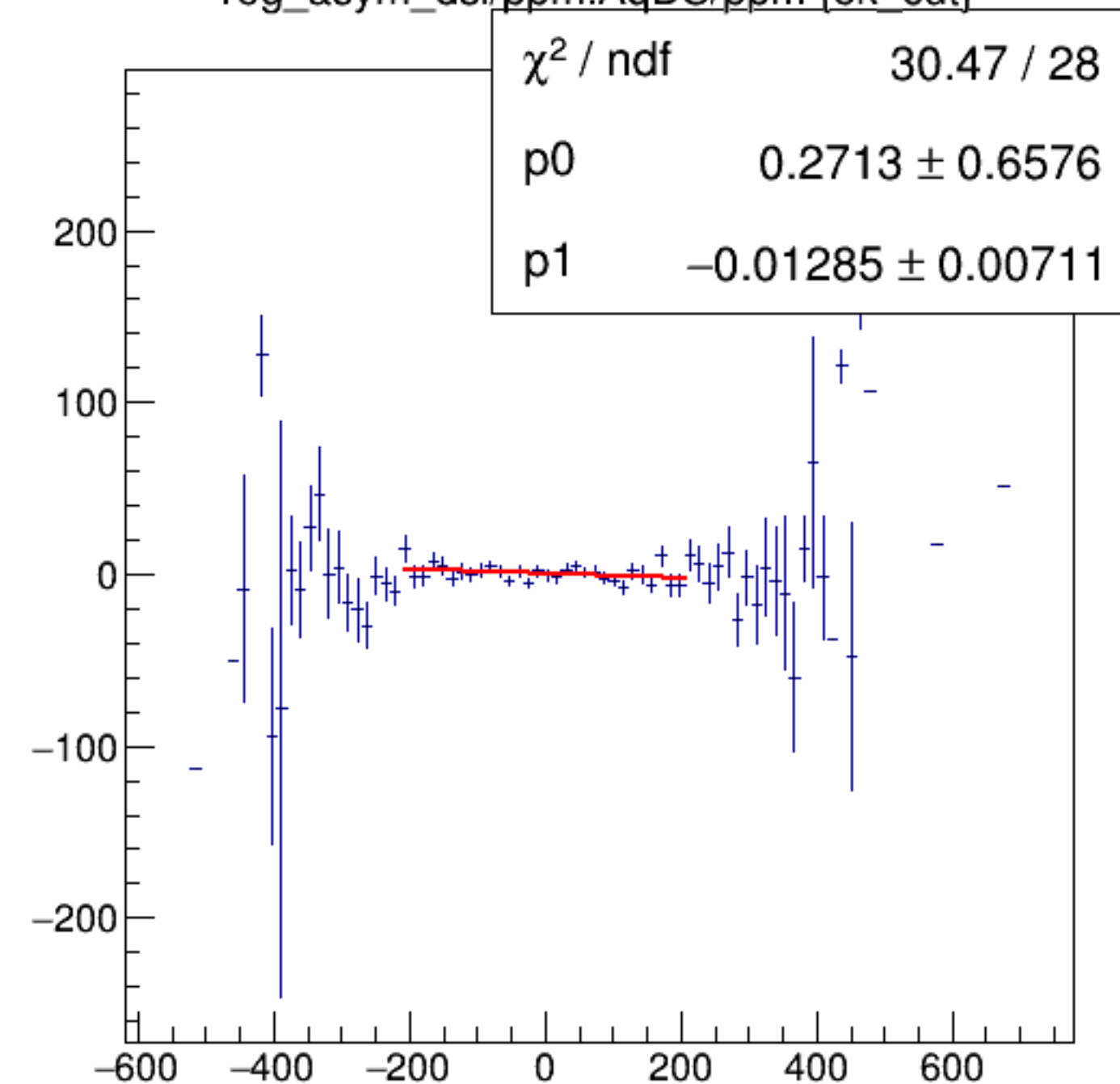
reg_asym_dsl/ppm:AqDS/ppm {ok_cut}
