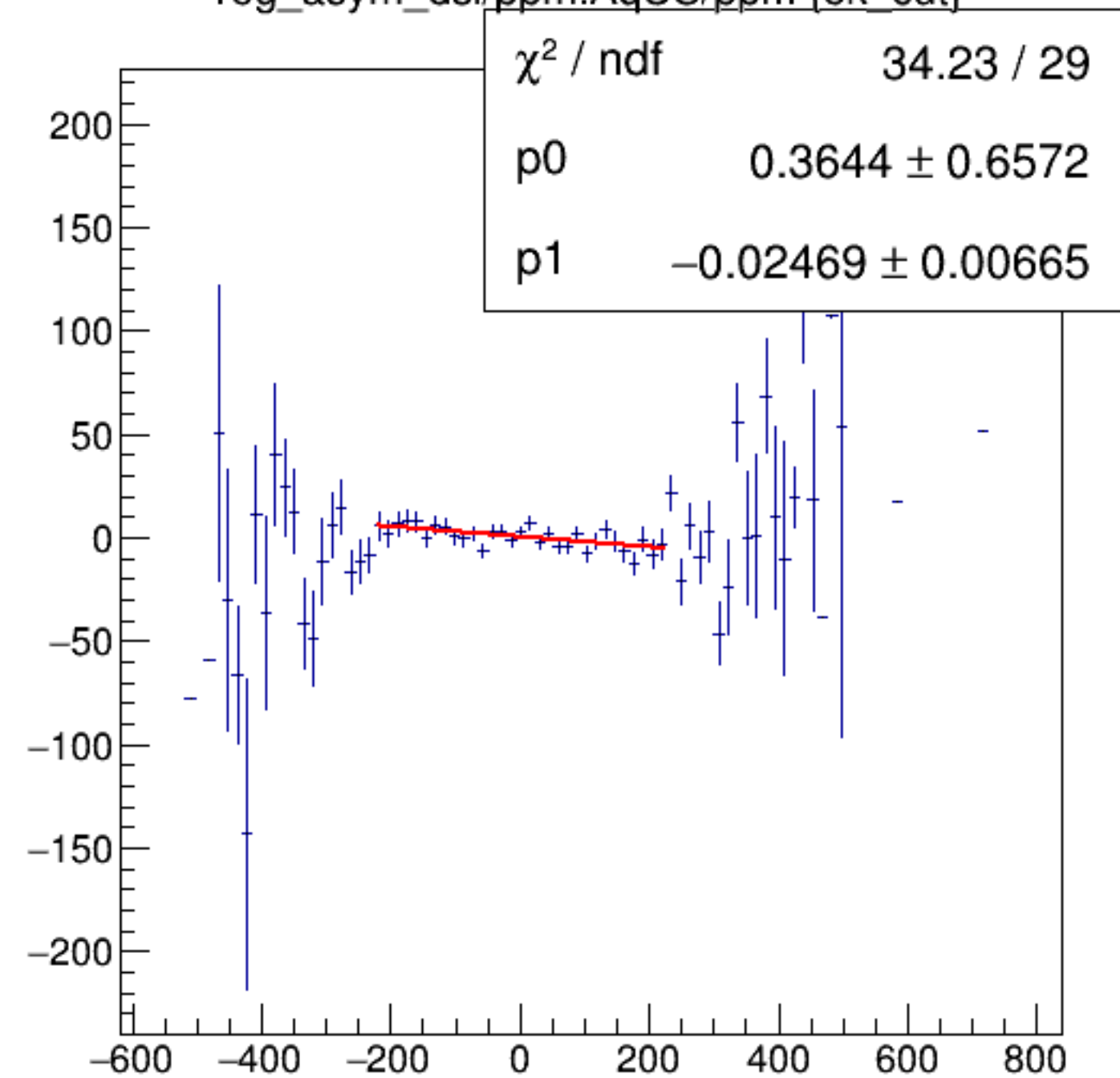
reg_asym_dsl/ppm:AqUS/ppm {ok_cut}
