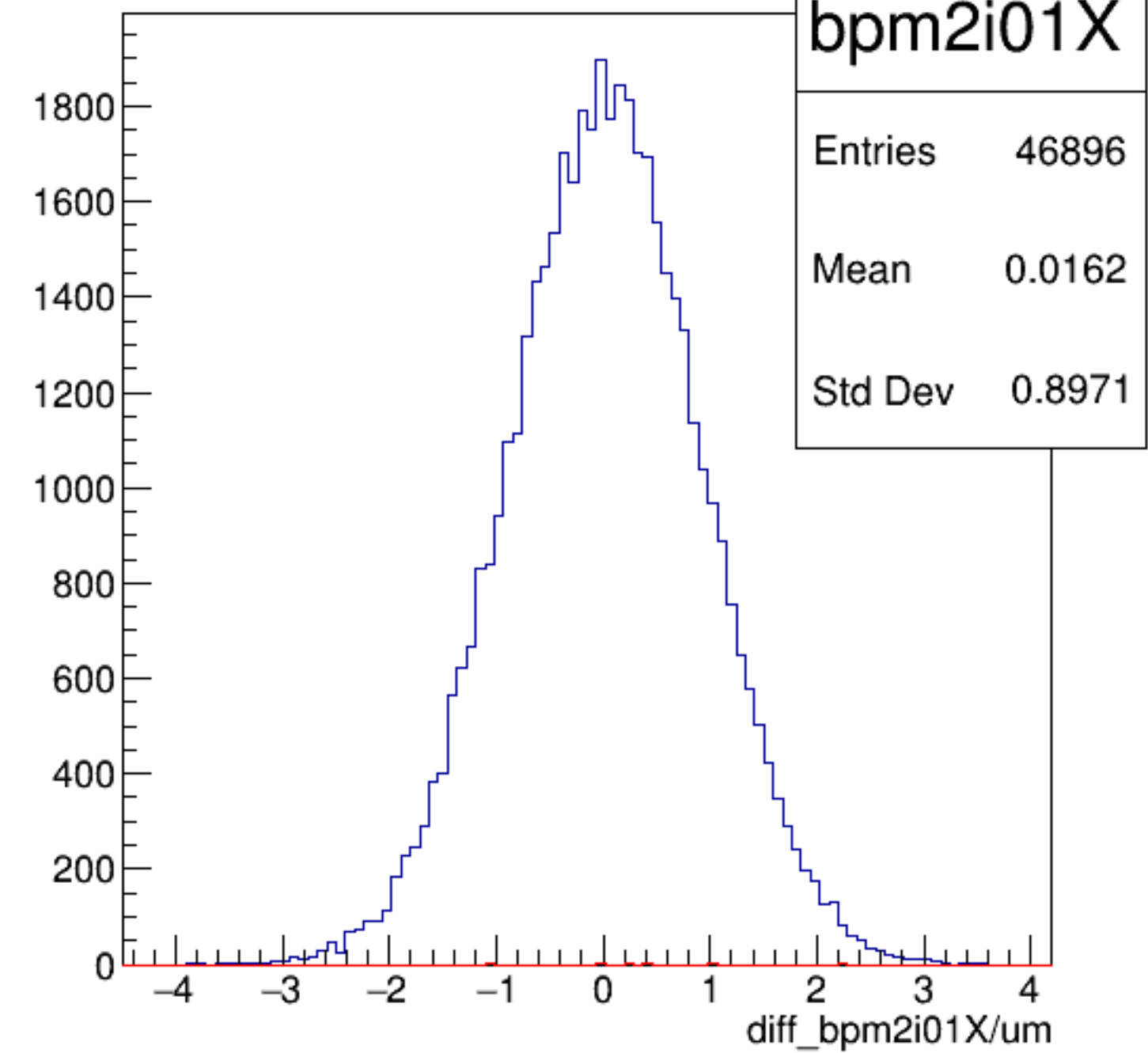
diff_bpm2i01X/um {ErrorFlag==0}
