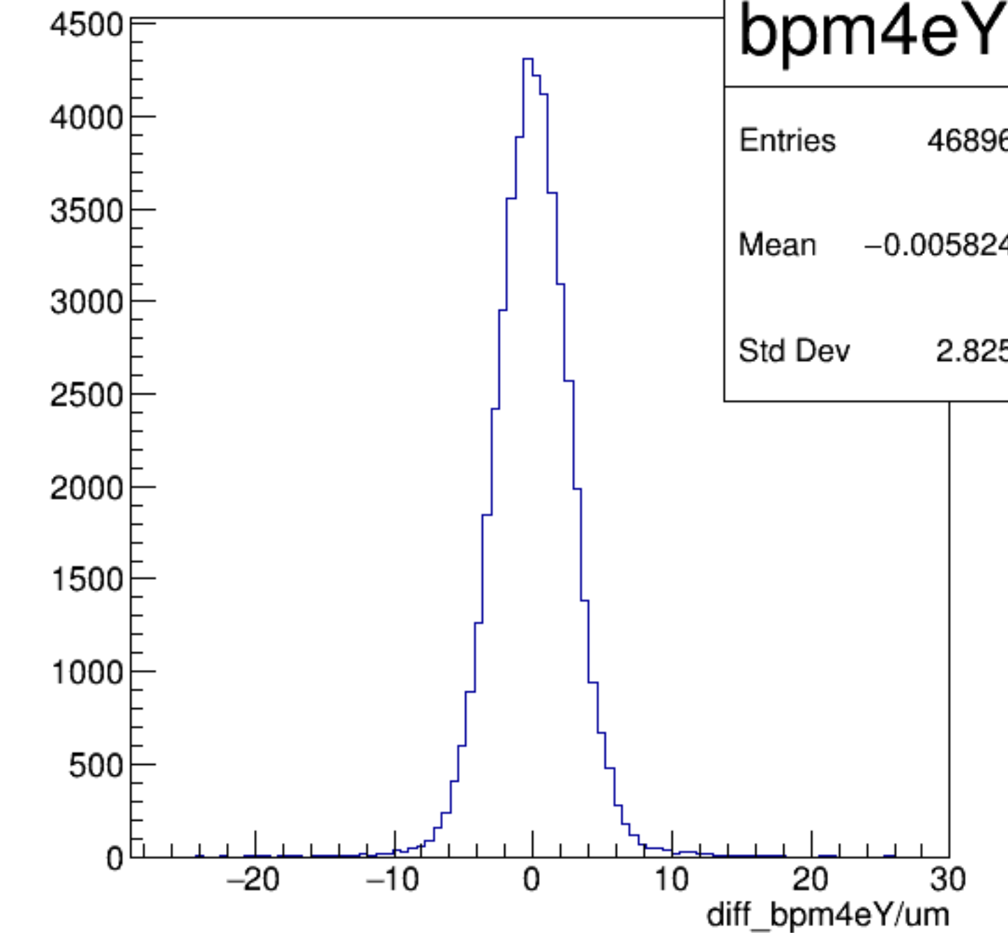
diff_bpm4eY/um {ErrorFlag==0}
