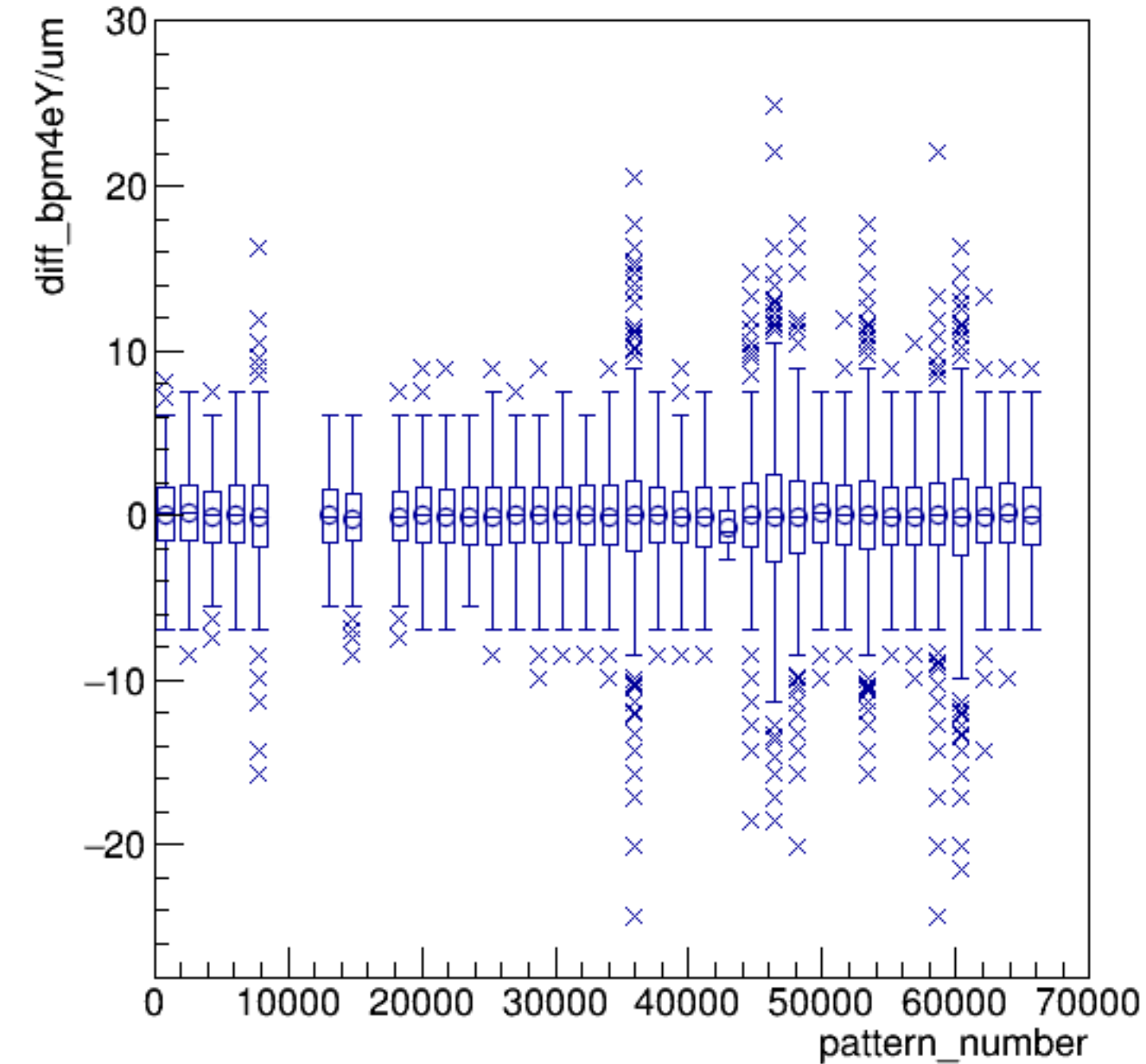
diff_bpm4eY/um:pattern_number {ErrorFlag==0}
