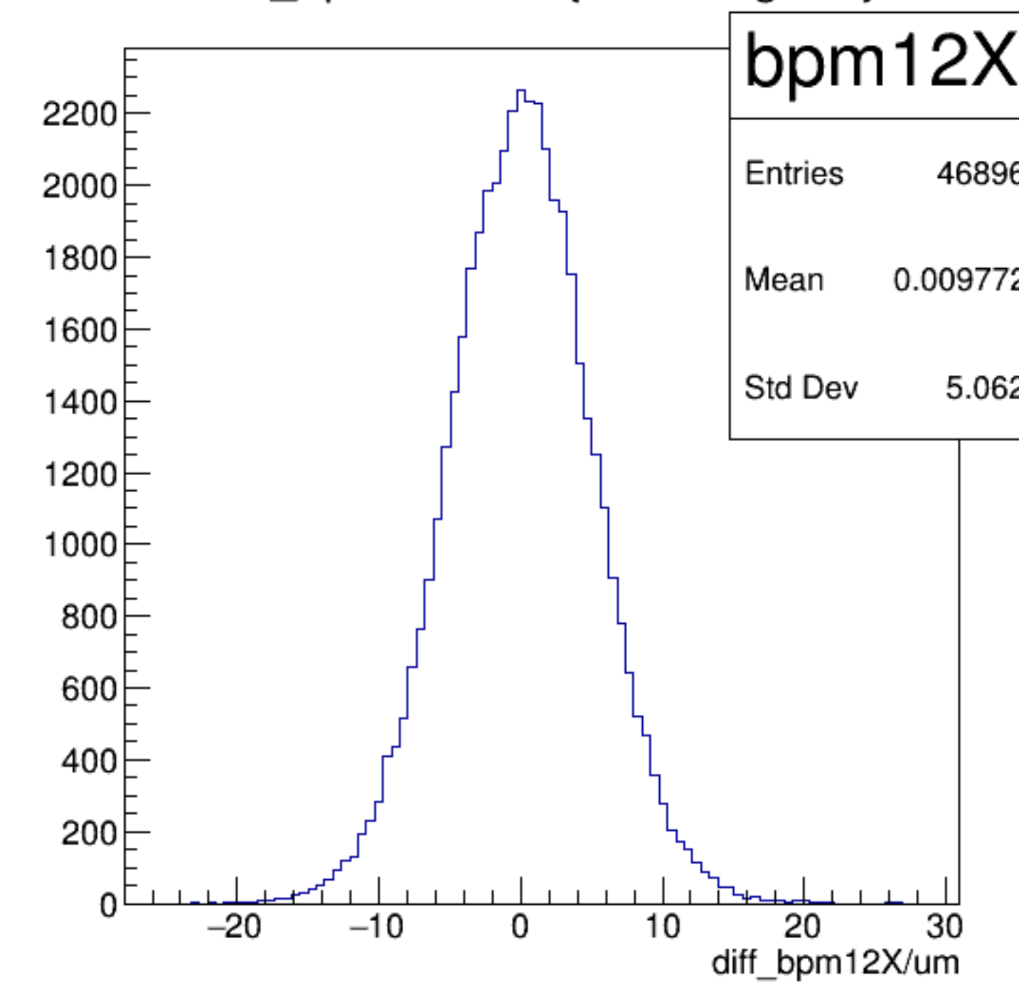
diff_bpm12X/um {ErrorFlag==0}
