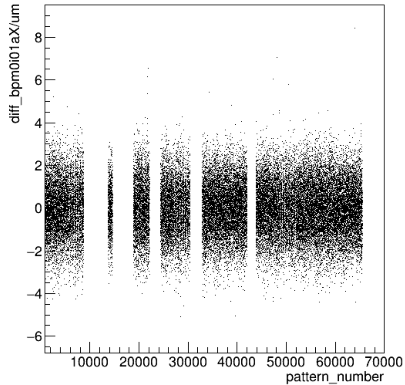
diff_bpm0i01aX/um:pattern_number {ErrorFlag==0}
