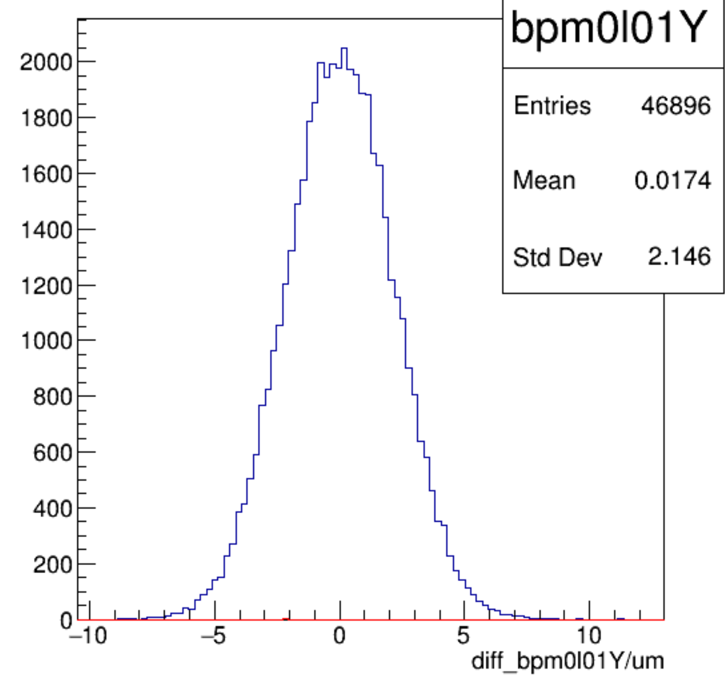
diff_bpm0l01Y/um {ErrorFlag==0}
