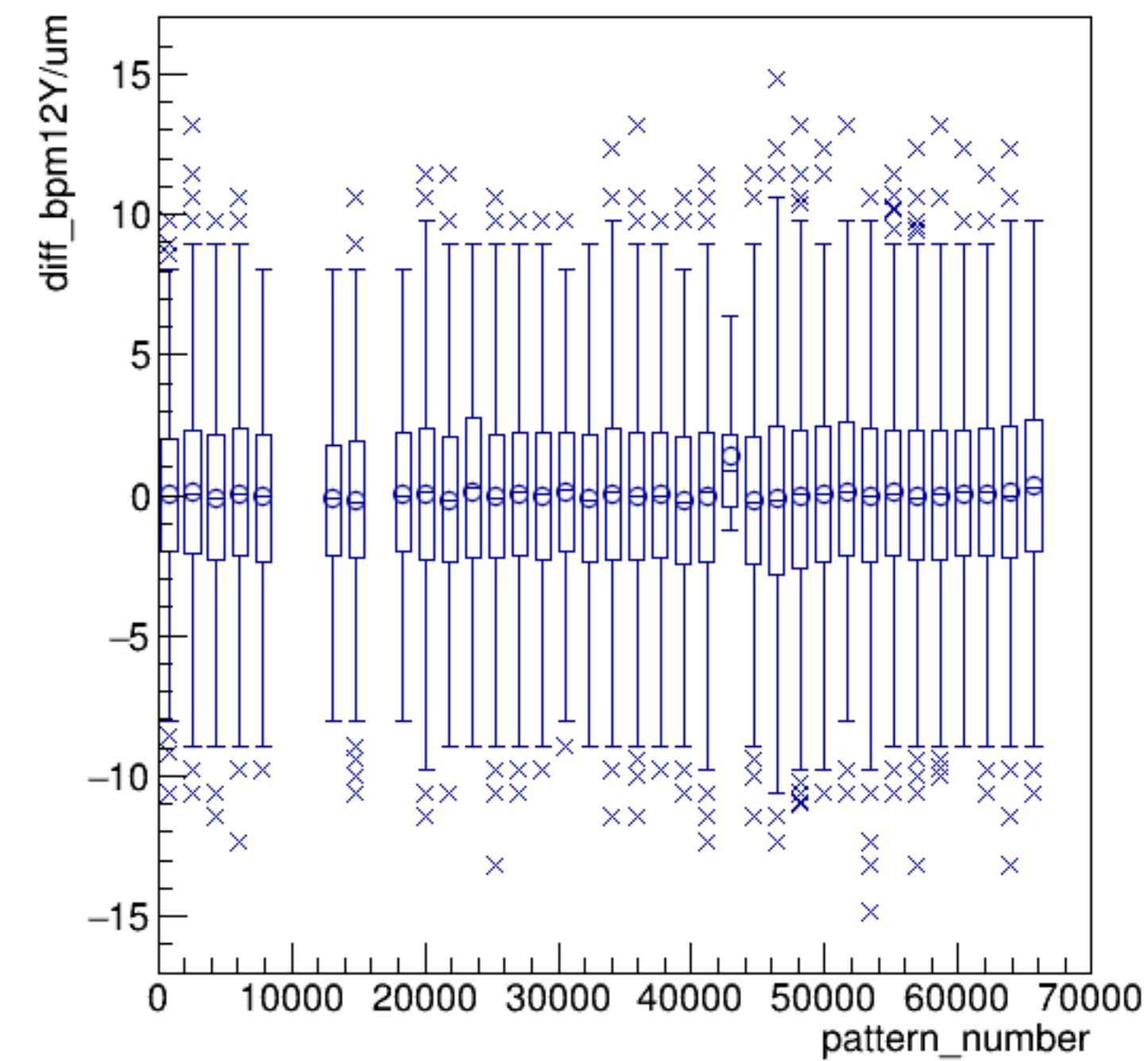
diff_bpm12Y/um:pattern_number {ErrorFlag==0}
