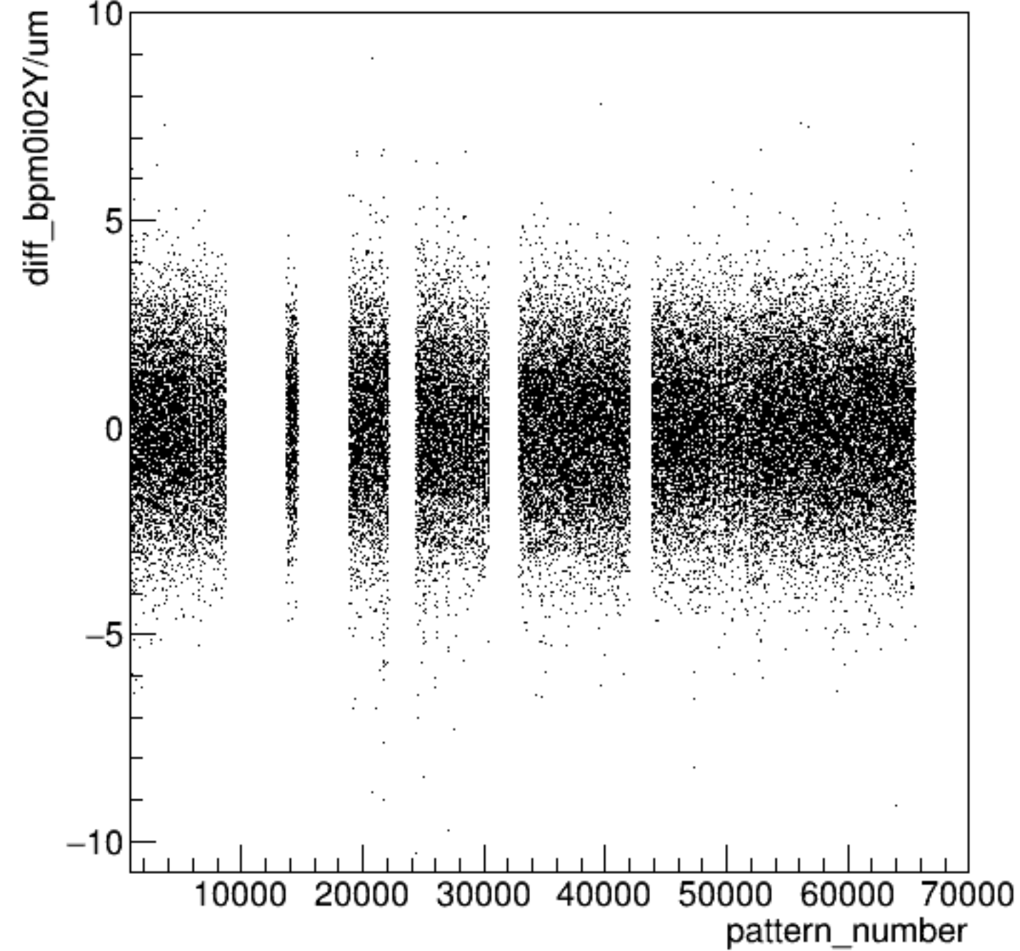
diff_bpm0i02Y/um:pattern_number {ErrorFlag==0}
