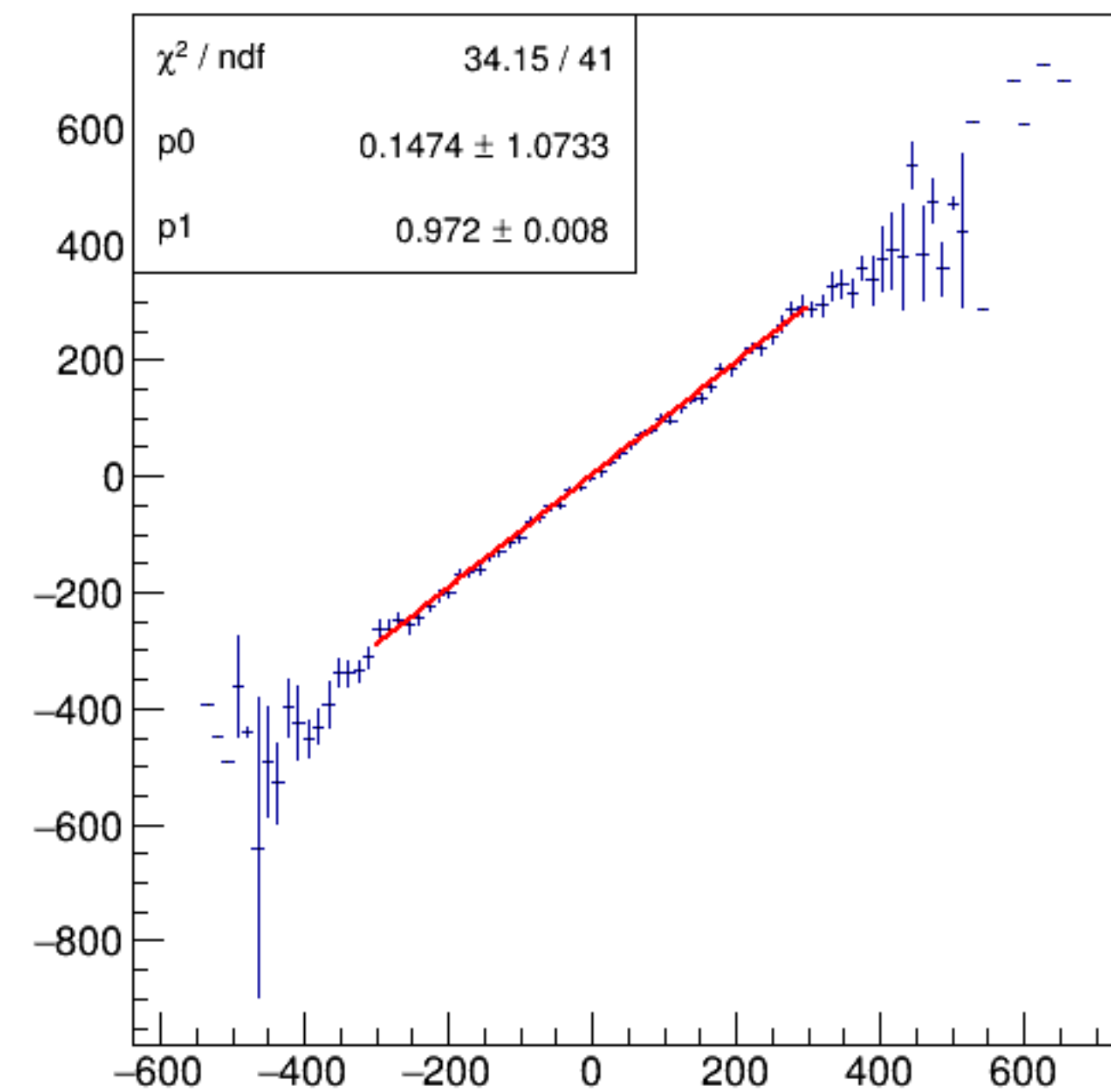
asym_bpm4aWS/ppm:Aq/ppm {ErrorFlag==0}
