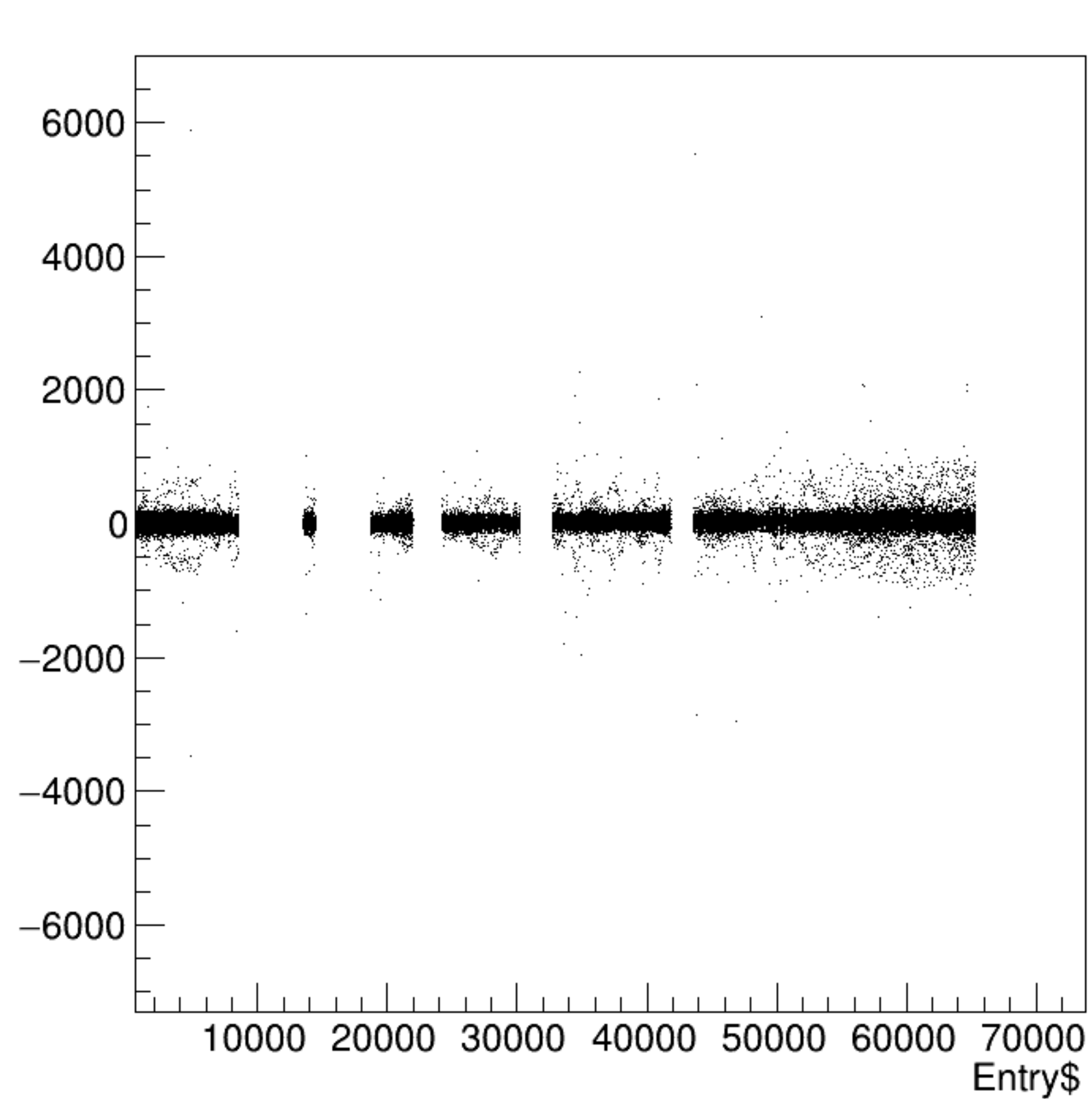
asym_bpm2i01WS/ppm:Entry$ {ErrorFlag==0}
