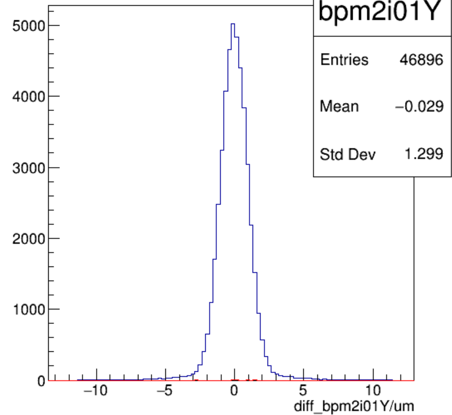
diff_bpm2i01Y/um {ErrorFlag==0}
