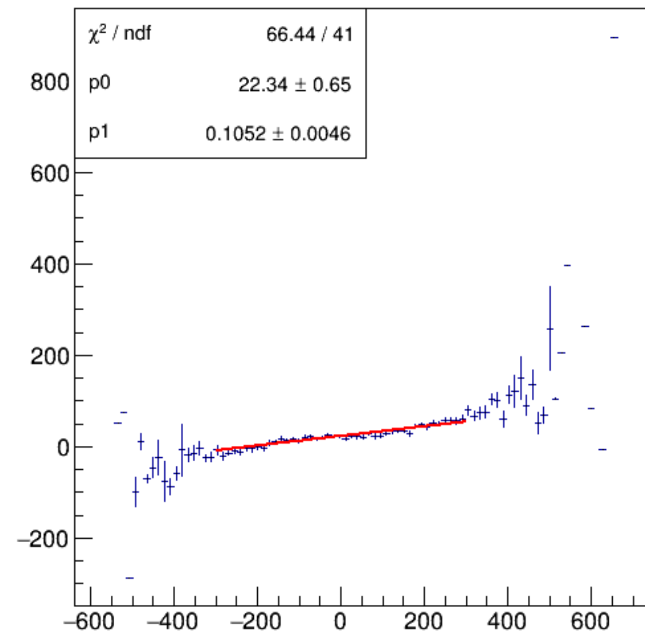
asym_bpm2i01WS/ppm:Aq/ppm {ErrorFlag==0}
