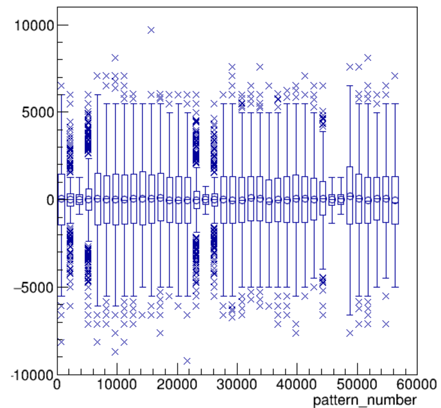
asym_sam1/ppm:pattern_number {ErrorFlag==0}
