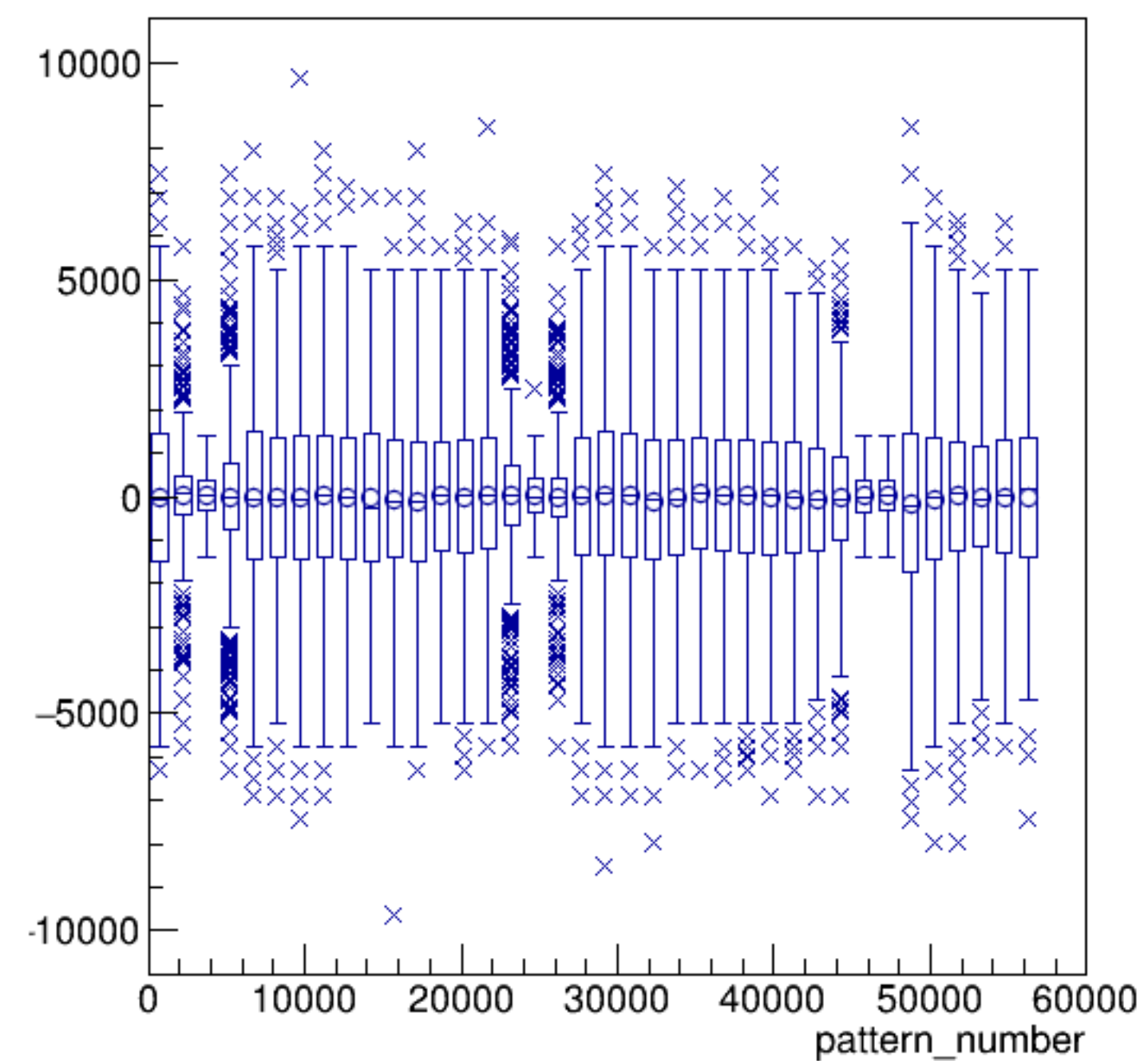
asym_sam5/ppm:pattern_number {ErrorFlag==0}
