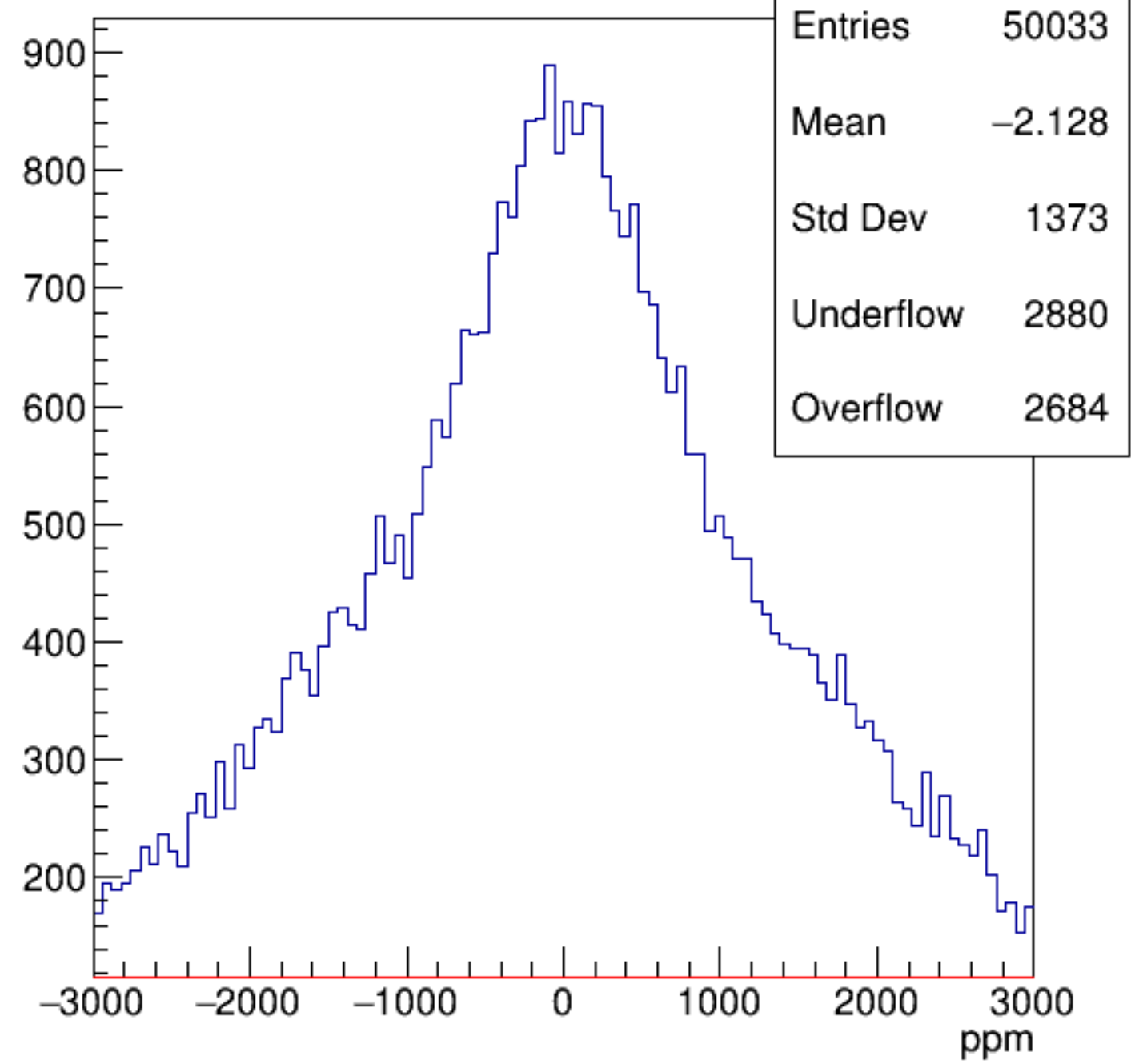
asym_sam5
