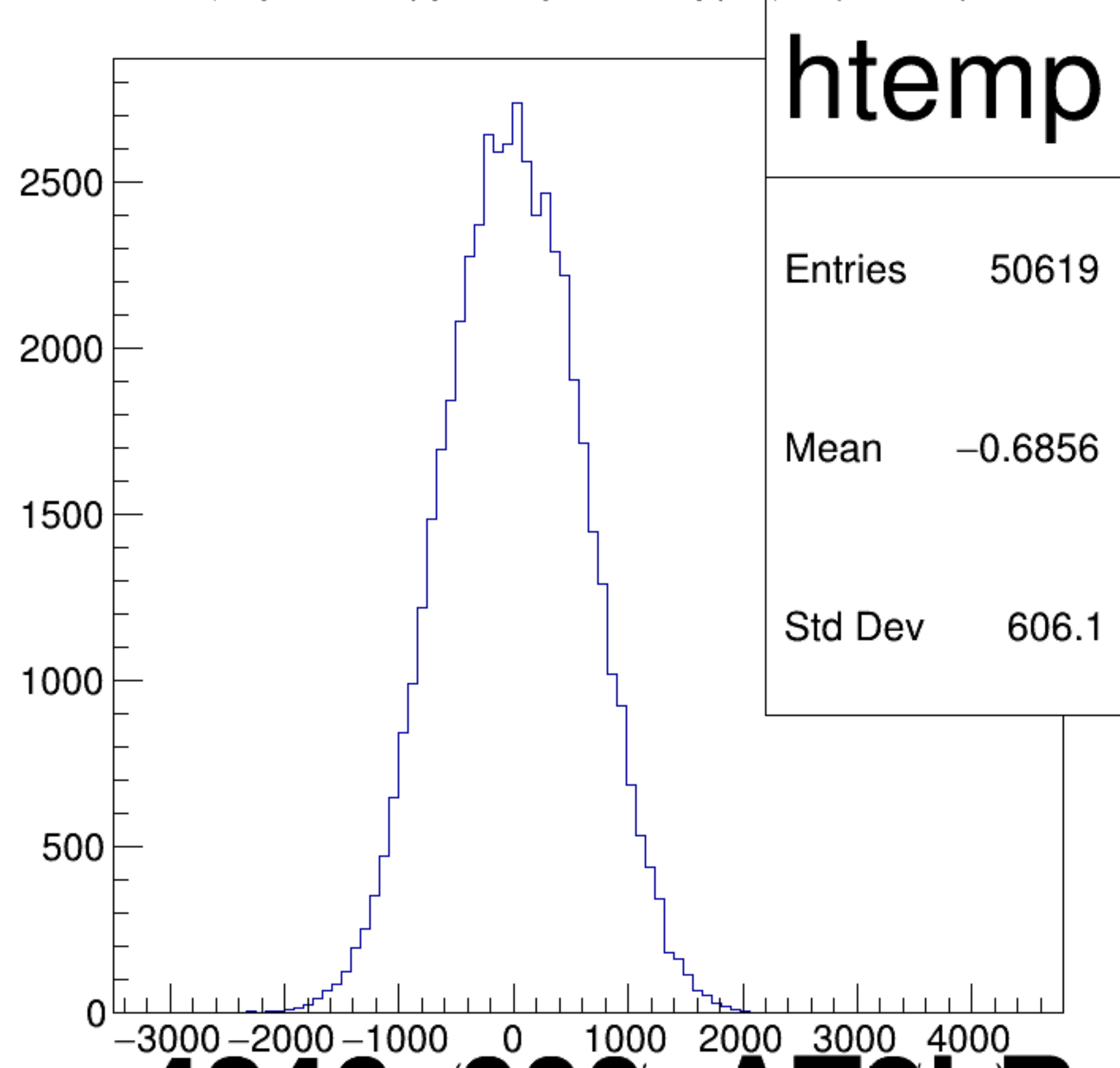
(asym_atl2/ppm-asym_atr2/ppm)/2 {ok_cut}
