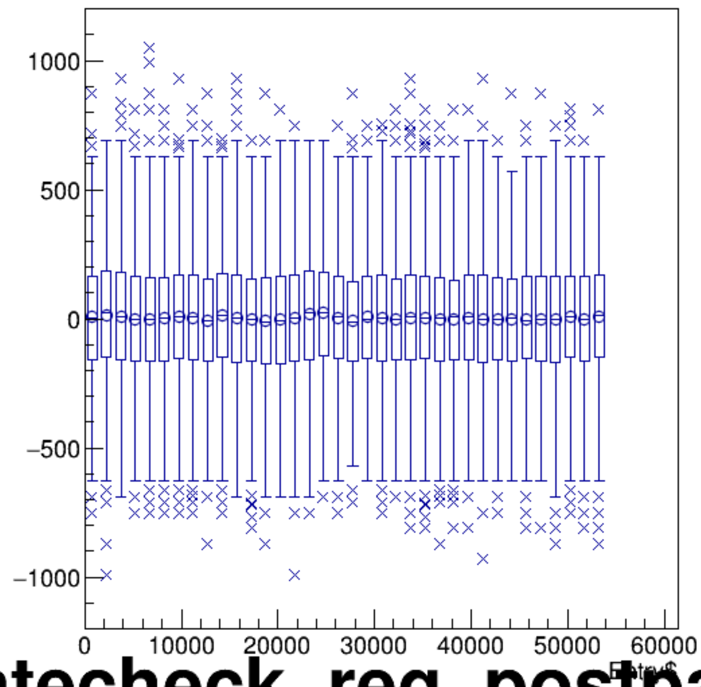
(reg_asym_atl2/ppm-reg_asym_atr2/ppm)/2:Entry$ {ok_cut}
