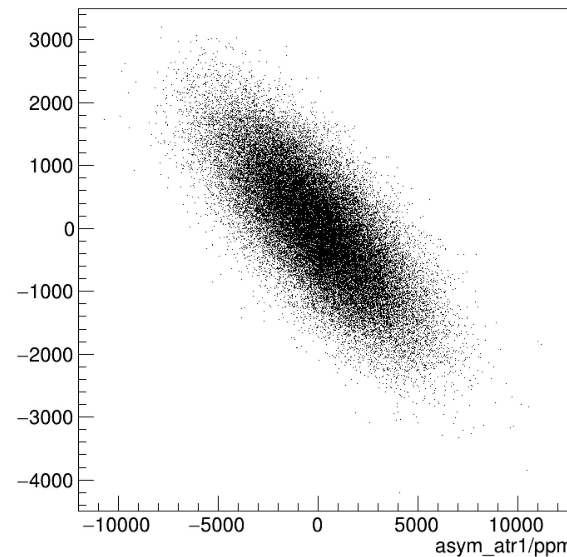
asym_atl1/ppm:asym_atr1/ppm {ok_cut}
