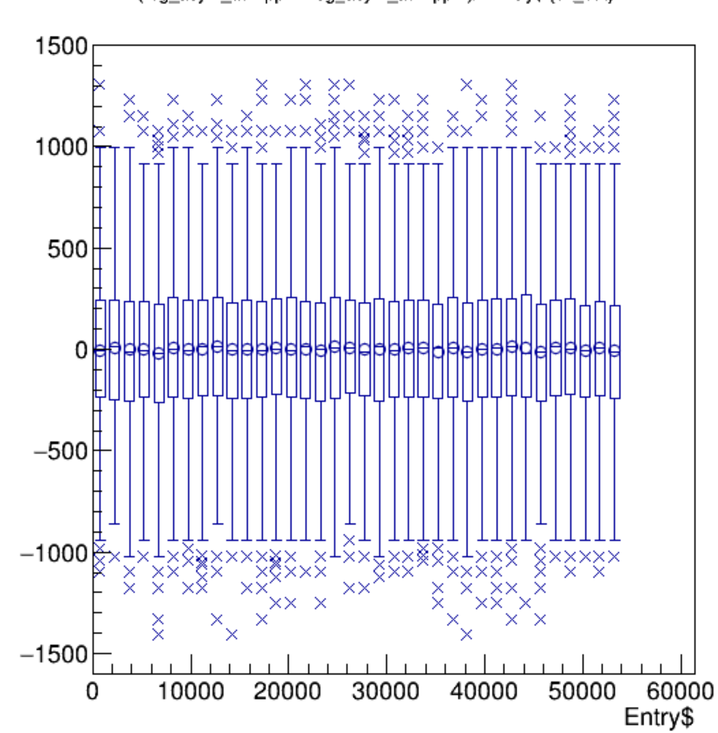
(reg_asym_atl1/ppm+reg_asym_atr1/ppm)/2:Entry$ {ok_cut}
