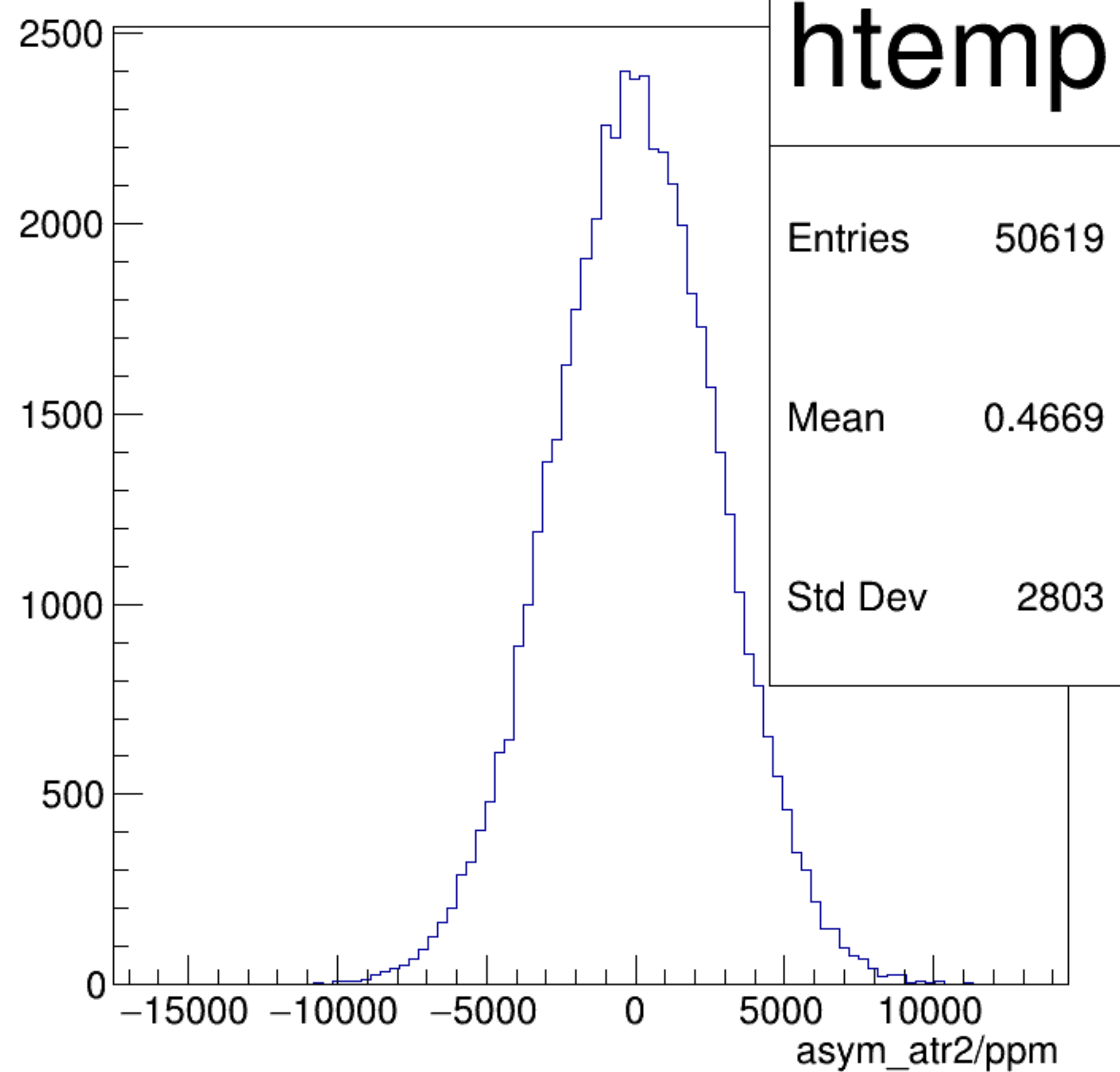
asym_atr2/ppm {ok_cut}
