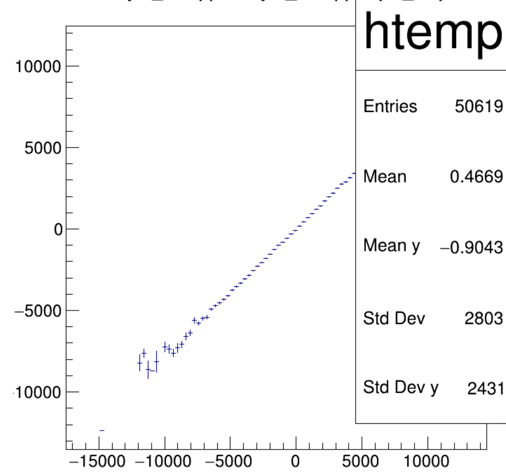
asym_atl2/ppm:asym_atr2/ppm {ok_cut}
