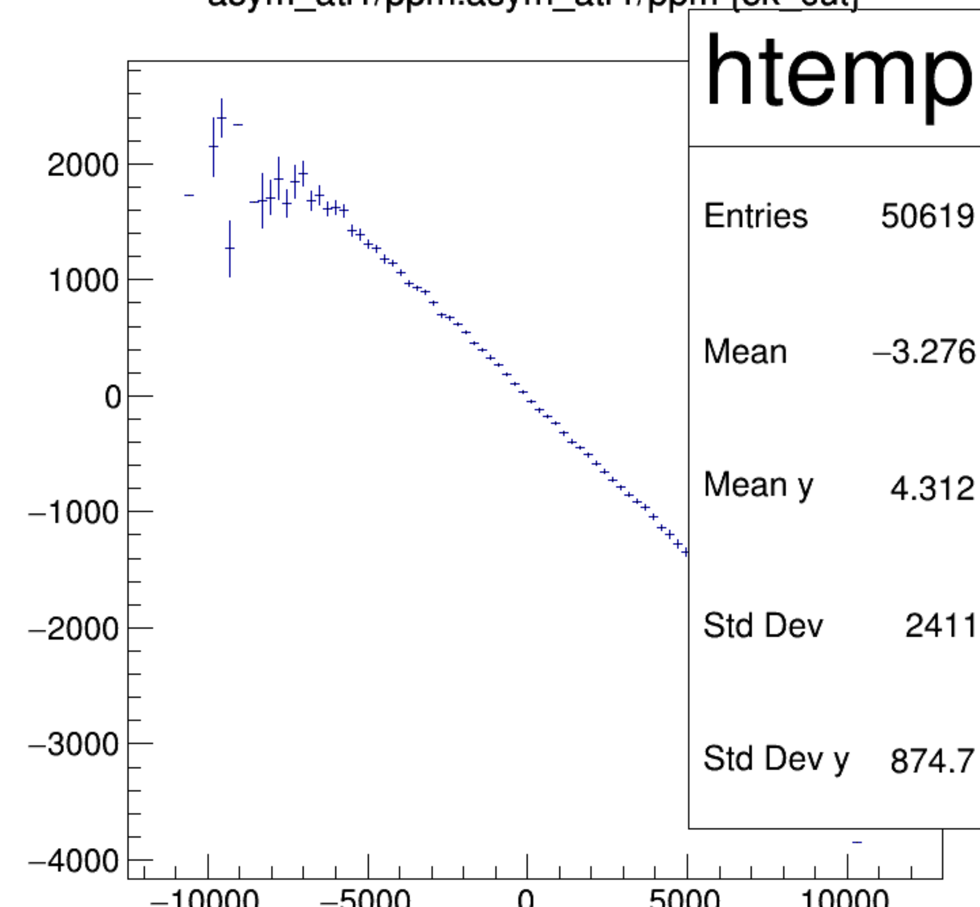
asym_atl1/ppm:asym_atr1/ppm {ok_cut}
