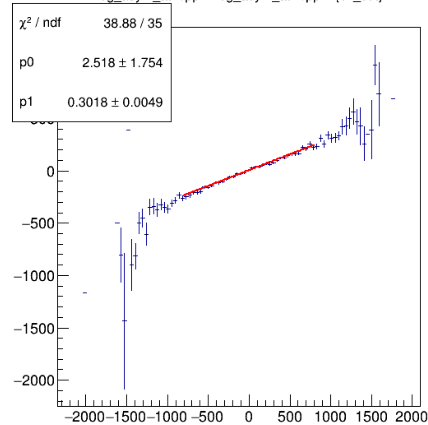
reg_asym_atl2/ppm:reg_asym_atr2/ppm {ok_cut}
