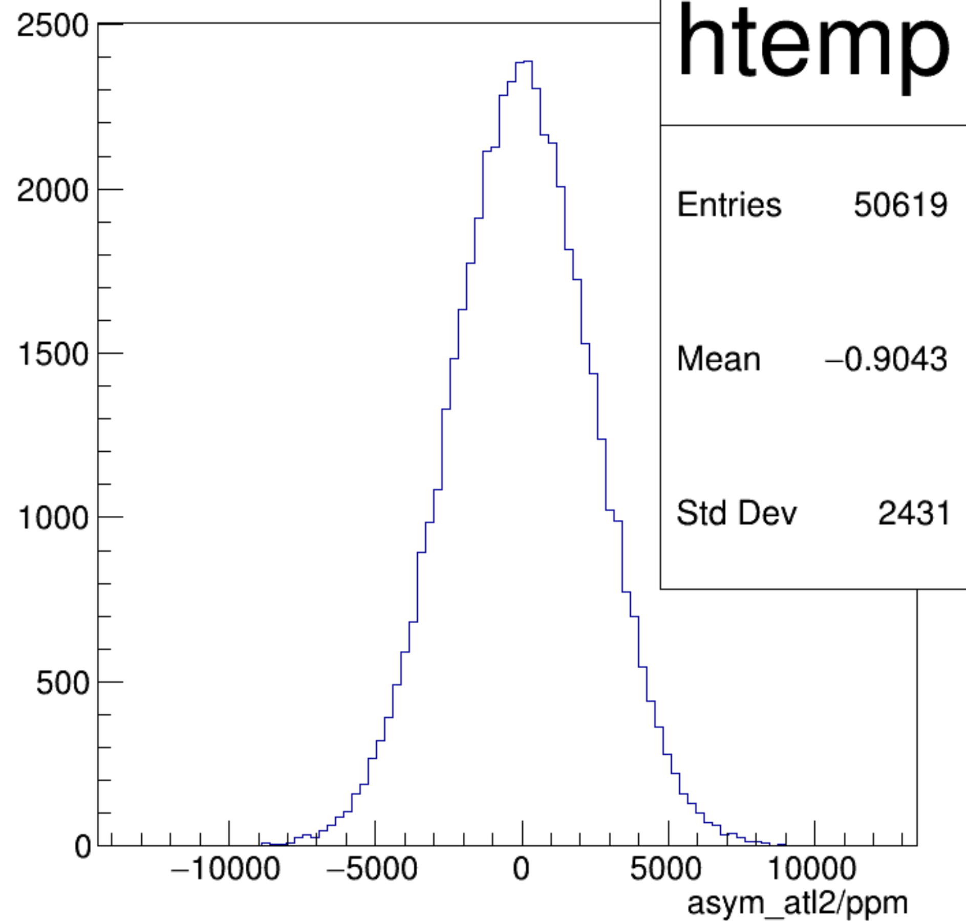
asym_atl2/ppm {ok_cut}
