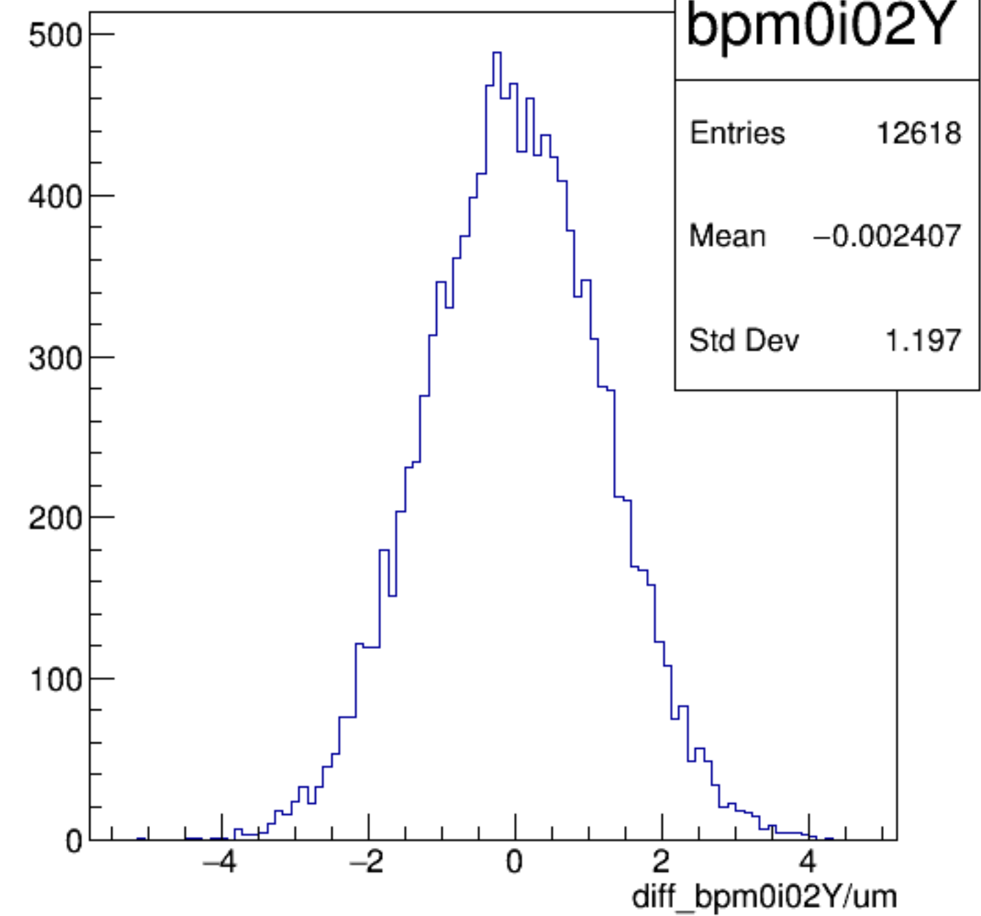
diff_bpm0i02Y/um {ErrorFlag==0}
