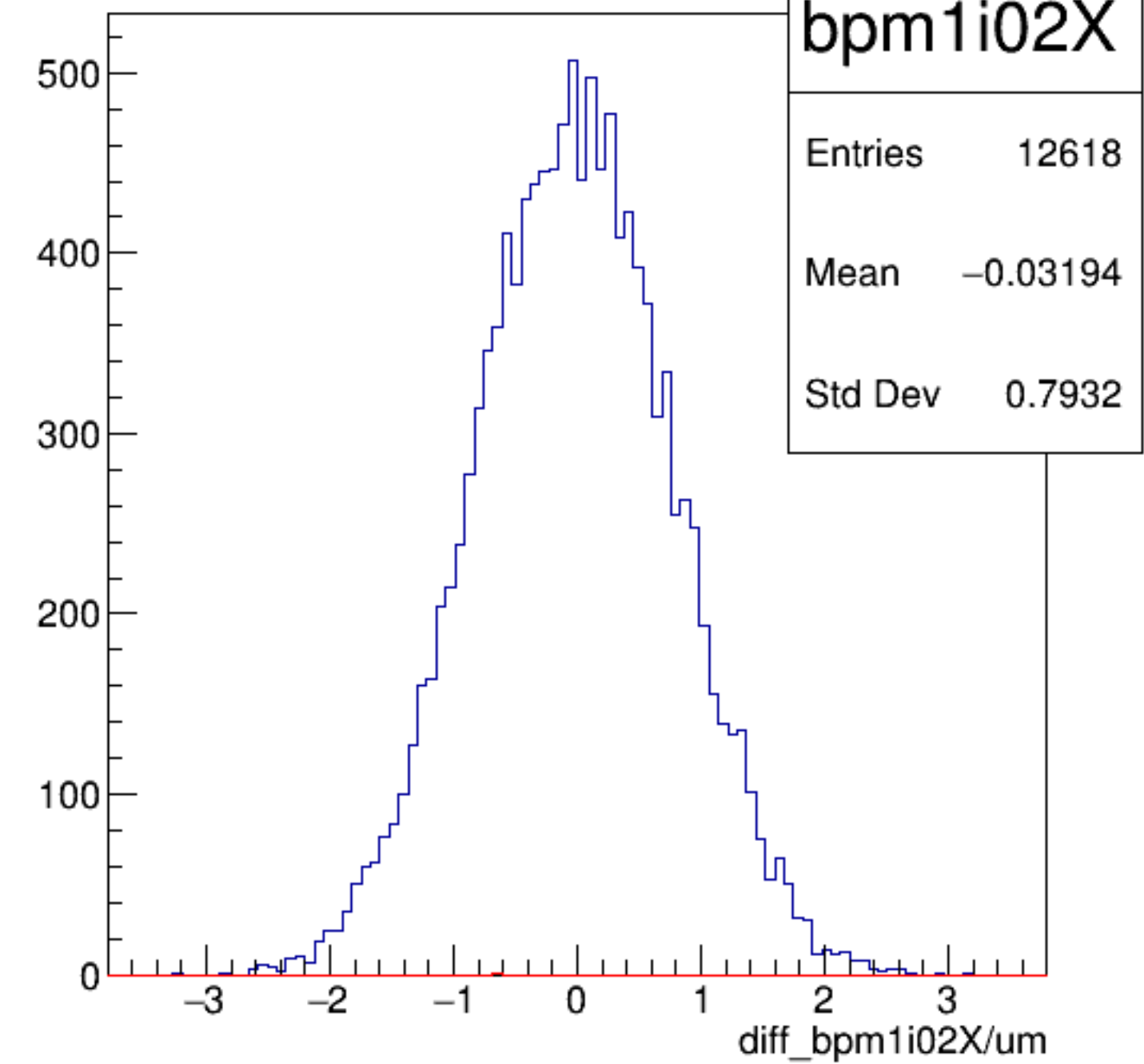
diff_bpm1i02X/um {ErrorFlag==0}
