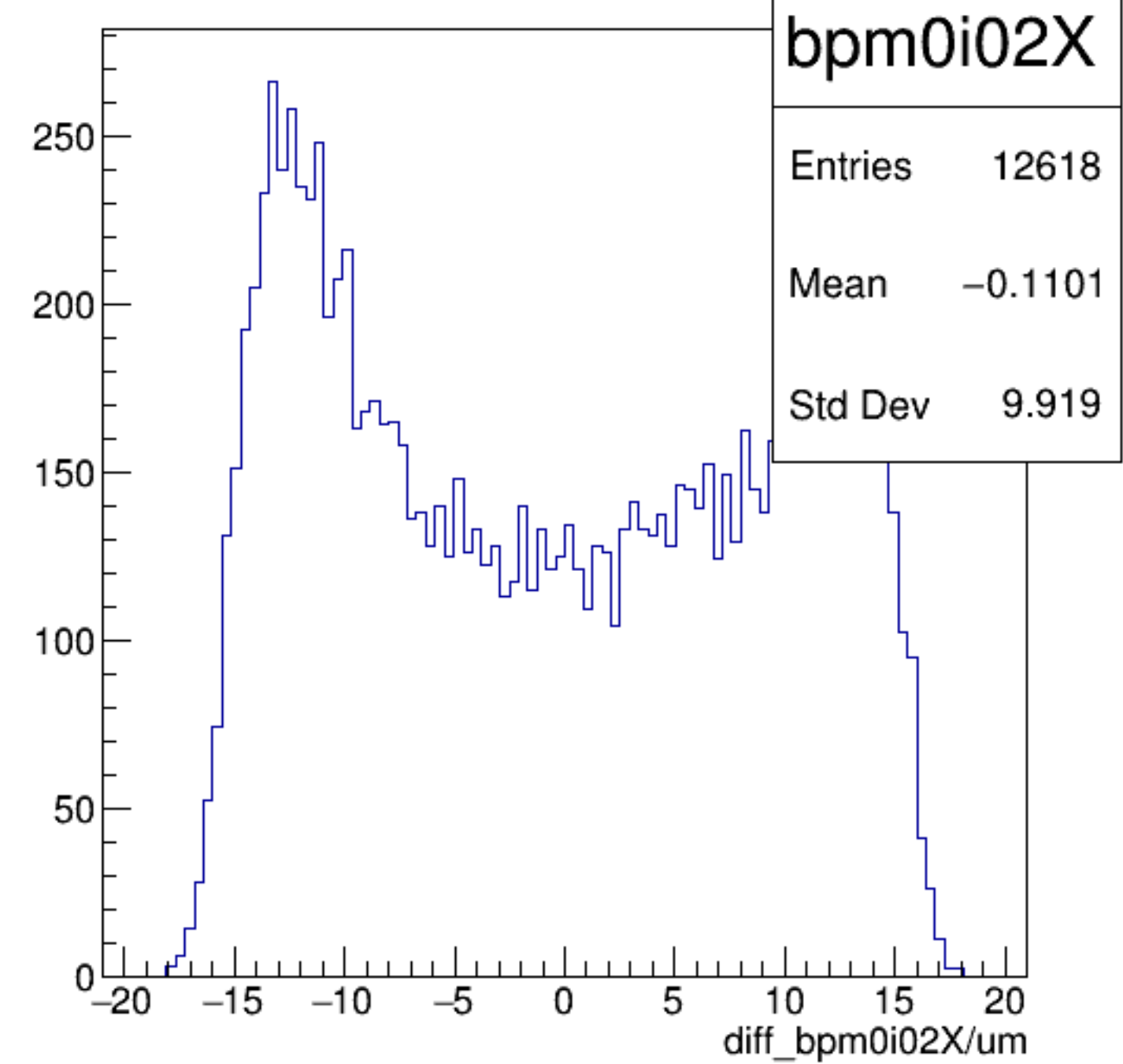
diff_bpm0i02X/um {ErrorFlag==0}
