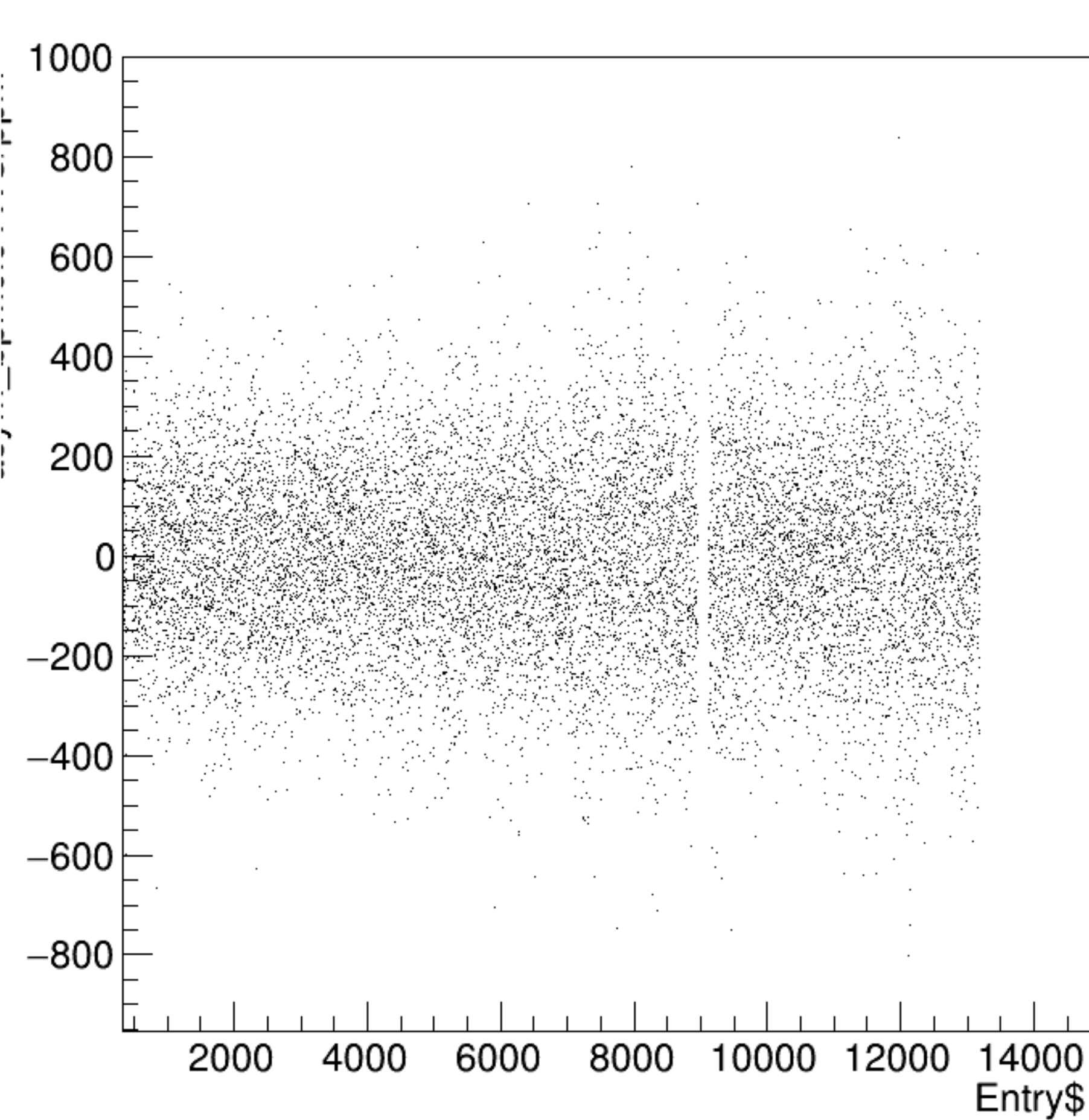
asym_bpm0l01WS/ppm:Entry$ {ErrorFlag==0}
