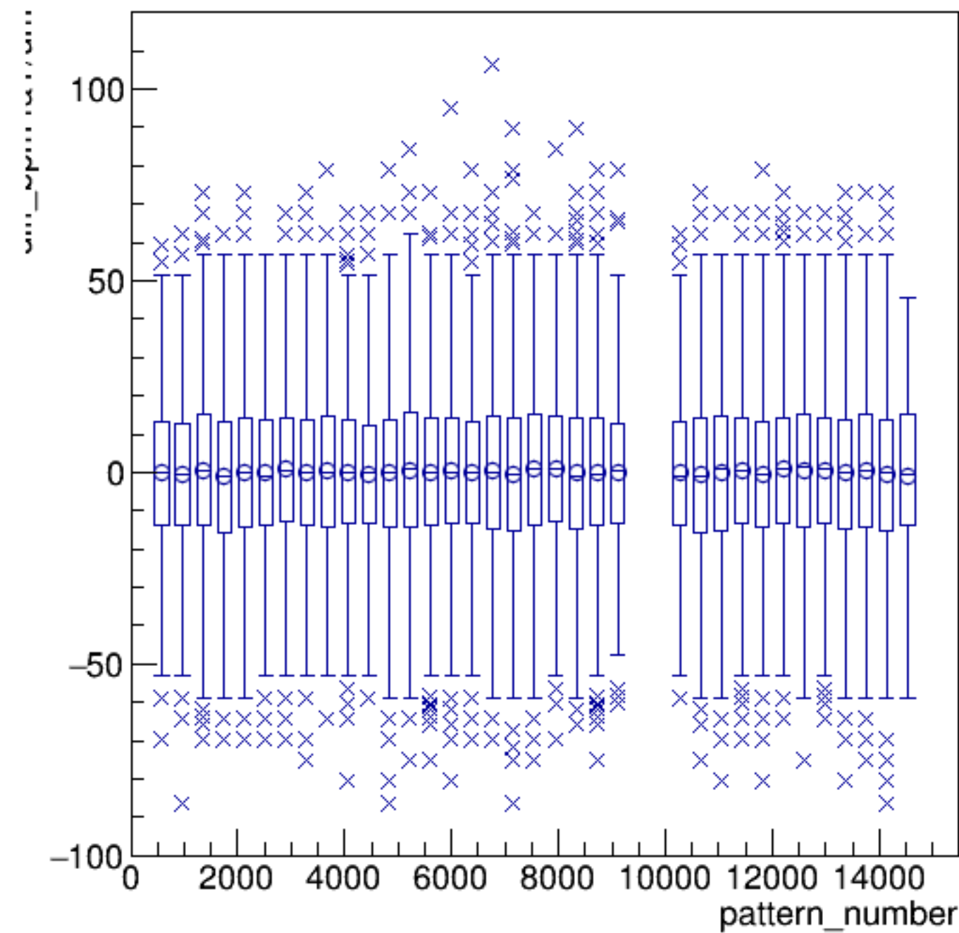
diff_bpm4aY/um:pattern_number {ErrorFlag==0}
