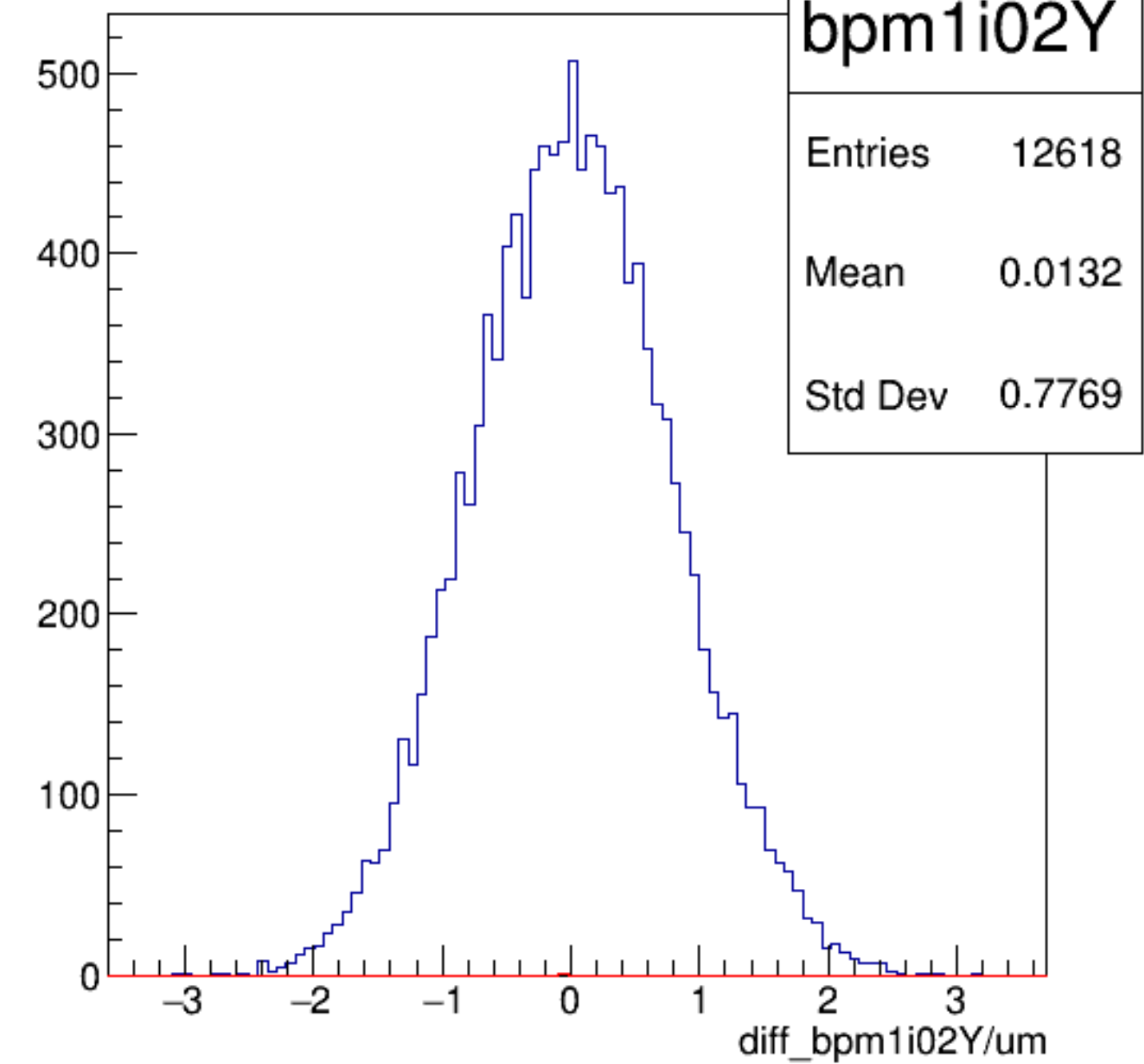
diff_bpm1i02Y/um {ErrorFlag==0}
