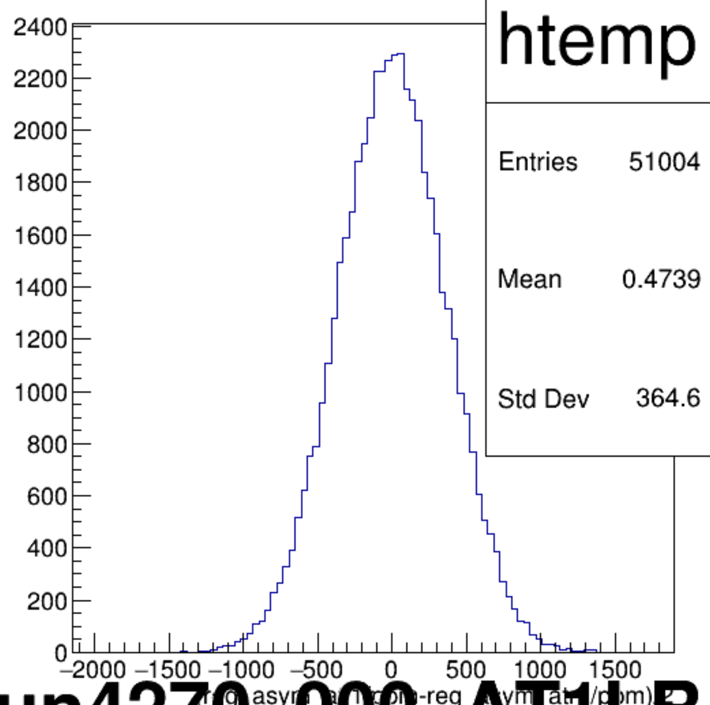
(reg_asym_atl1/ppm-reg_asym_atr1/ppm)/2 {ok_cut}
