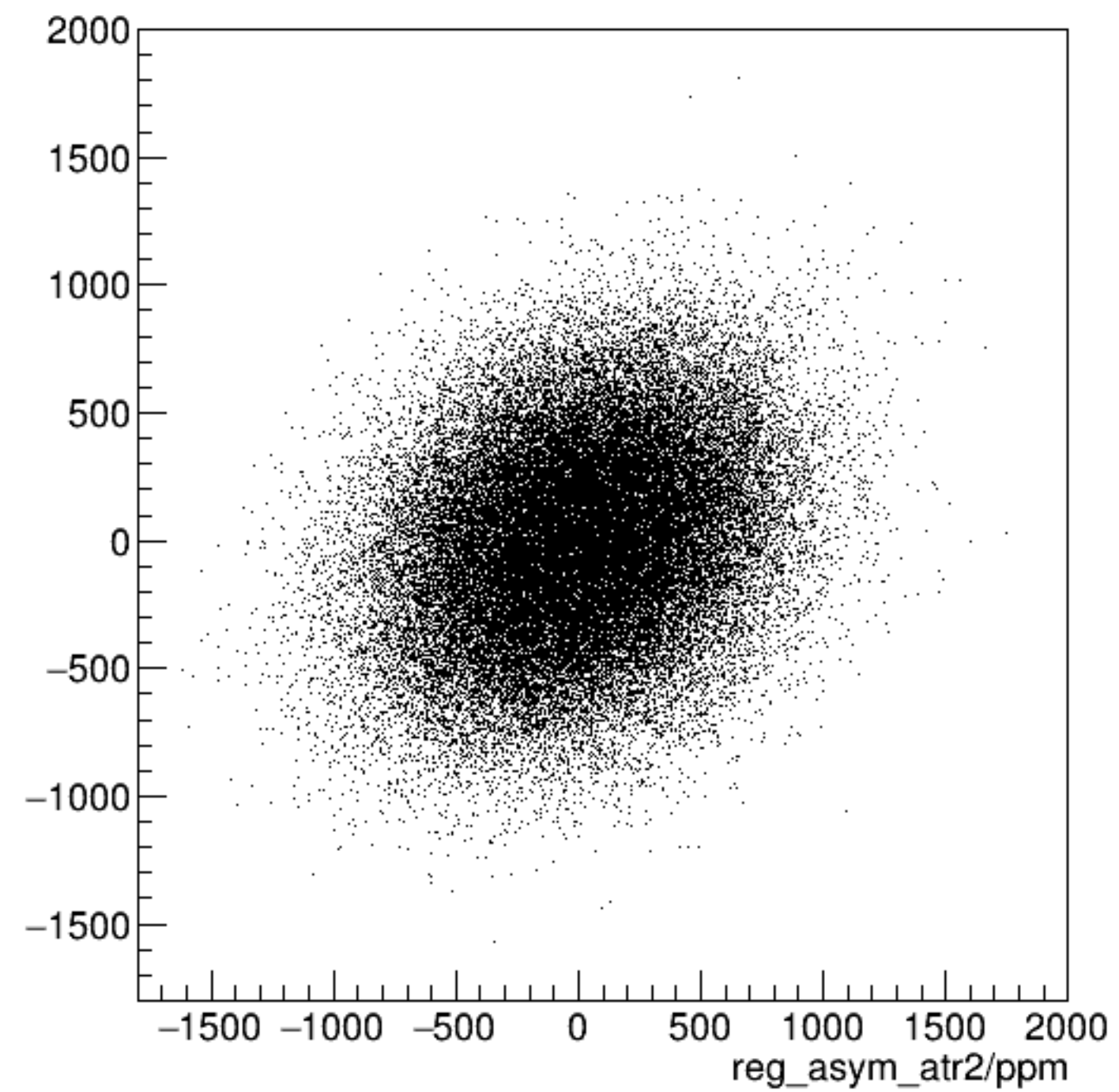
reg_asym_atl2/ppm:reg_asym_atr2/ppm {ok_cut}
