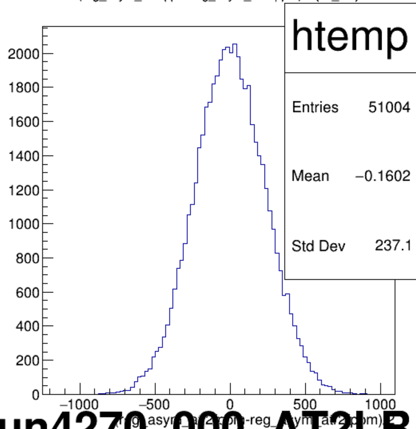
(reg_asym_atl2/ppm-reg_asym_atr2/ppm)/2 {ok_cut}
