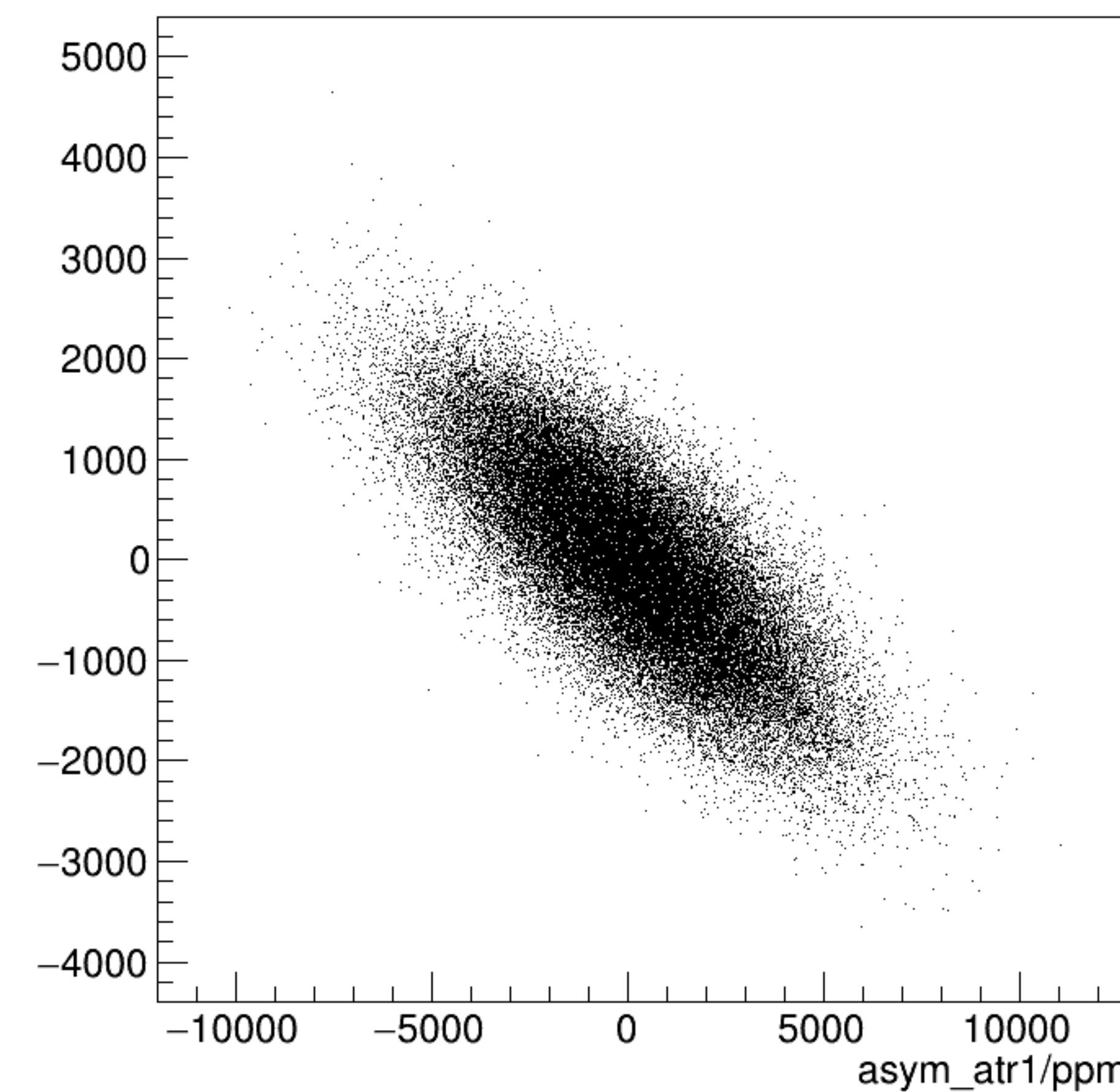
asym_atl1/ppm:asym_atr1/ppm {ok_cut}
