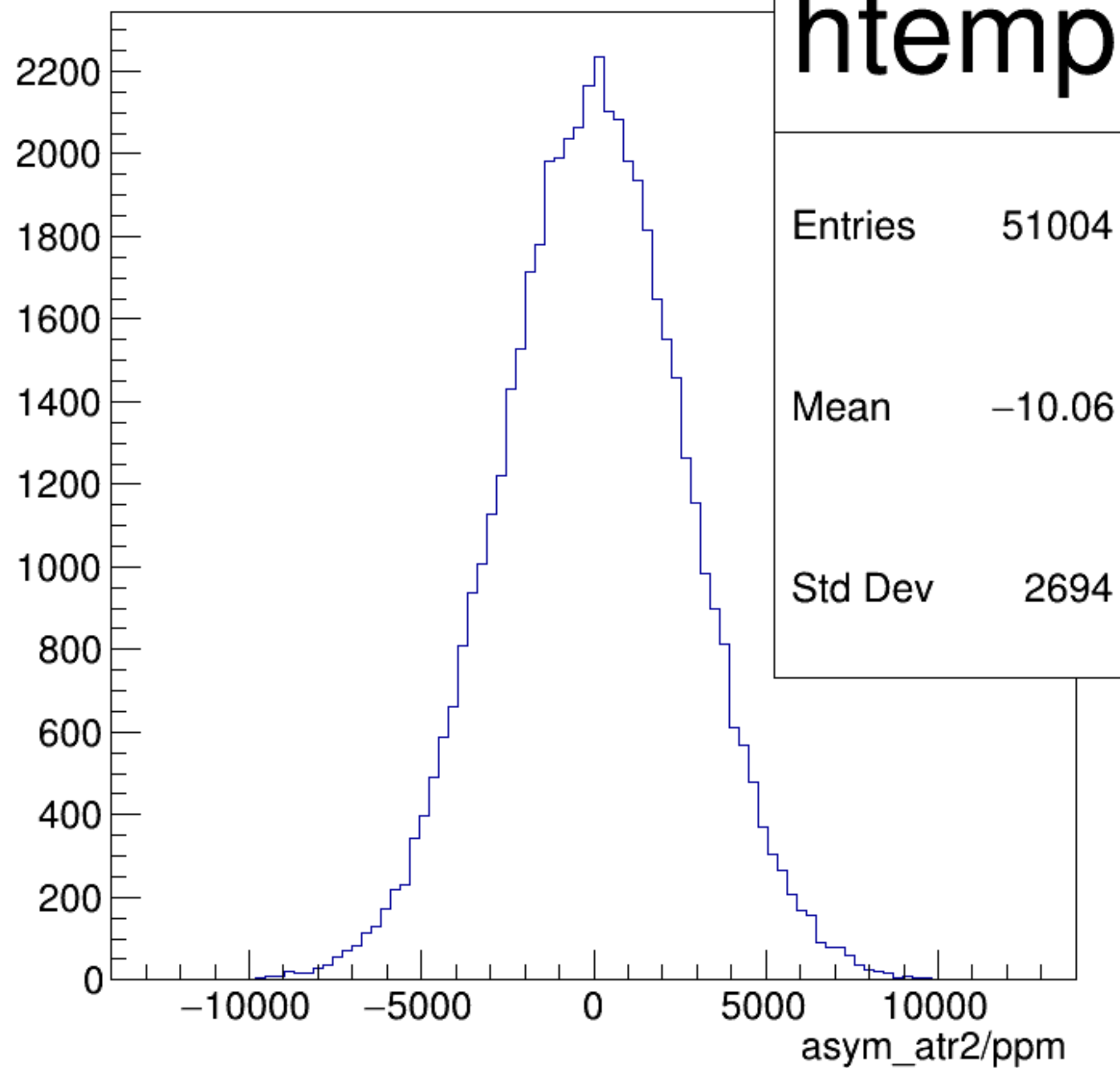
asym_atr2/ppm {ok_cut}
