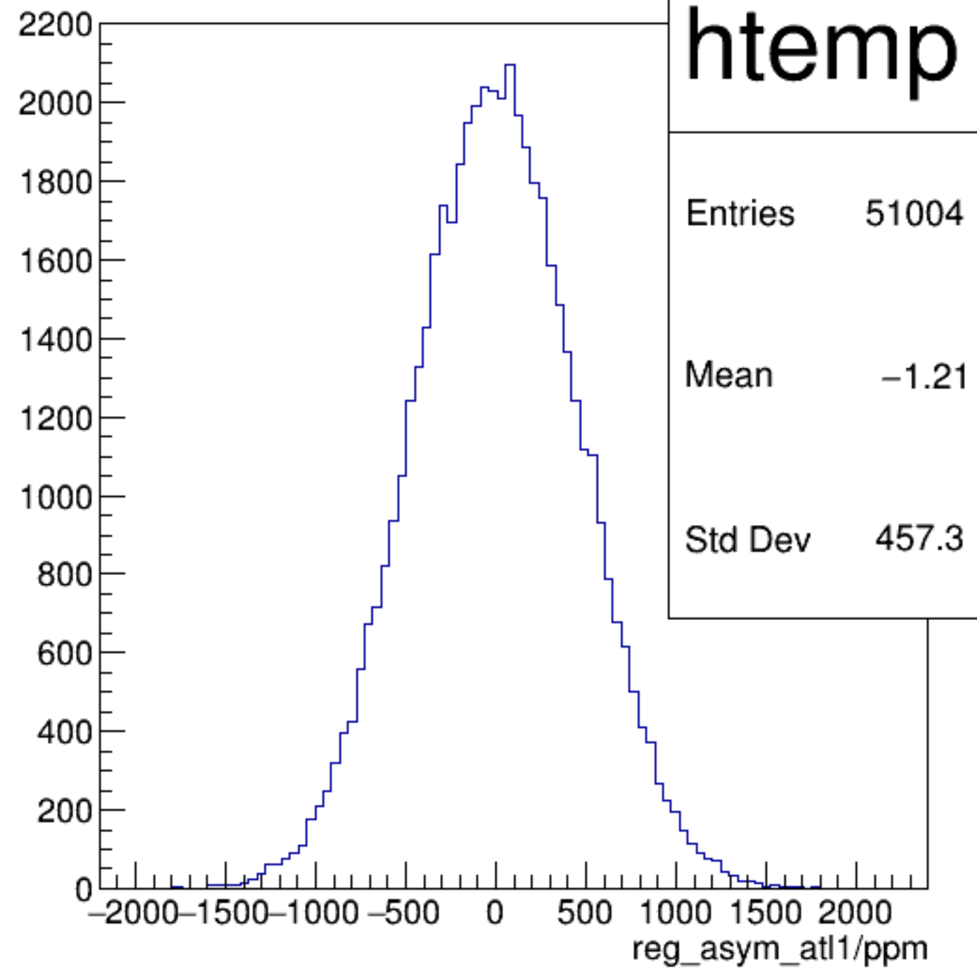
reg_asym_atl1/ppm {ok_cut}
