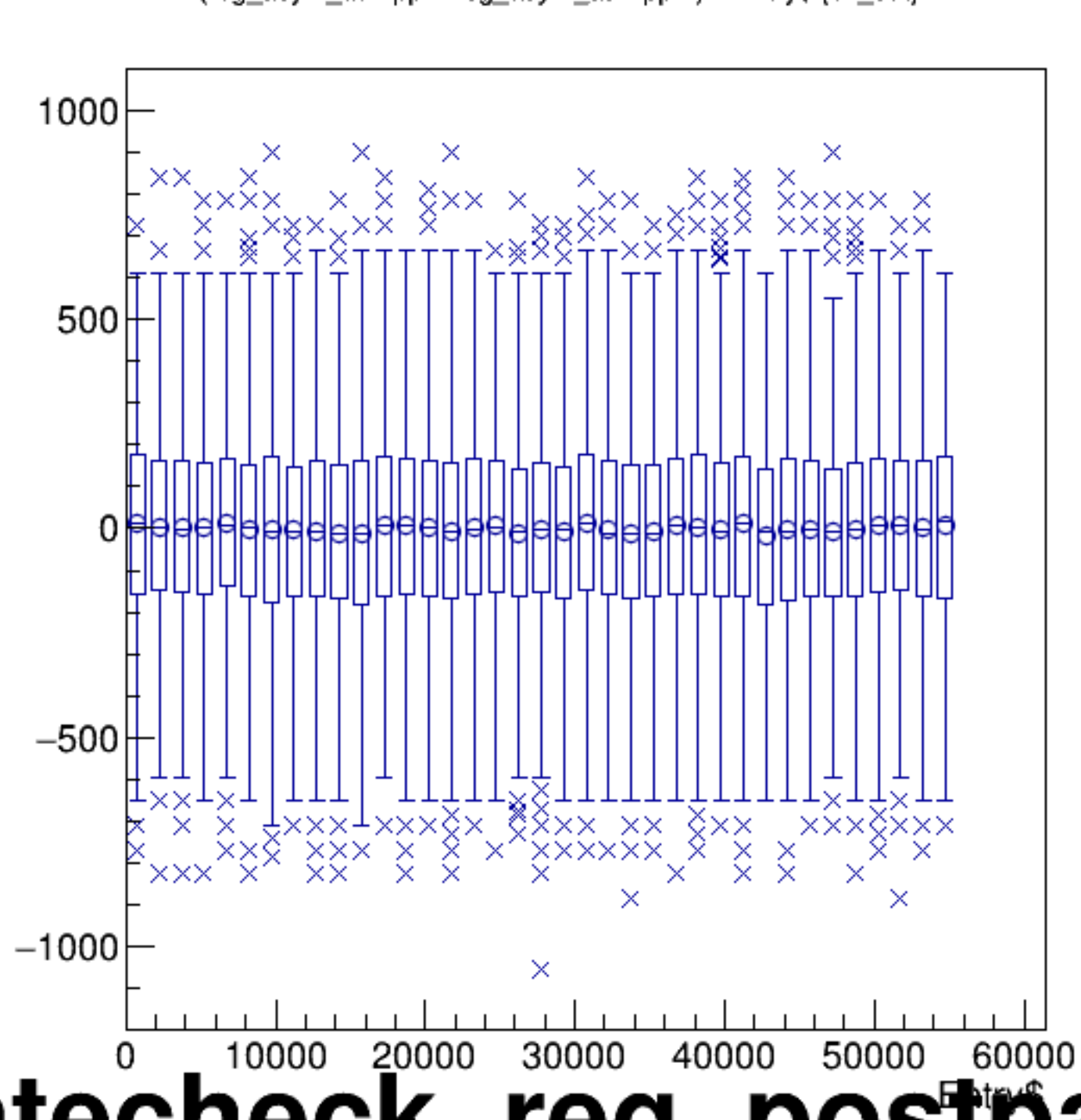
(reg_asym_atl2/ppm-reg_asym_atr2/ppm)/2:Entry$ {ok_cut}
