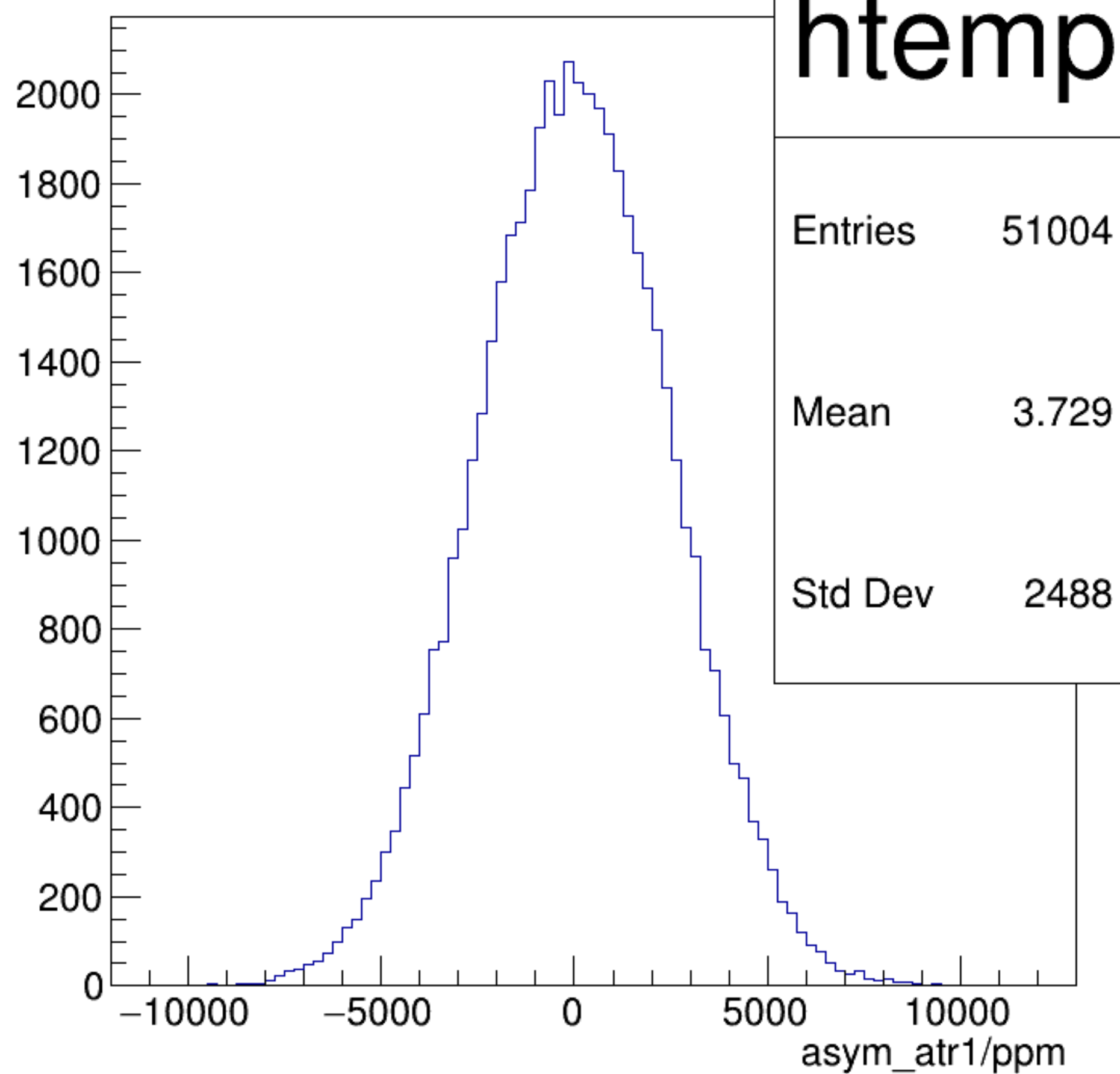
asym_atr1/ppm {ok_cut}
