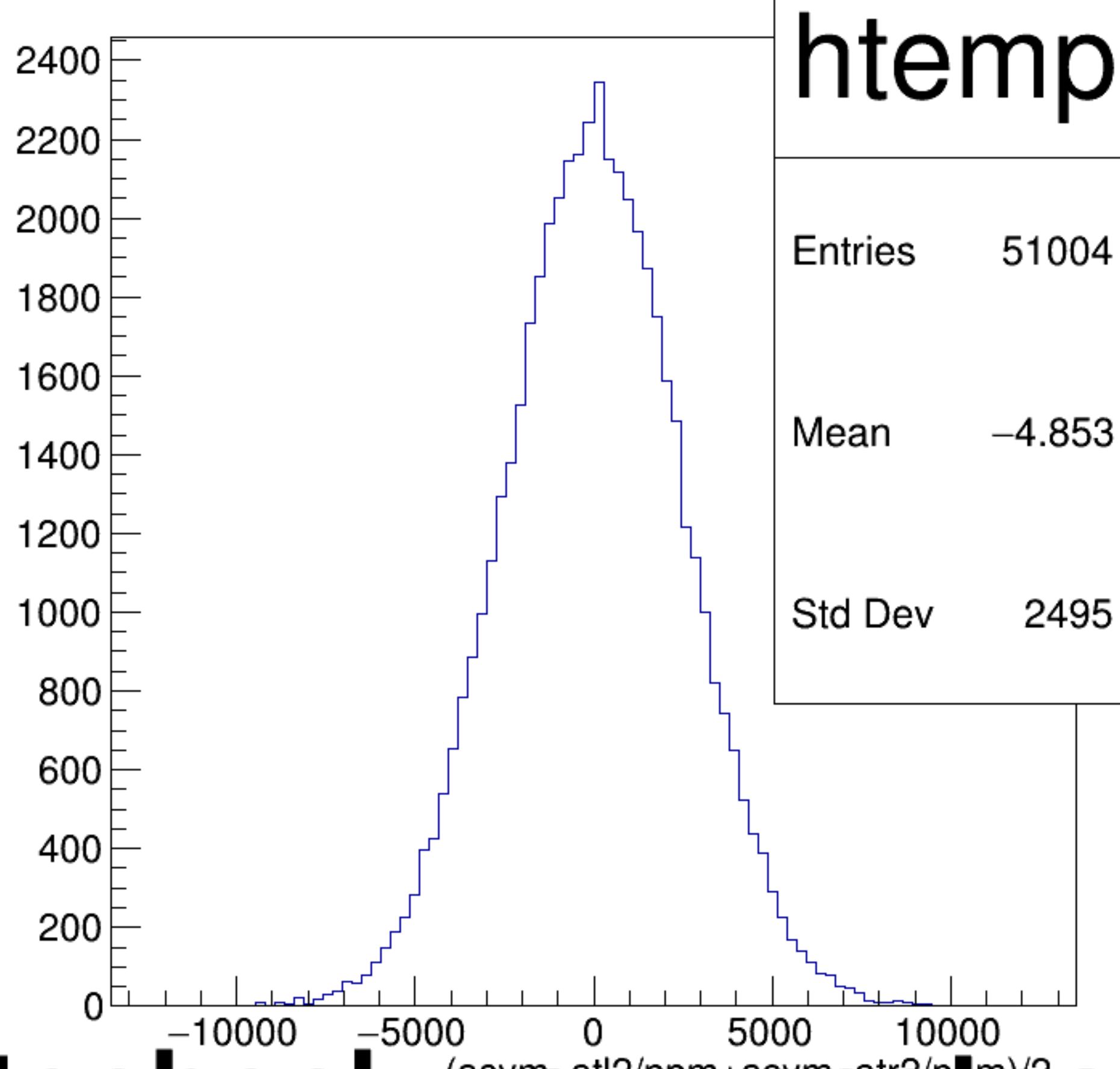
(asym_atl2/ppm+asym_atr2/ppm)/2 {ok_cut}
