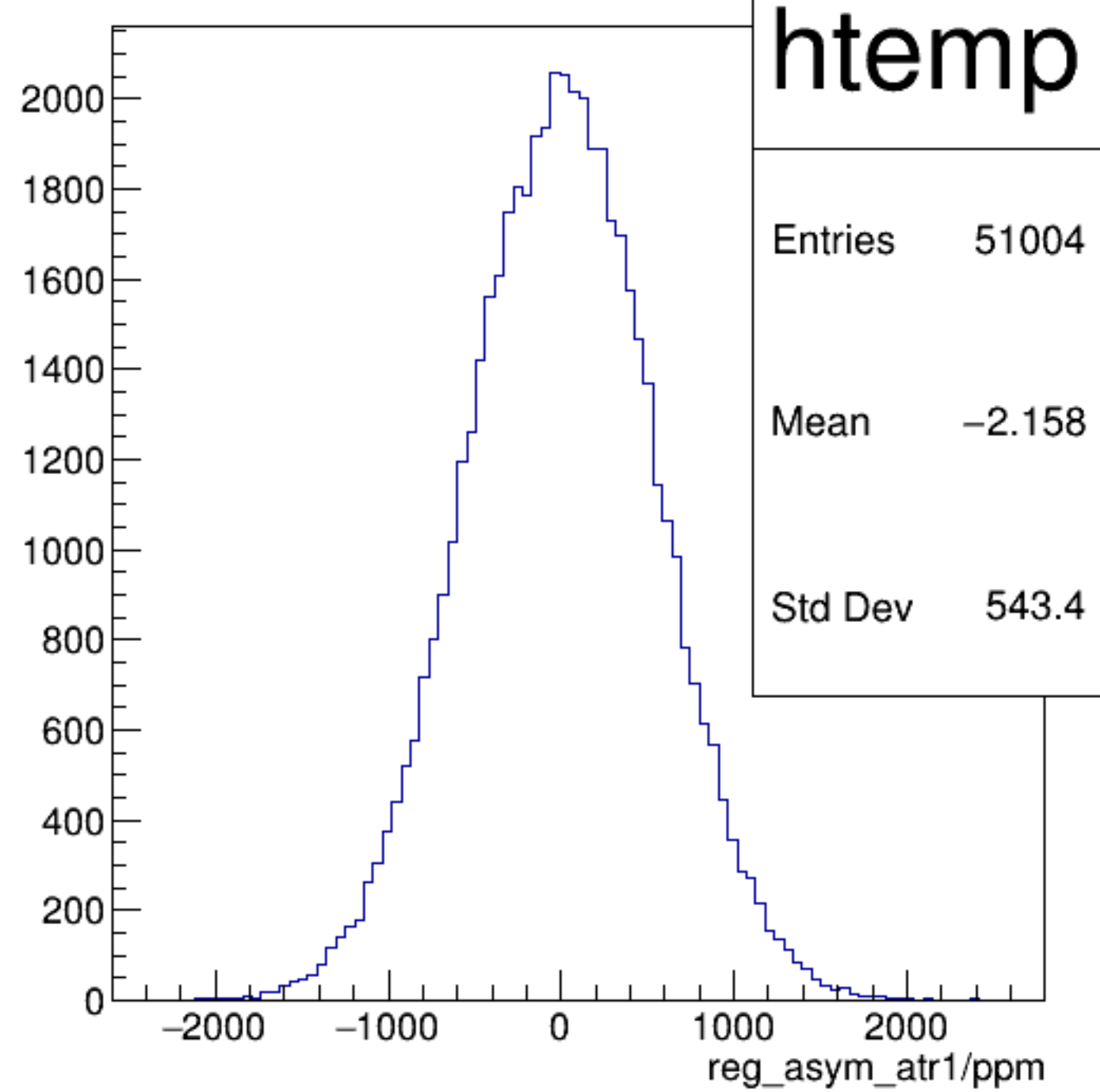
reg_asym_atr1/ppm {ok_cut}
