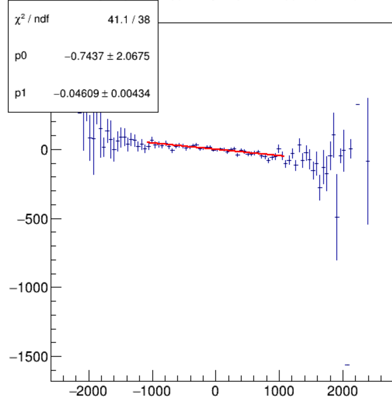
reg_asym_atl1/ppm:reg_asym_atr1/ppm {ok_cut}
