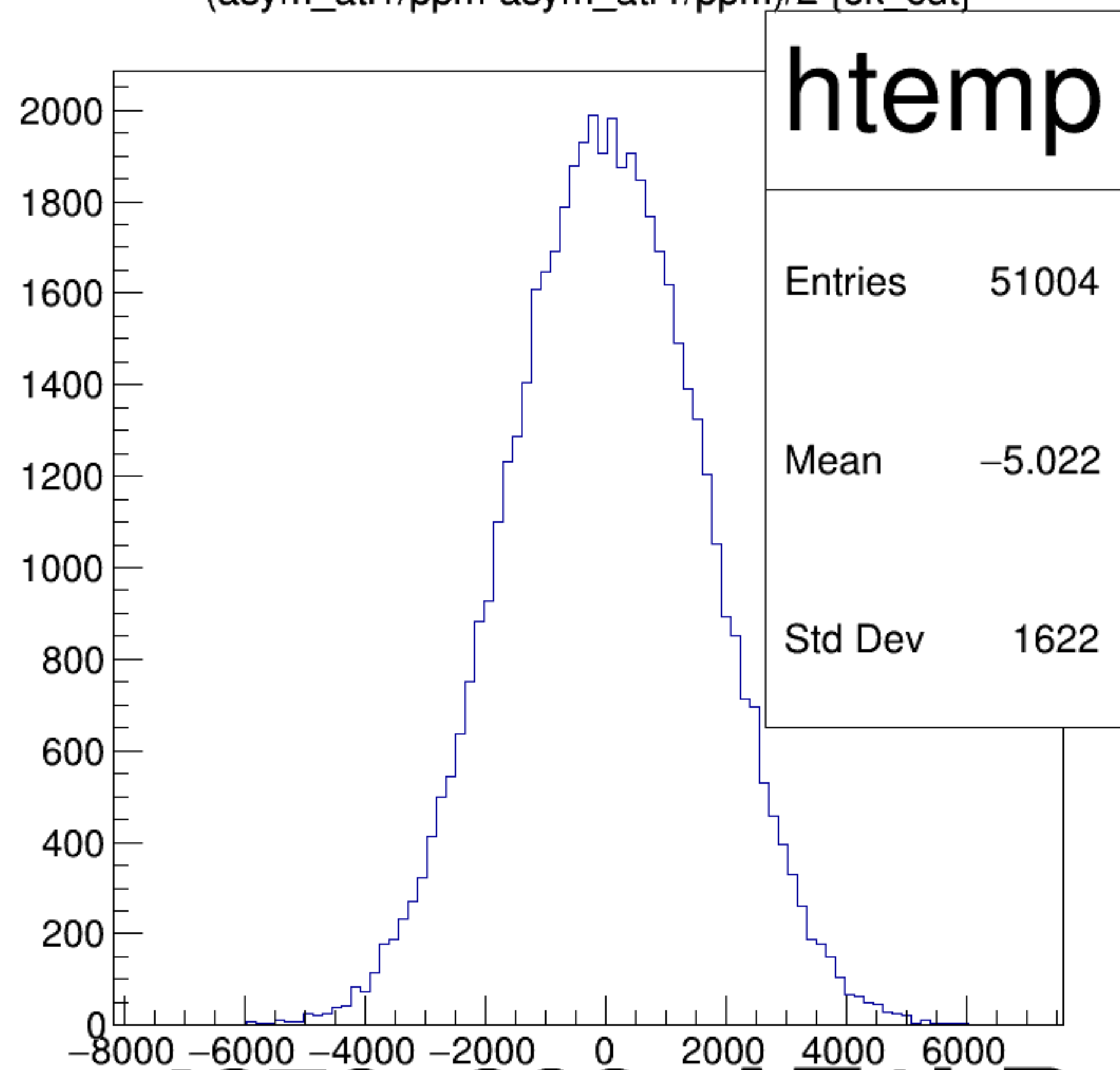
(asym_atl1/ppm-asym_atr1/ppm)/2 {ok_cut}
