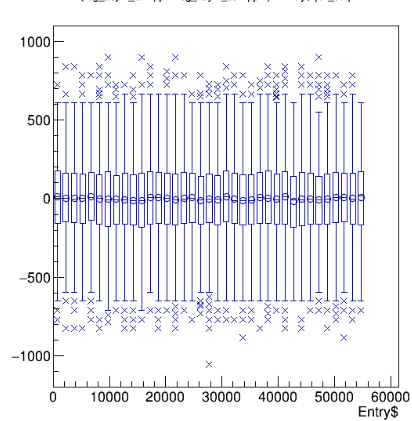
(reg_asym_atl2/ppm-reg_asym_atr2/ppm)/2:Entry$ {ok_cut}
