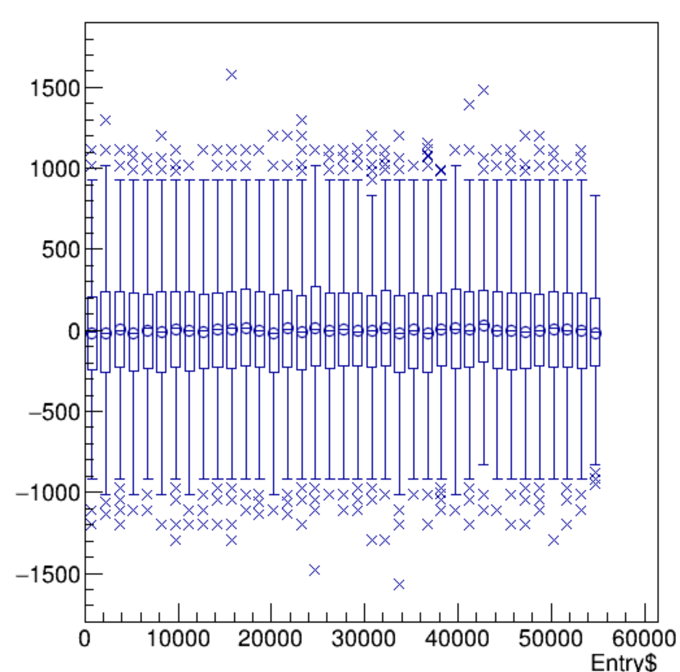
(reg_asym_atl1/ppm+reg_asym_atr1/ppm)/2:Entry$ {ok_cut}
