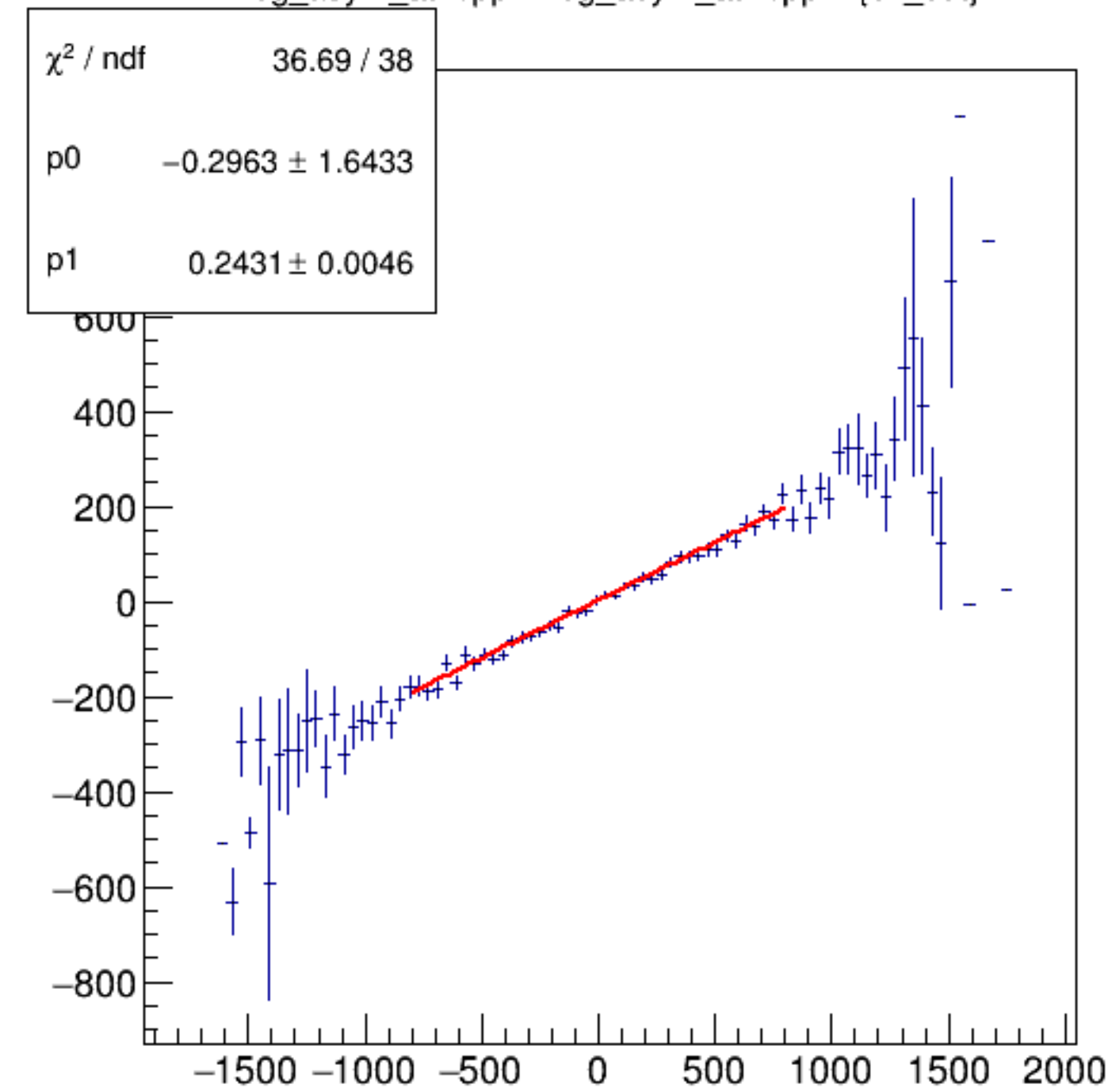
reg_asym_atl2/ppm:reg_asym_atr2/ppm {ok_cut}
