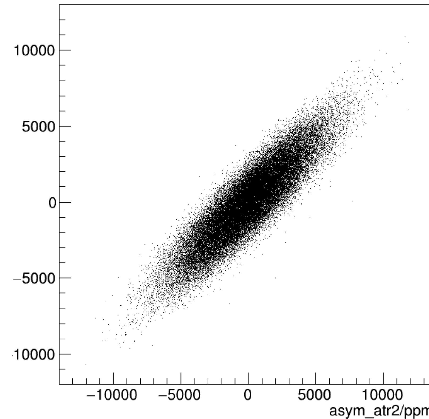
asym_atl2/ppm:asym_atr2/ppm {ok_cut}
