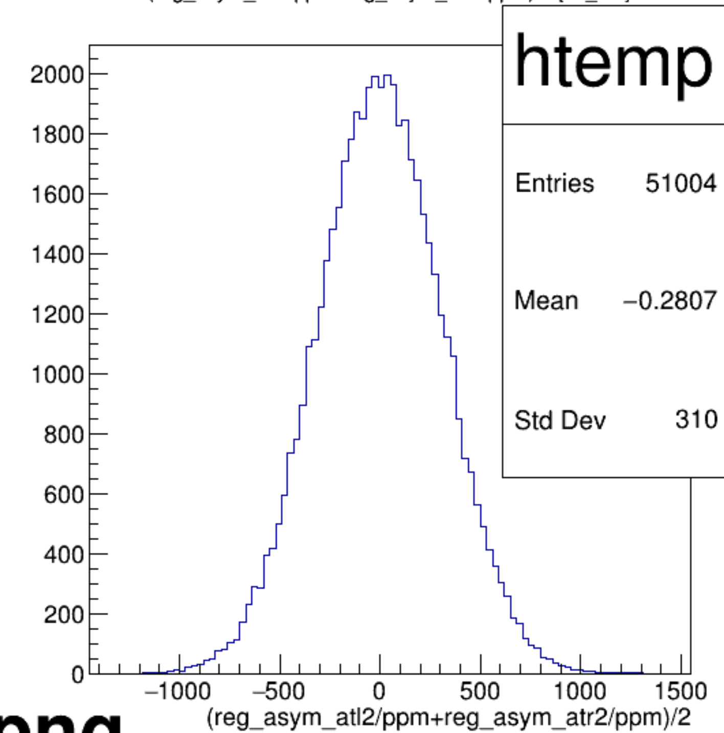
(reg_asym_atl2/ppm+reg_asym_atr2/ppm)/2 {ok_cut}
