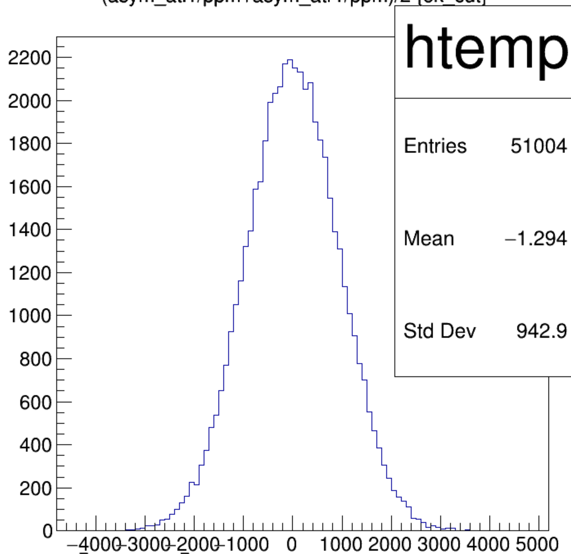
(asym_atl1/ppm+asym_atr1/ppm)/2 {ok_cut}
