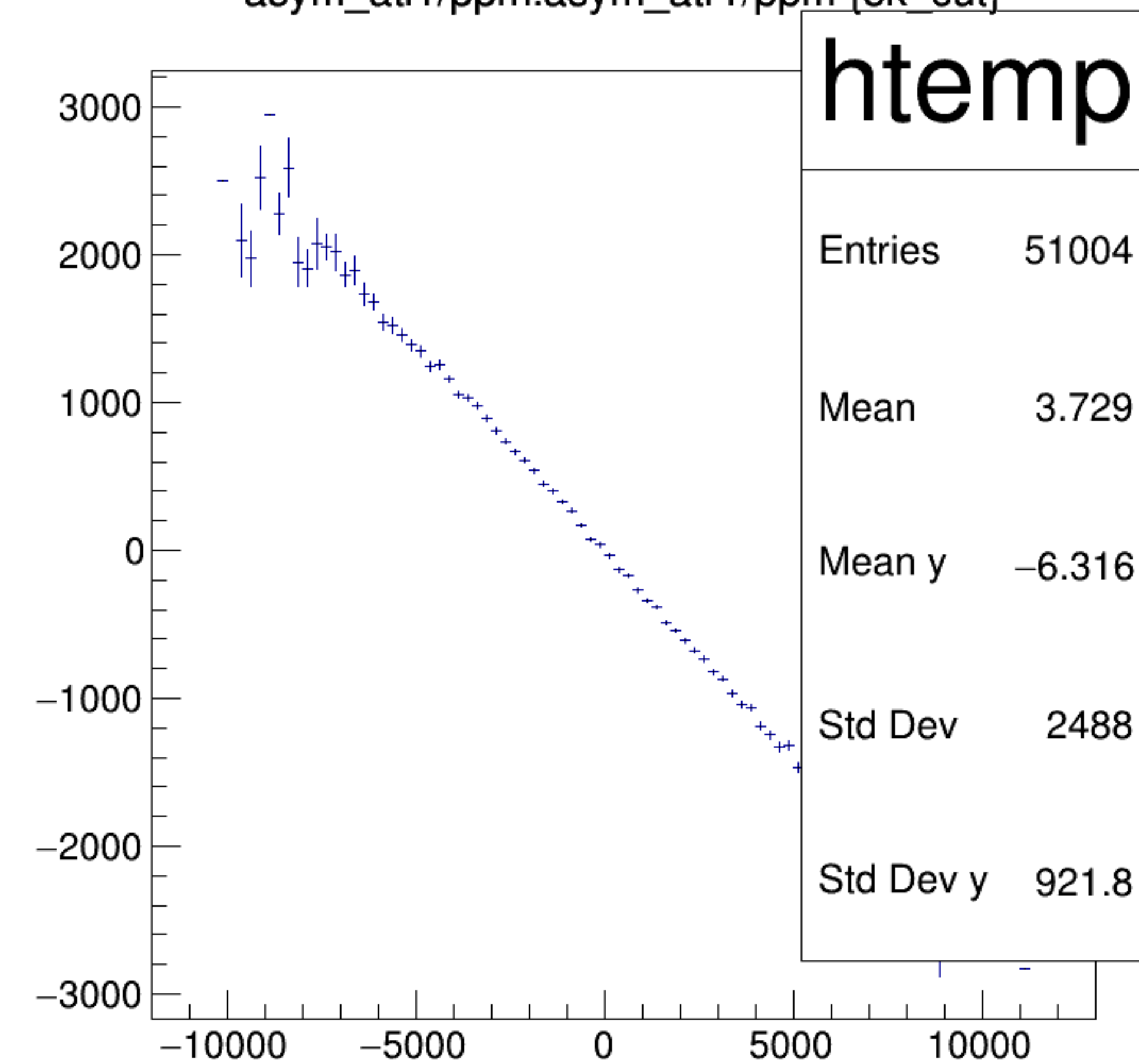
asym_atl1/ppm:asym_atr1/ppm {ok_cut}
