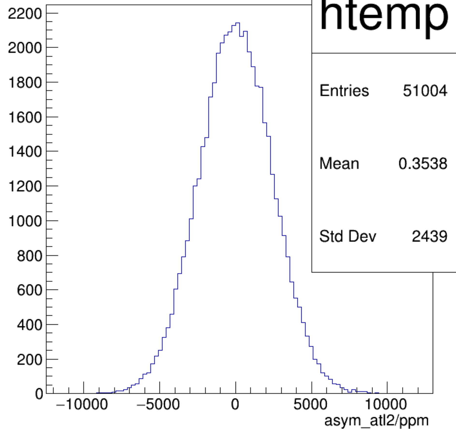
asym_atl2/ppm {ok_cut}
