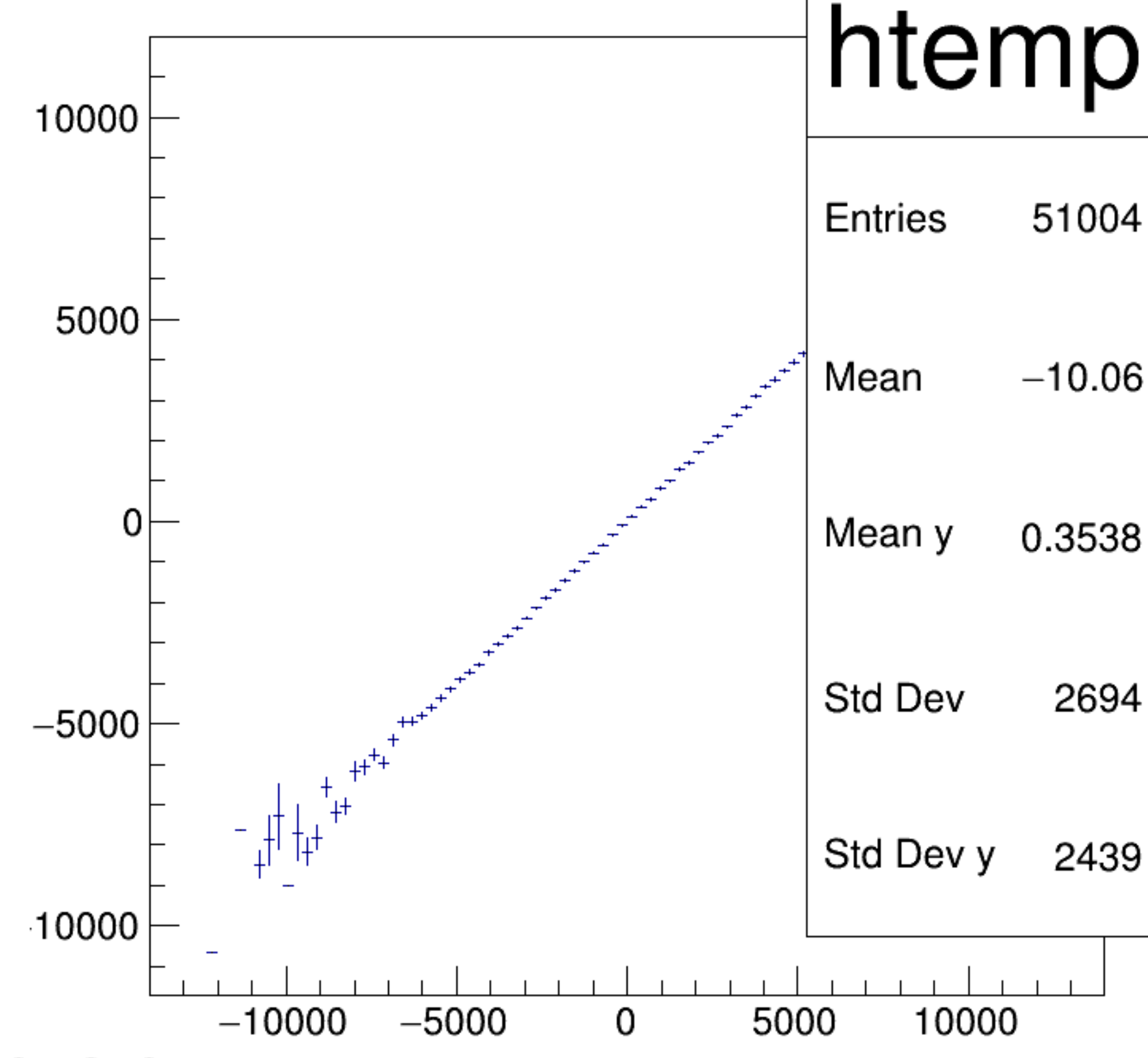
asym_atl2/ppm:asym_atr2/ppm {ok_cut}
