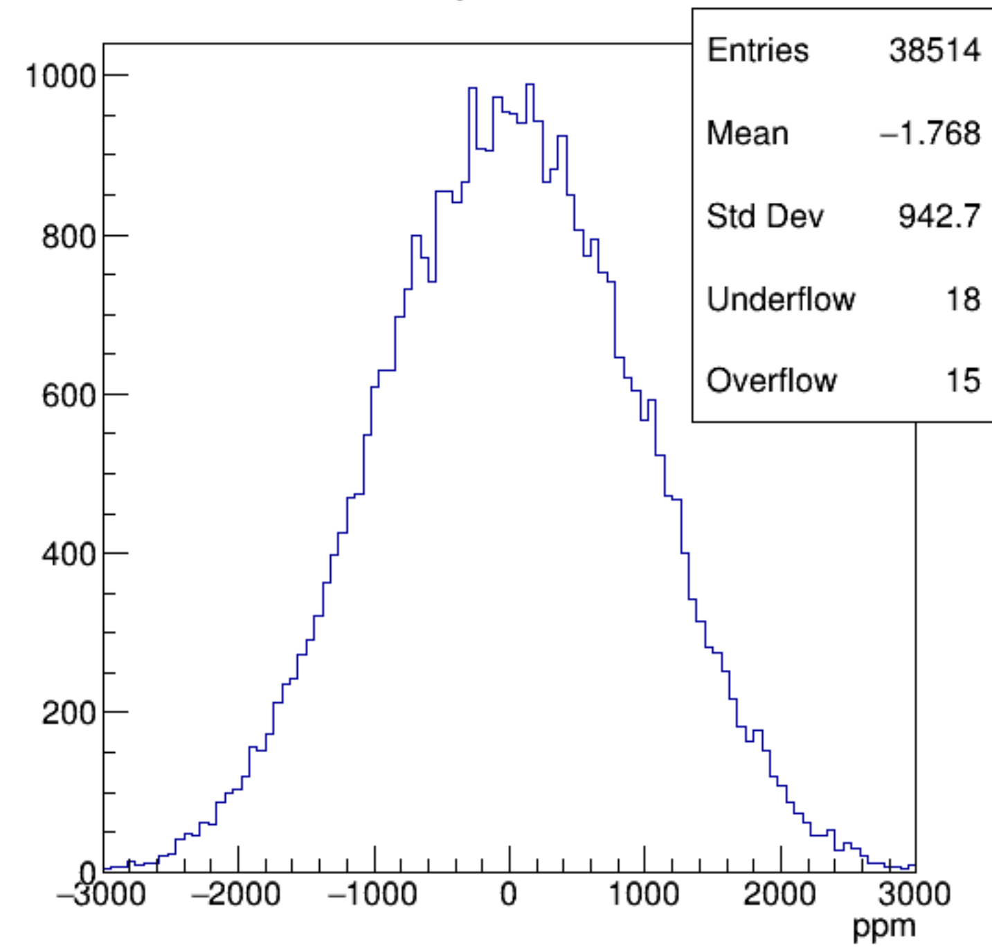
asym_atl1
