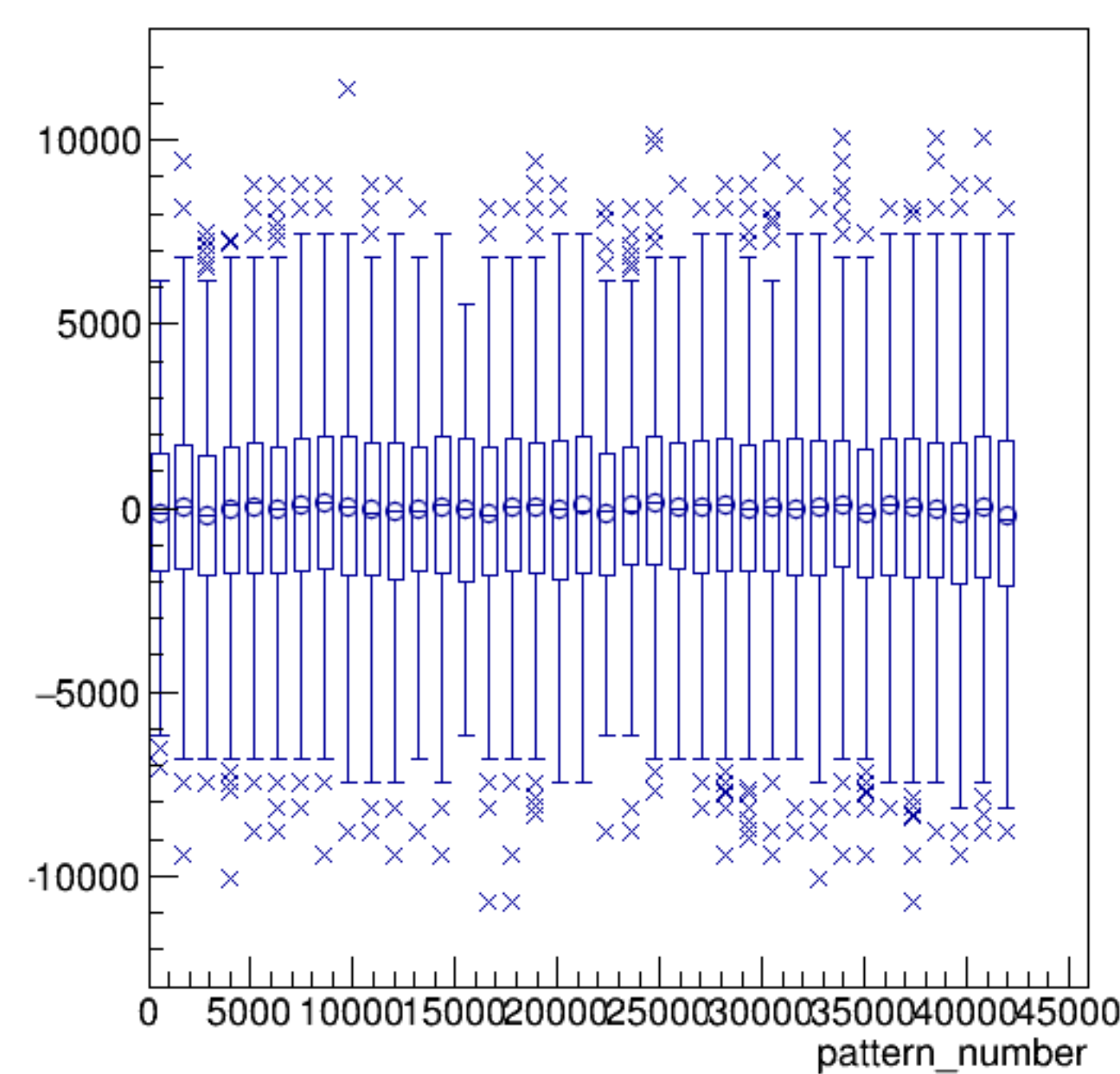
asym_atl2/ppm:pattern_number {ErrorFlag==0}
