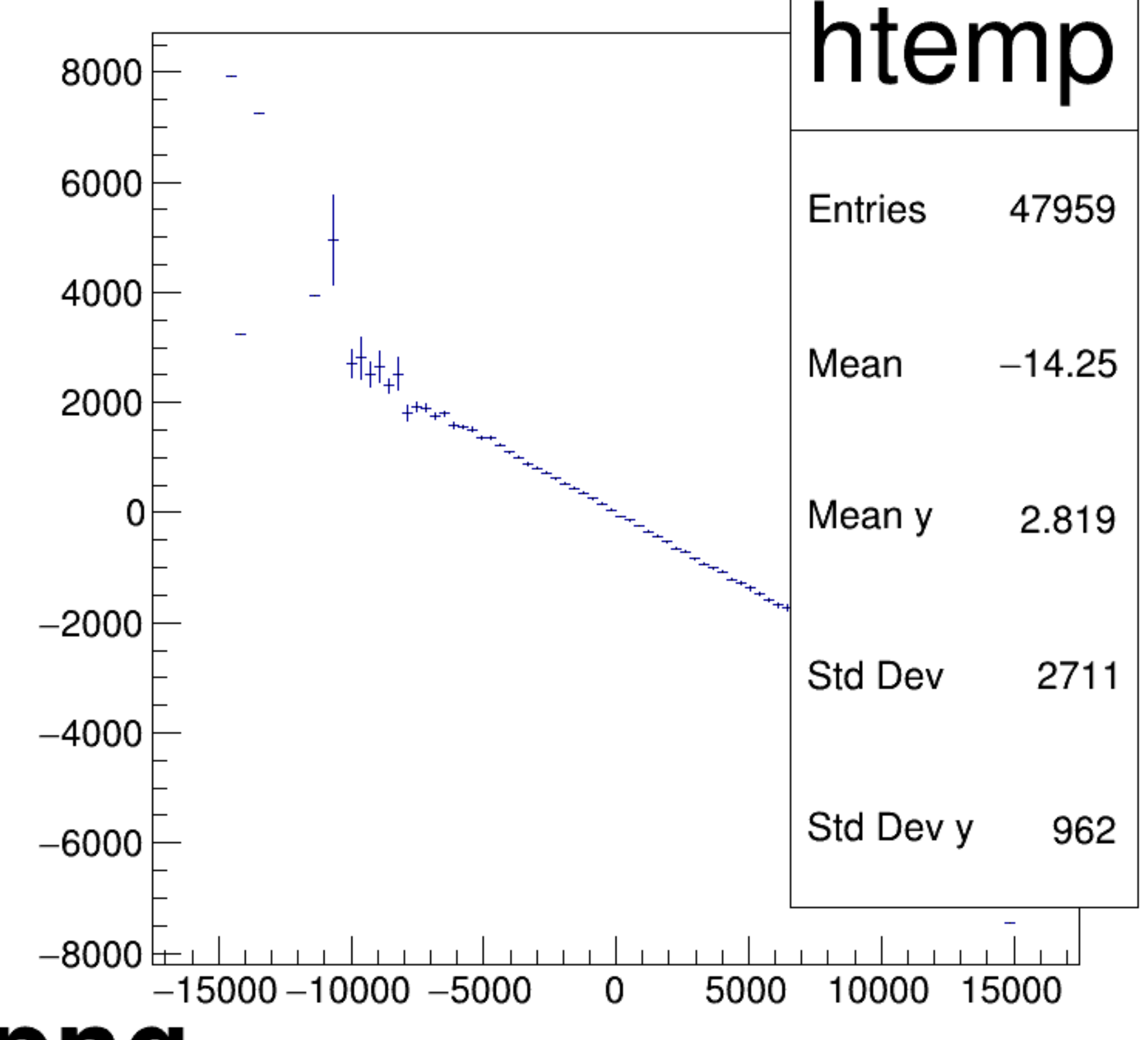
asym_atl1/ppm:asym_atr1/ppm {ok_cut}
