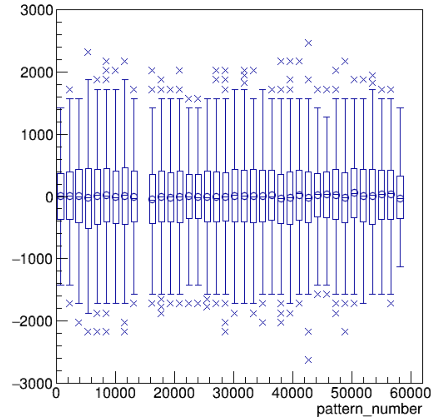
asym_usl/ppm:pattern_number {ErrorFlag==0}
