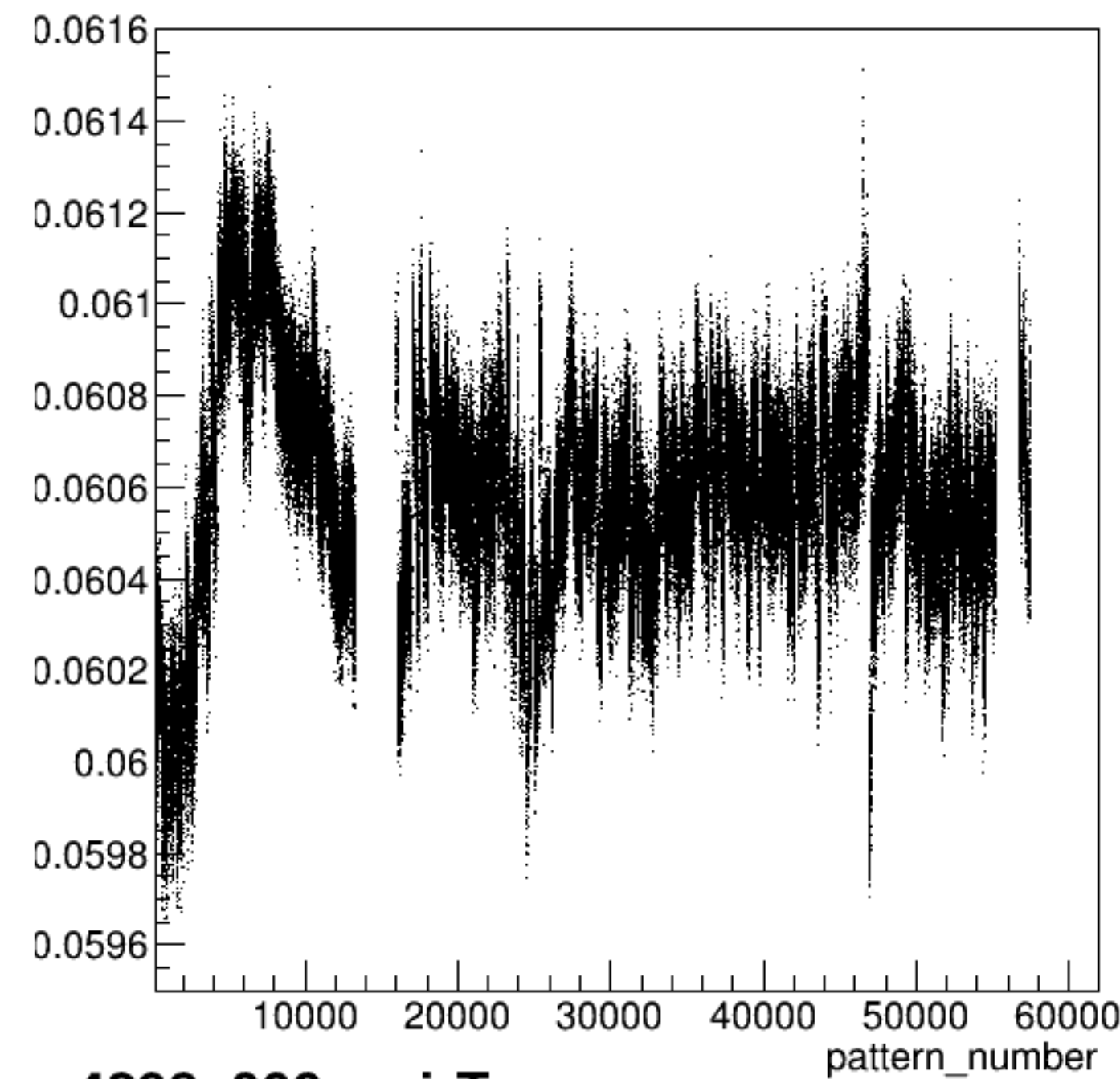
yield_usr:pattern_number {ErrorFlag==0}
