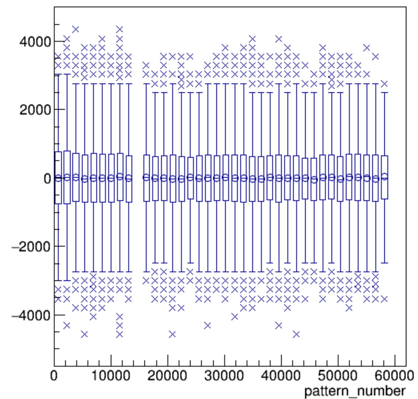
asym_dsr/ppm:pattern_number {ErrorFlag==0}
