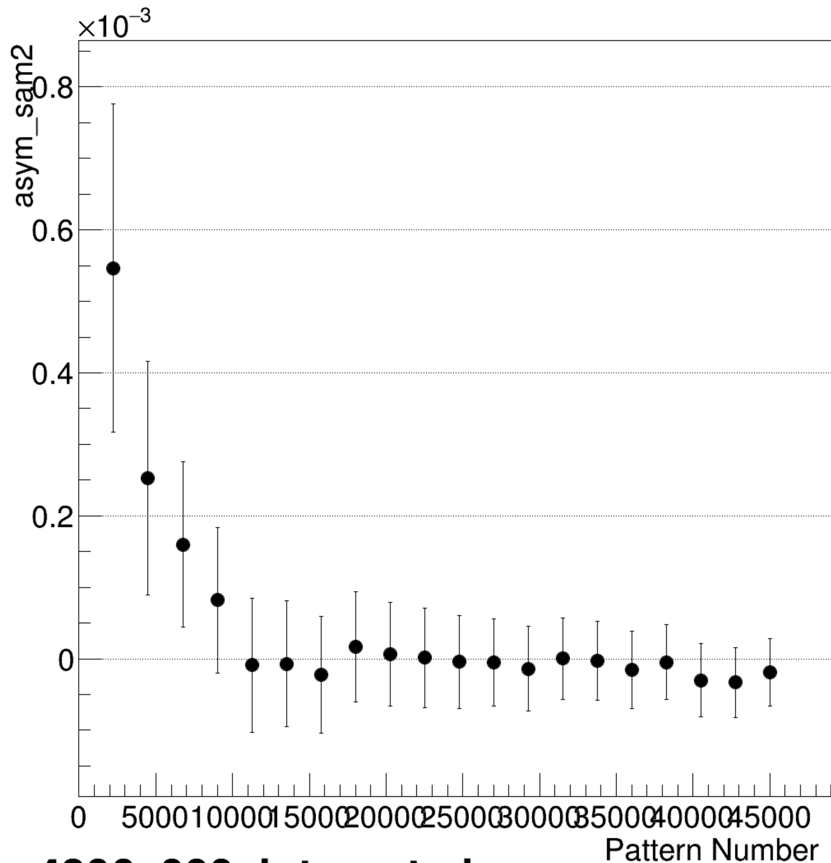
asym_sam2 Integrated Convergence
