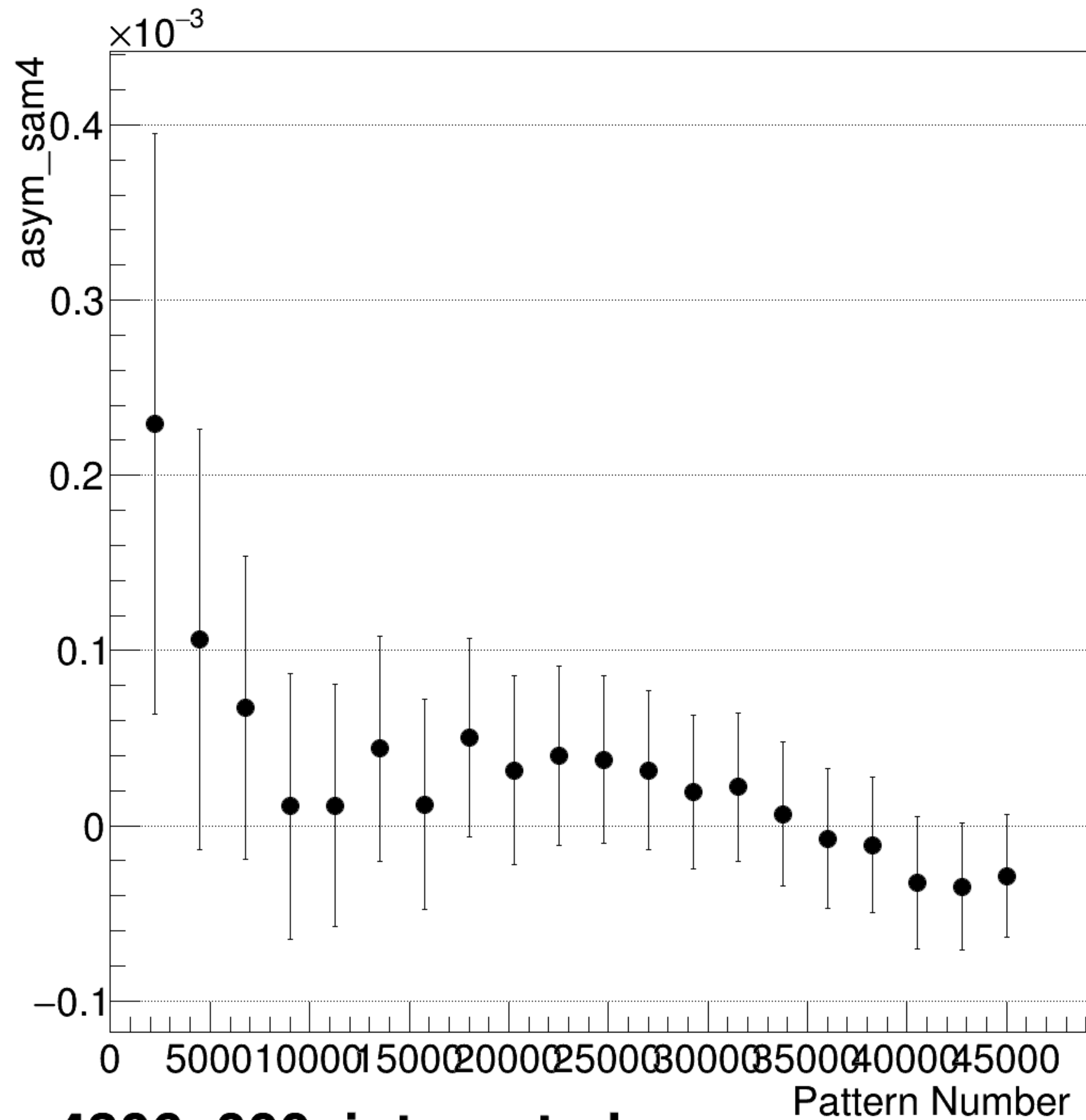
asym_sam4 Integrated Convergence
