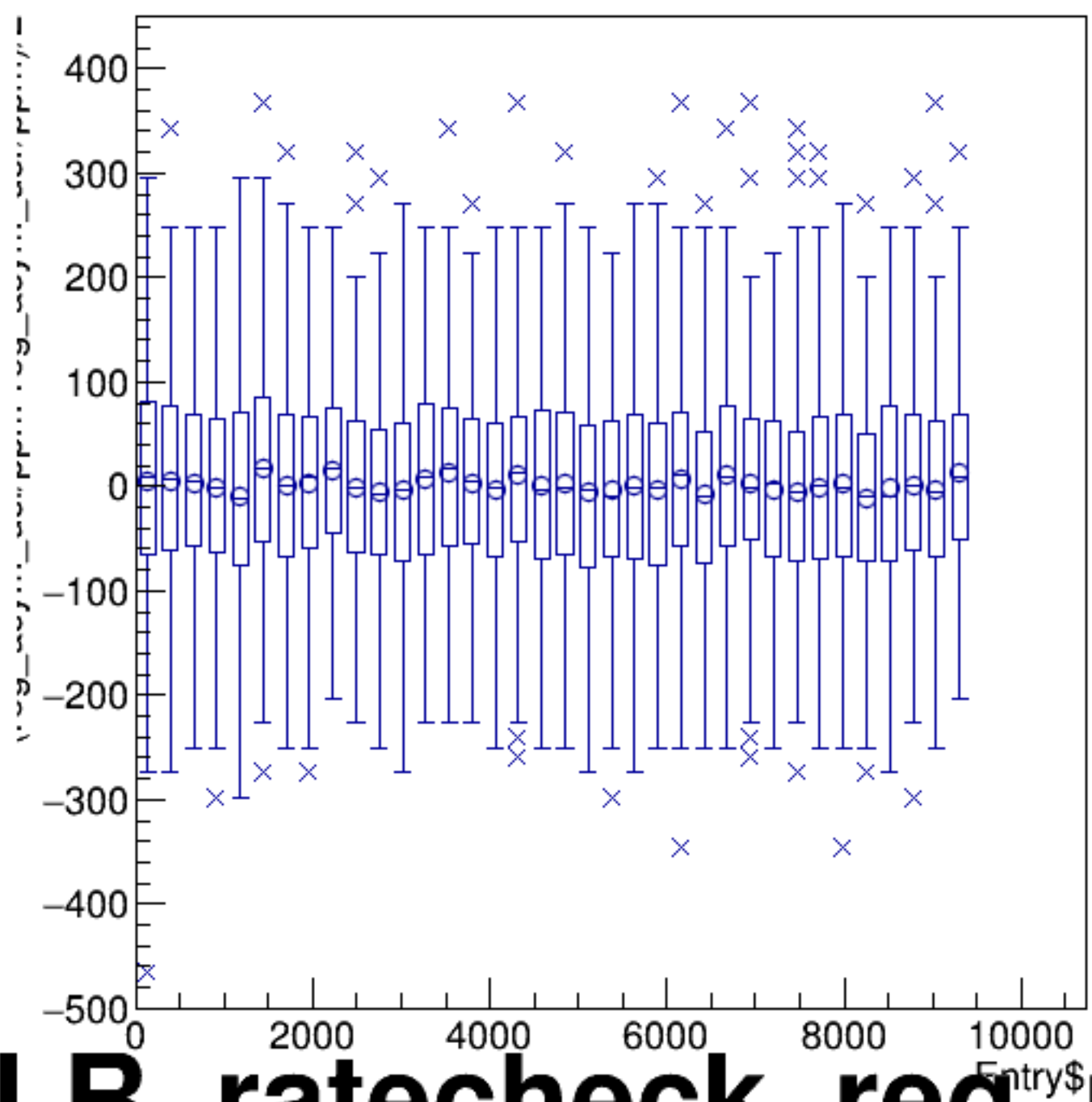
(reg_asym_usl/ppm-reg_asym_usr/ppm)/2:Entry$ {ok_cut}
