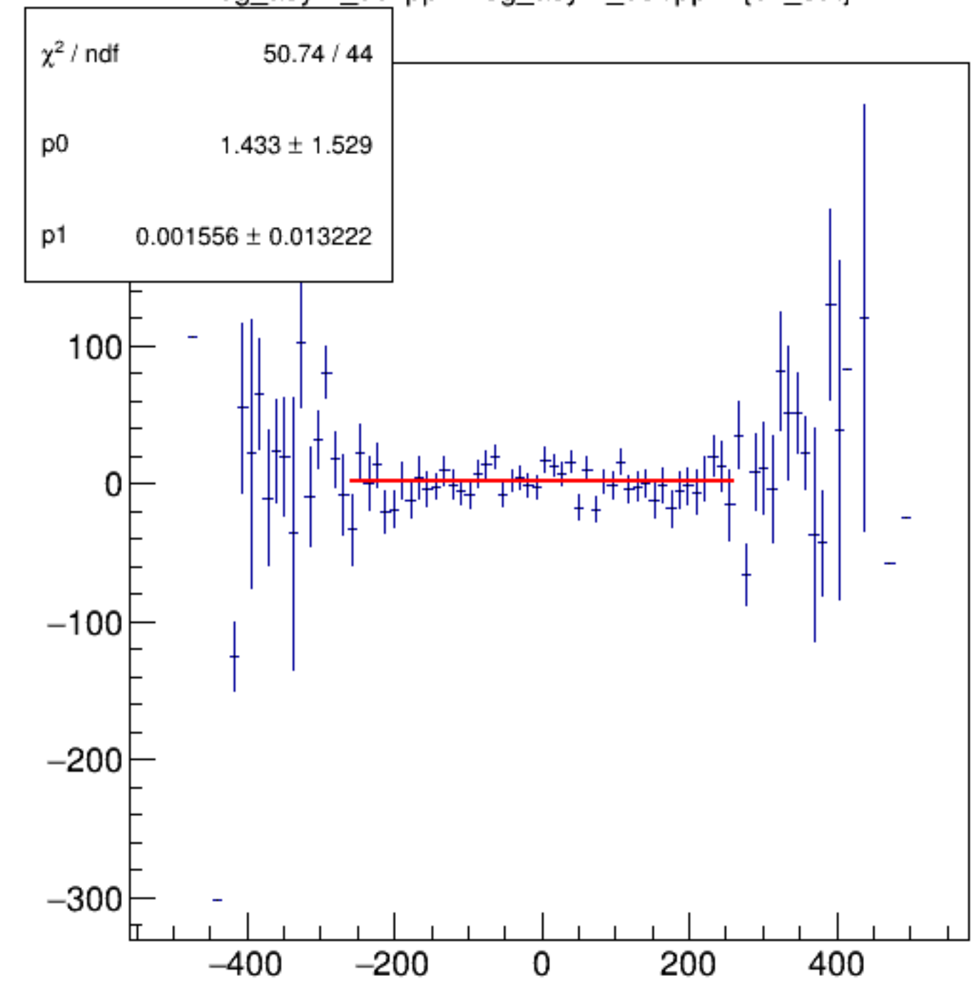
reg_asym_usl/ppm:reg_asym_usr/ppm {ok_cut}
