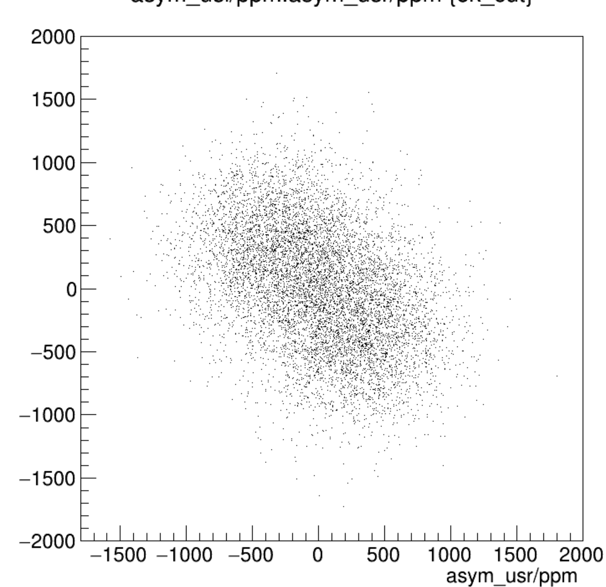
asym_usl/ppm:asym_usr/ppm {ok_cut}
