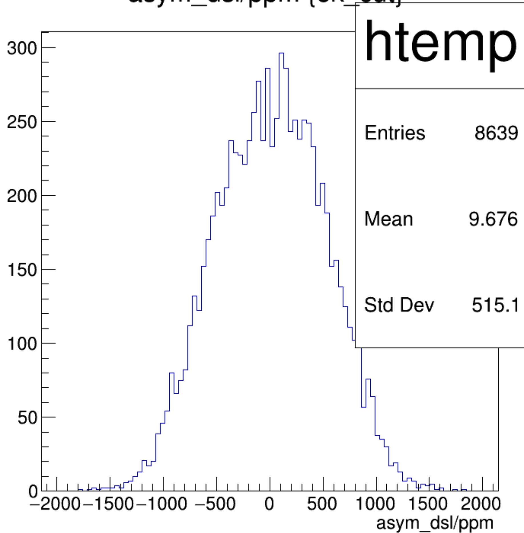
asym_dsl/ppm {ok_cut}
