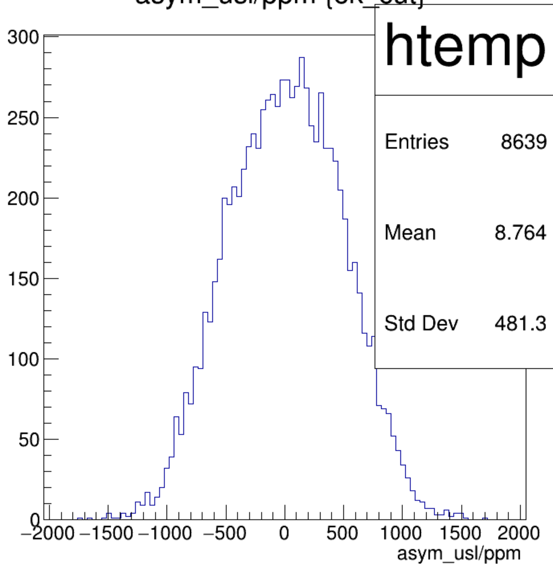
asym_usl/ppm {ok_cut}
