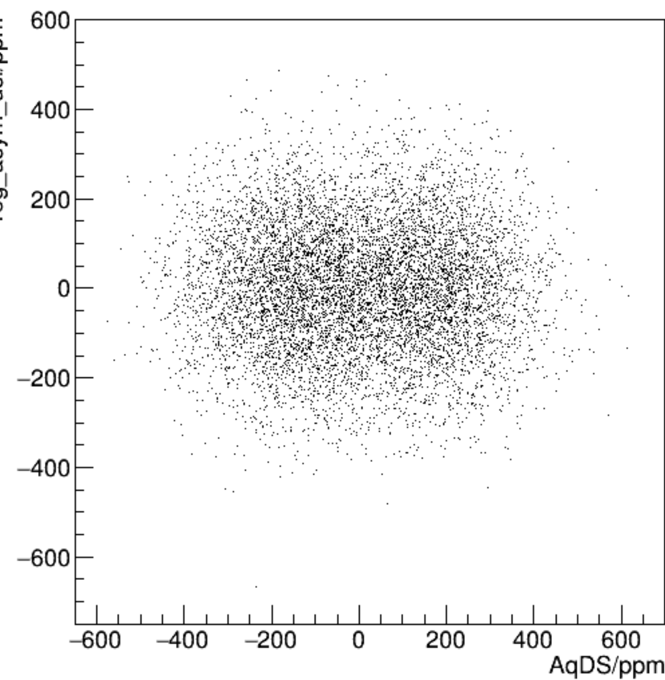
reg_asym_usl/ppm:AqDS/ppm {ok_cut}
