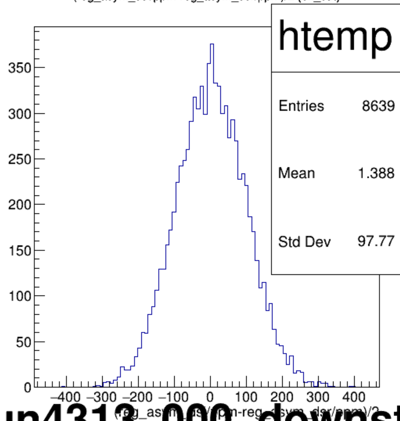
(reg_asym_dsl/ppm-reg_asym_dsr/ppm)/2 {ok_cut}
