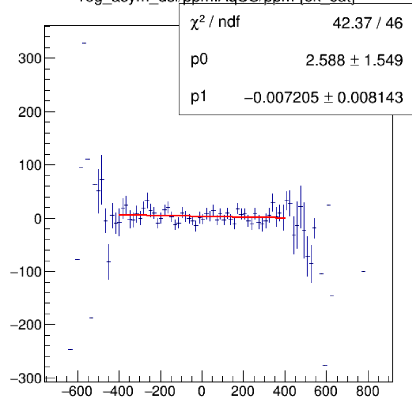
reg_asym_dsl/ppm:AqUS/ppm {ok_cut}
