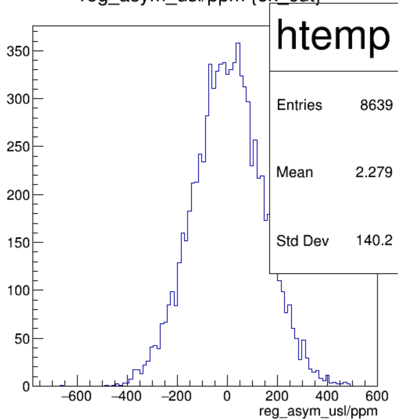
reg_asym_usl/ppm {ok_cut}
