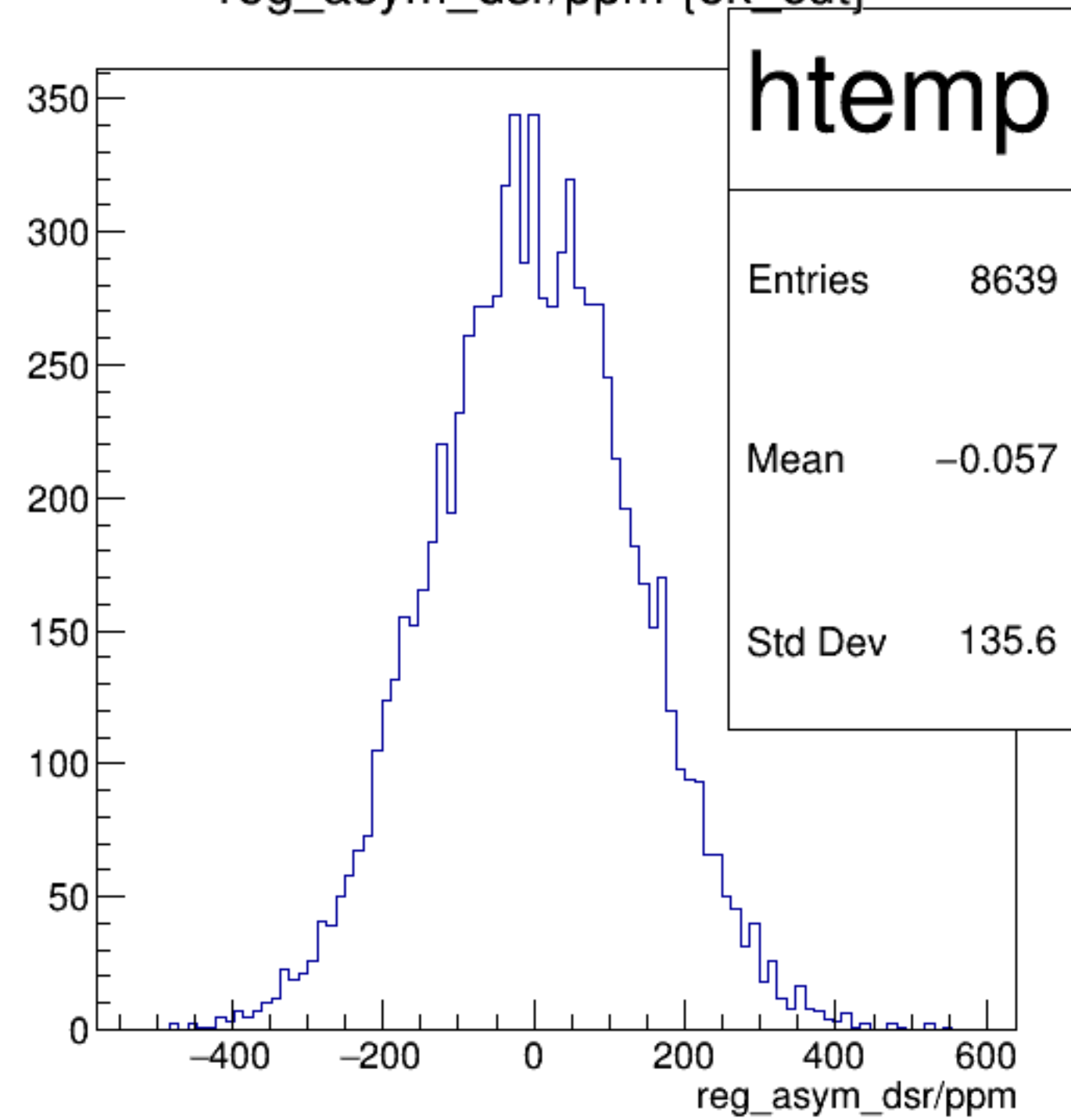
reg_asym_dsr/ppm {ok_cut}
