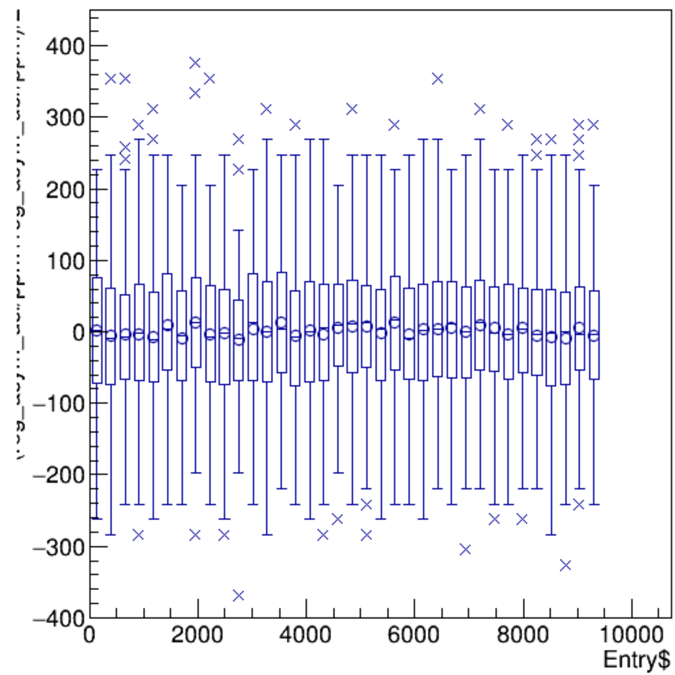
(reg_asym_usl/ppm+reg_asym_usr/ppm)/2:Entry$ {ok_cut}
