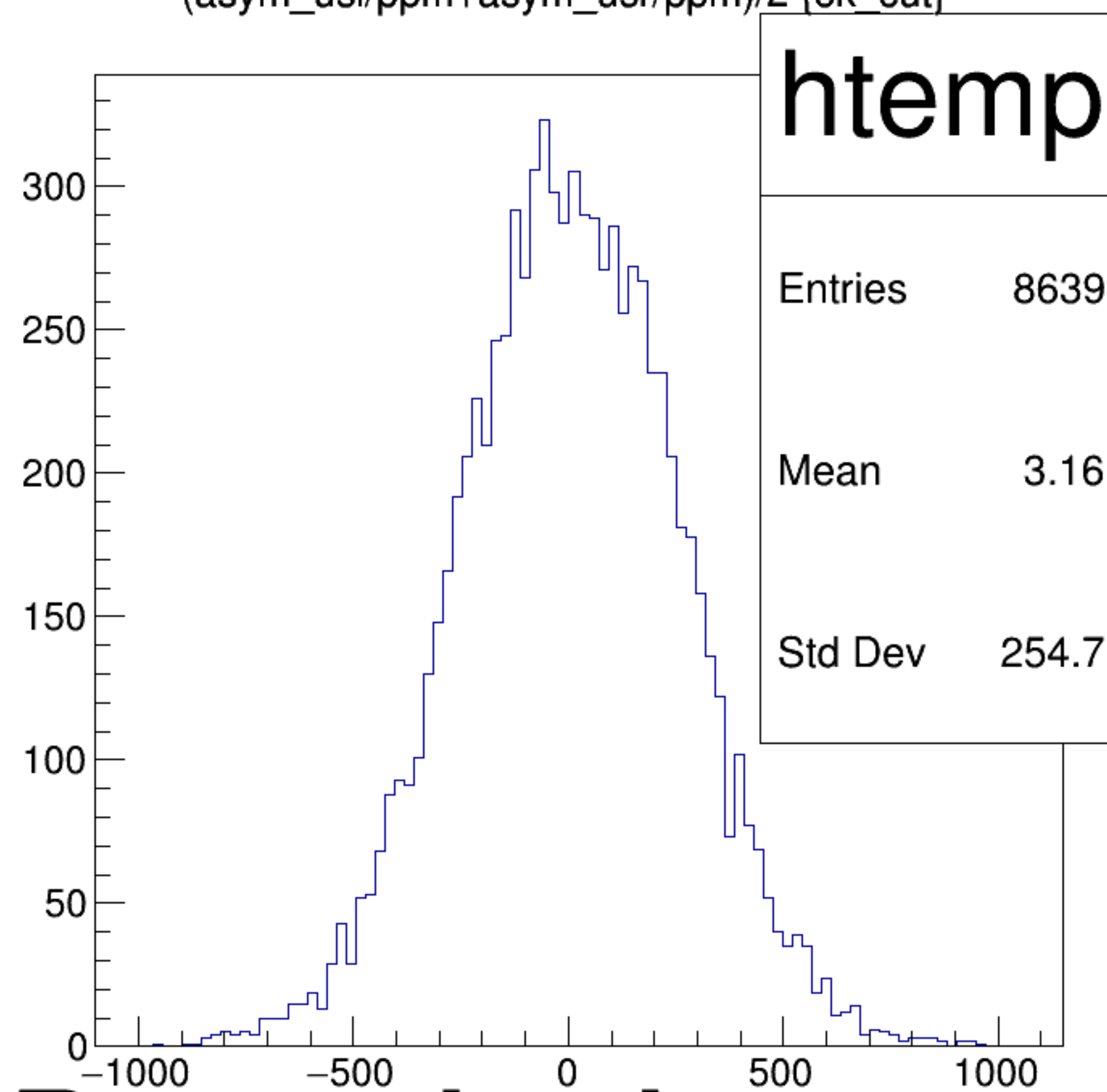
(asym_usl/ppm+asym_usr/ppm)/2 {ok_cut}
