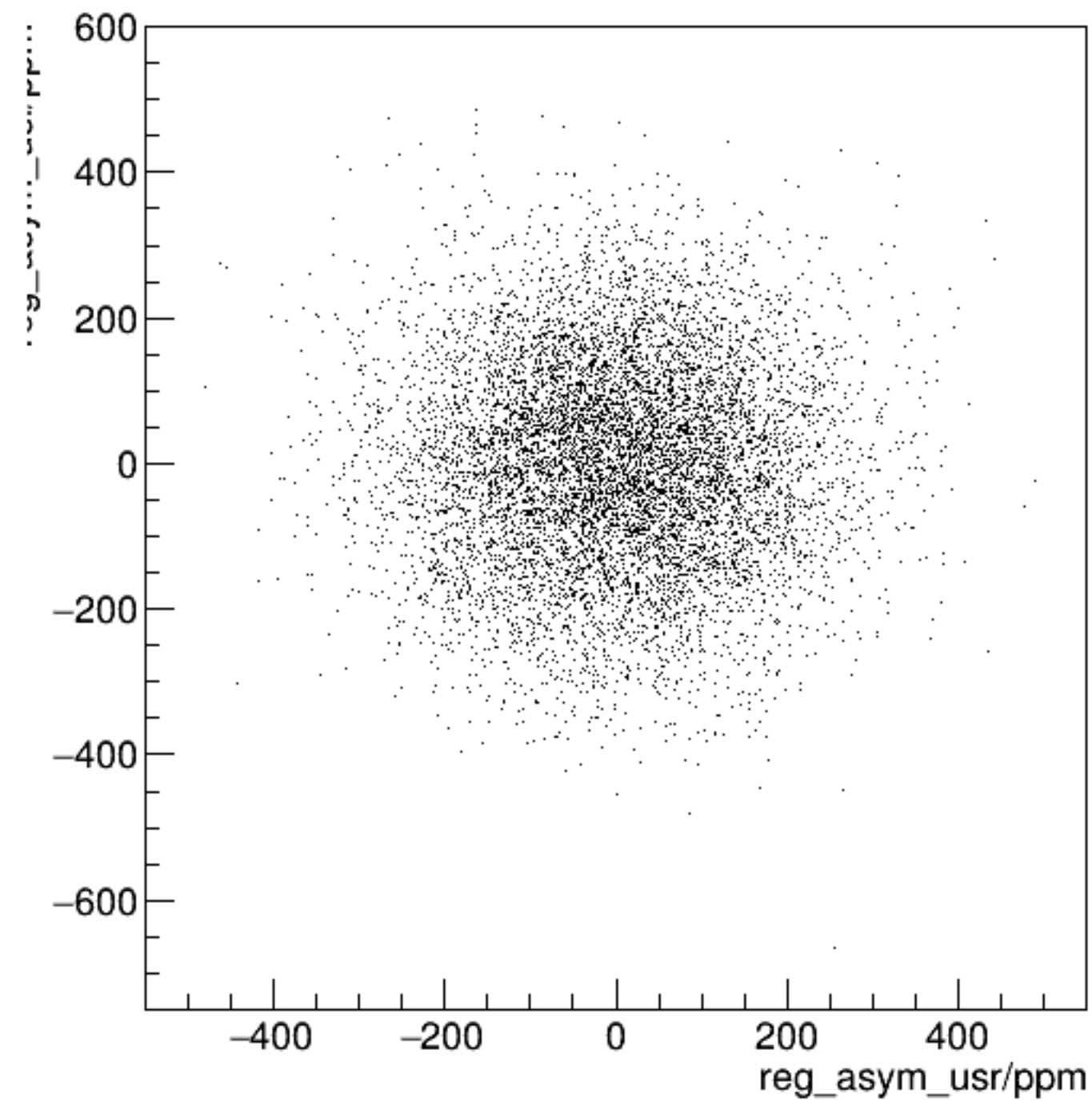
reg_asym_usl/ppm:reg_asym_usr/ppm {ok_cut}
