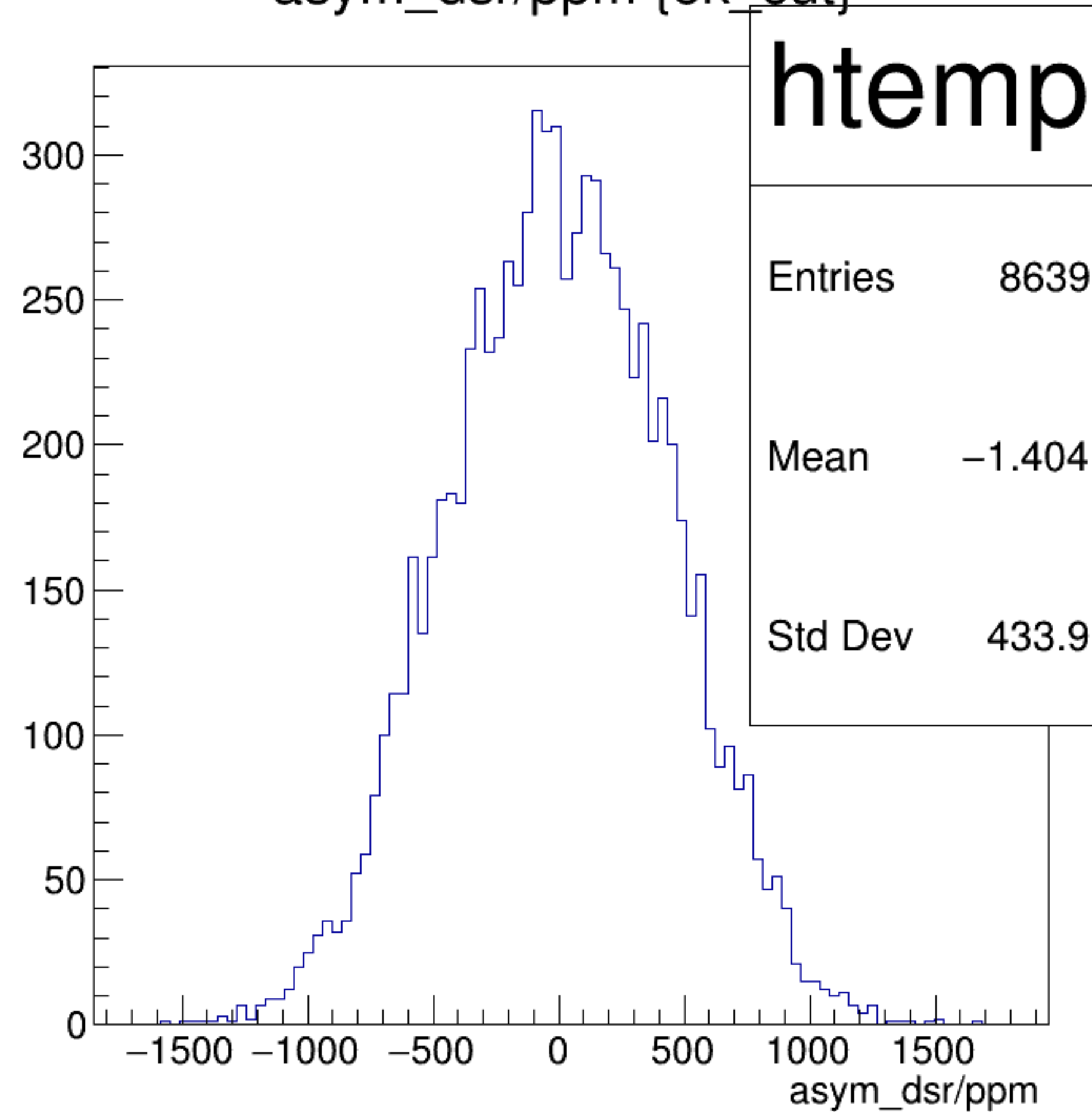
asym_dsr/ppm {ok_cut}
