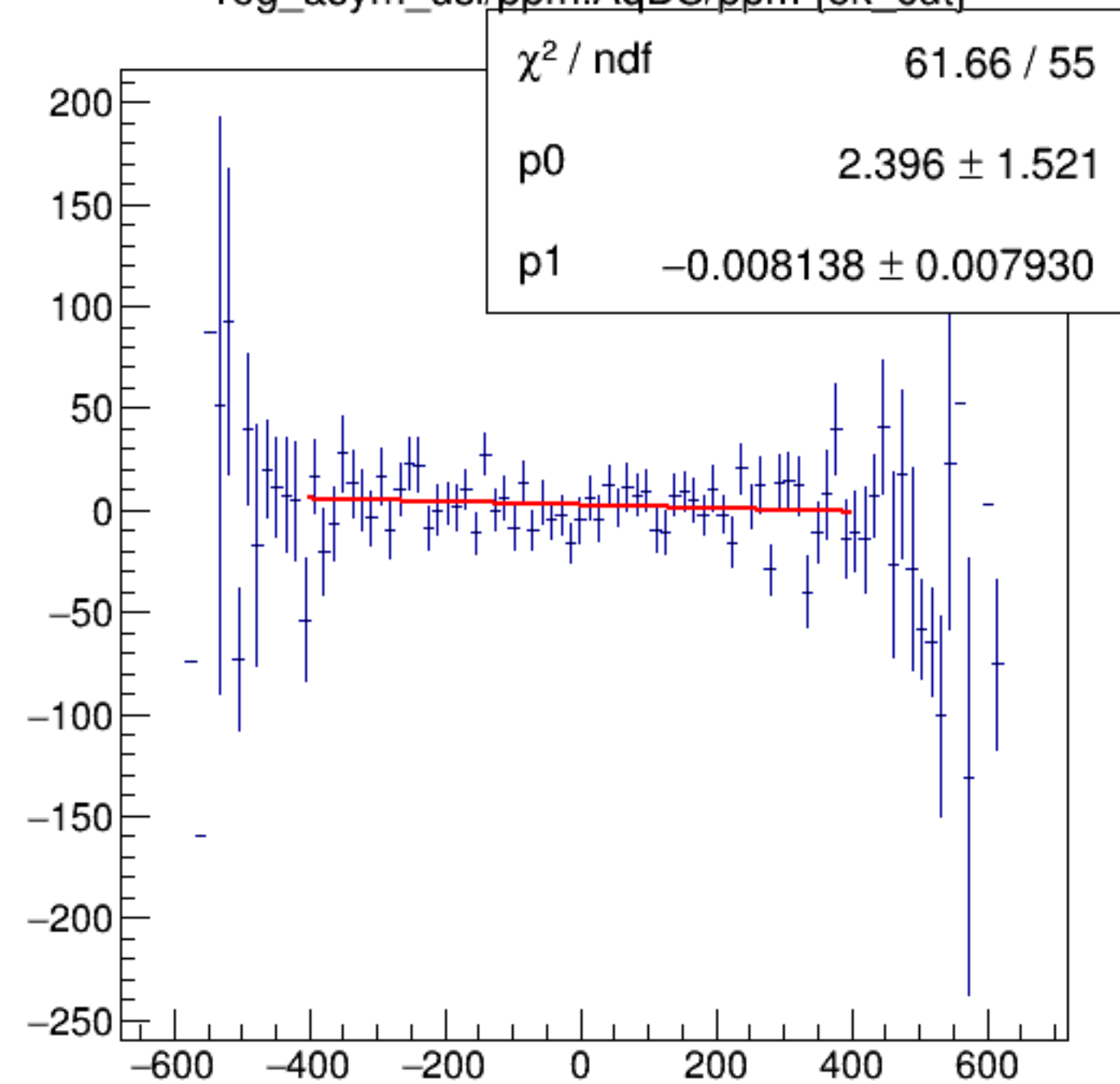
reg_asym_usl/ppm:AqDS/ppm {ok_cut}
