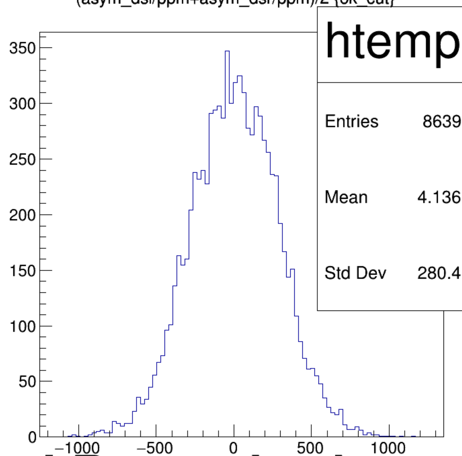
(asym_dsl/ppm+asym_dsr/ppm)/2 {ok_cut}
