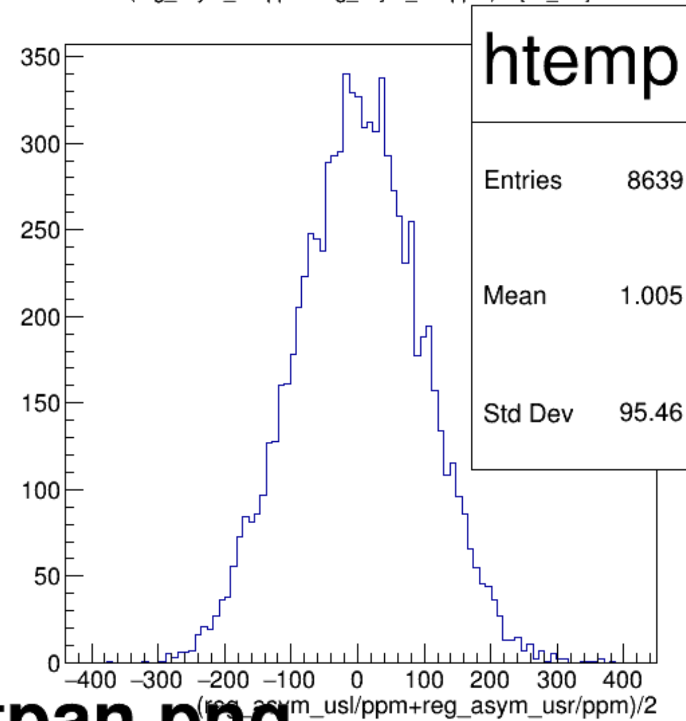
(reg_asym_usl/ppm+reg_asym_usr/ppm)/2 {ok_cut}
