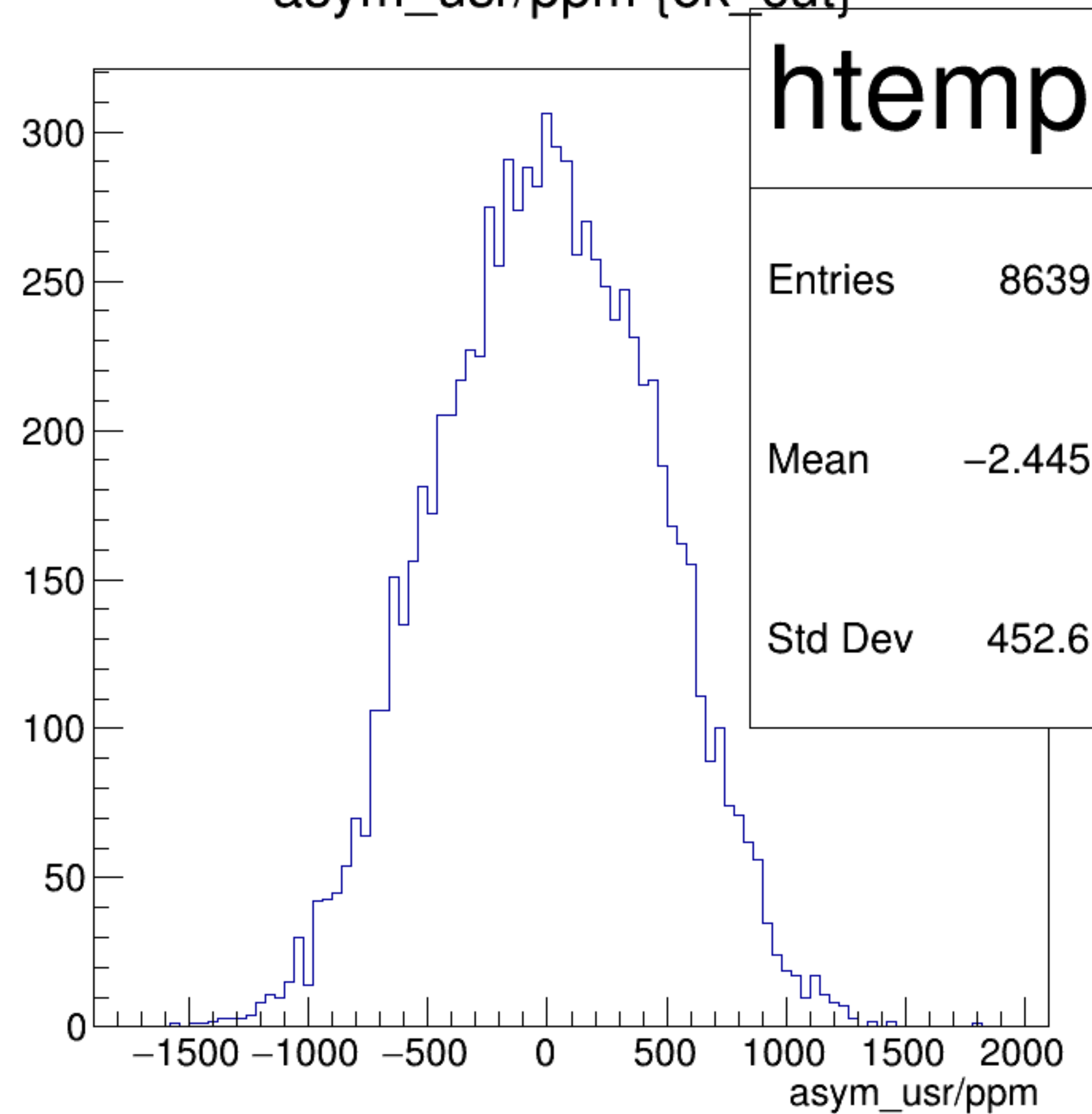
asym_usr/ppm {ok_cut}
