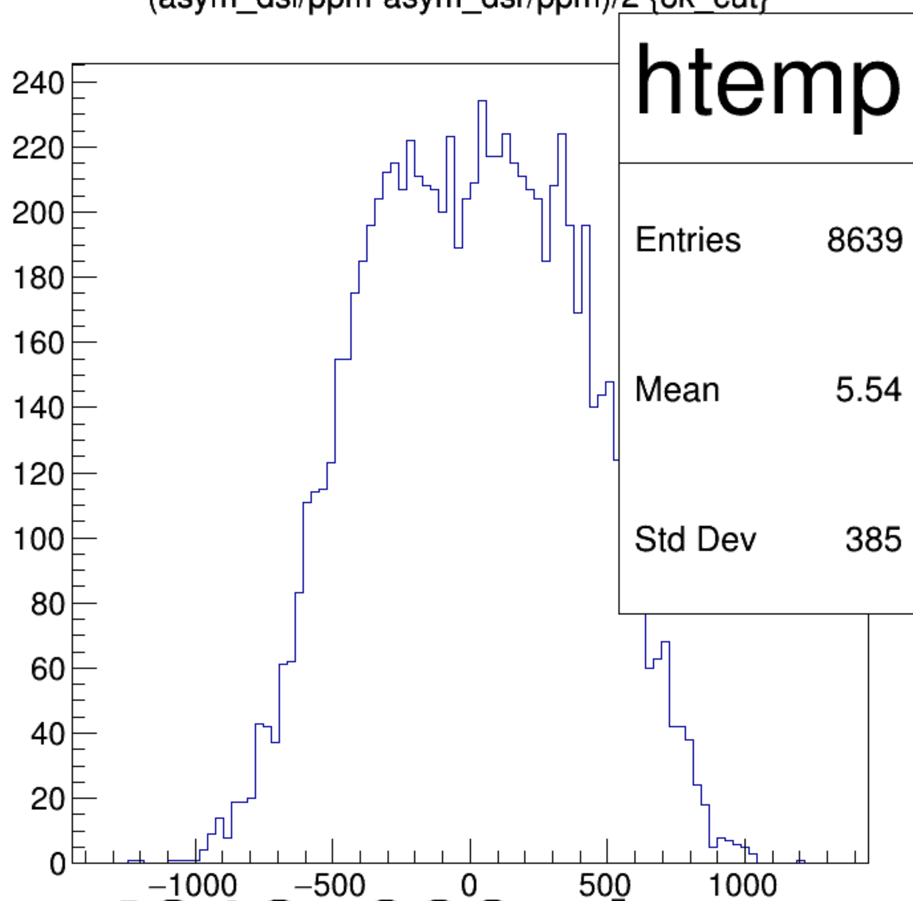
(asym_dsl/ppm-asym_dsr/ppm)/2 {ok_cut}
