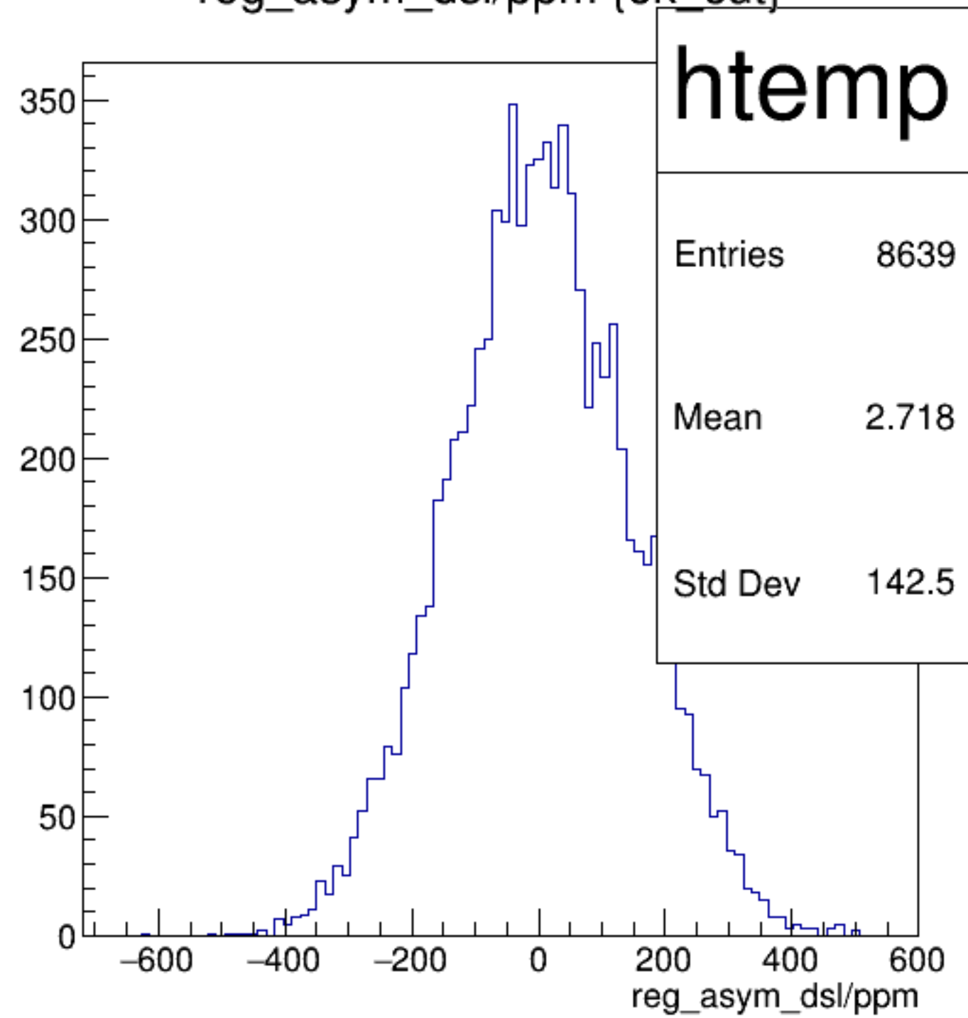
reg_asym_dsl/ppm {ok_cut}
