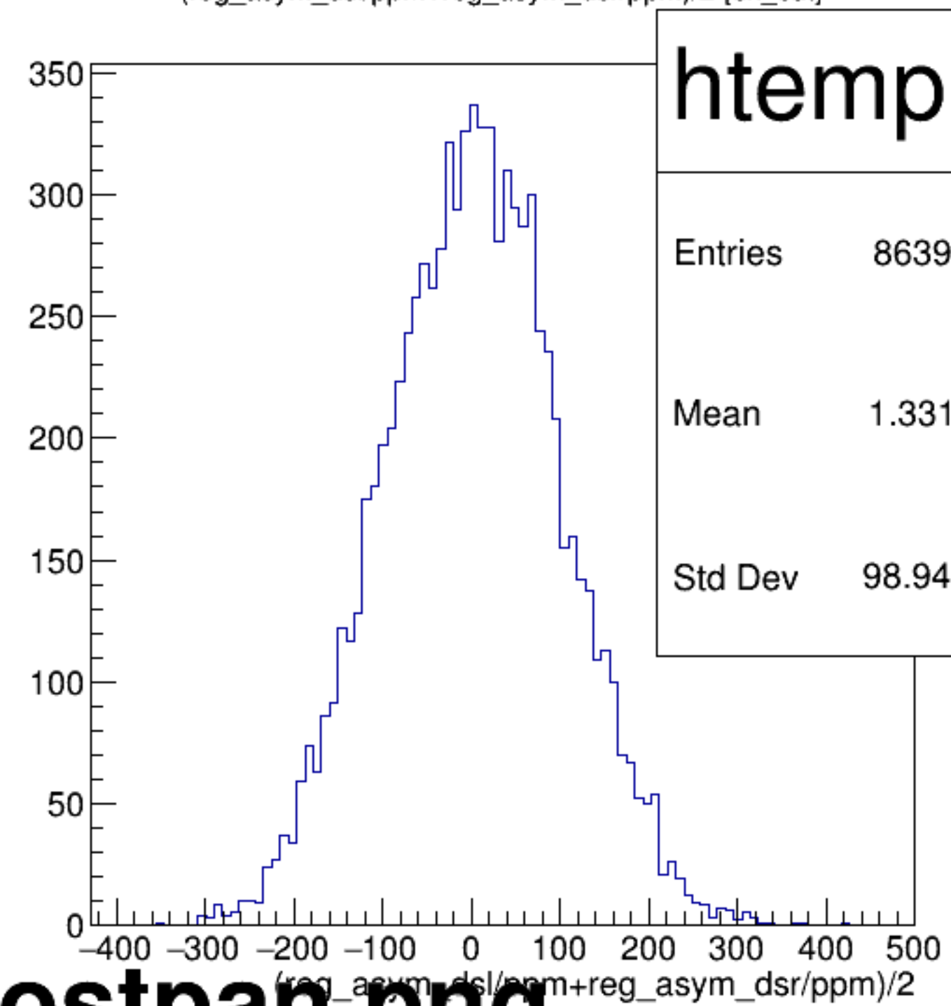
(reg_asym_dsl/ppm+reg_asym_dsr/ppm)/2 {ok_cut}
