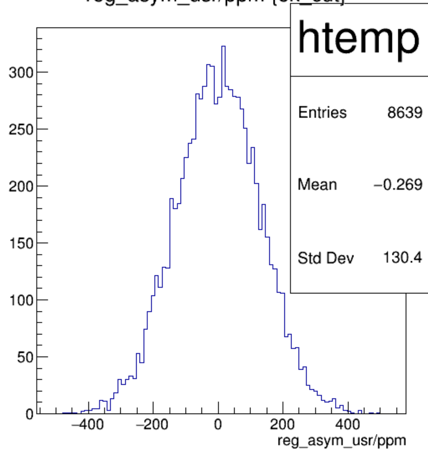
reg_asym_usr/ppm {ok_cut}
