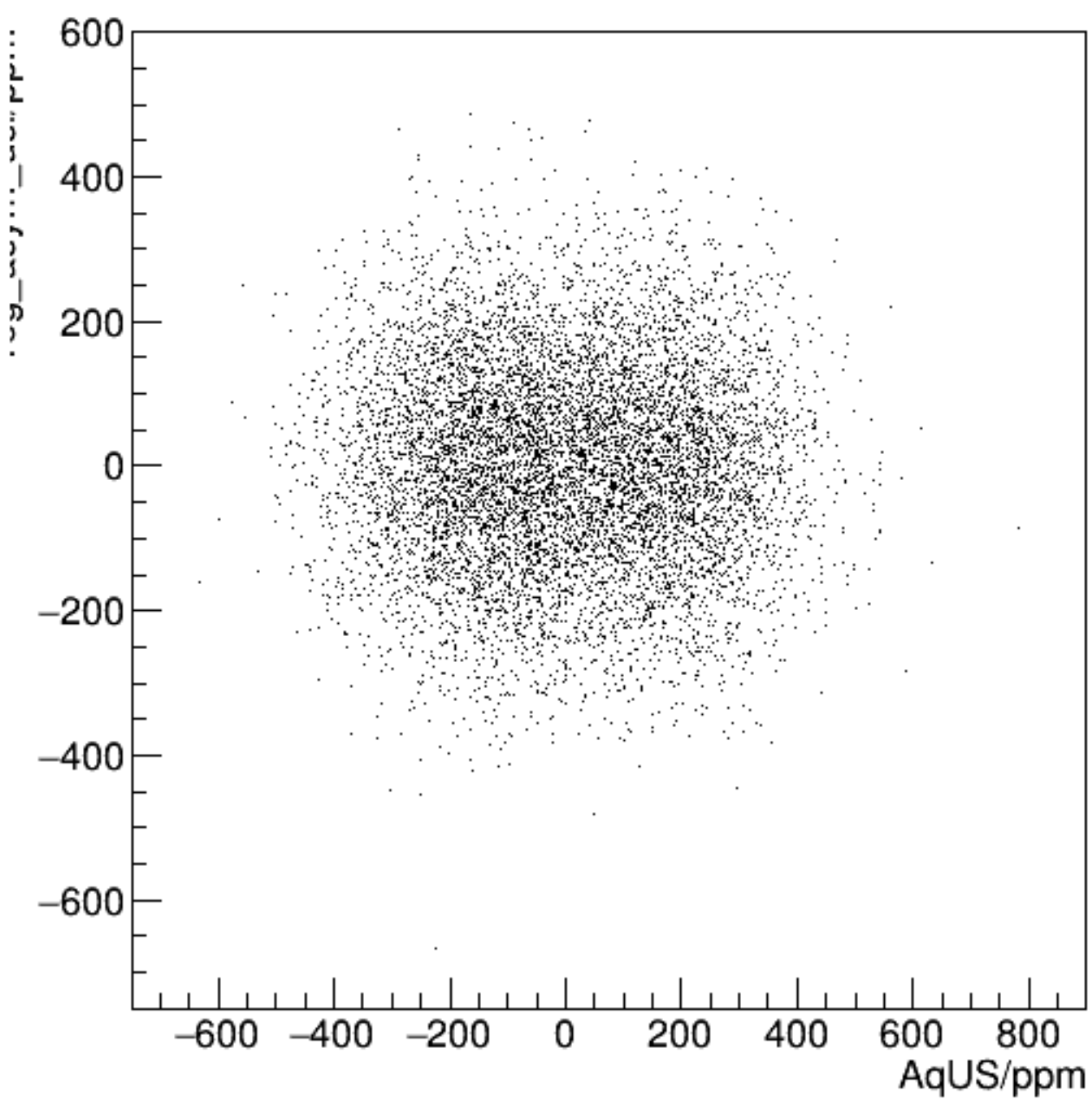
reg_asym_usl/ppm:AqUS/ppm {ok_cut}
