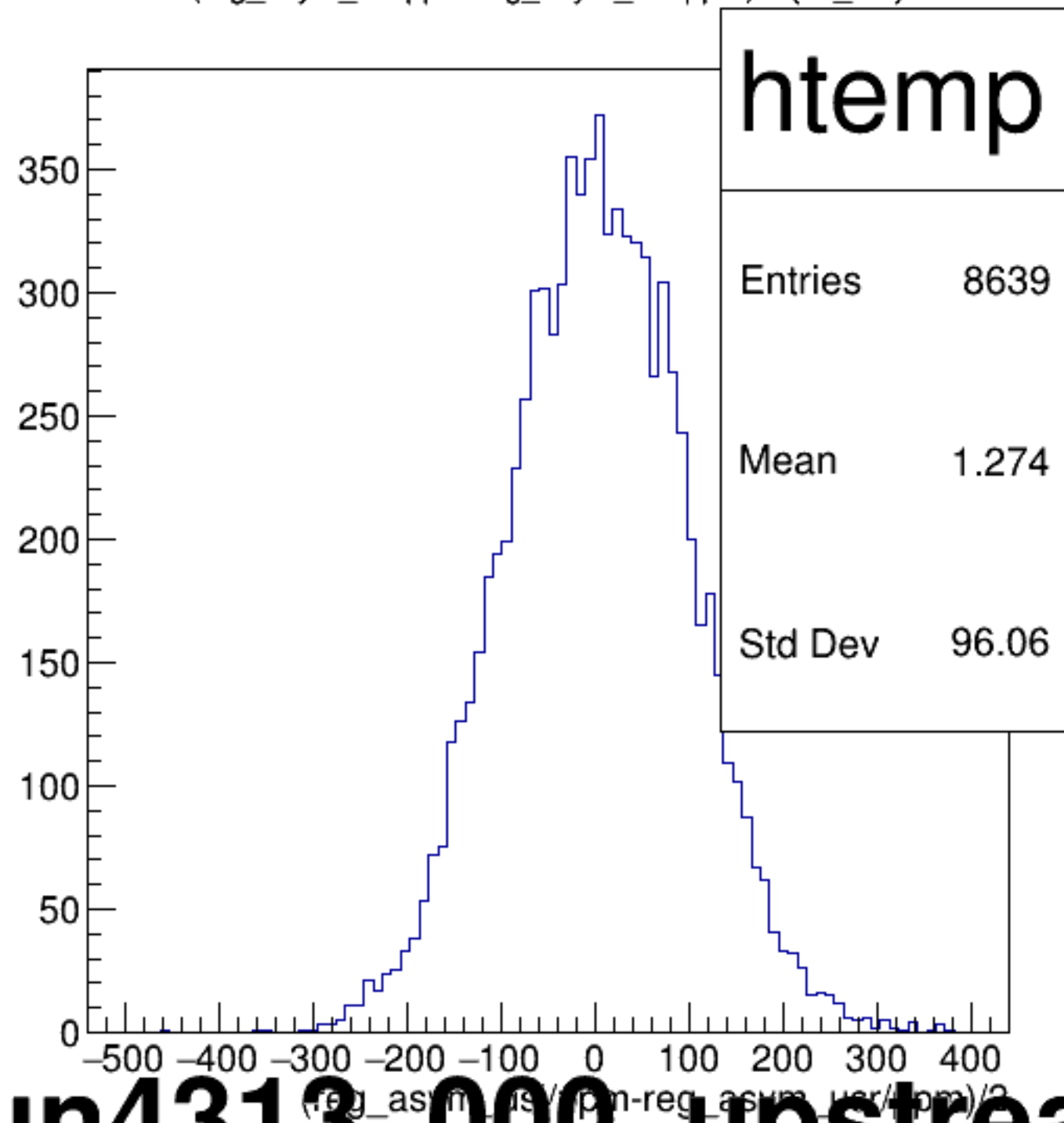
(reg_asym_usl/ppm-reg_asym_usr/ppm)/2 {ok_cut}
