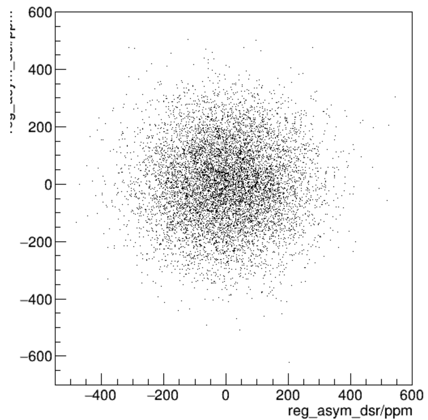
reg_asym_dsl/ppm:reg_asym_dsr/ppm {ok_cut}
