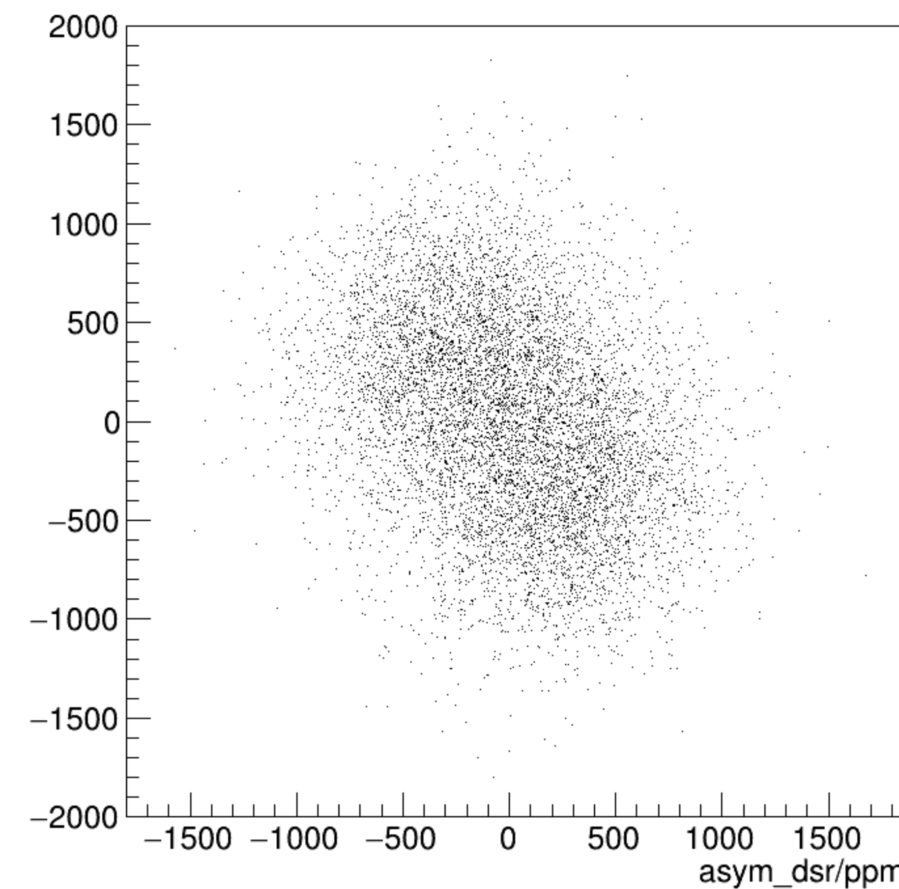
asym_dsl/ppm:asym_dsr/ppm {ok_cut}
