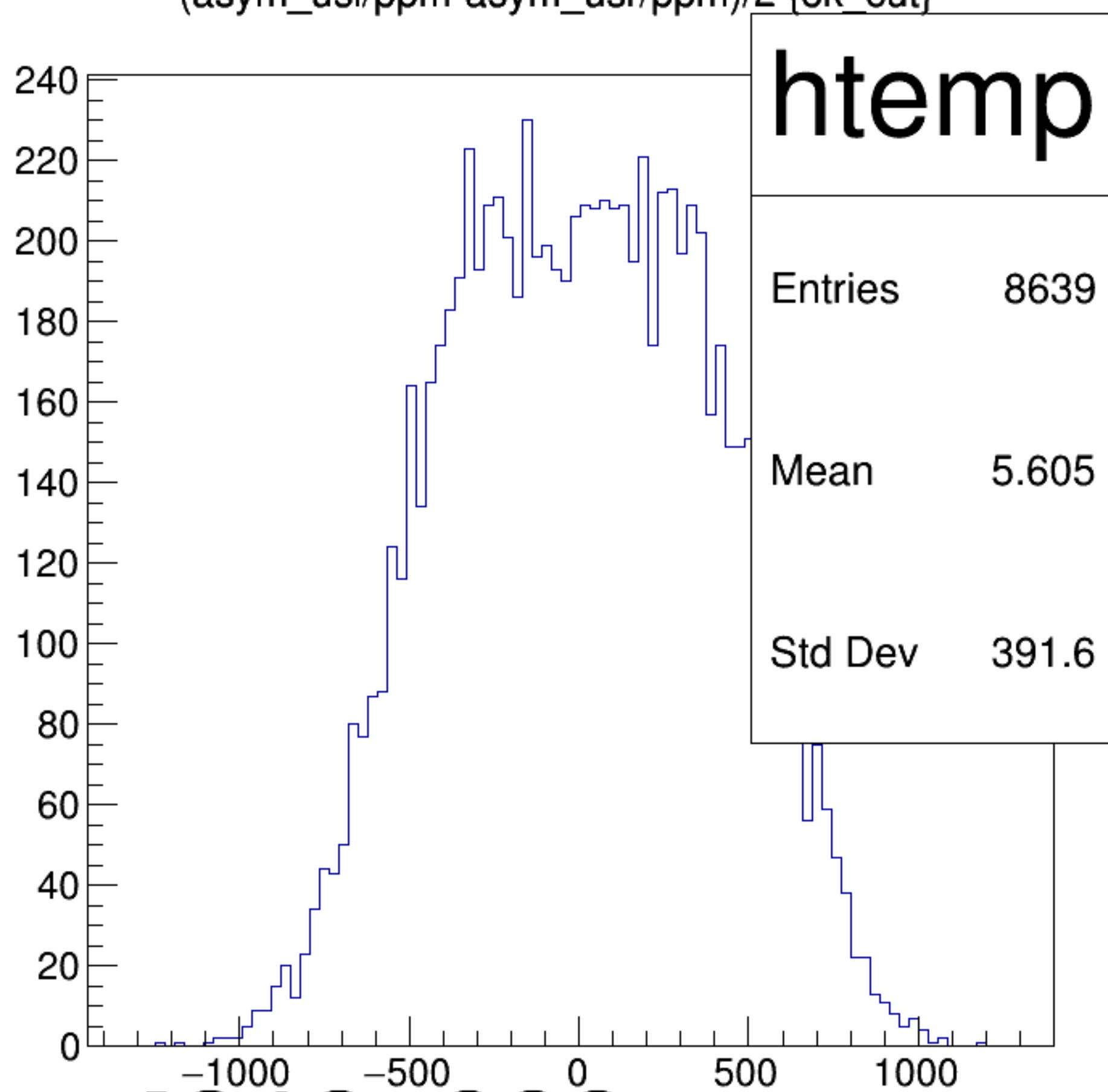
(asym_usl/ppm-asym_usr/ppm)/2 {ok_cut}
