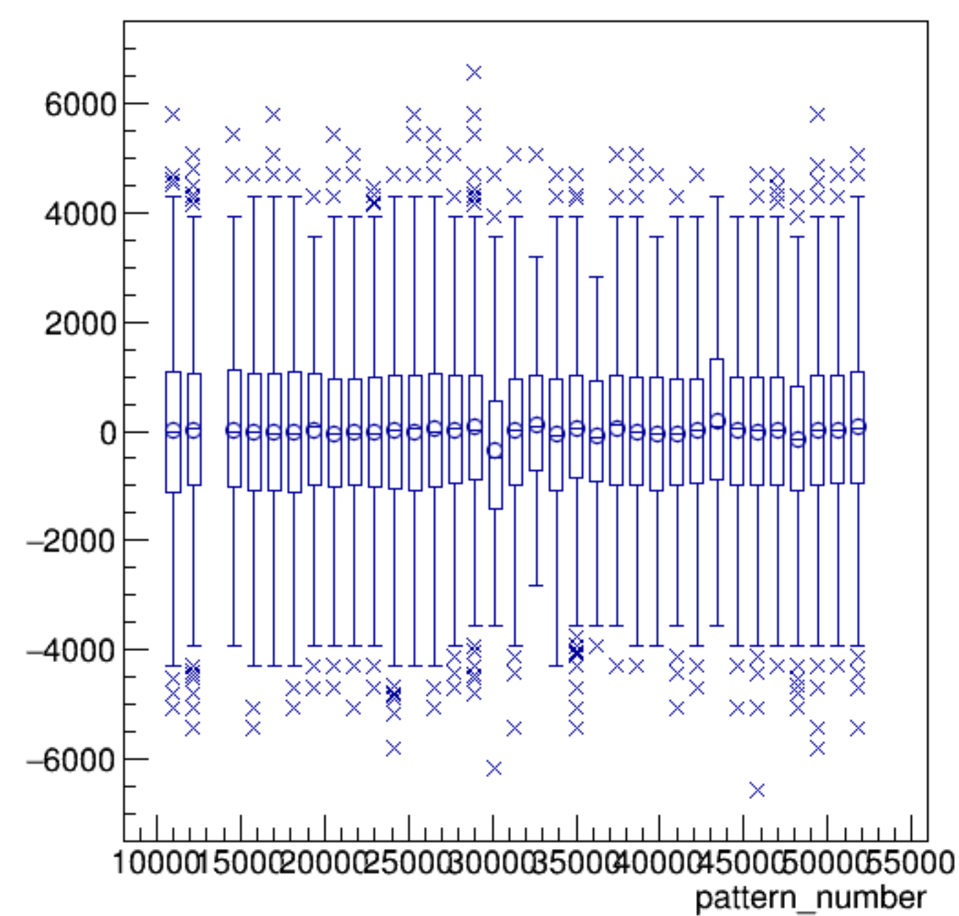
asym_atl1/ppm:pattern_number {ErrorFlag==0}
