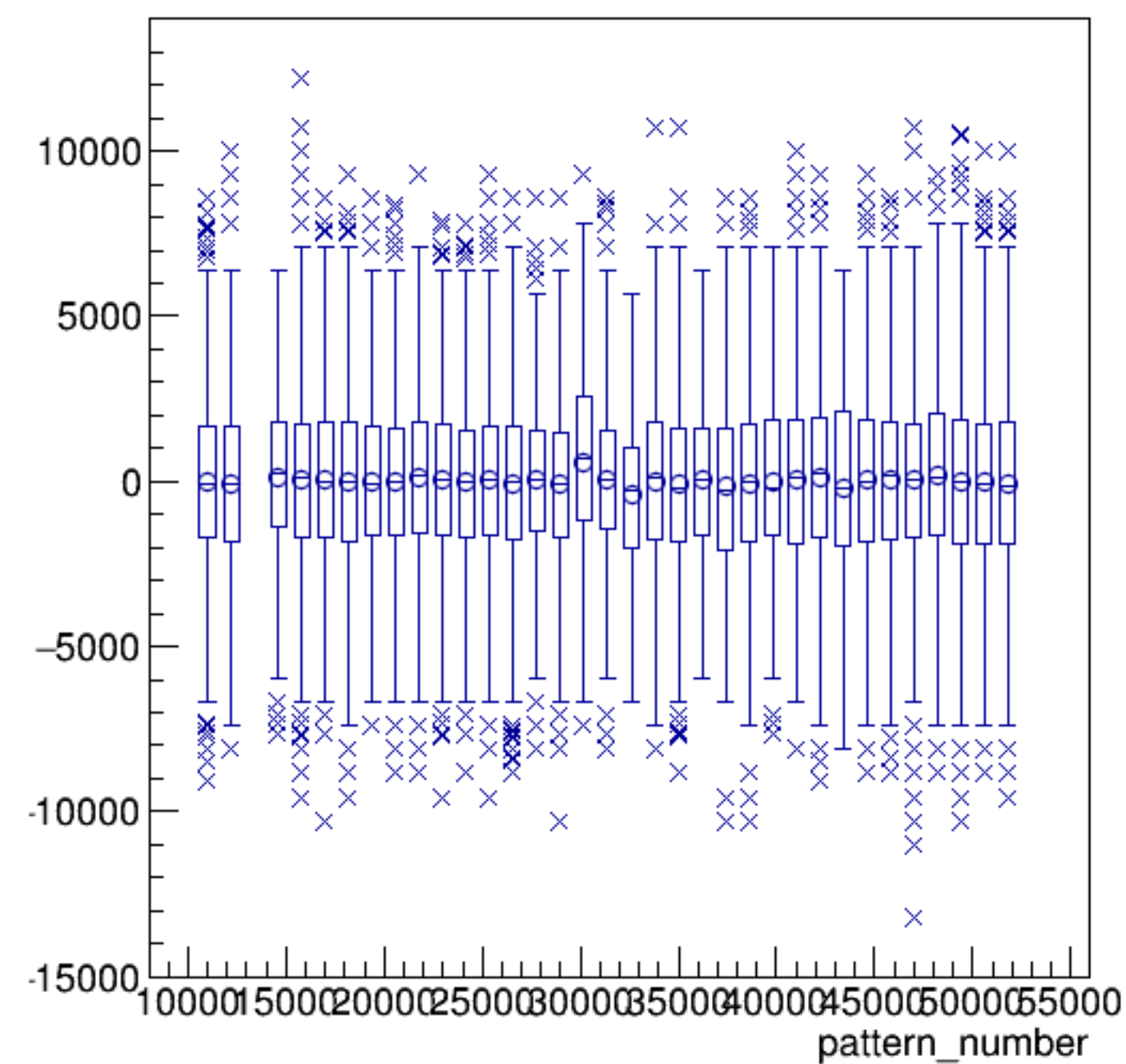
asym_atr2/ppm:pattern_number {ErrorFlag==0}
