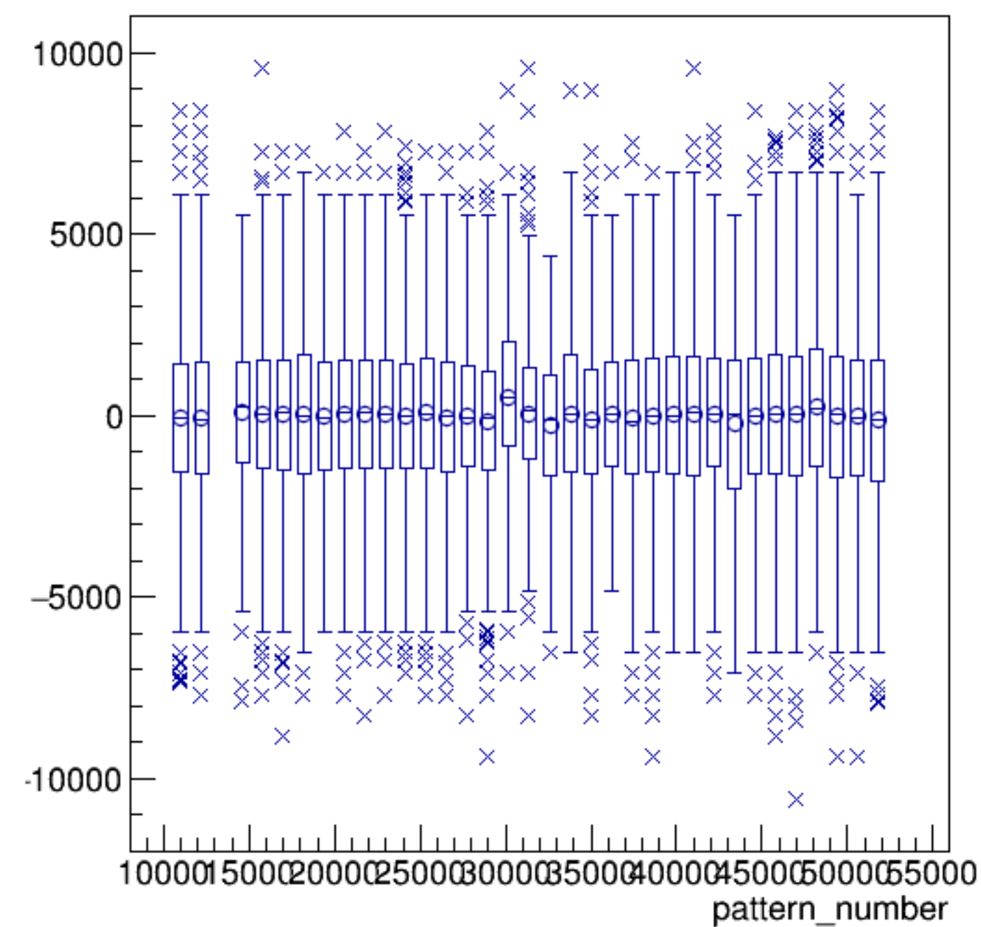
asym_atl2/ppm:pattern_number {ErrorFlag==0}
