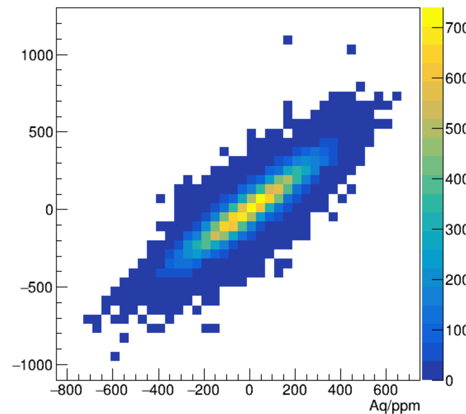
asym_bpm0l01WS/ppm:Aq/ppm {ErrorFlag==0}
