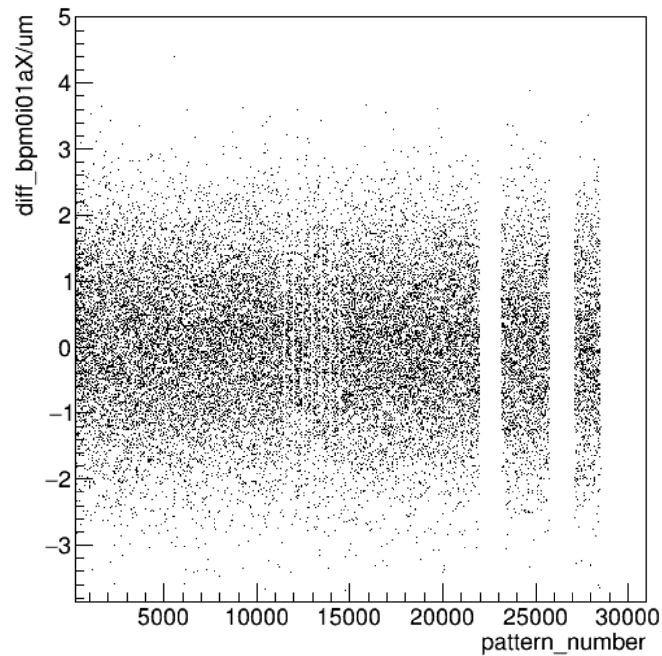
diff_bpm0i01aX/um:pattern_number {ErrorFlag==0}
