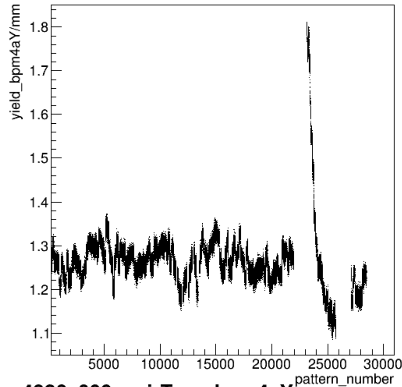
yield_bpm4aY/mm:pattern_number {ErrorFlag==0}
