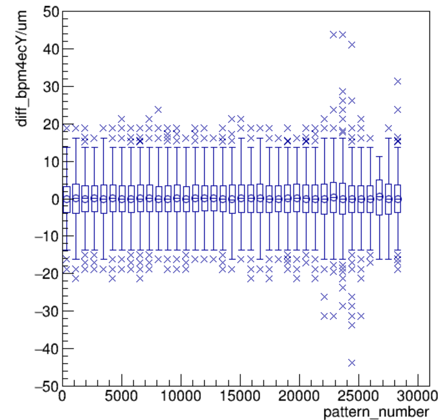
diff_bpm4ecY/um:pattern_number {ErrorFlag==0}
