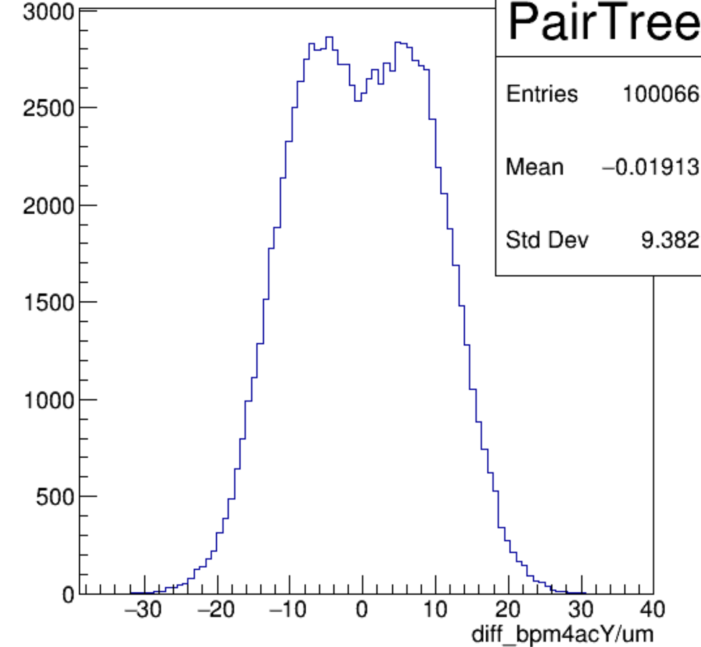
diff_bpm4acY/um {ErrorFlag==0}
