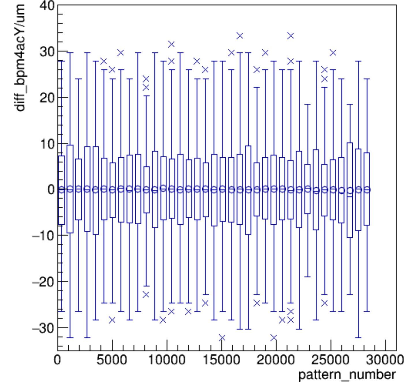
diff_bpm4acY/um:pattern_number {ErrorFlag==0}
