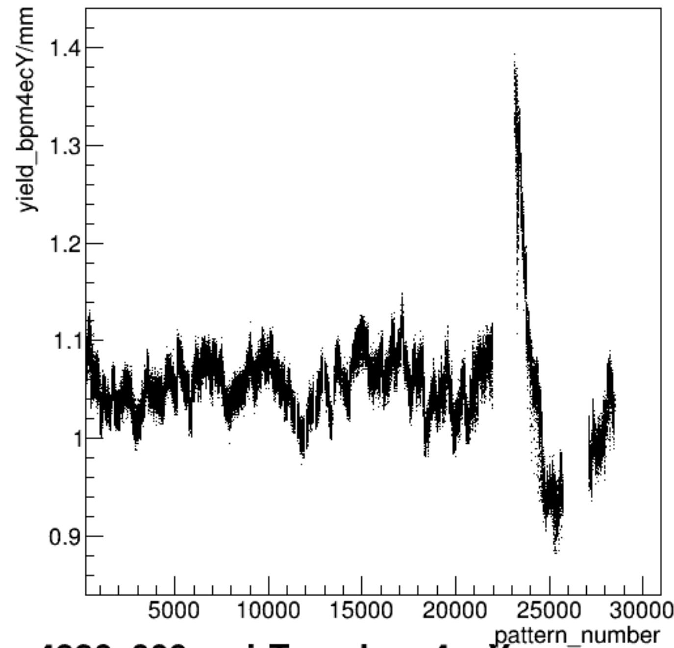
yield_bpm4ecY/mm:pattern_number {ErrorFlag==0}
