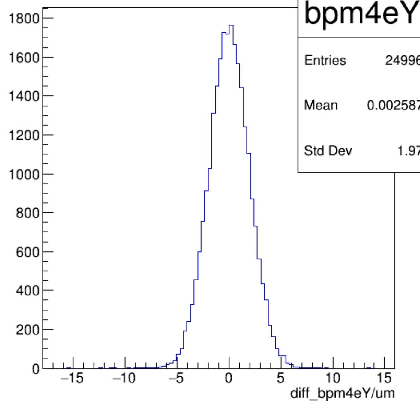
diff_bpm4eY/um {ErrorFlag==0}
