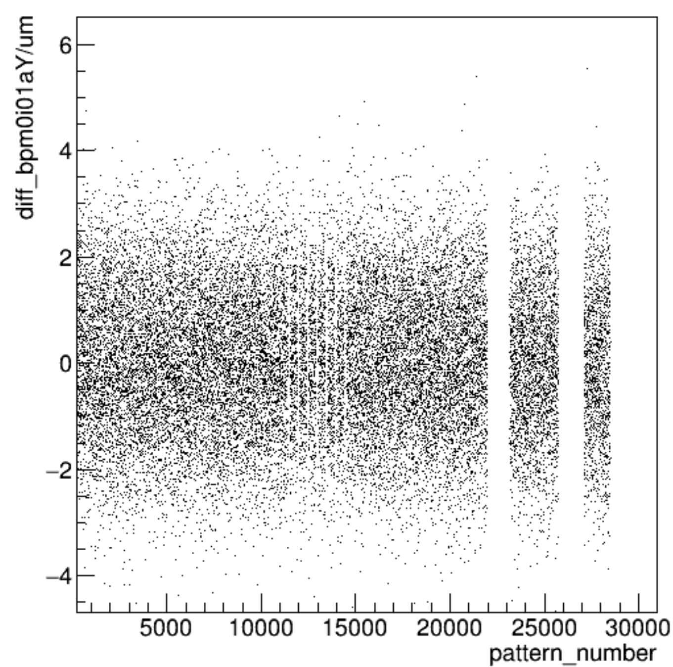
diff_bpm0i01aY/um:pattern_number {ErrorFlag==0}
