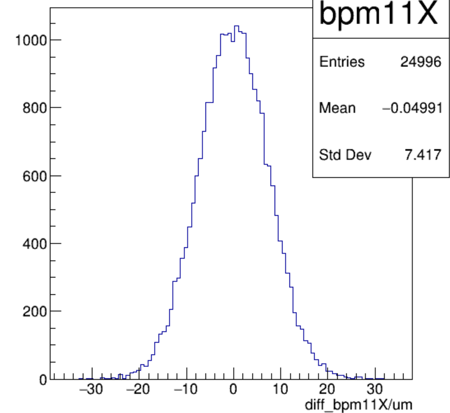
diff_bpm11X/um {ErrorFlag==0}
