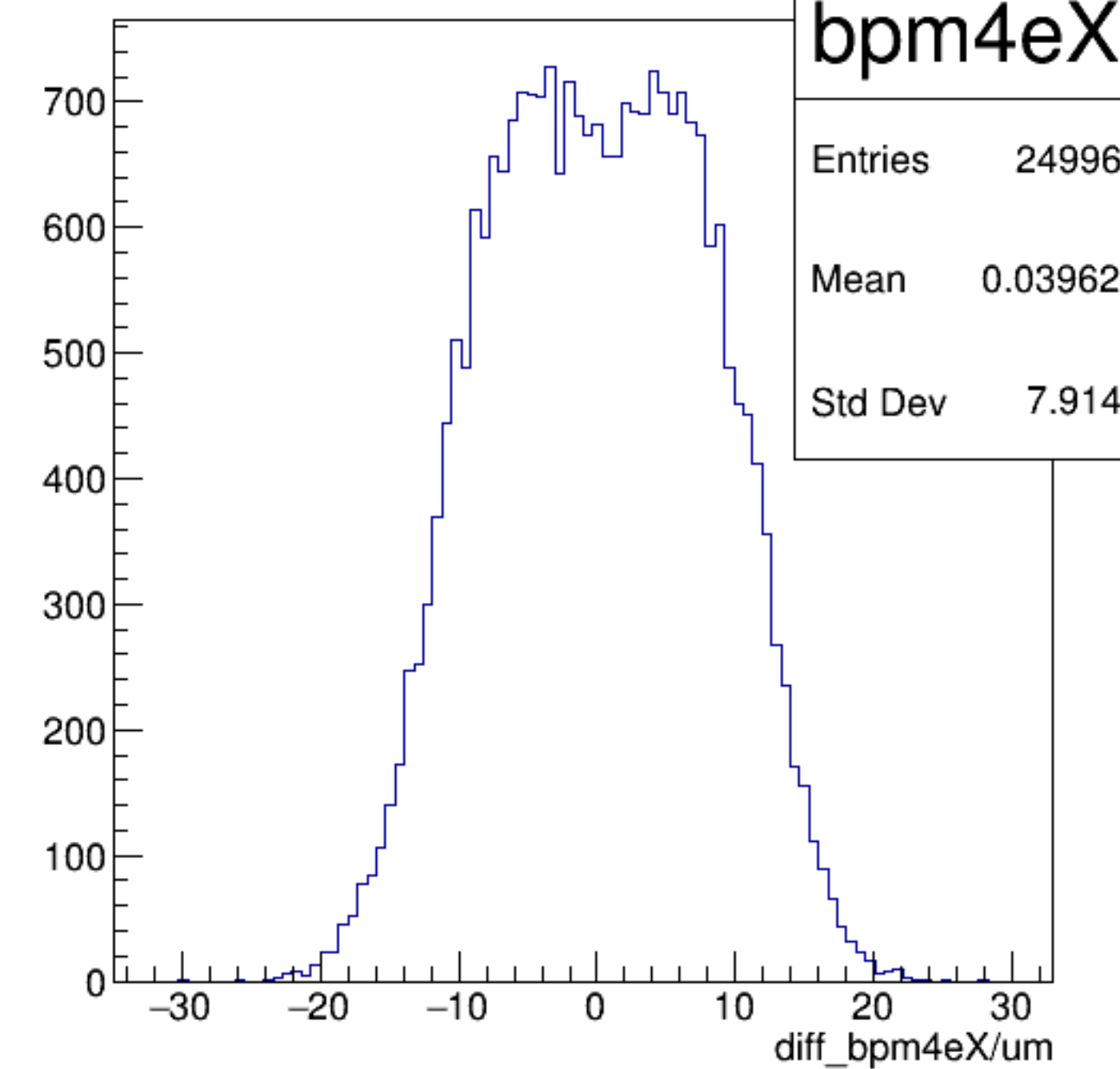
diff_bpm4eX/um {ErrorFlag==0}
