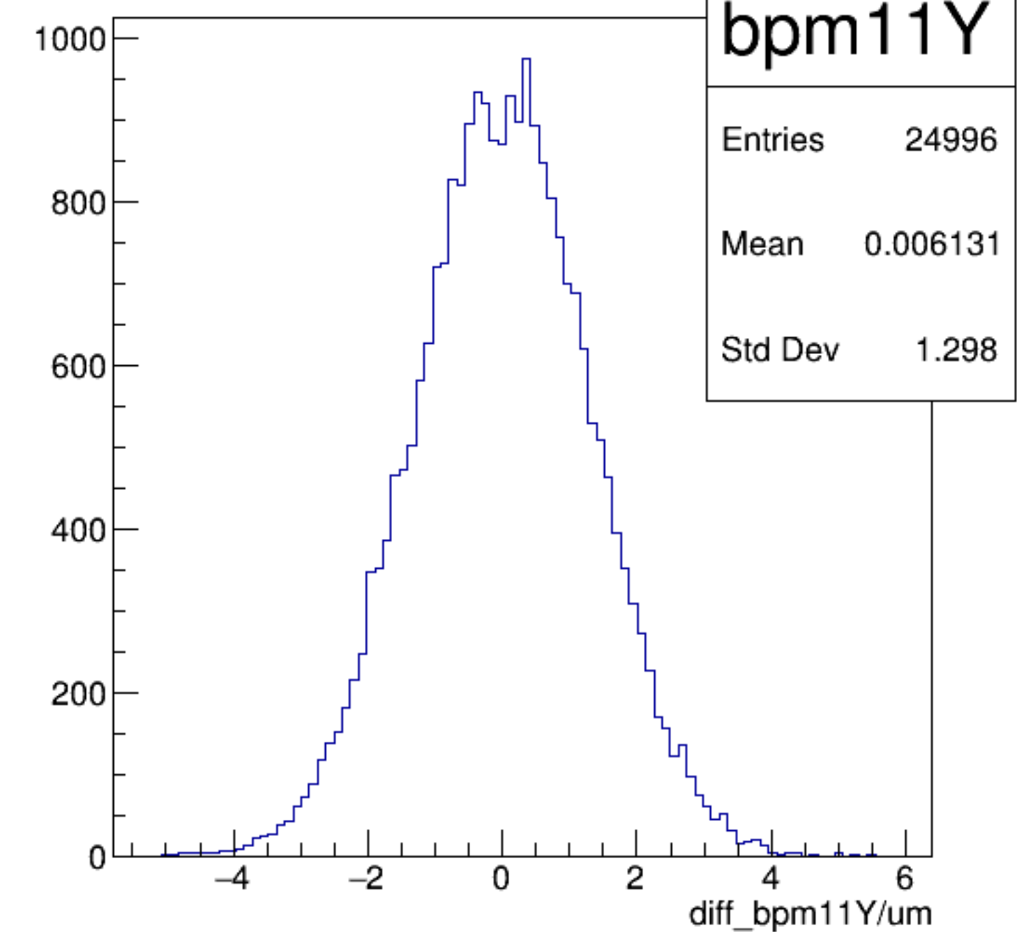
diff_bpm11Y/um {ErrorFlag==0}
