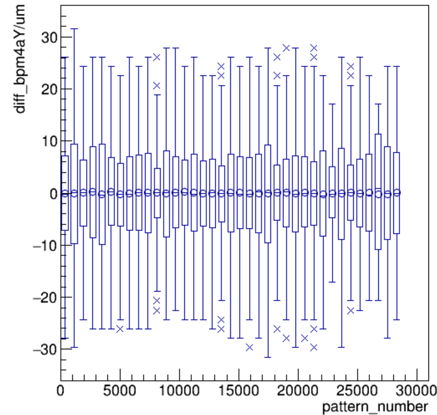
diff_bpm4aY/um:pattern_number {ErrorFlag==0}
