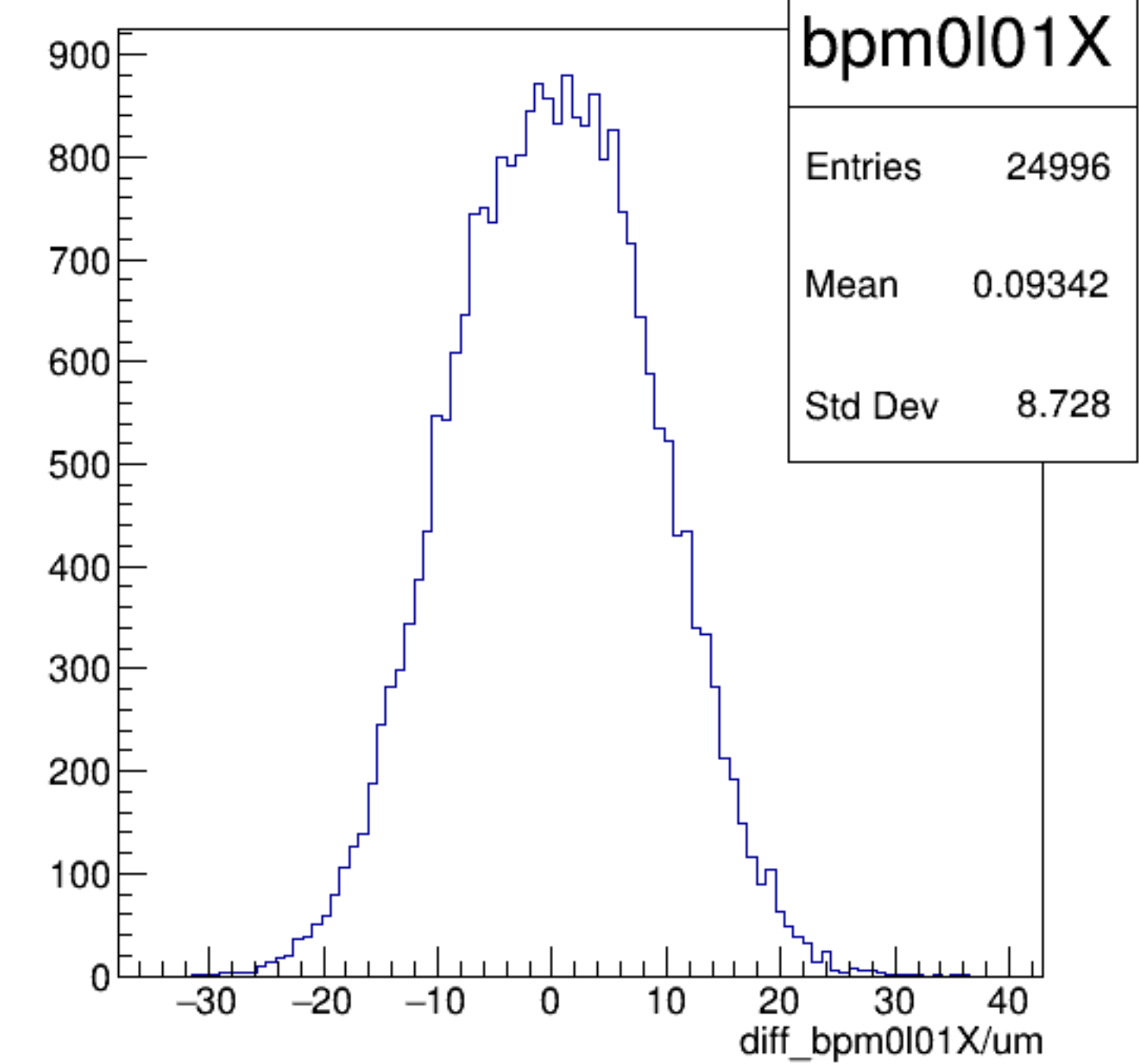
diff_bpm0l01X/um {ErrorFlag==0}
