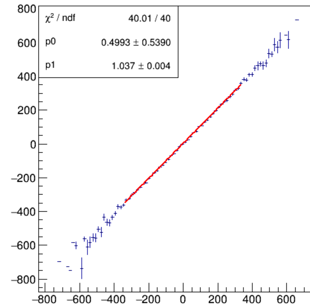
asym_bpm0l01WS/ppm:Aq/ppm {ErrorFlag==0}
