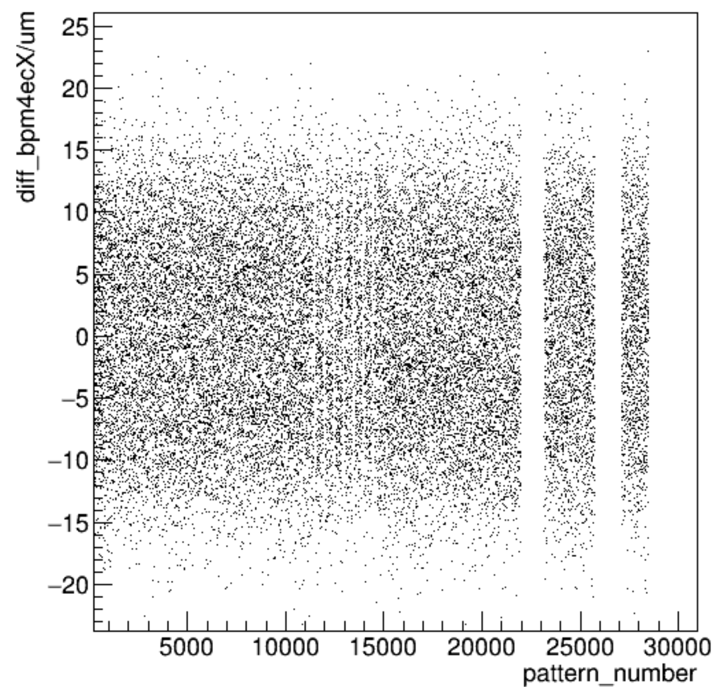
diff_bpm4ecX/um:pattern_number {ErrorFlag==0}
