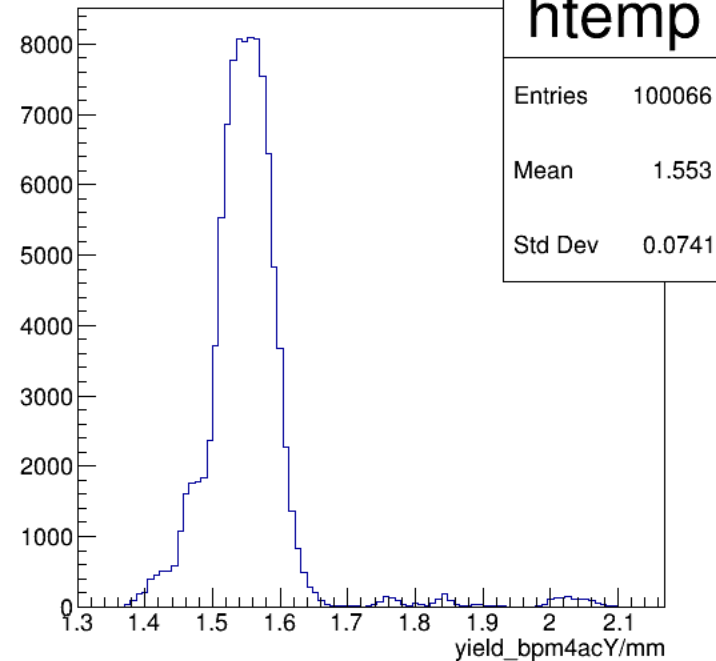
yield_bpm4acY/mm {ErrorFlag==0}
