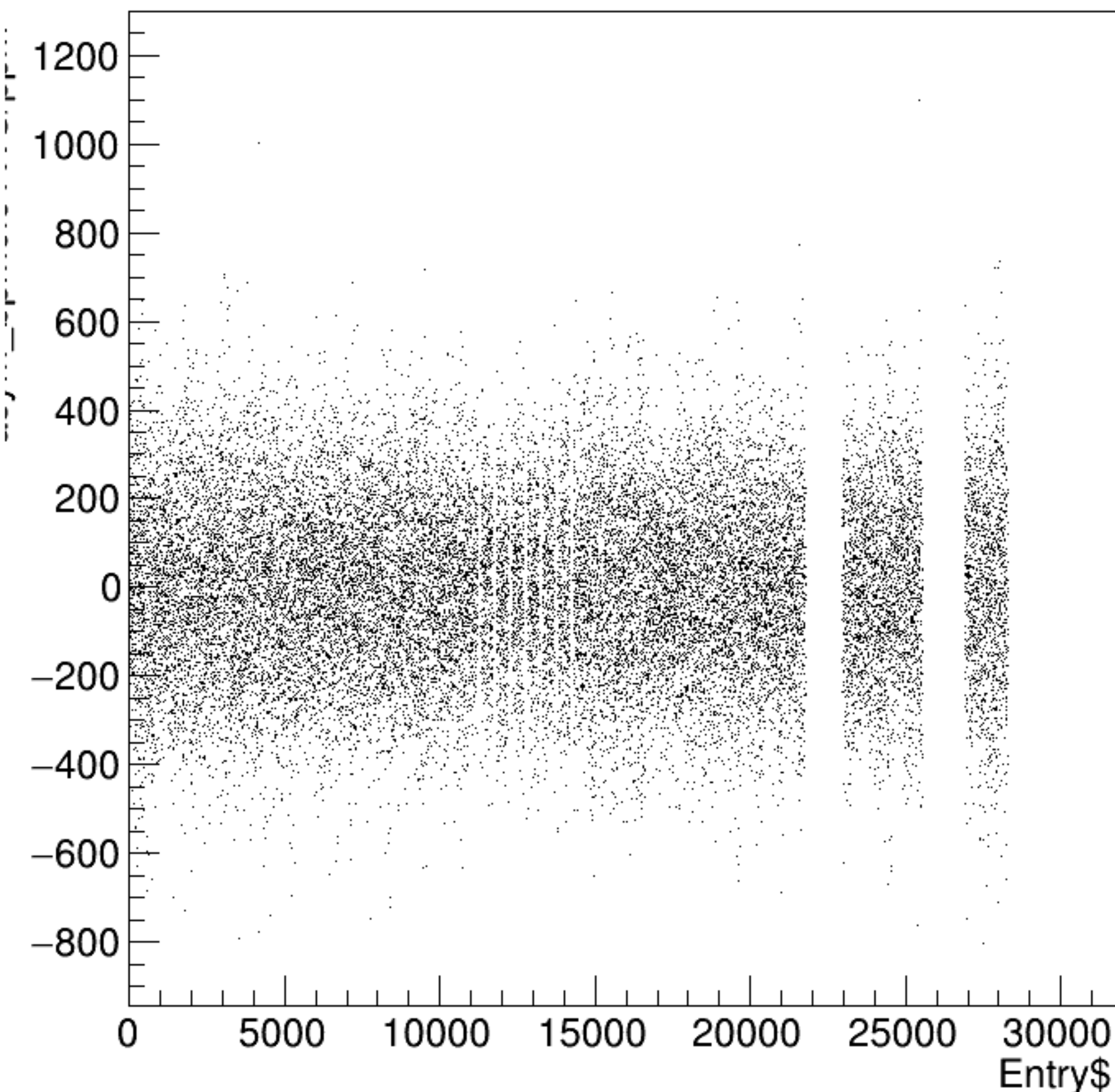
asym_bpm0l01WS/ppm:Entry$ {ErrorFlag==0}
