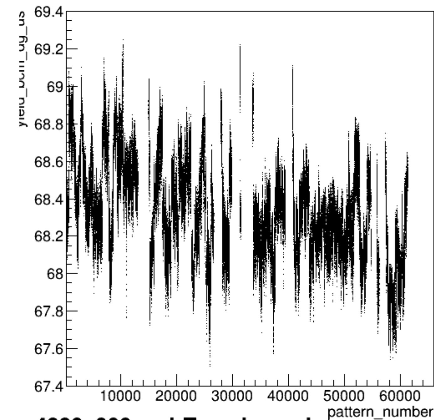
yield_bcm_dg_us:pattern_number {ErrorFlag==0}
