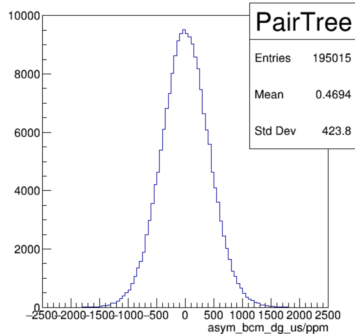
asym_bcm_dg_us/ppm {ErrorFlag==0}
