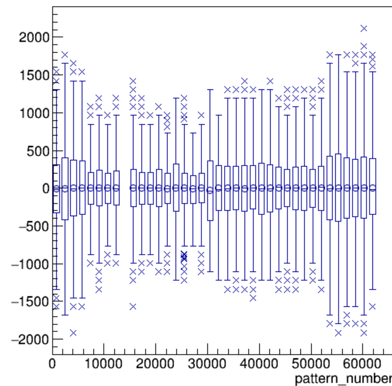
asym_bcm_dg_ds/ppm:pattern_number {ErrorFlag==0}
