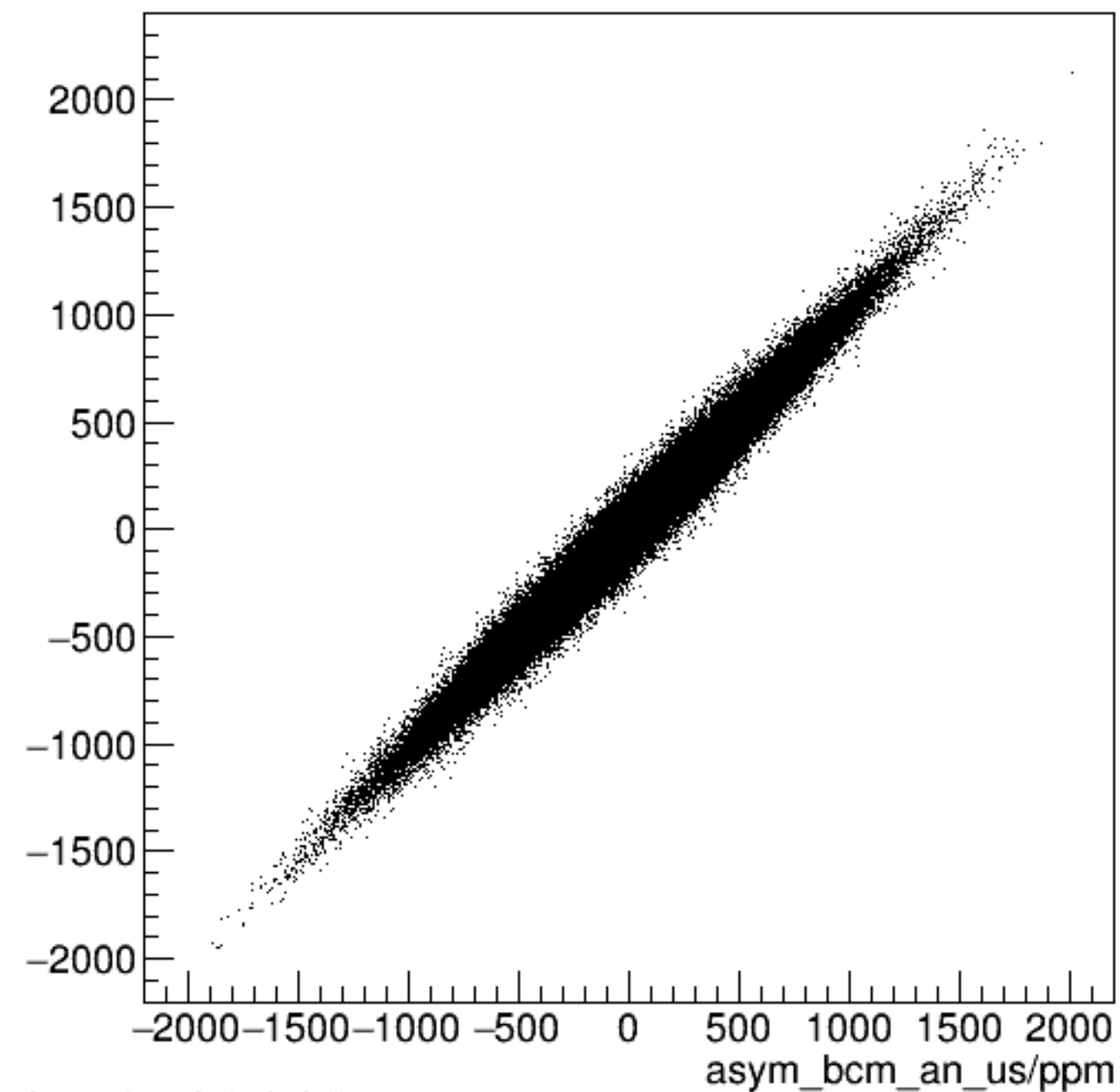
run4339_000_asym_bcm_dg_ds_vs_asym_bcm_an_us_pr.png
