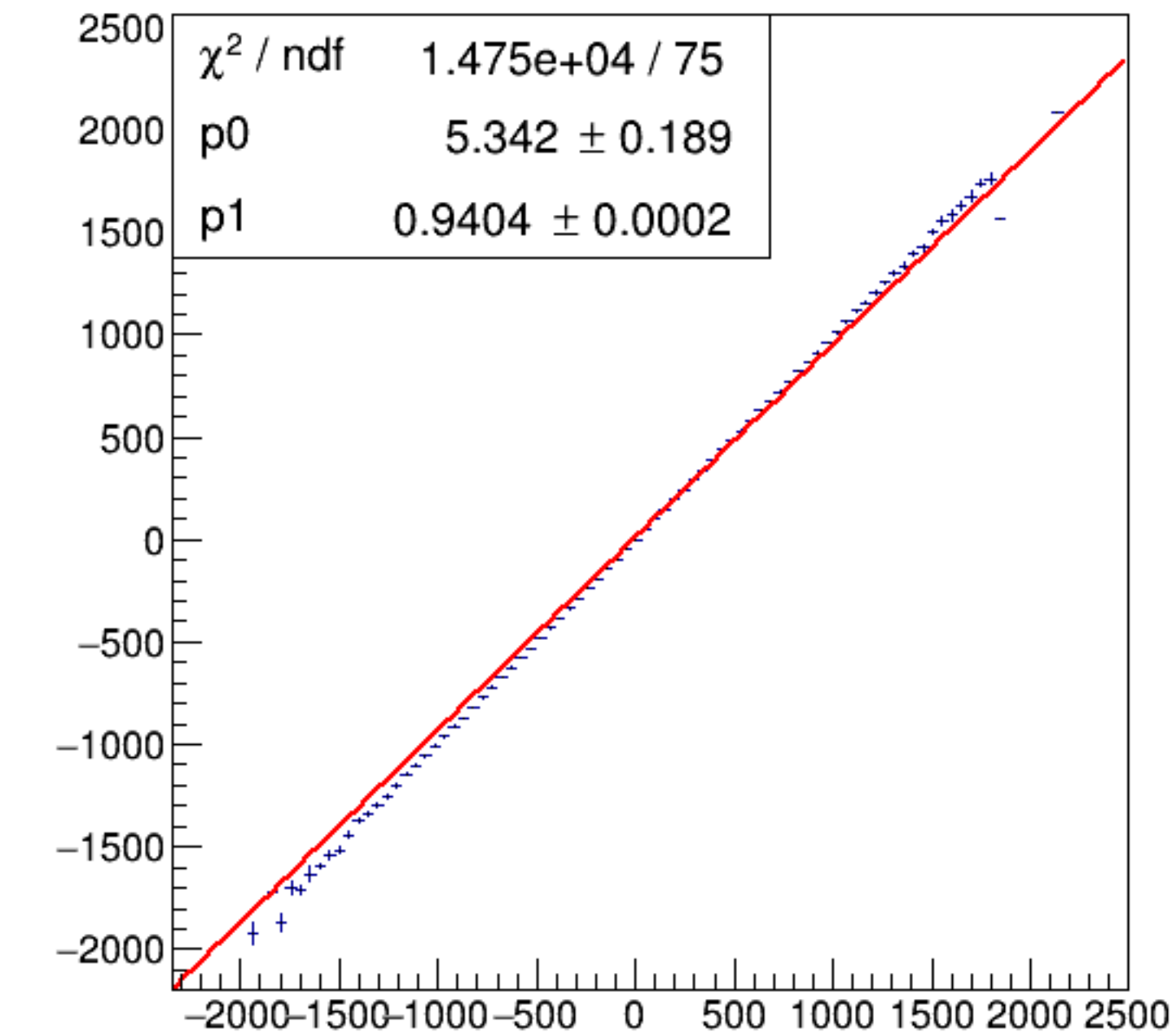
run4339_000_asym_bcm_dg_us_vs_asym_bcm_dg_ds_pr.png
