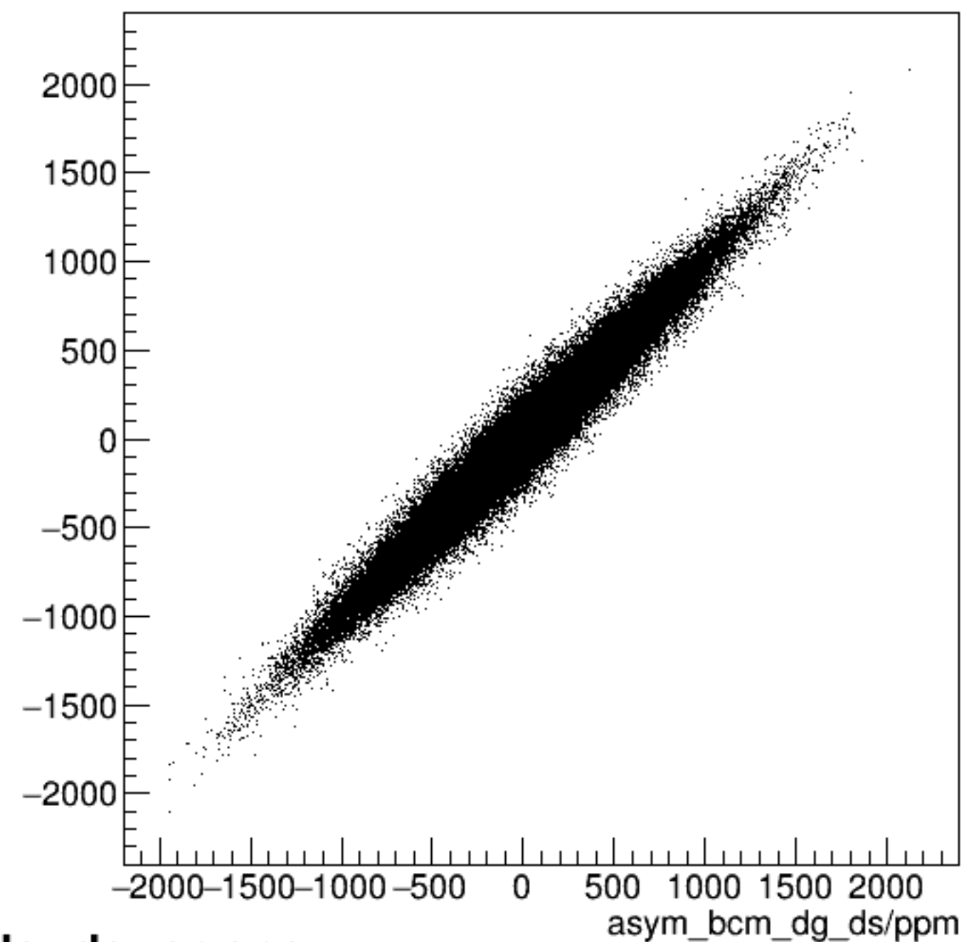
run4339_000_asym_bcm_dg_us_vs_asym_bcm_dg_ds_pr.png
