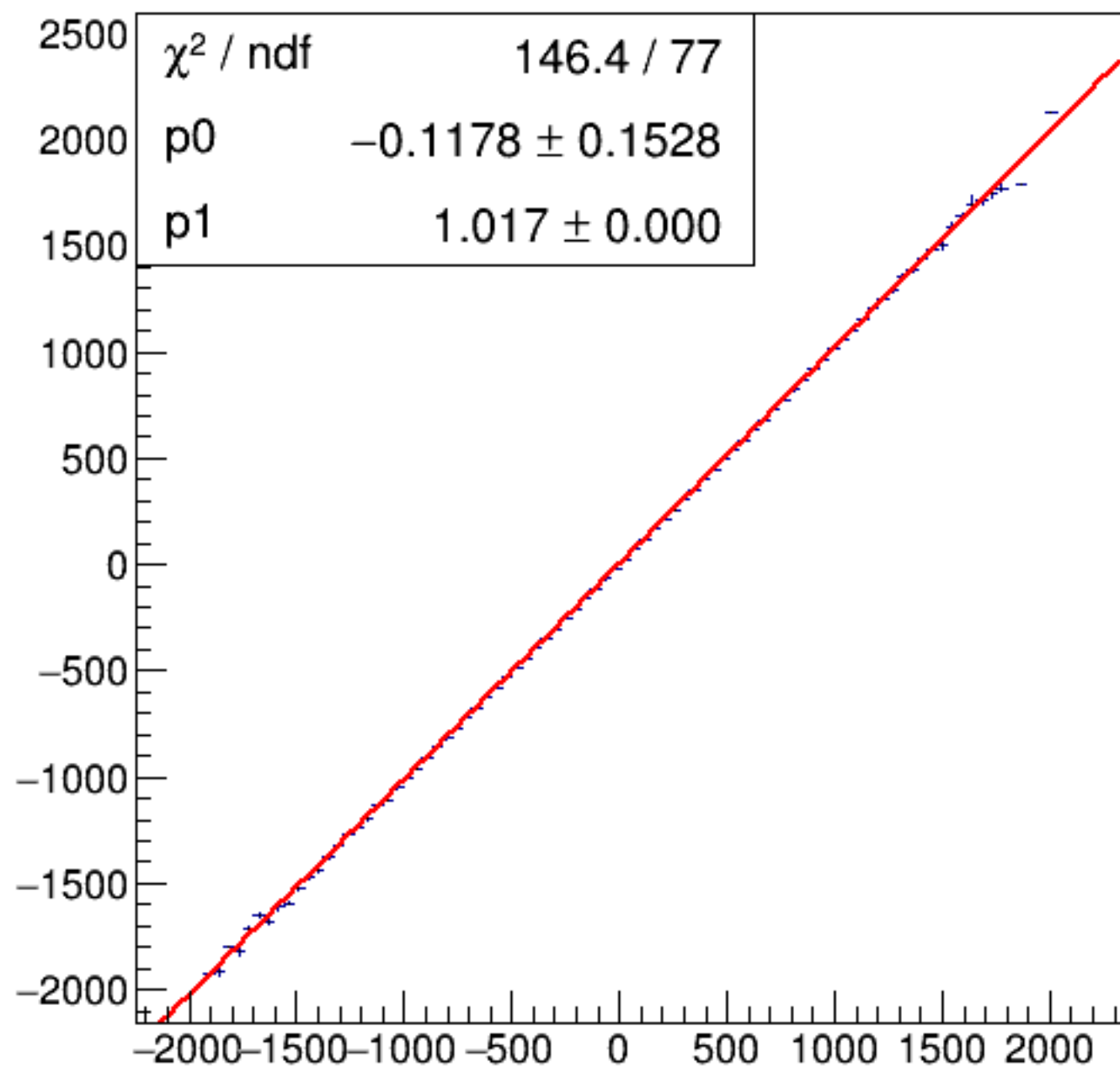
run4339_000_asym_bcm_dg_ds_vs_asym_bcm_an_us_pr.png
