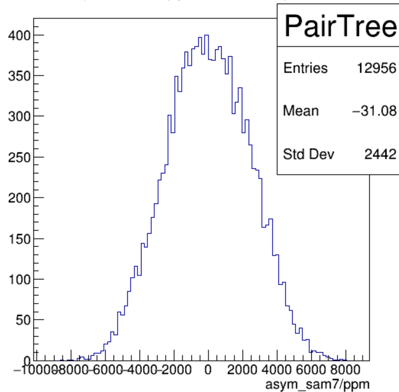
asym_sam7/ppm {ErrorFlag==0}
