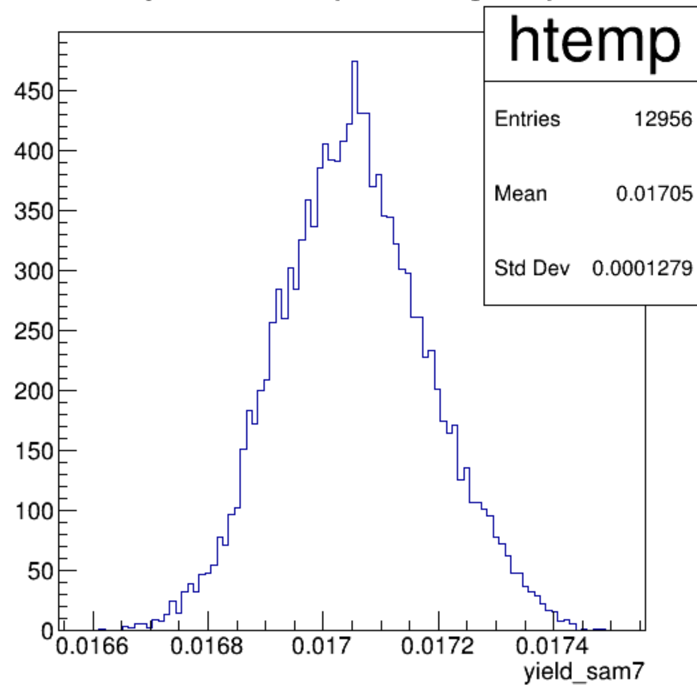
yield_sam7 {ErrorFlag==0}
