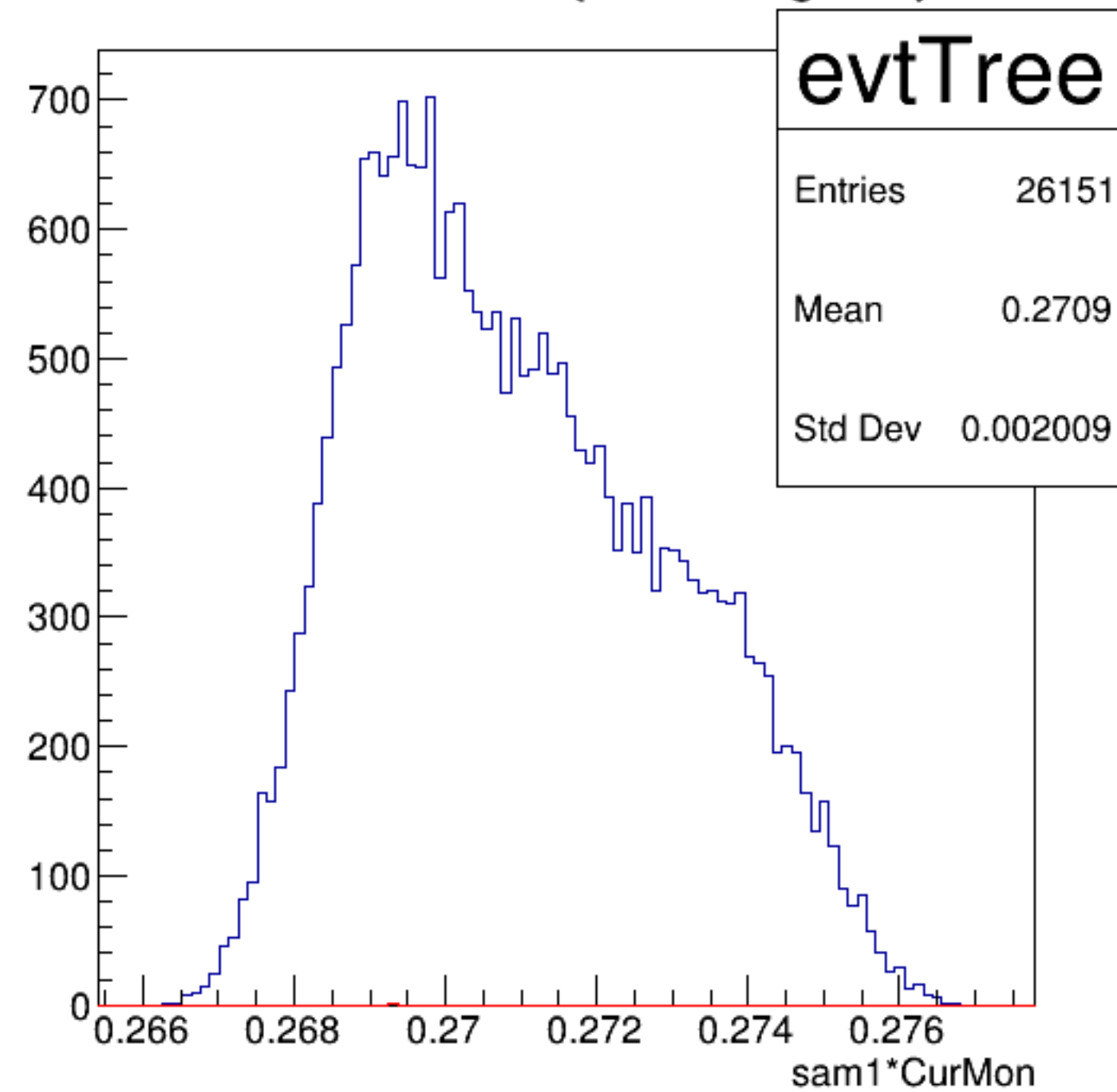
sam1*CurMon {ErrorFlag==0}
