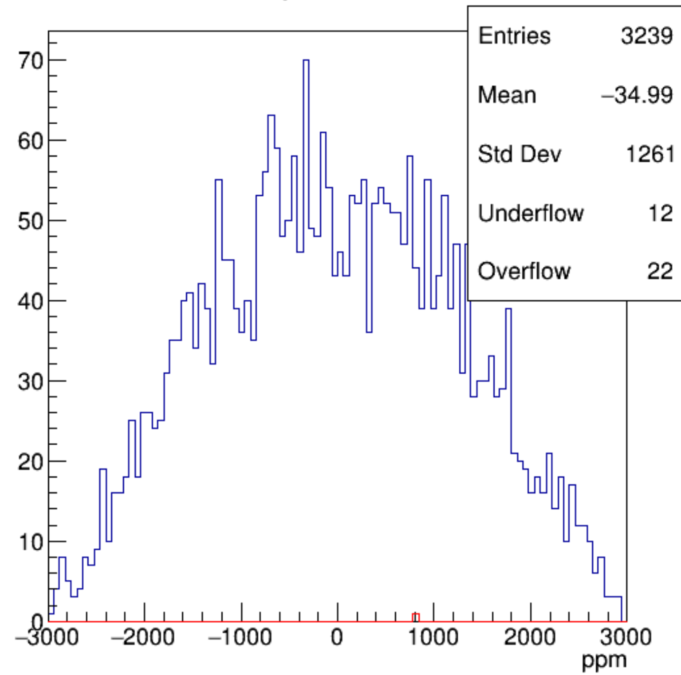
asym_sam8
