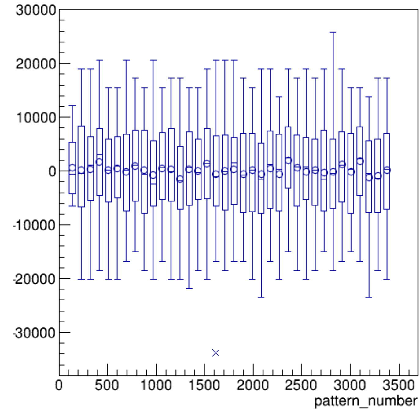
asym_sam3/ppm:pattern_number {ErrorFlag==0}
