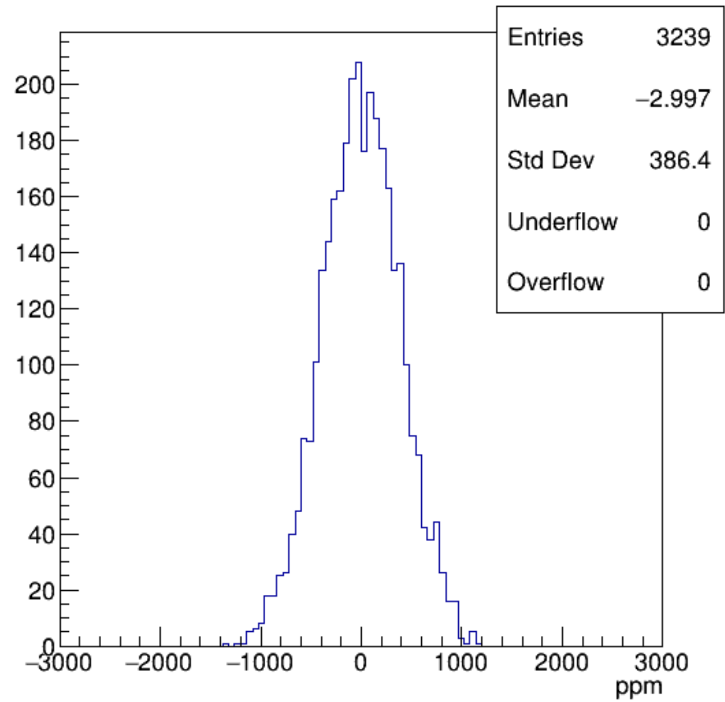
asym_sam5
