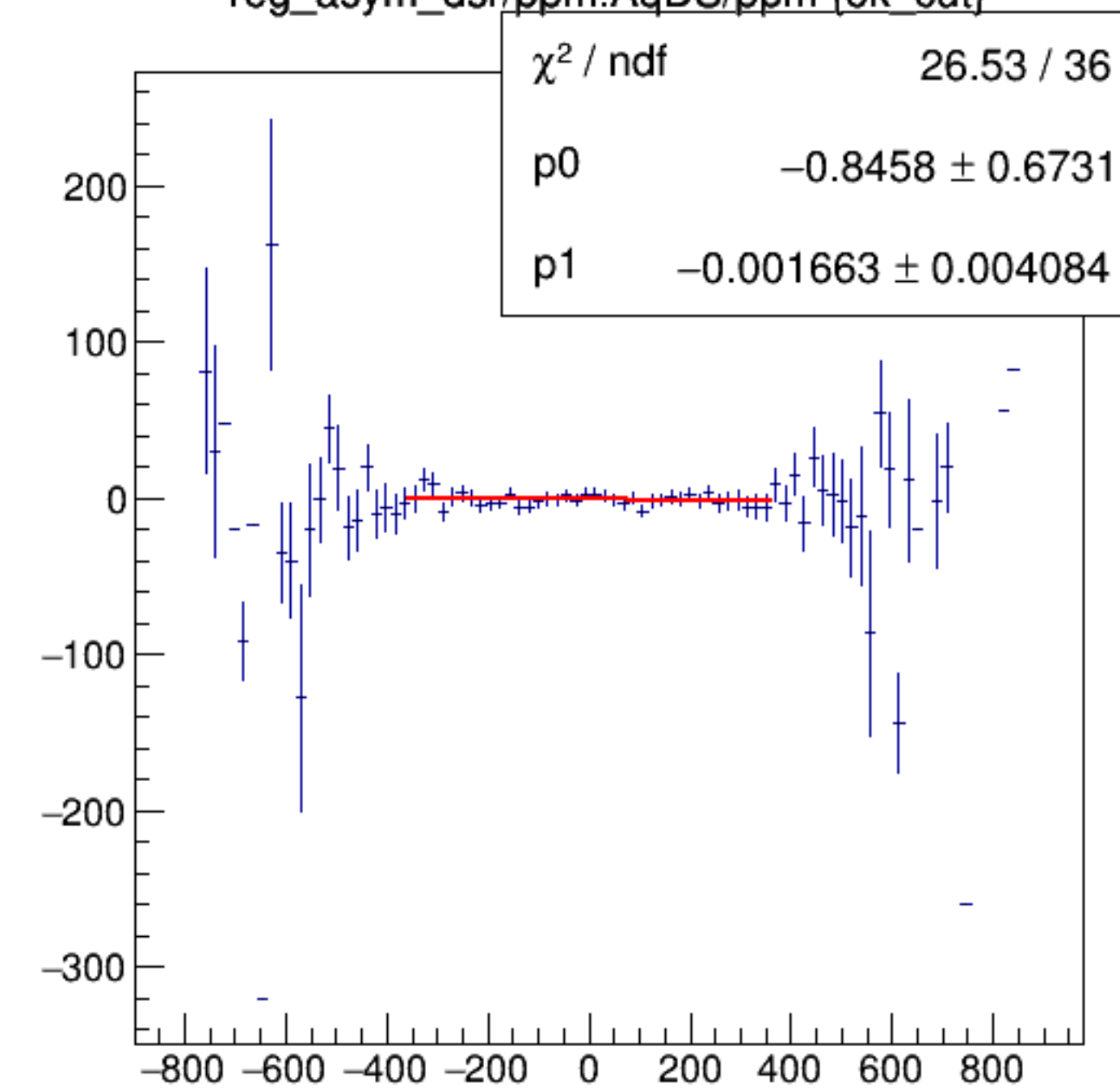
reg_asym_dsr/ppm:AqDS/ppm {ok_cut}
