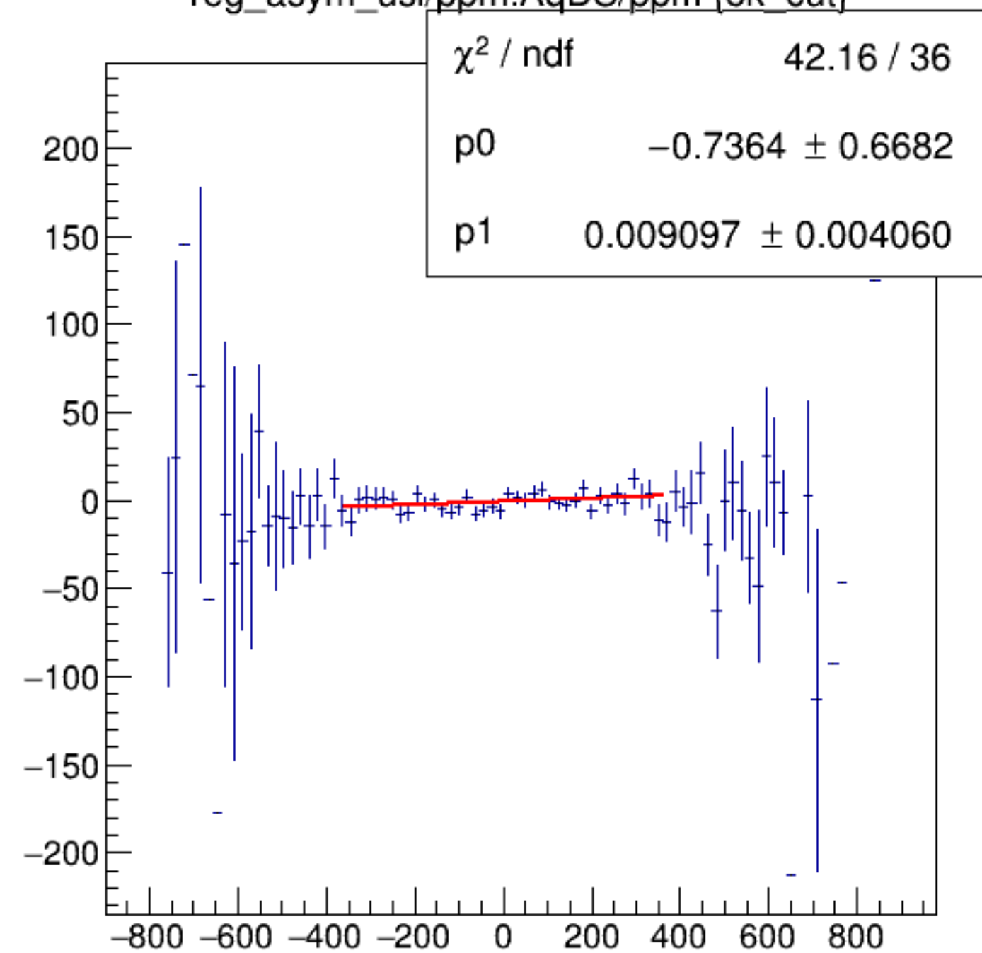
reg_asym_usl/ppm:AqDS/ppm {ok_cut}
