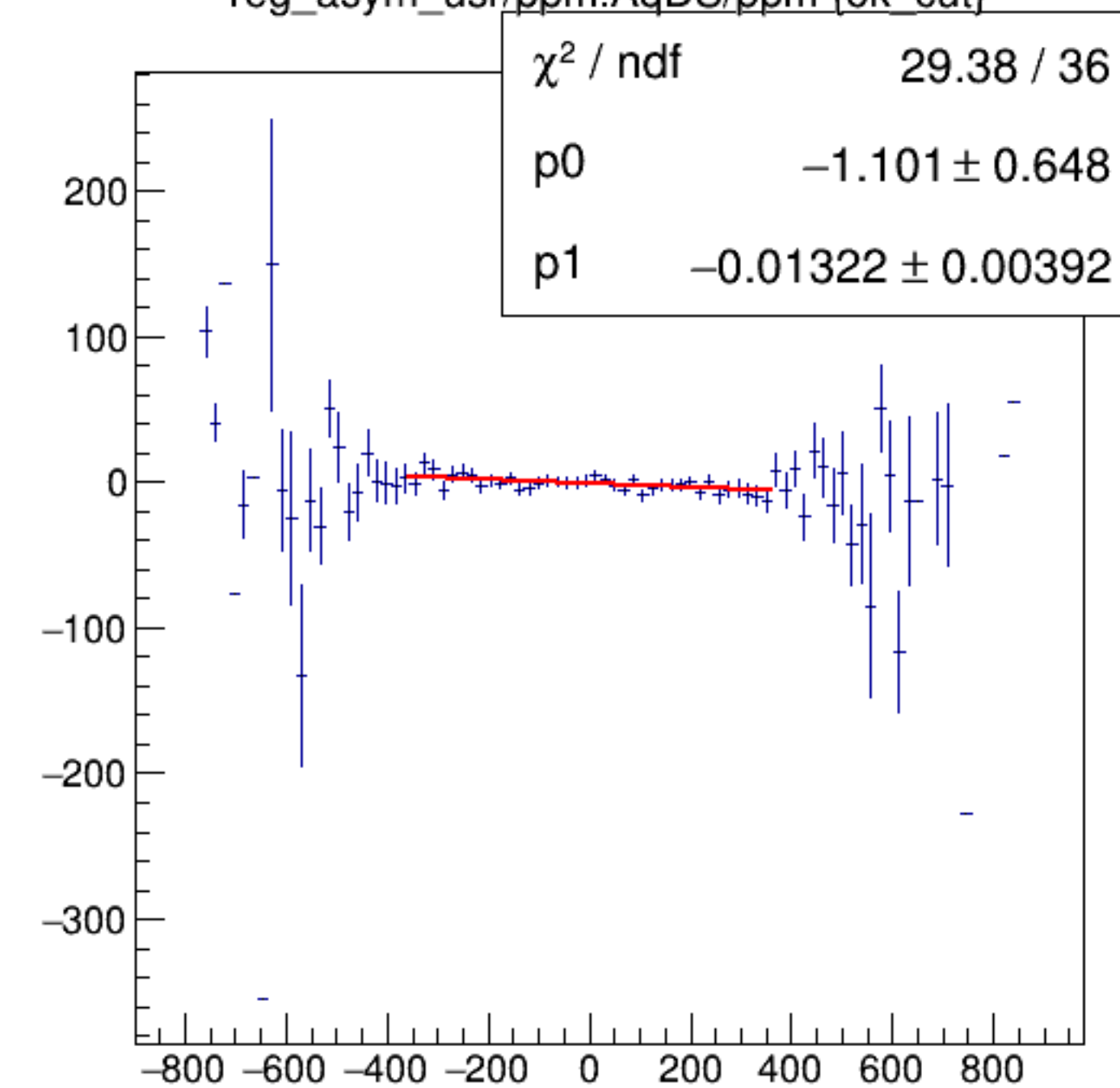
reg_asym_usr/ppm:AqDS/ppm {ok_cut}
