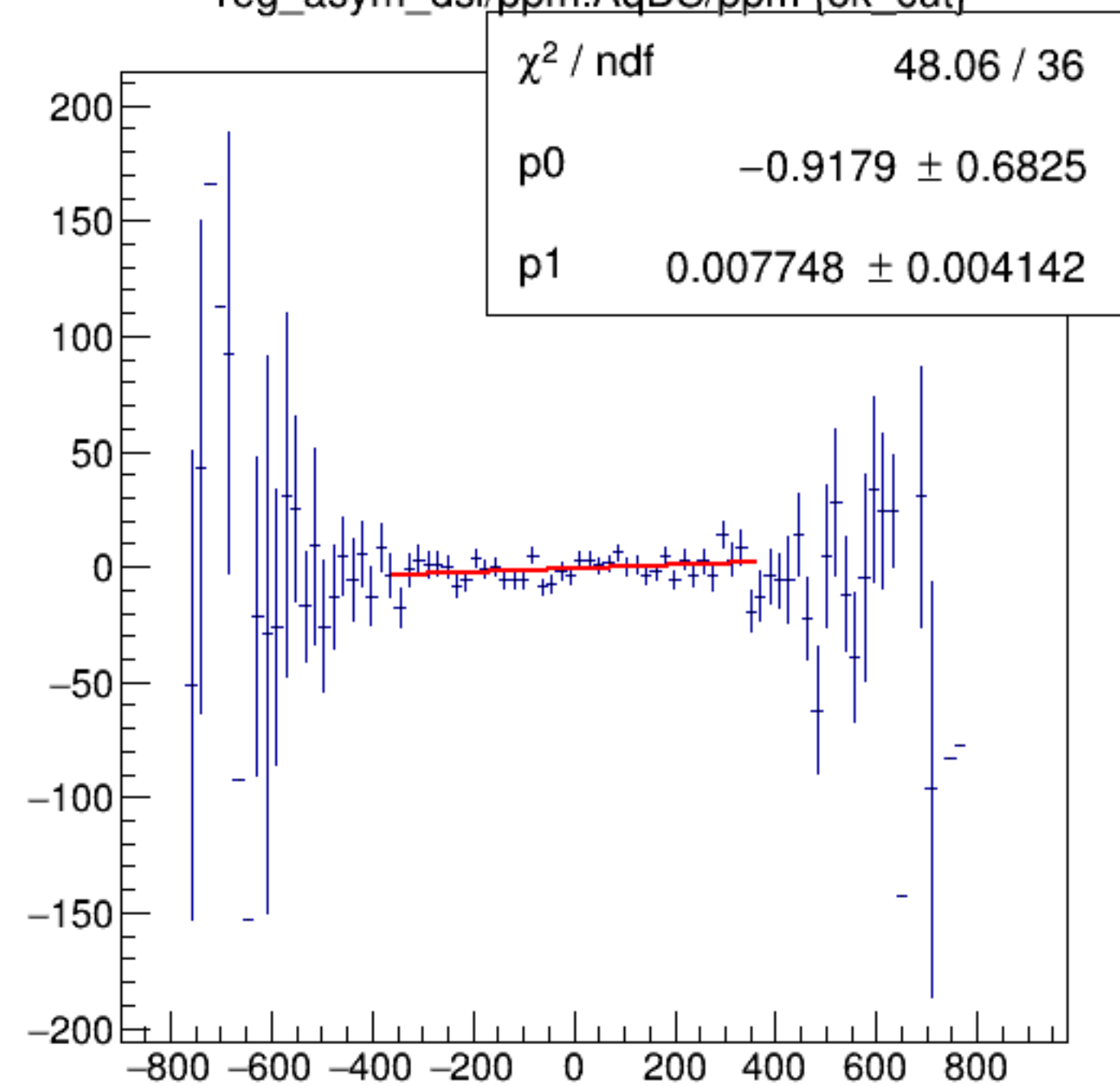
reg_asym_dsl/ppm:AqDS/ppm {ok_cut}
