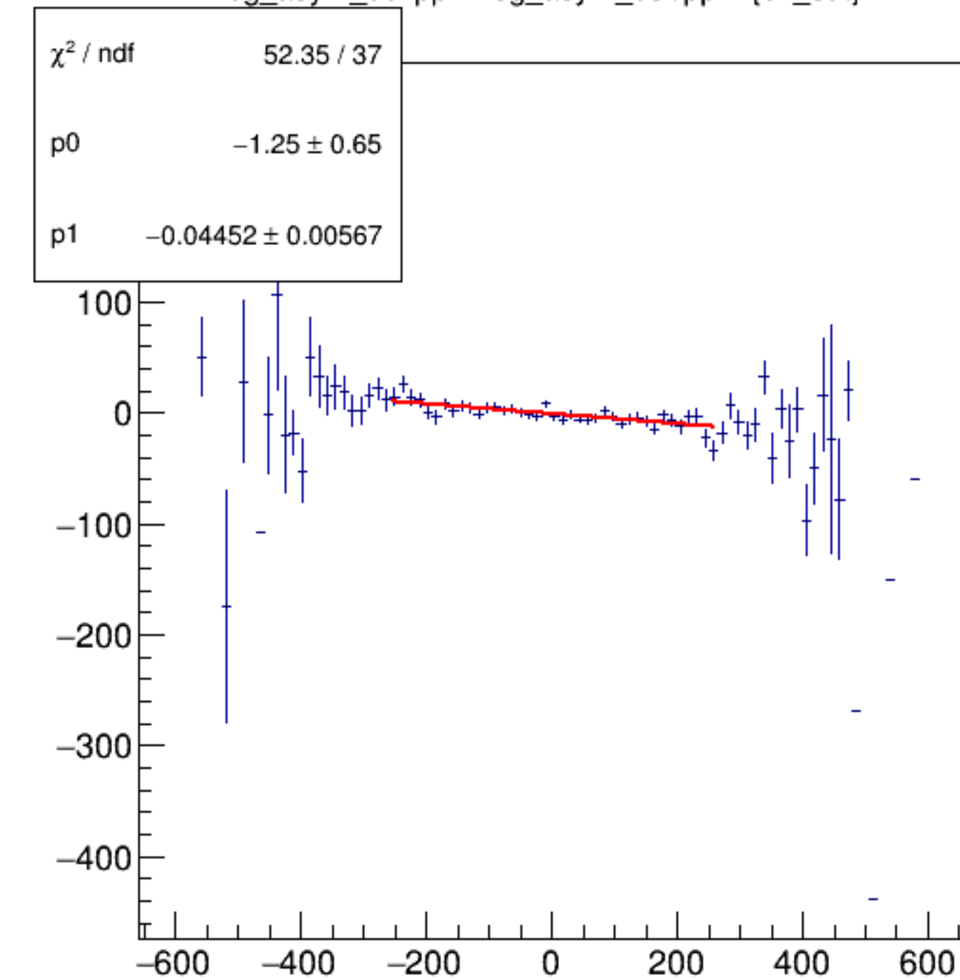
reg_asym_usl/ppm:reg_asym_usr/ppm {ok_cut}
