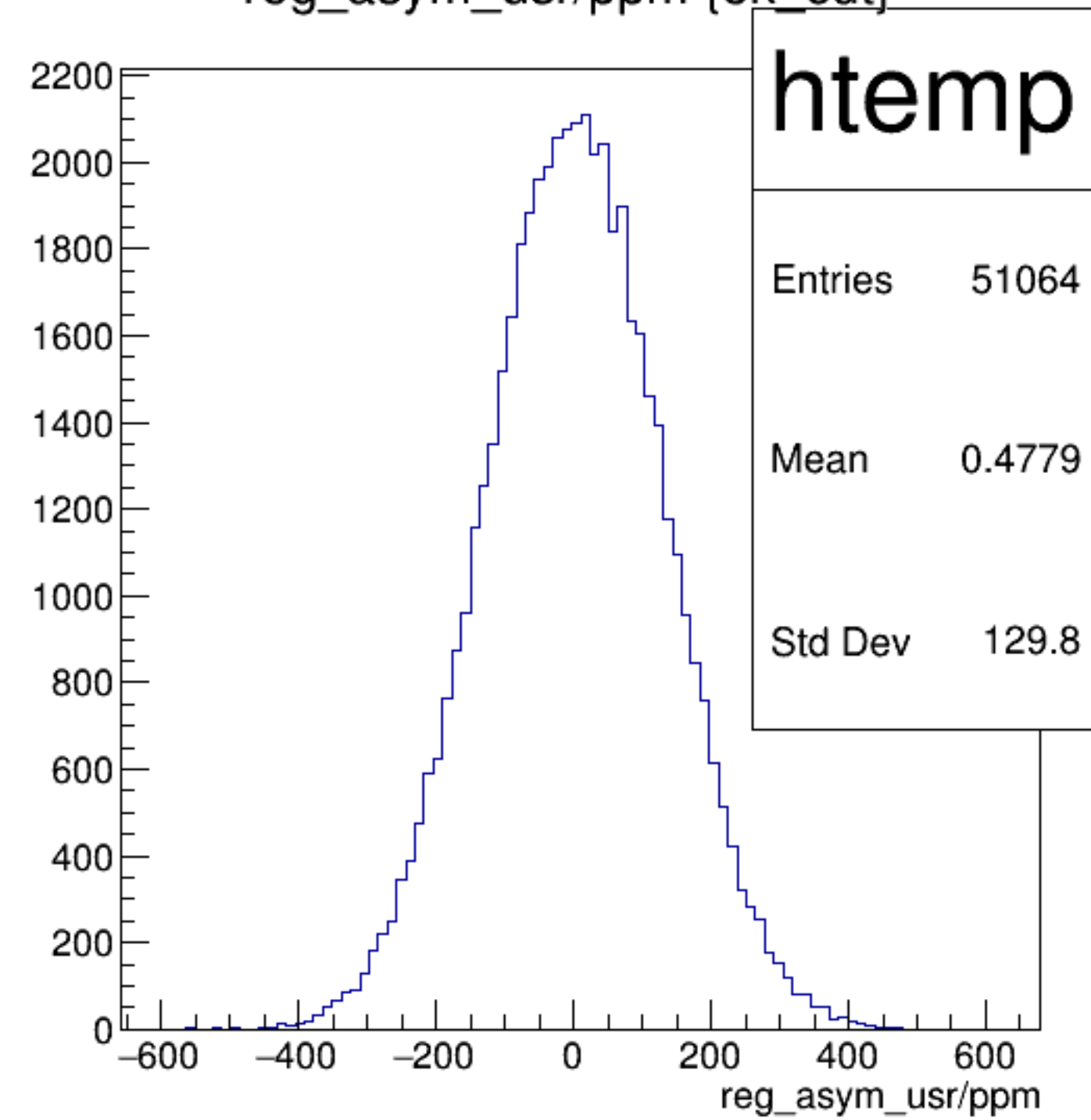
reg_asym_usr/ppm {ok_cut}
