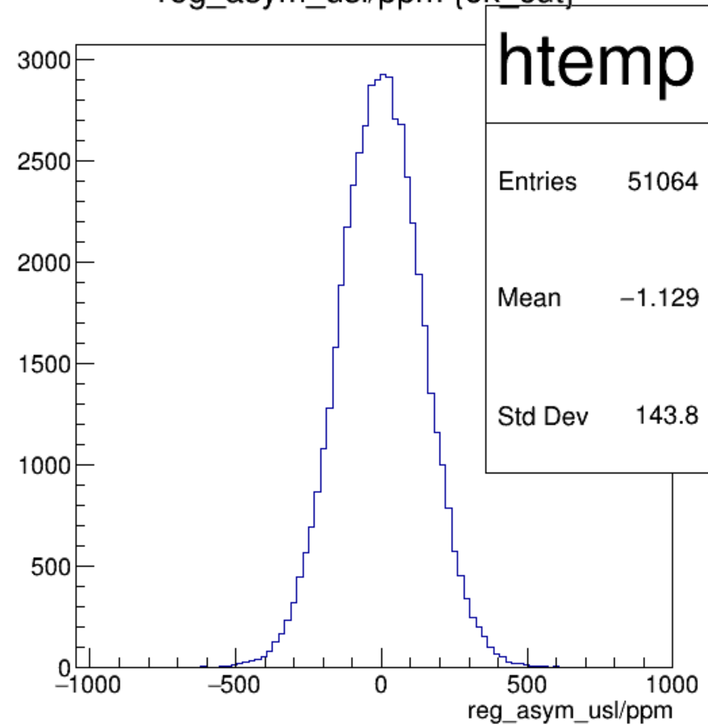
reg_asym_usl/ppm {ok_cut}
