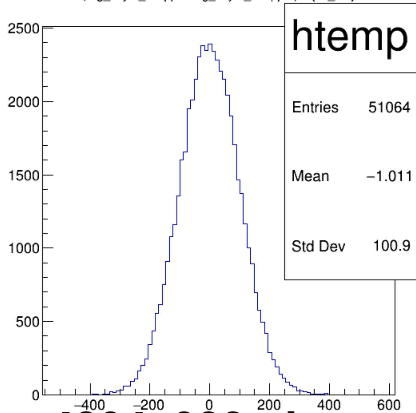
(reg_asym_dsl/ppm-reg_asym_dsr/ppm)/2 {ok_cut}
