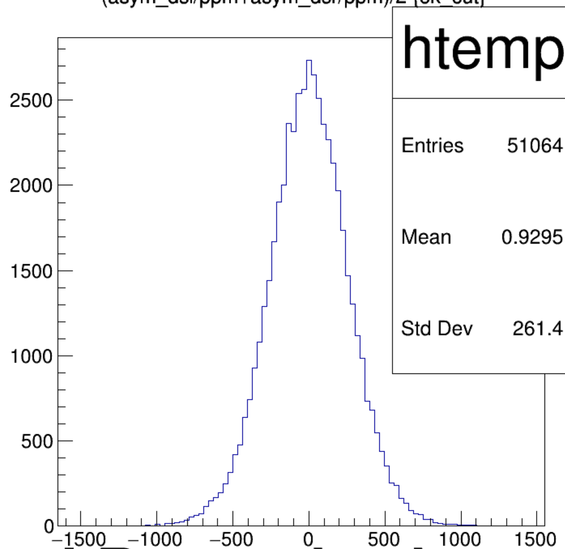
(asym_dsl/ppm+asym_dsr/ppm)/2 {ok_cut}
