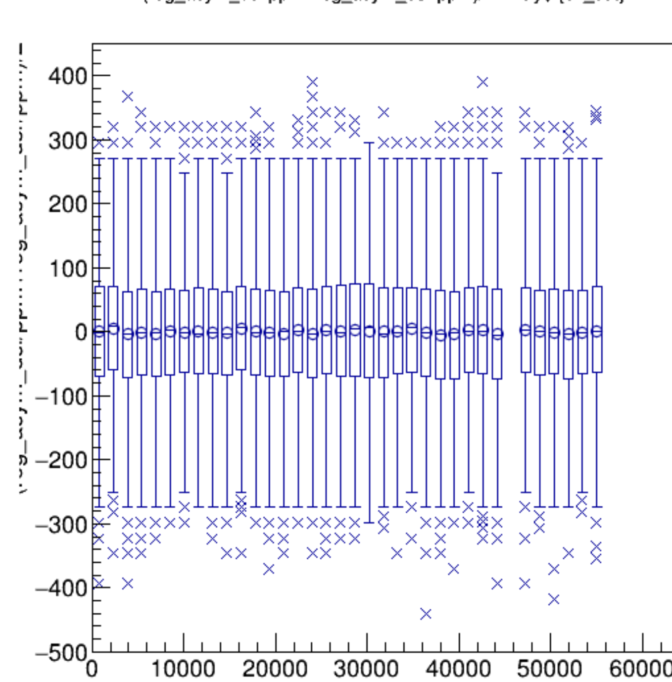
(reg_asym_dsl/ppm+reg_asym_dsr/ppm)/2:Entry$ {ok_cut}
