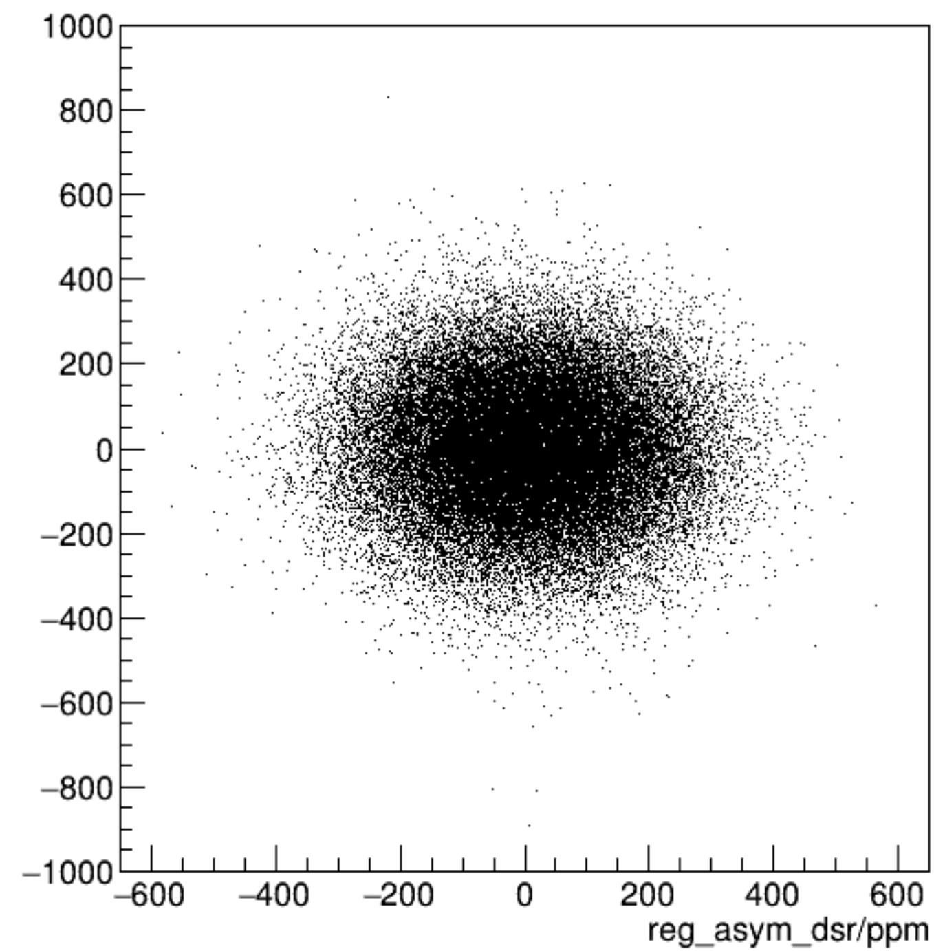
reg_asym_dsl/ppm:reg_asym_dsr/ppm {ok_cut}
