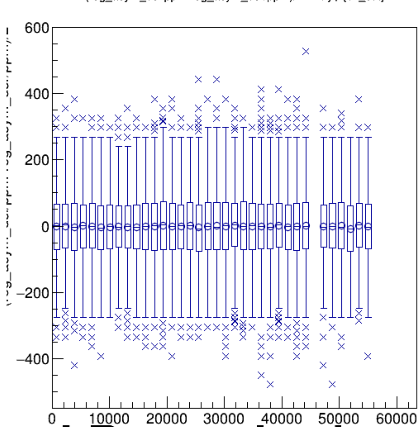
(reg_asym_dsl/ppm-reg_asym_dsr/ppm)/2:Entry$ {ok_cut}
