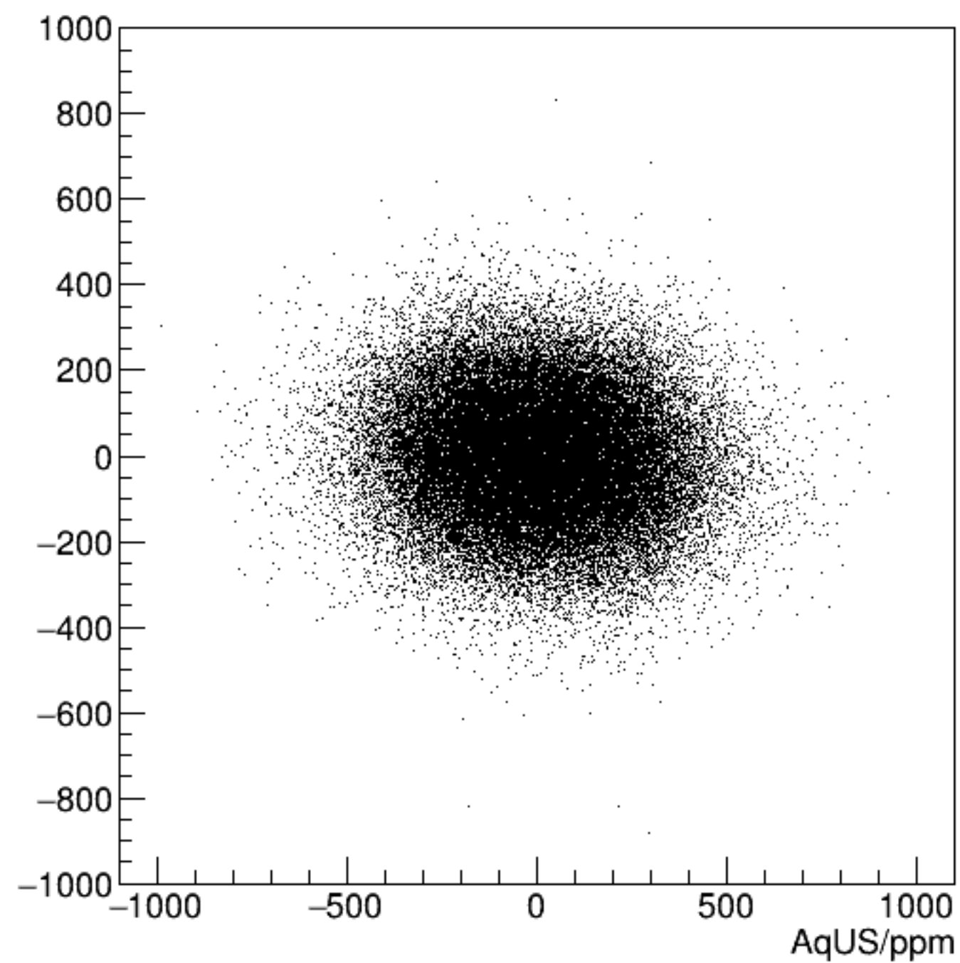
reg_asym_usl/ppm:AqUS/ppm {ok_cut}
