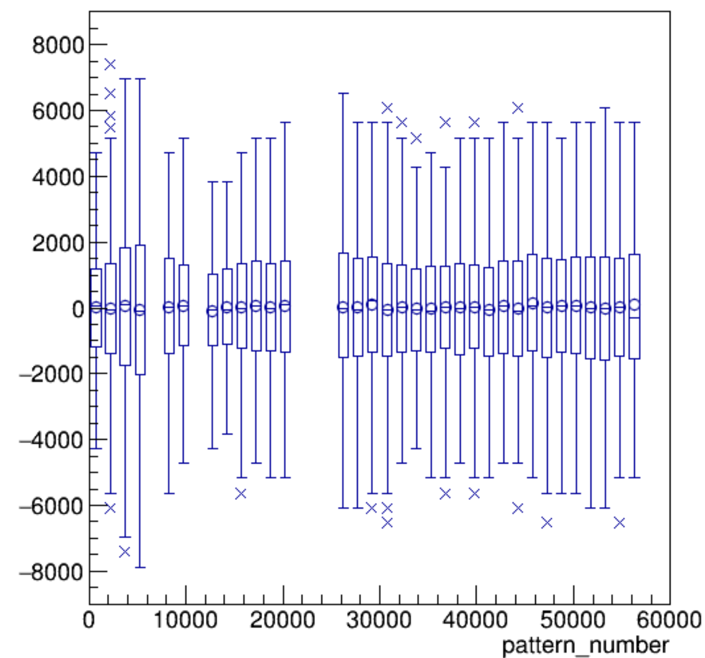
asym_sam6/ppm:pattern_number {ErrorFlag==0}
