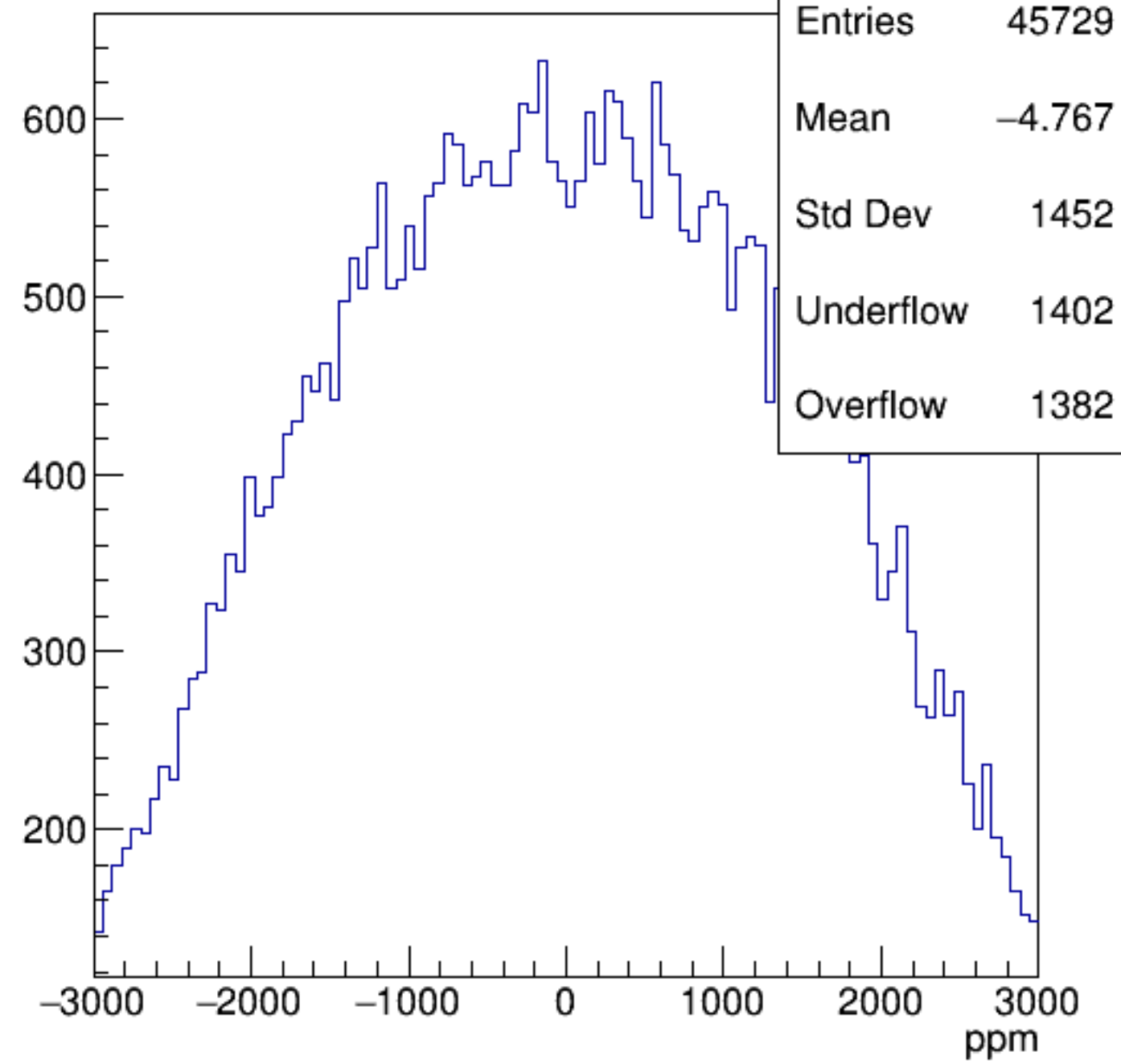
asym_sam7
