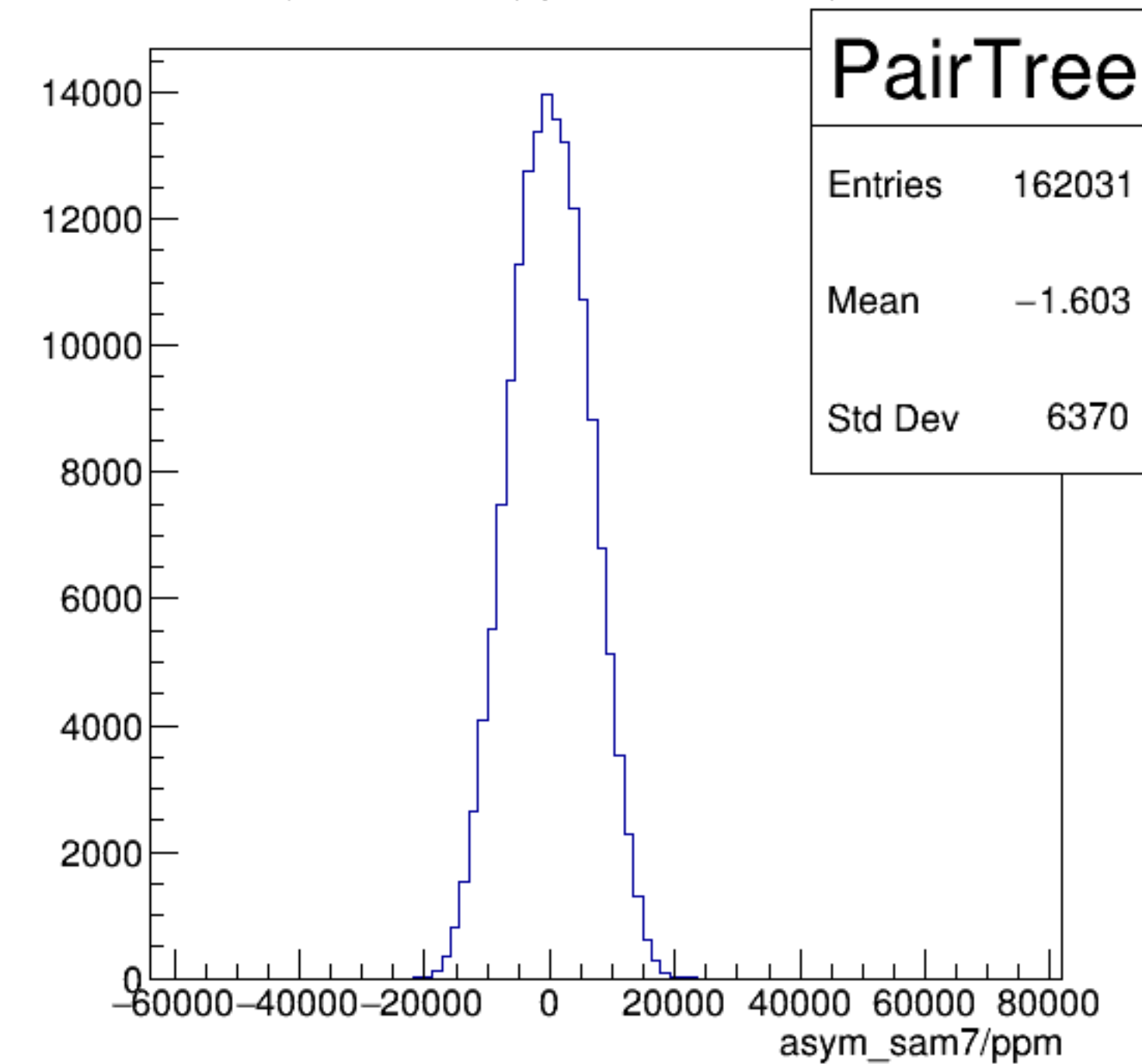
asym_sam7/ppm {ErrorFlag==0}
