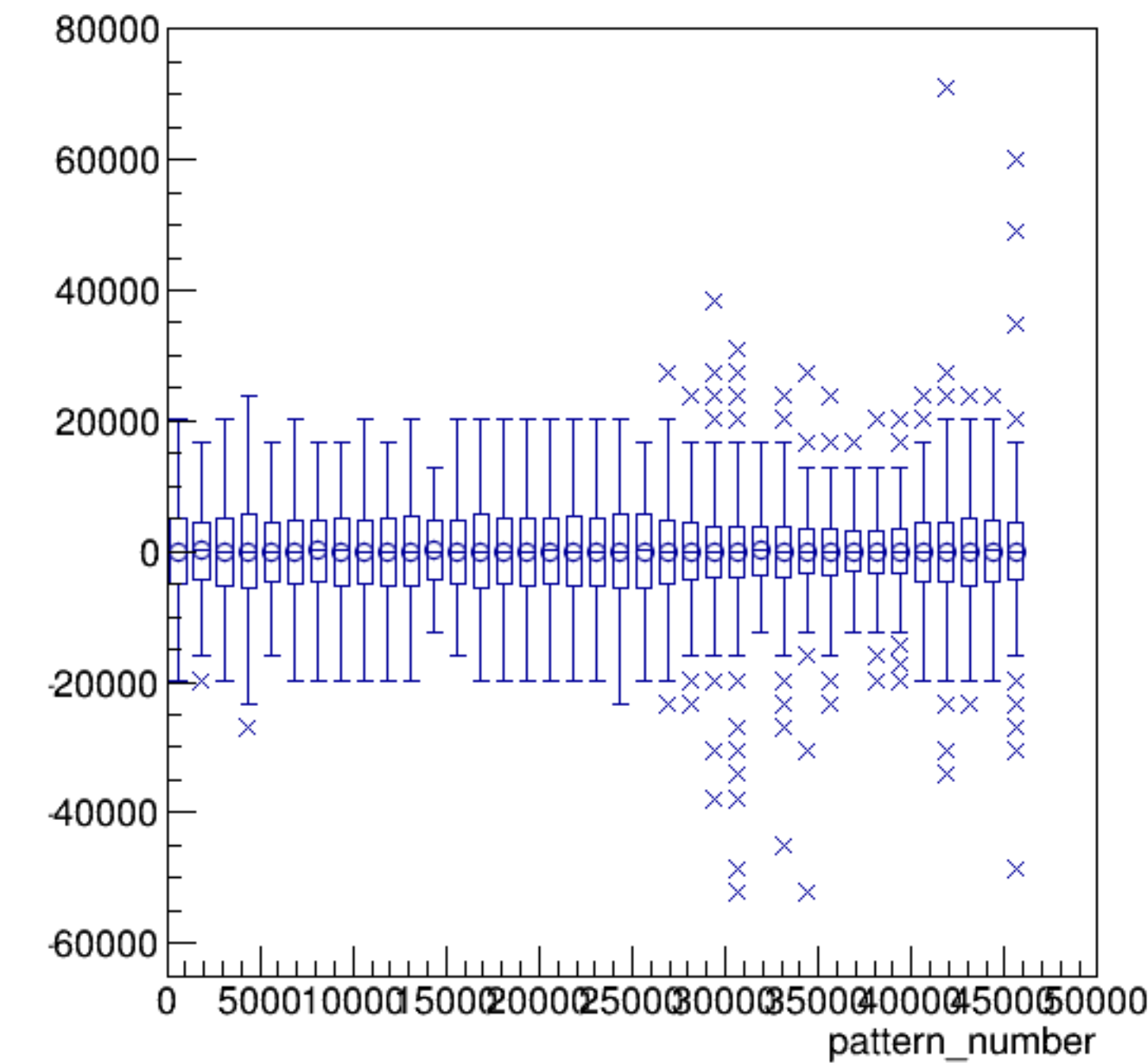
asym_sam7/ppm:pattern_number {ErrorFlag==0}
