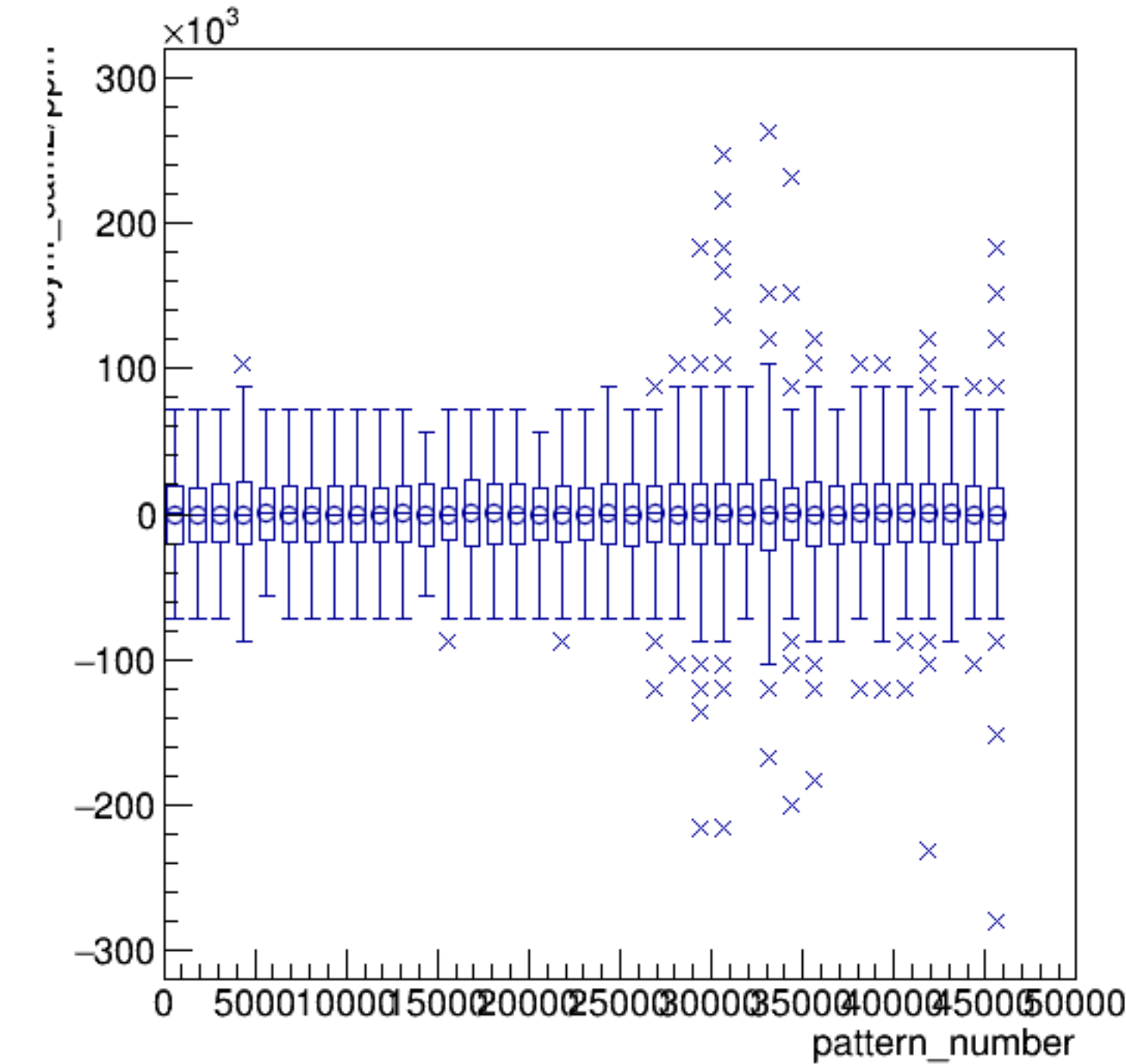
asym_sam2/ppm:pattern_number {ErrorFlag==0}
