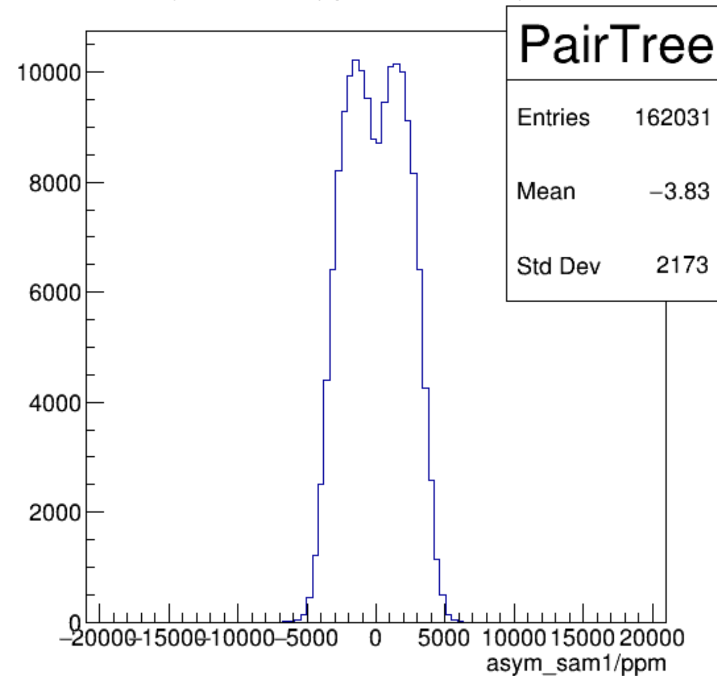
asym_sam1/ppm {ErrorFlag==0}
