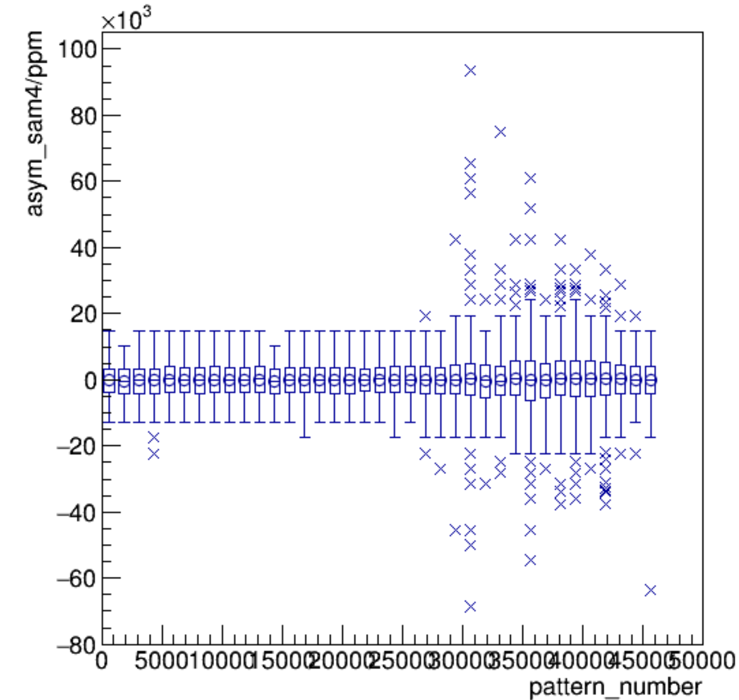
asym_sam4/ppm:pattern_number {ErrorFlag==0}
