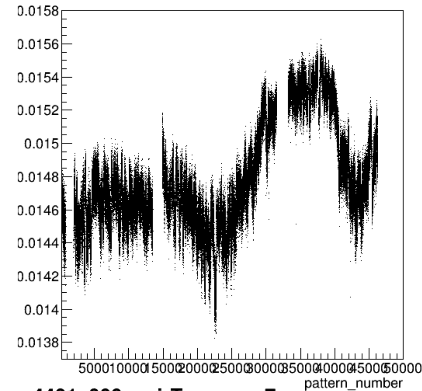
yield_sam7:pattern_number {ErrorFlag==0}
