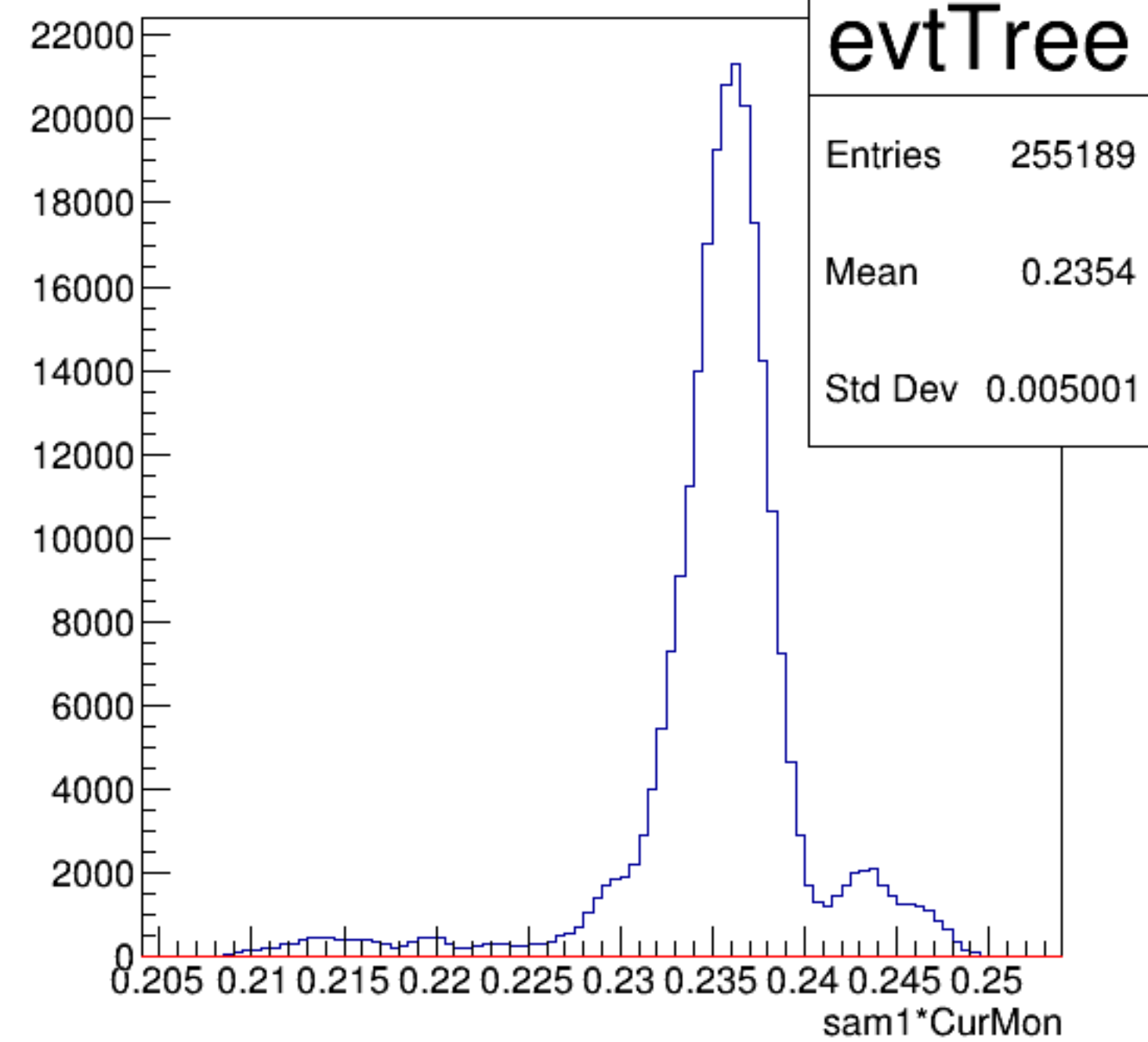
sam1*CurMon {ErrorFlag==0}
