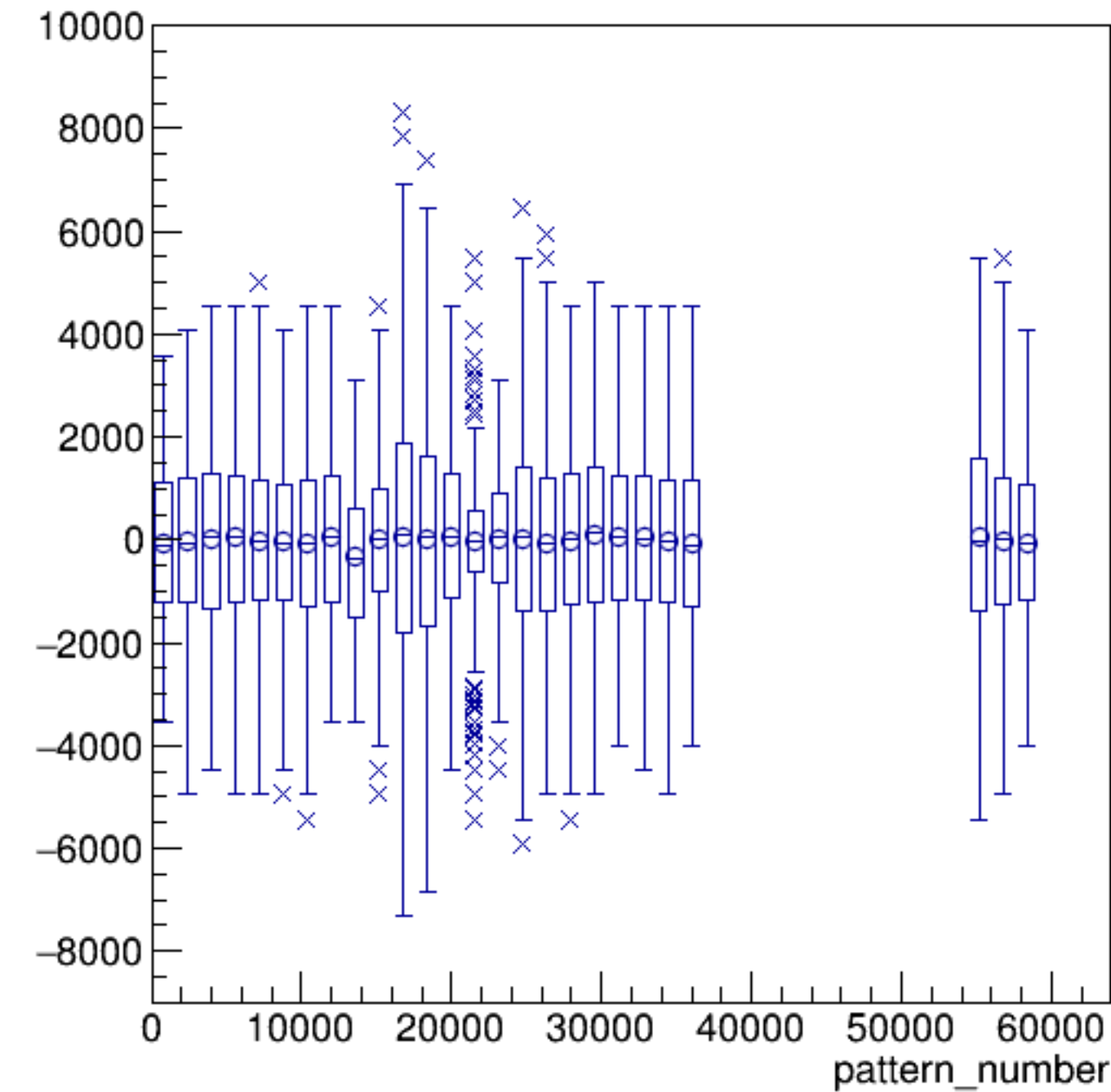
asym_sam7/ppm:pattern_number {ErrorFlag==0}
