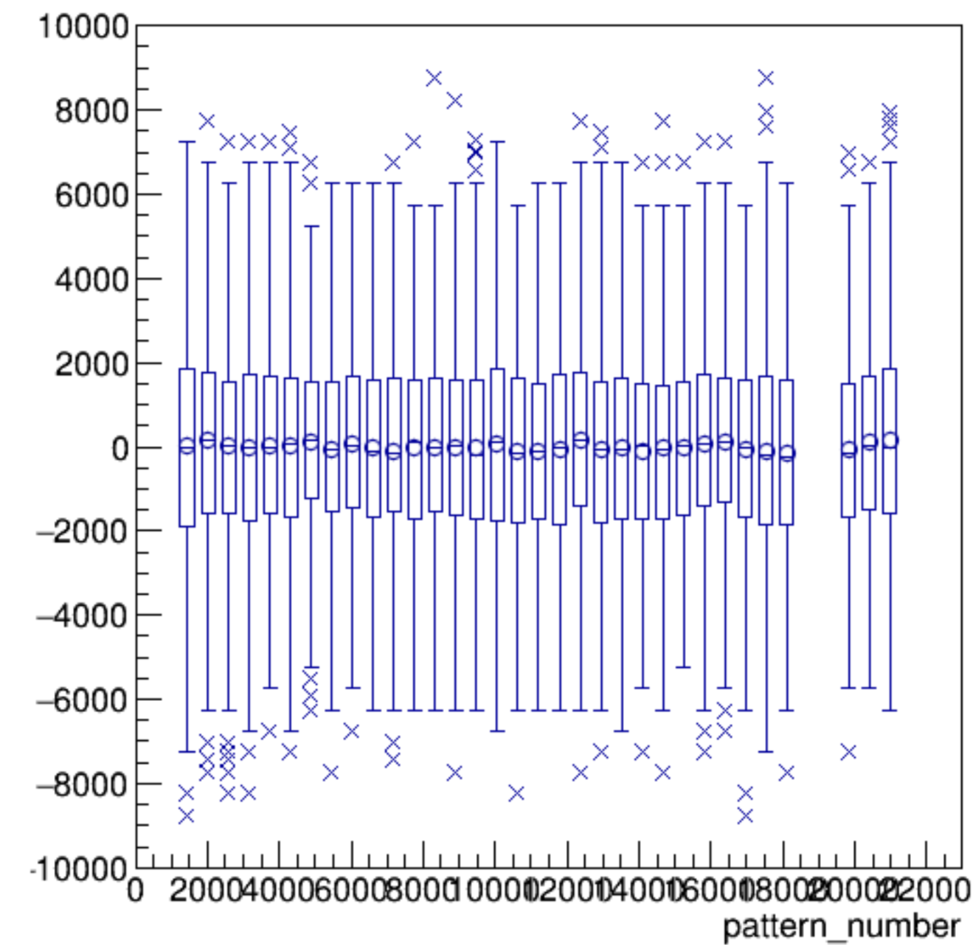
asym_sam7/ppm:pattern_number {ErrorFlag==0}
