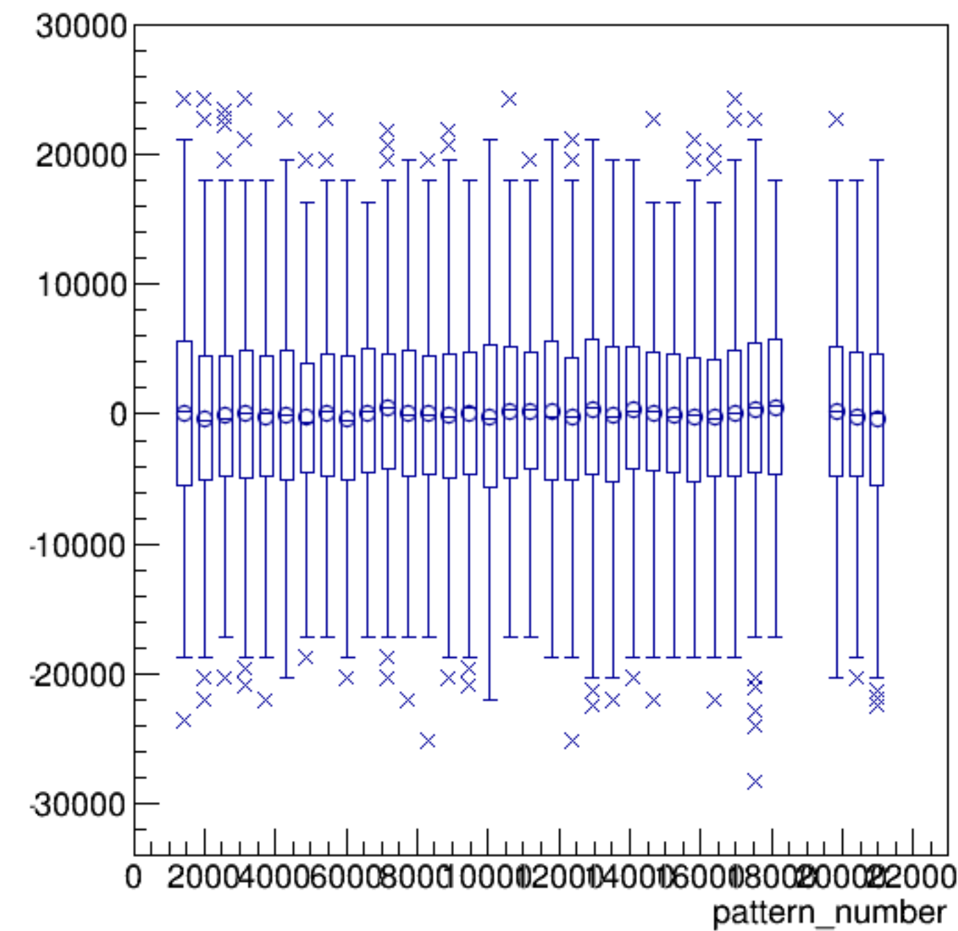
asym_sam2/ppm:pattern_number {ErrorFlag==0}
