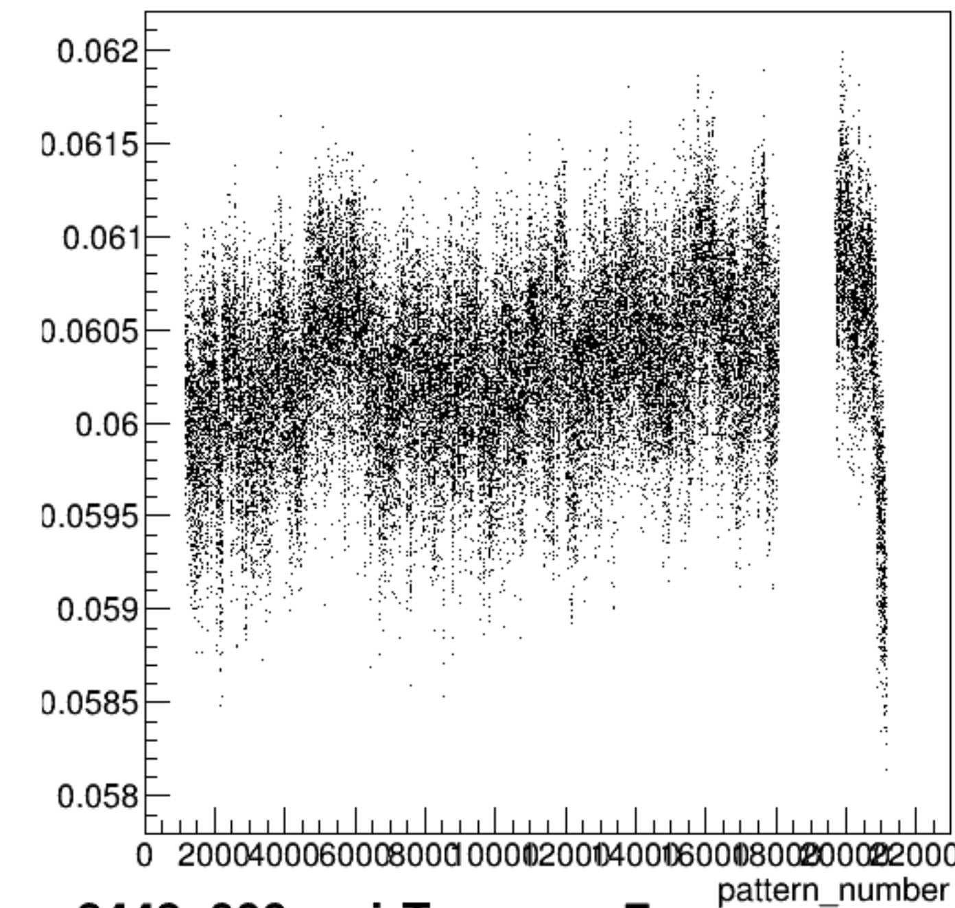
yield_sam7:pattern_number {ErrorFlag==0}
