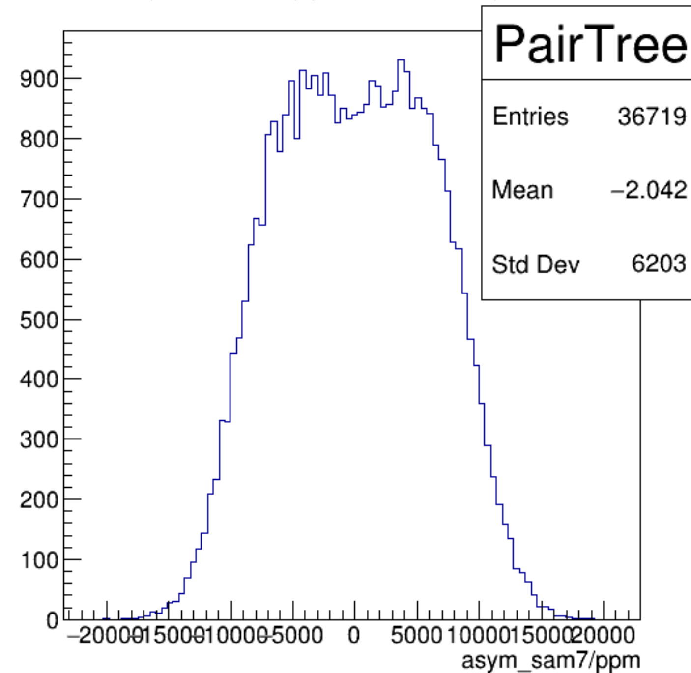
asym_sam7/ppm {ErrorFlag==0}
