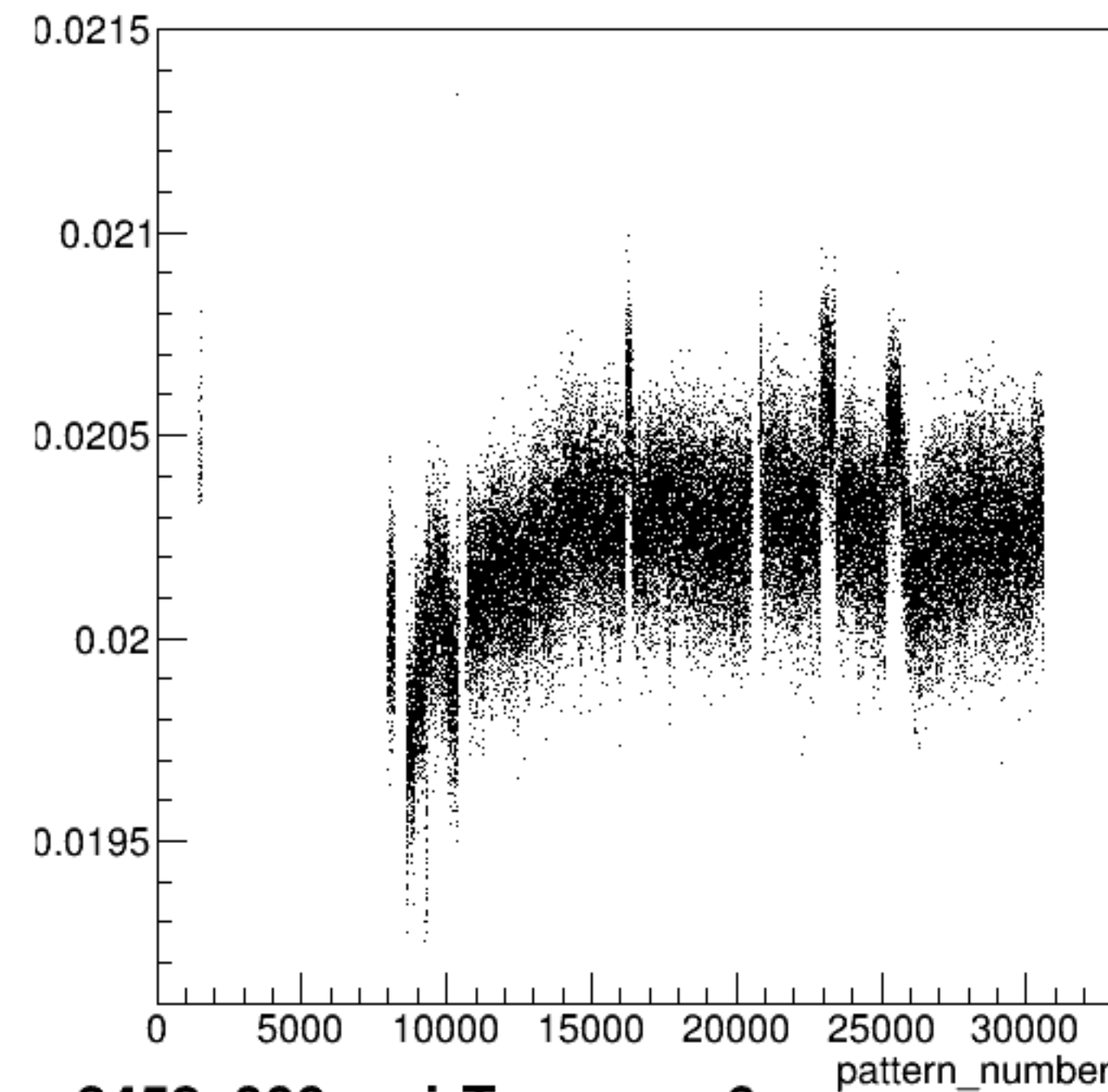
yield_sam6:pattern_number {ErrorFlag==0}
