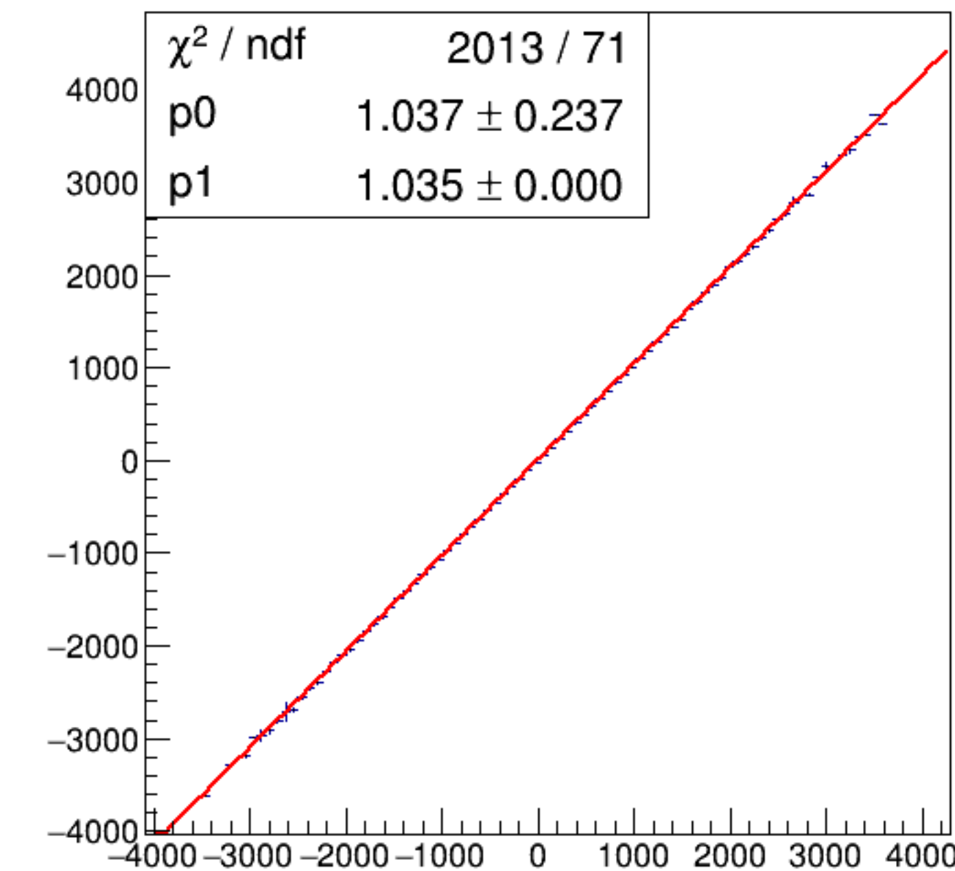
run4471_000_asym_bcm_dg_us_vs_asym_bcm_an_ds3_mul.png
