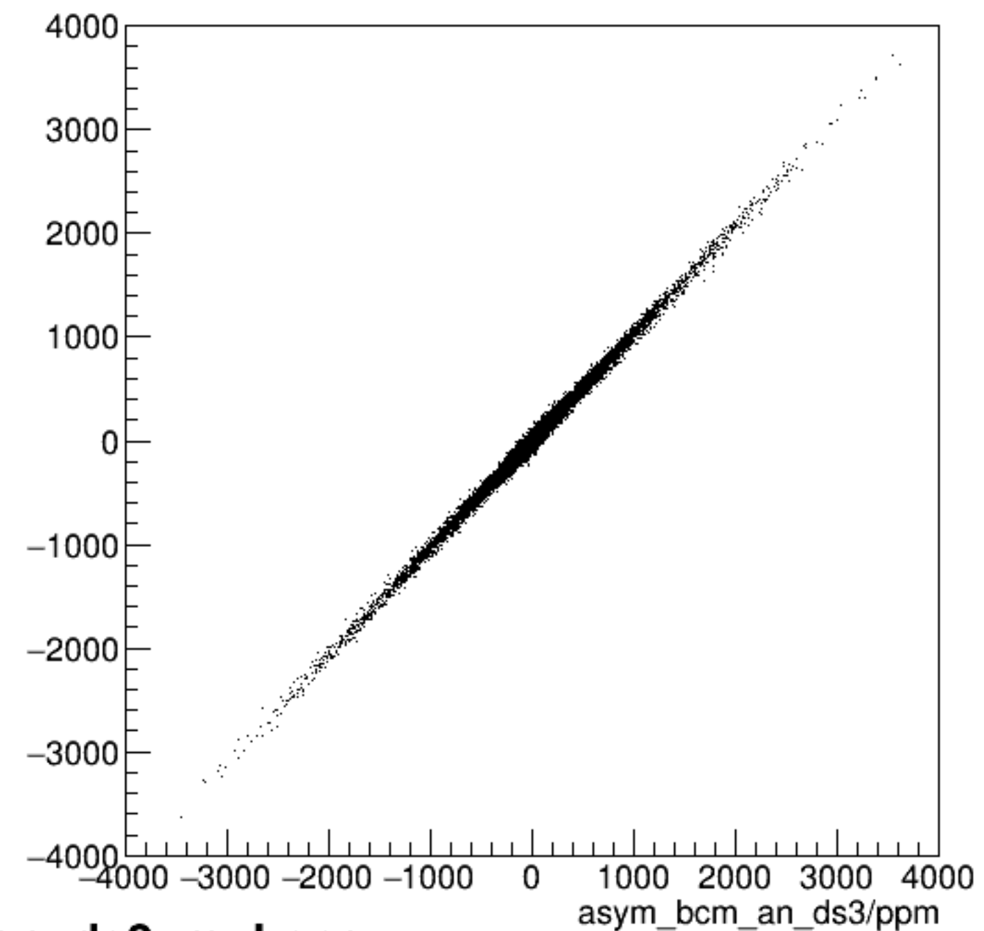
run4471_000_asym_bcm_dg_us_vs_asym_bcm_an_ds3_mul.png
