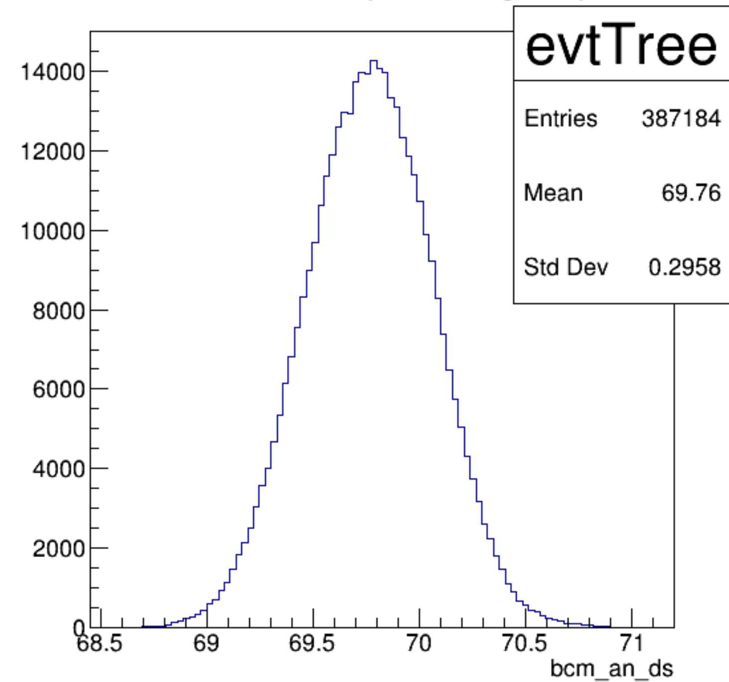
bcm_an_ds {ErrorFlag==0}
