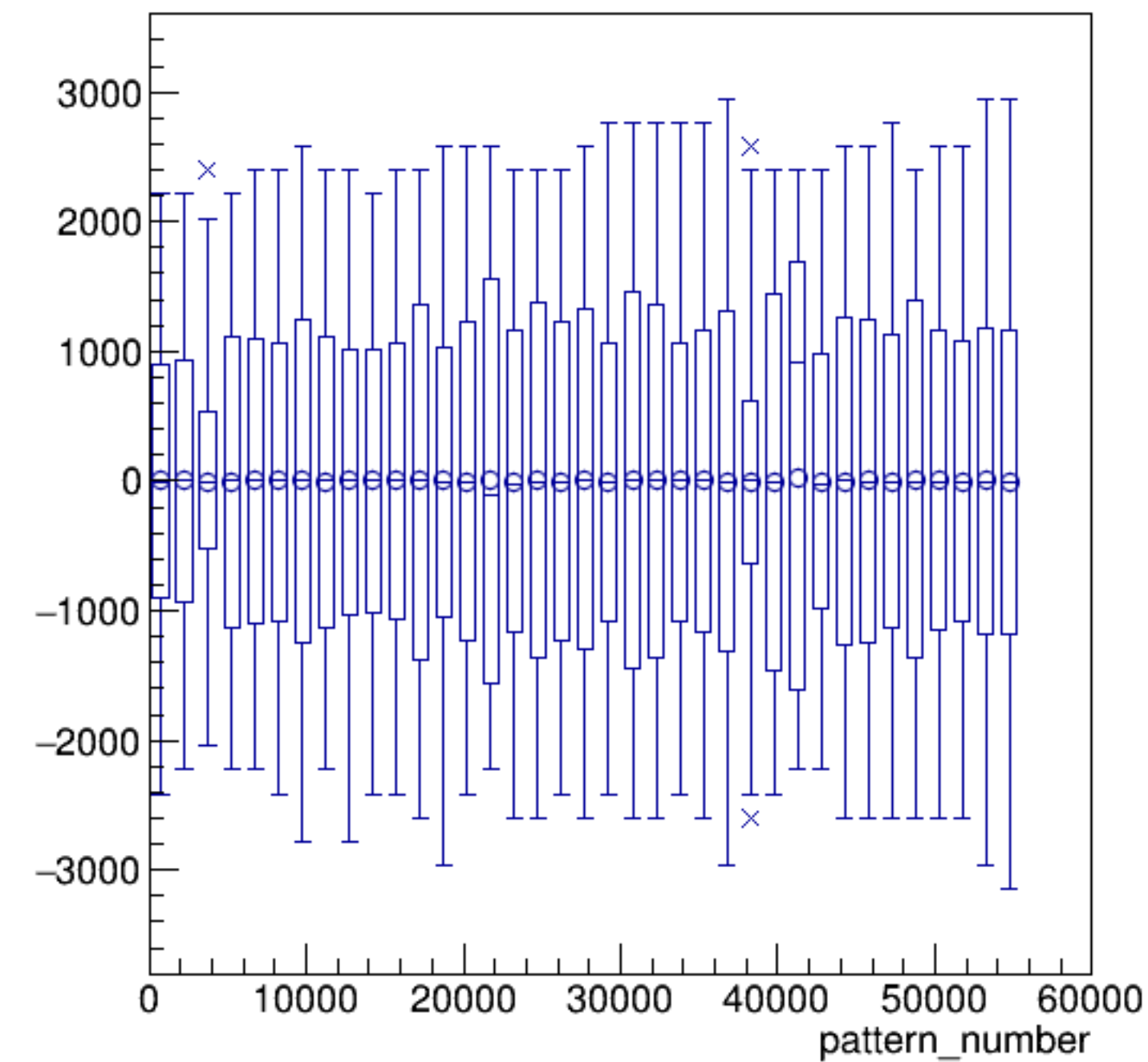
asym_bcm_dg_us/ppm:pattern_number {ErrorFlag==0}
