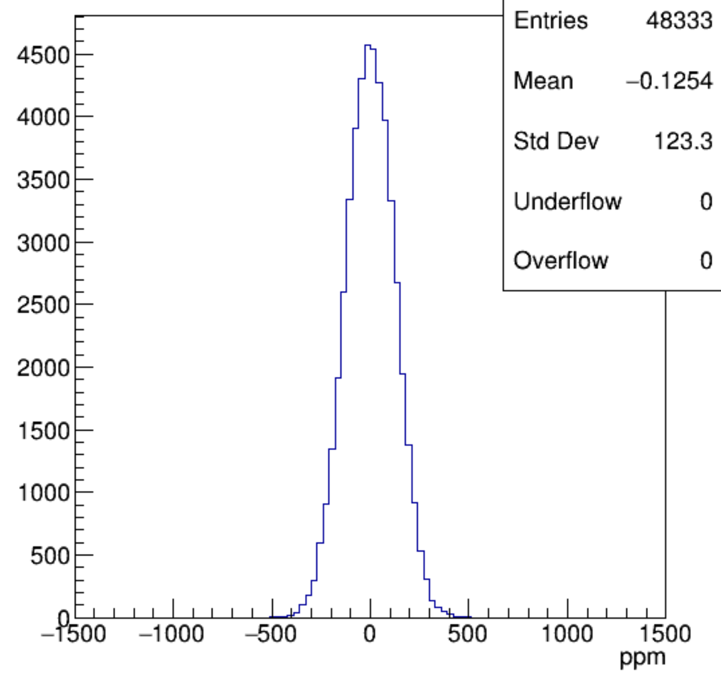
asym_bcm_dg_ds
