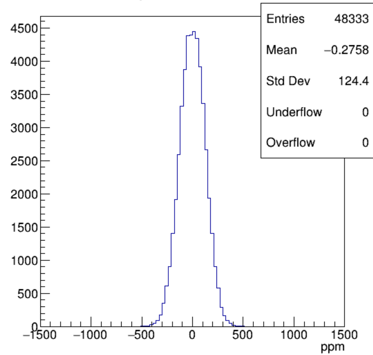
asym_bcm_an_ds
