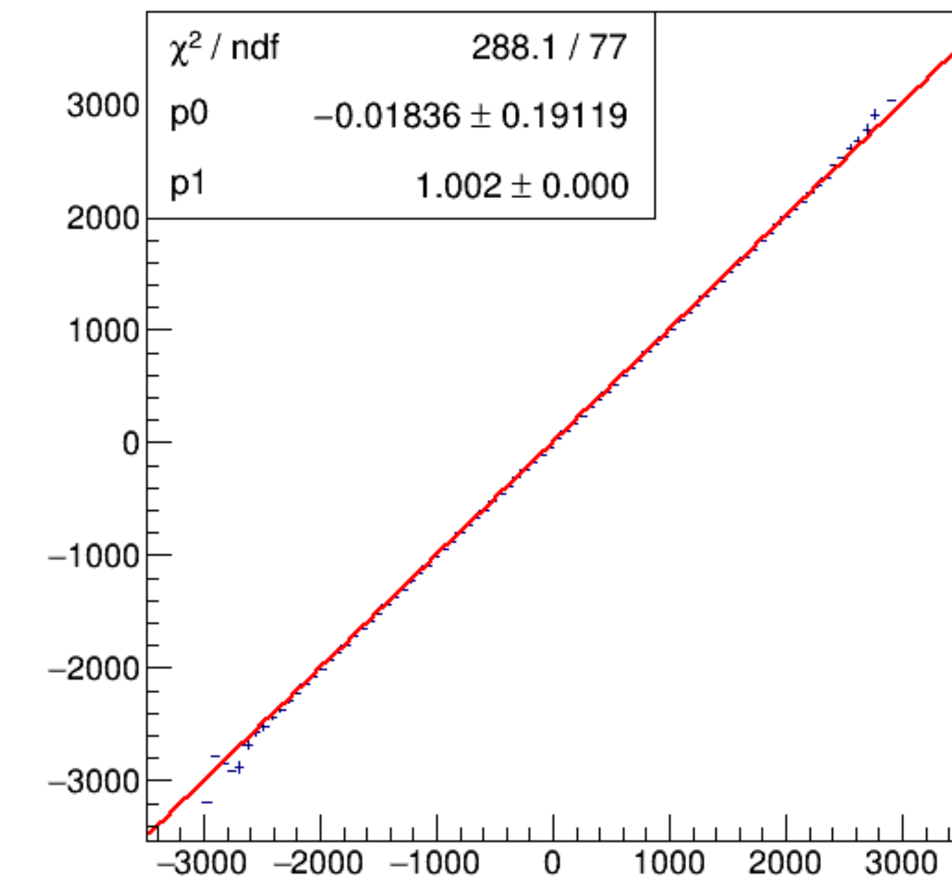
run4474_000_asym_bcm_dg_us_vs_asym_bcm_an_ds3_pr.png
