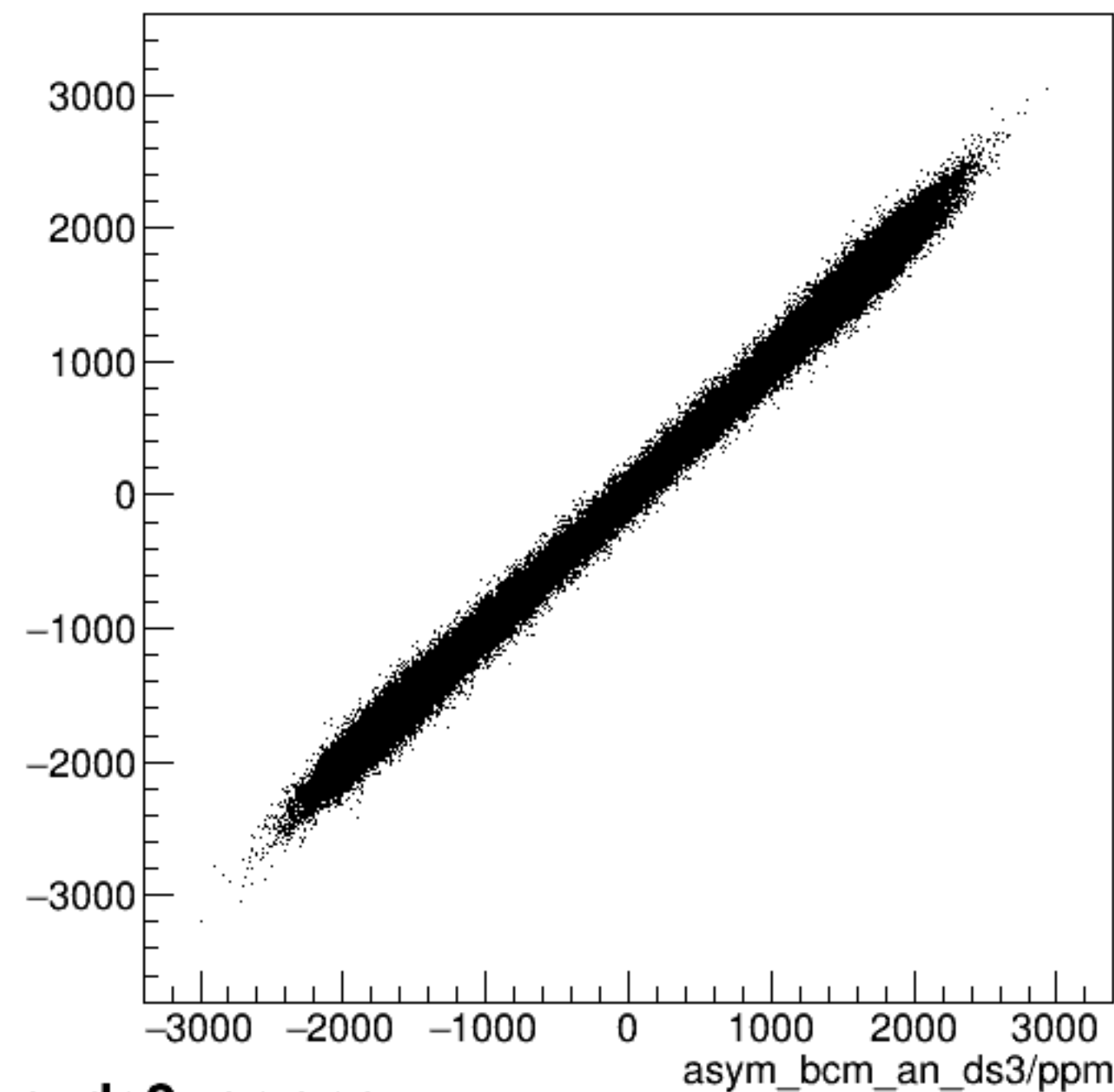
run4474_000_asym_bcm_dg_us_vs_asym_bcm_an_ds3_pr.png
