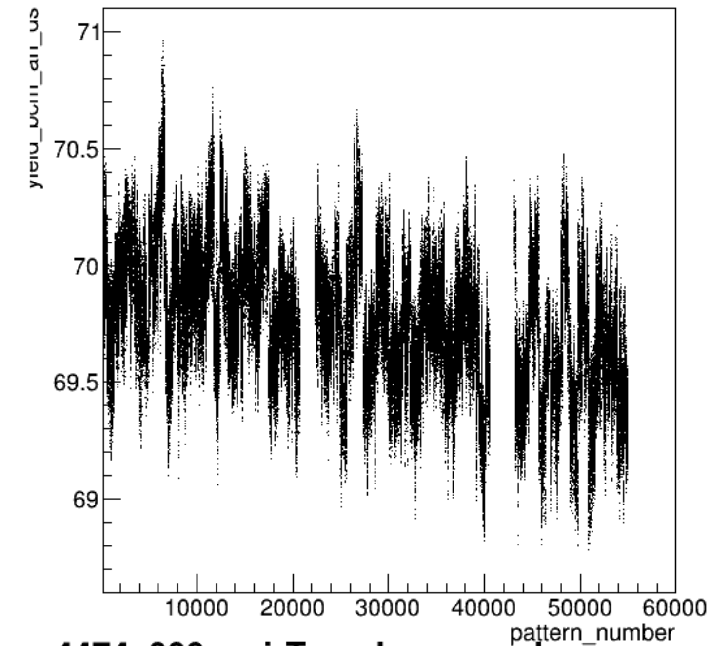
yield_bcm_an_ds:pattern_number {ErrorFlag==0}
