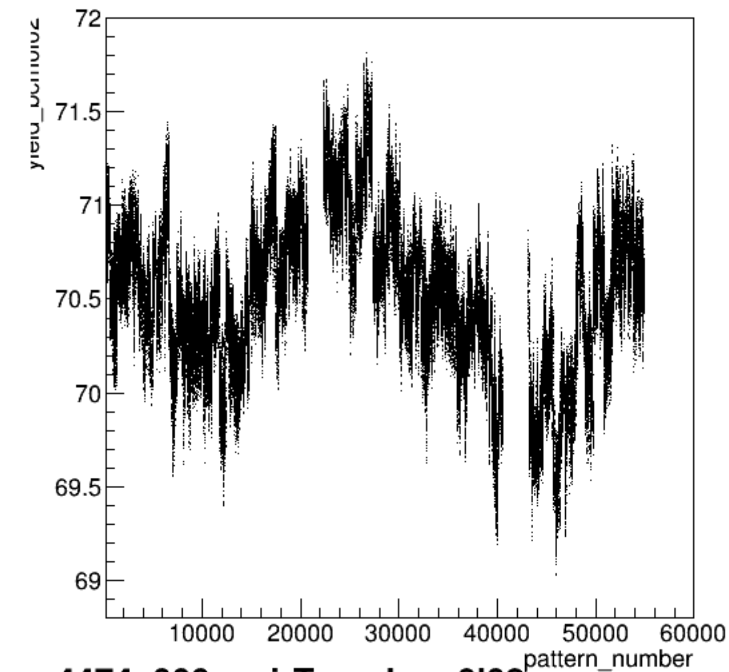
yield_bcm0l02:pattern_number {ErrorFlag==0}
