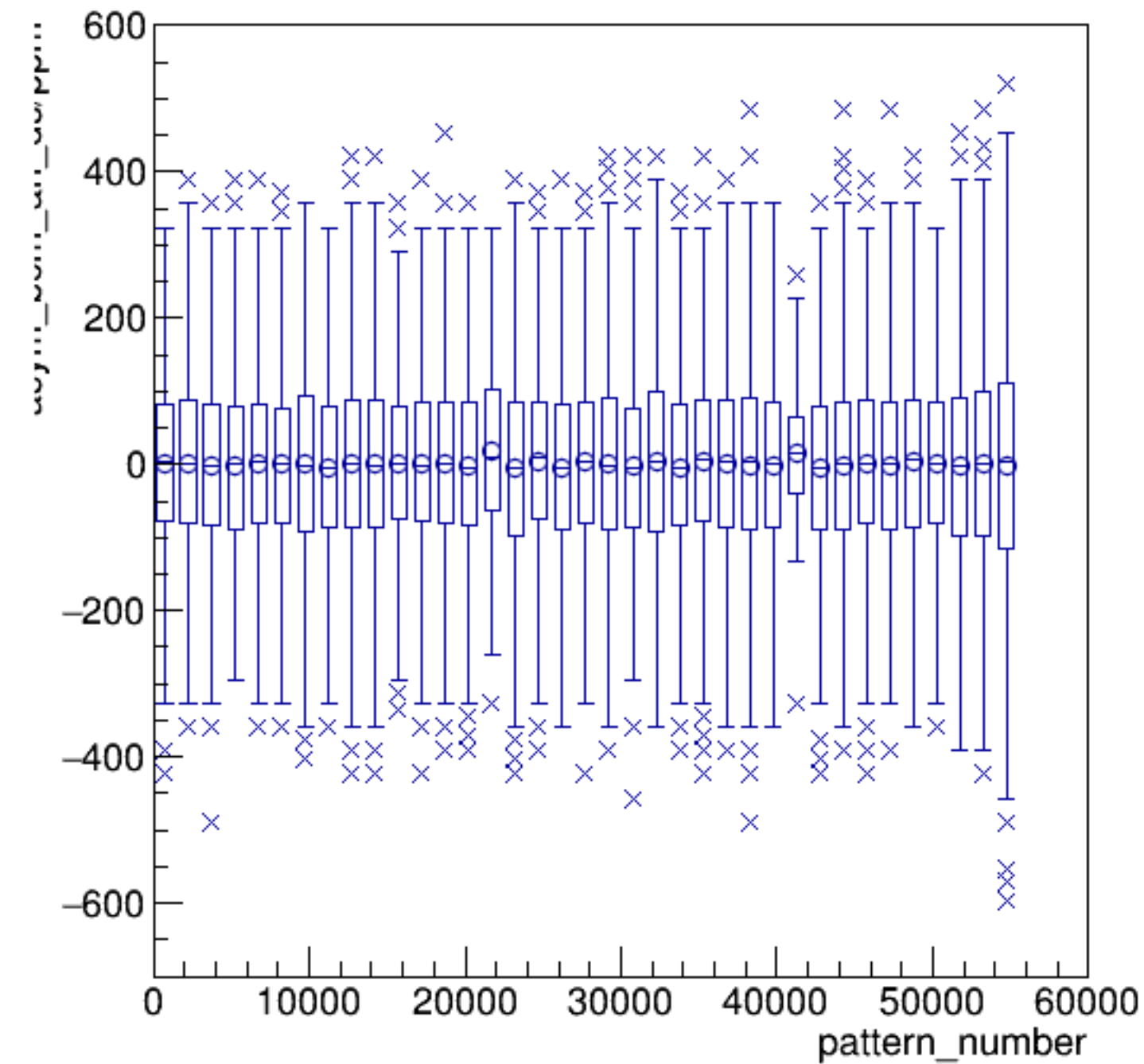
asym_bcm_an_ds/ppm:pattern_number {ErrorFlag==0}
