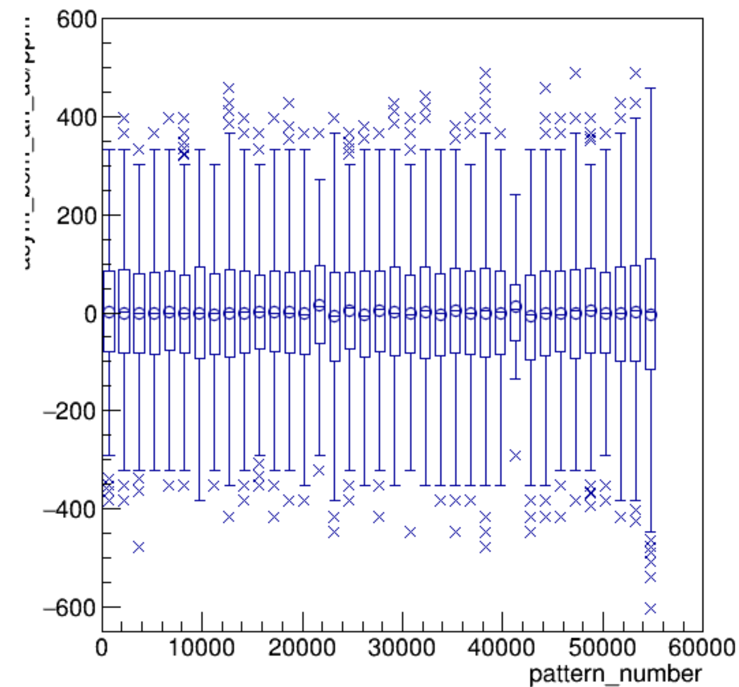
asym_bcm_an_us/ppm:pattern_number {ErrorFlag==0}
