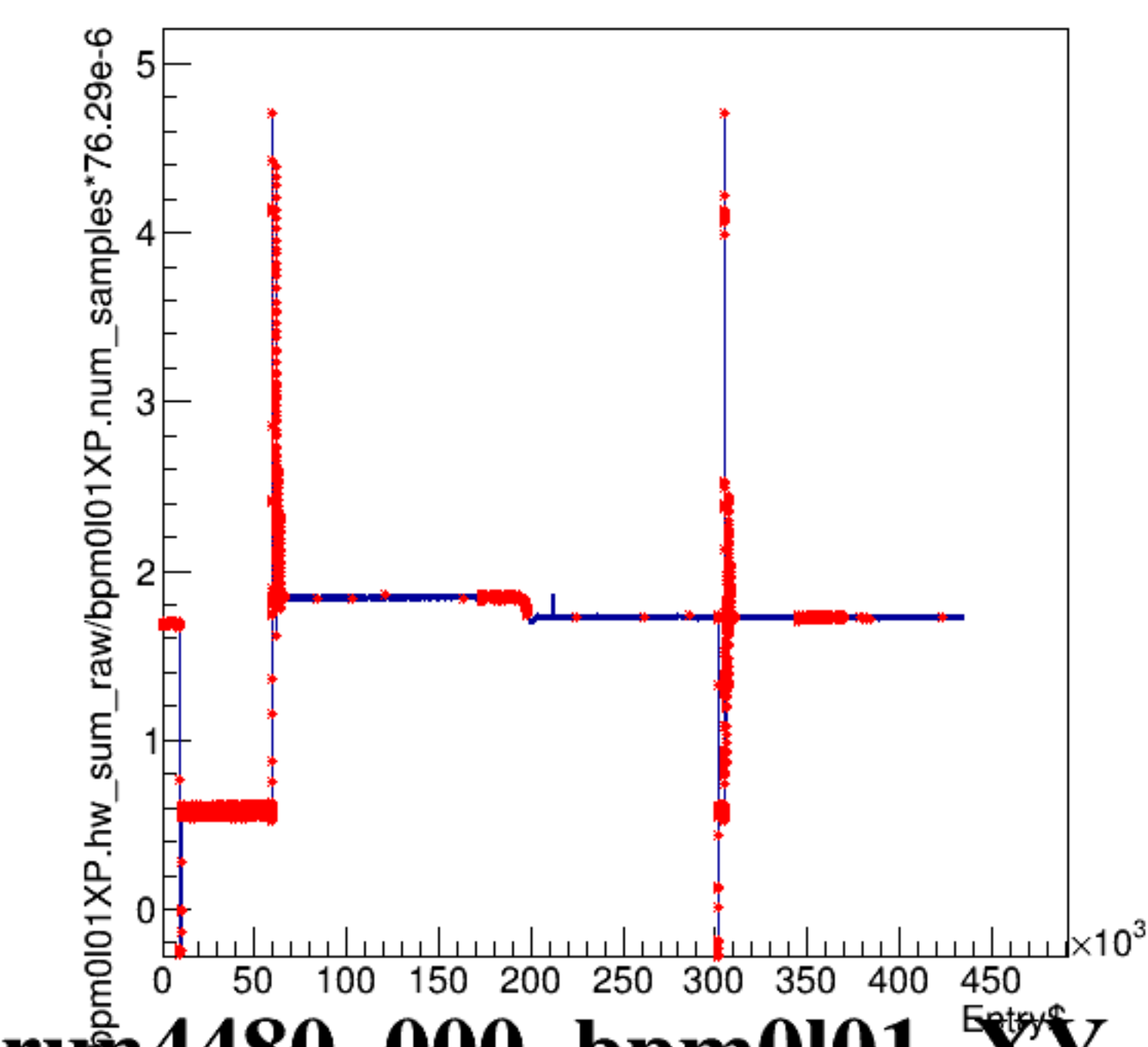
bpm0l01XP.hw_sum_raw/bpm0l01XP.num_samples*76.29e-6:Entry$
