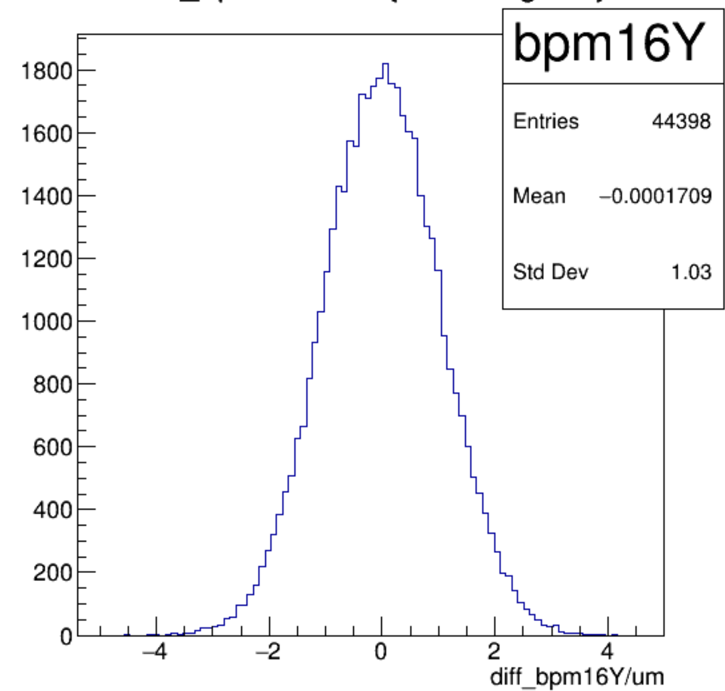
diff_bpm16Y/um {ErrorFlag==0}
