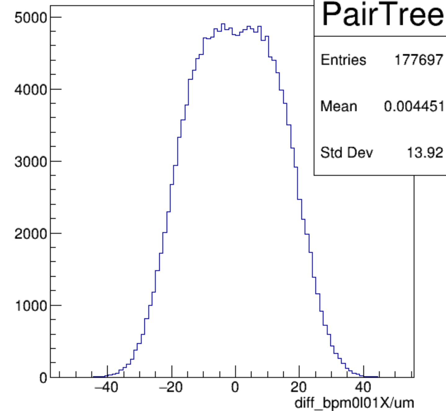
diff_bpm0l01X/um {ErrorFlag==0}
