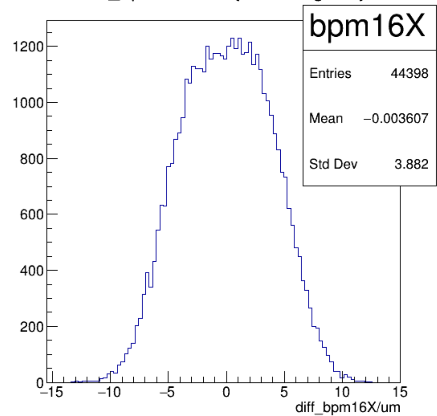
diff_bpm16X/um {ErrorFlag==0}
