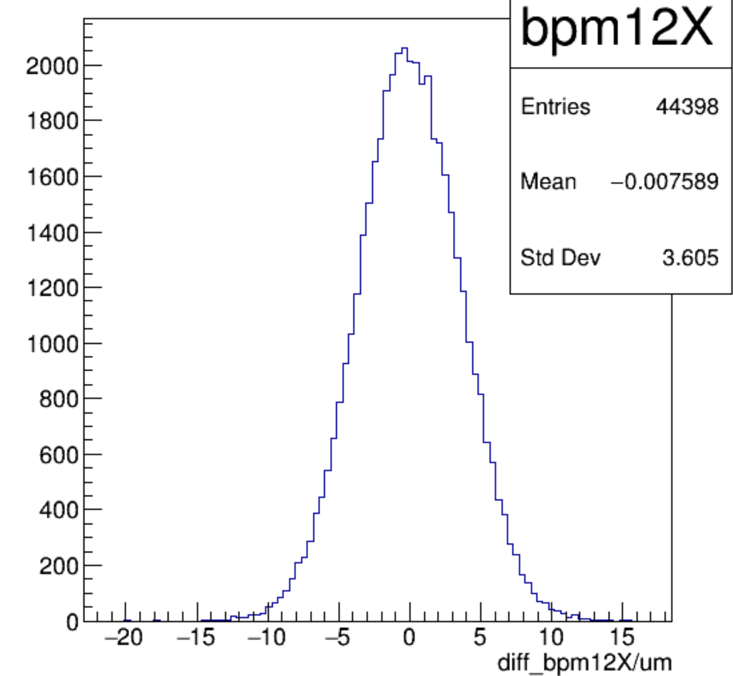
diff_bpm12X/um {ErrorFlag==0}
